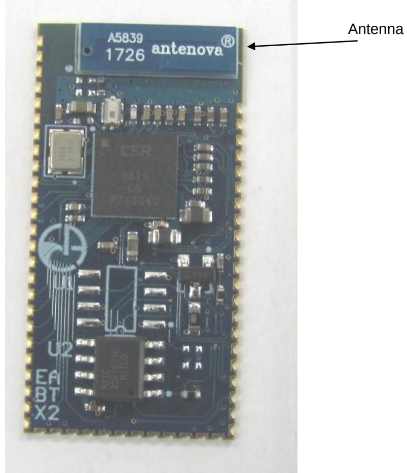
Photograph of PC Board: Component Side
