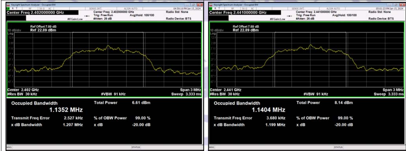
8DPSK_3-DH1_Channel 0
