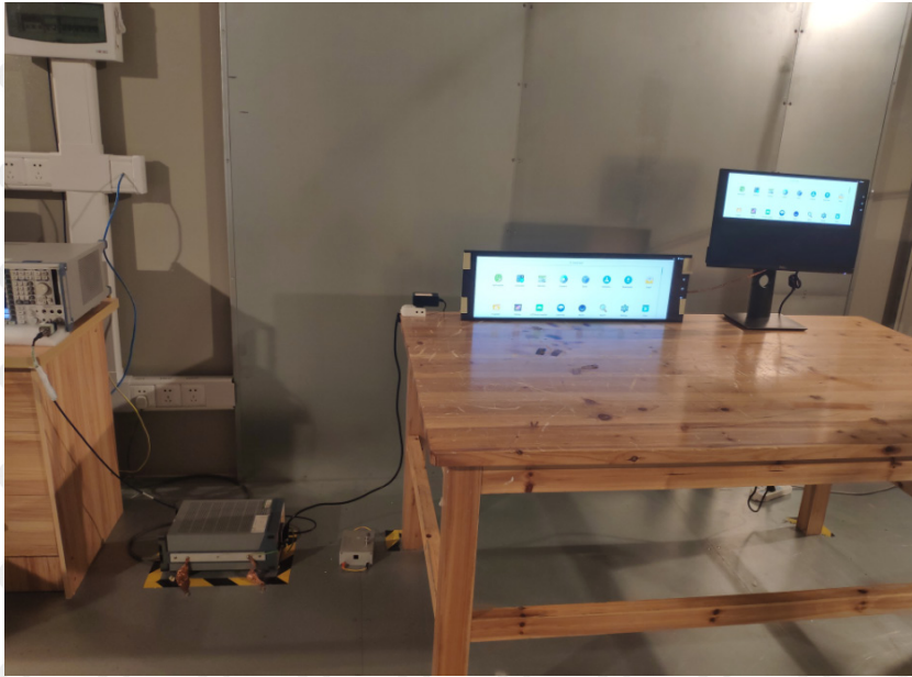
Photograph of test setup for Conducted Emission
