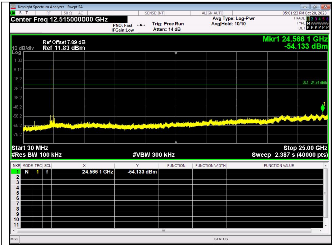
Spurious Emission Channel 0
