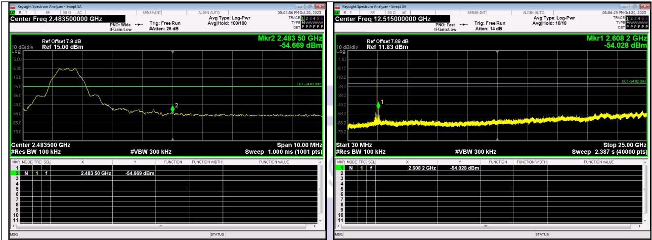
Out Of Band Emission Channel 39
