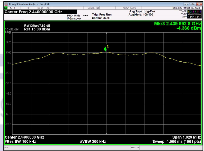
In-Band Reference Level Channel 19
