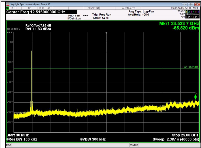
Spurious Emissions Channel 19
