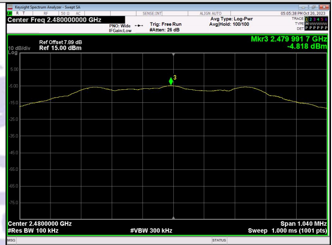
In-Band Reference Level Channel 39
