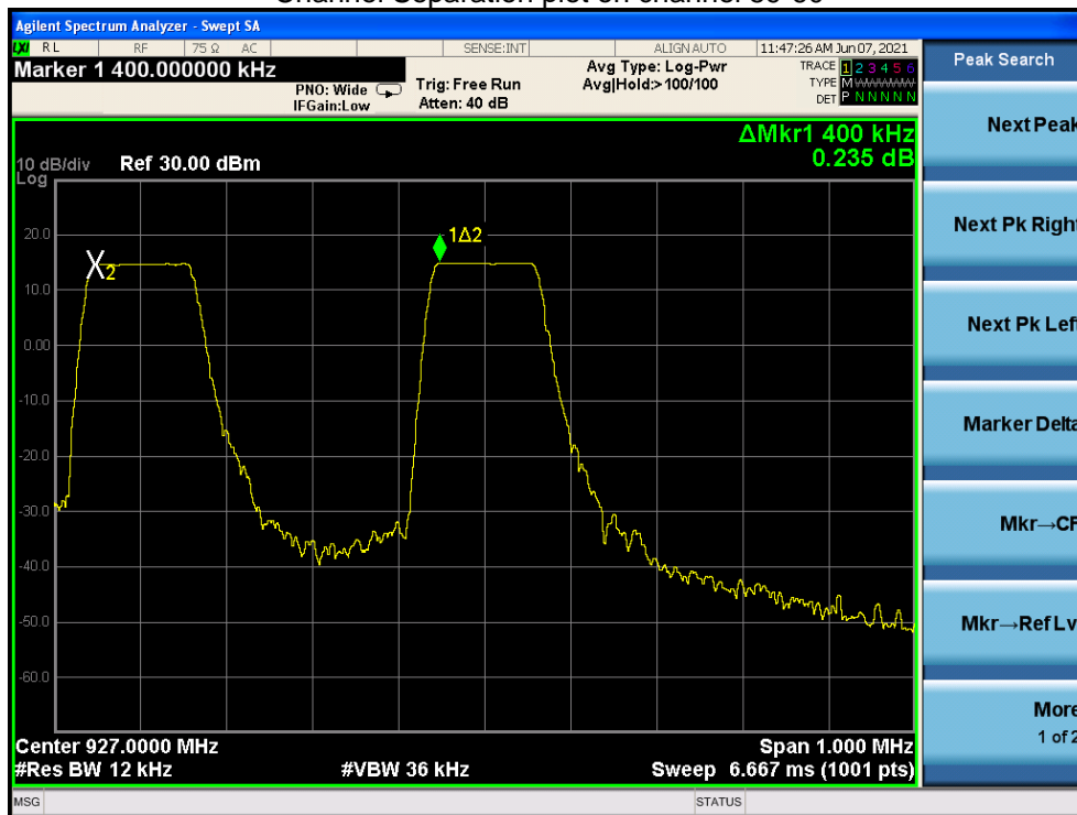
Channel Separation plot on channel 59-60
