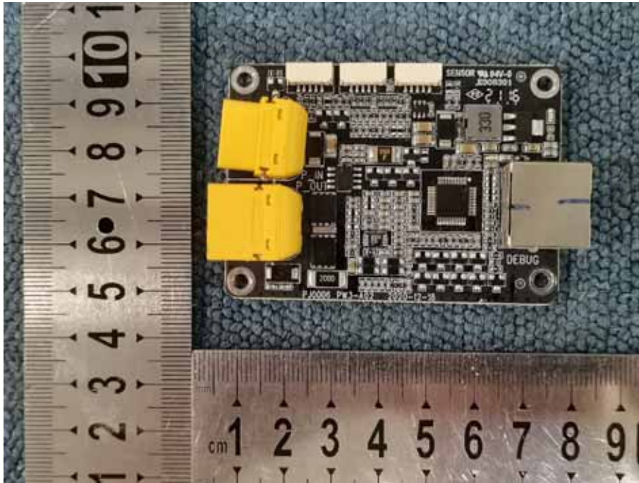
Accessory - PUDU Charging Pile(MAIN BOARD TOP VIEW)
