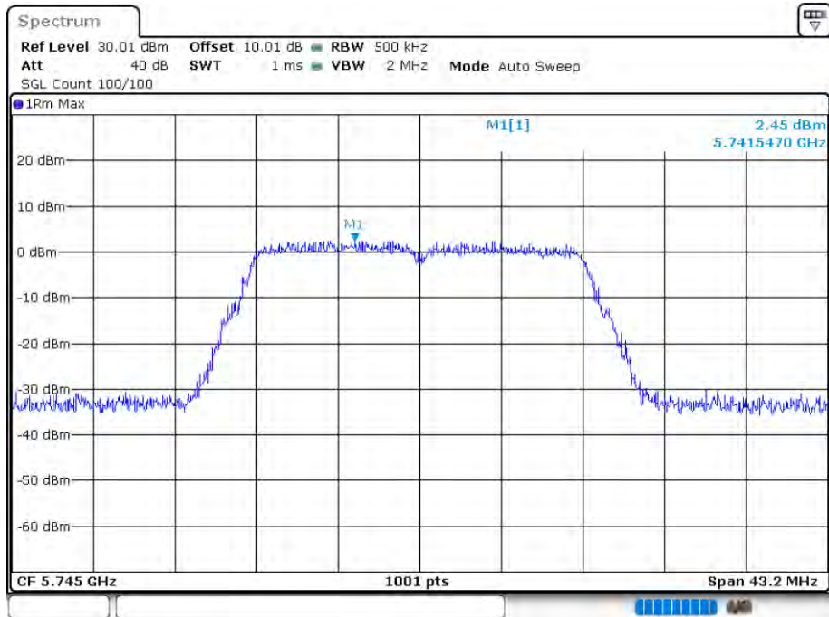
PSD NVNT 802.11ac20 5745MHz Ant 2
