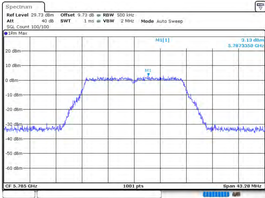
PSD NVNT 802.11a 5785MHz Ant 2
