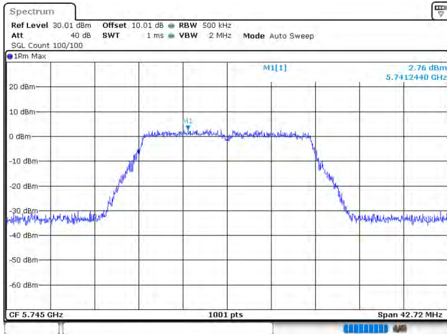
PSD NVNT 802.11a 5745MHz Ant 2
