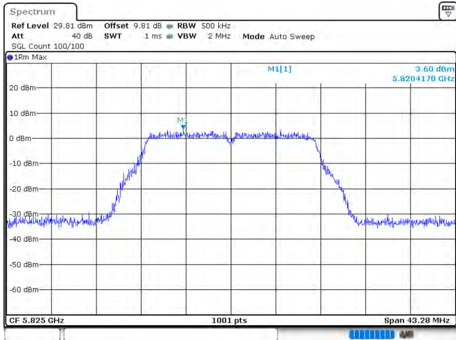
PSD NVNT 802.11a 5825MHz Ant 2
