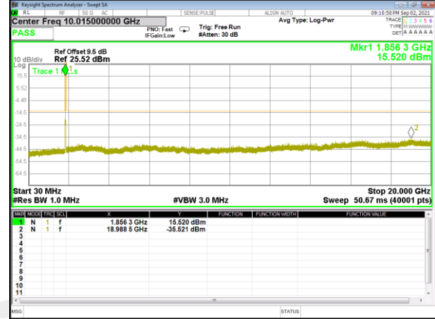
Band 2_15M_16QAM_Middle
