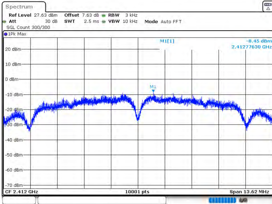
PSD NVNT 802.11b 2412MHz Ant3
