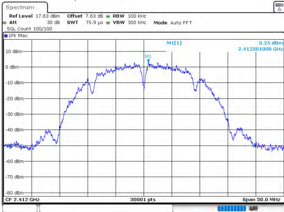
Tx. Spurious NVNT 802.11b 2412MHz Ant3 Ref
