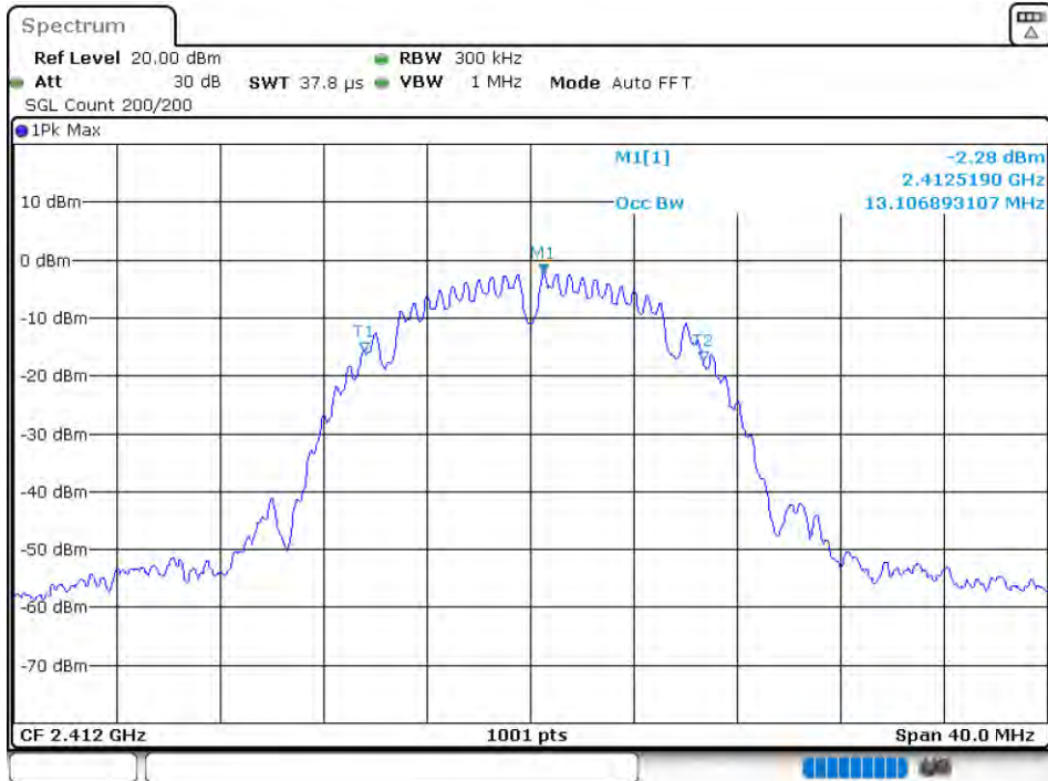
OBW NVNT 802.11b 2412MHz Ant3
