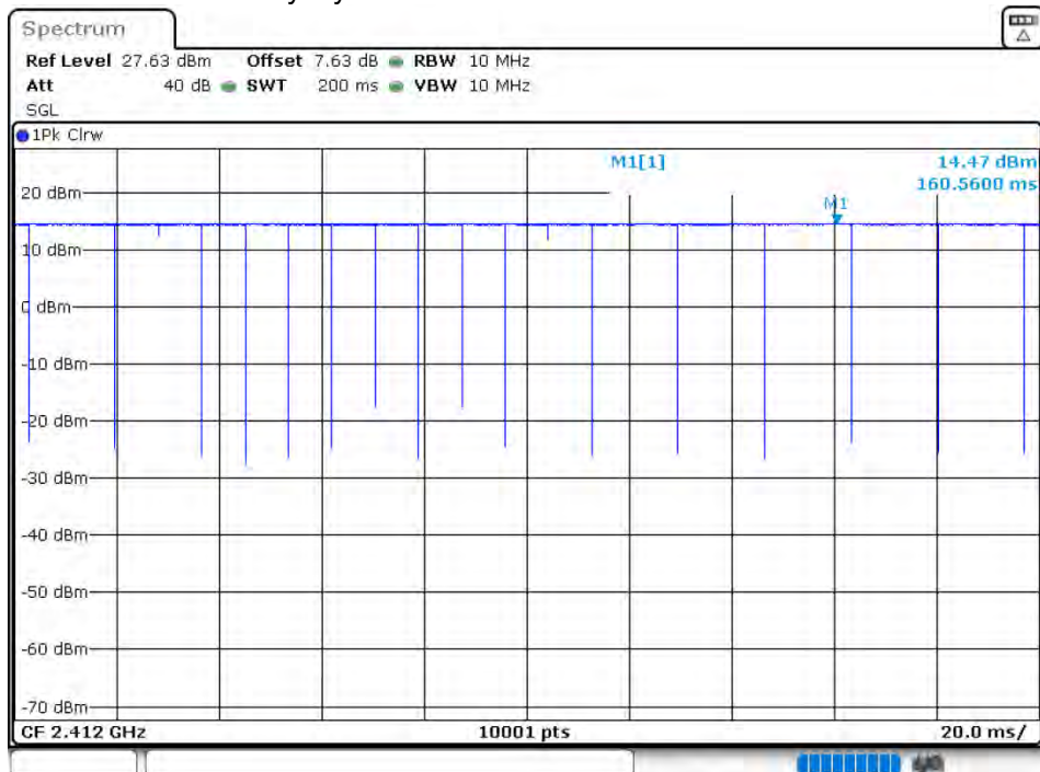
Duty Cycle NVHT 802.11b 2412MHz Ant 1
