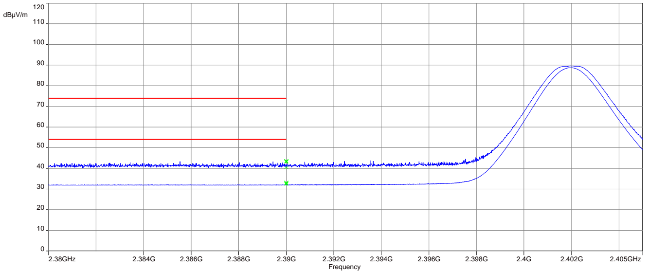
Plot 1: Lower restricted band, 1 Mbit/s
