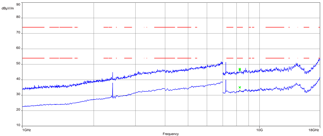
Plot 4: 1 GHz to 18 GHz, TX mode, 2402 MHz, vertical & horizontal polarization, 2 Mbit/s
