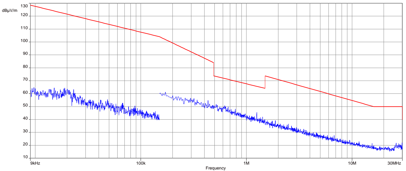
Plot 2: 9 kHz to 30 MHz, 2440 MHz, transmit mode, 1 Mbit/s
