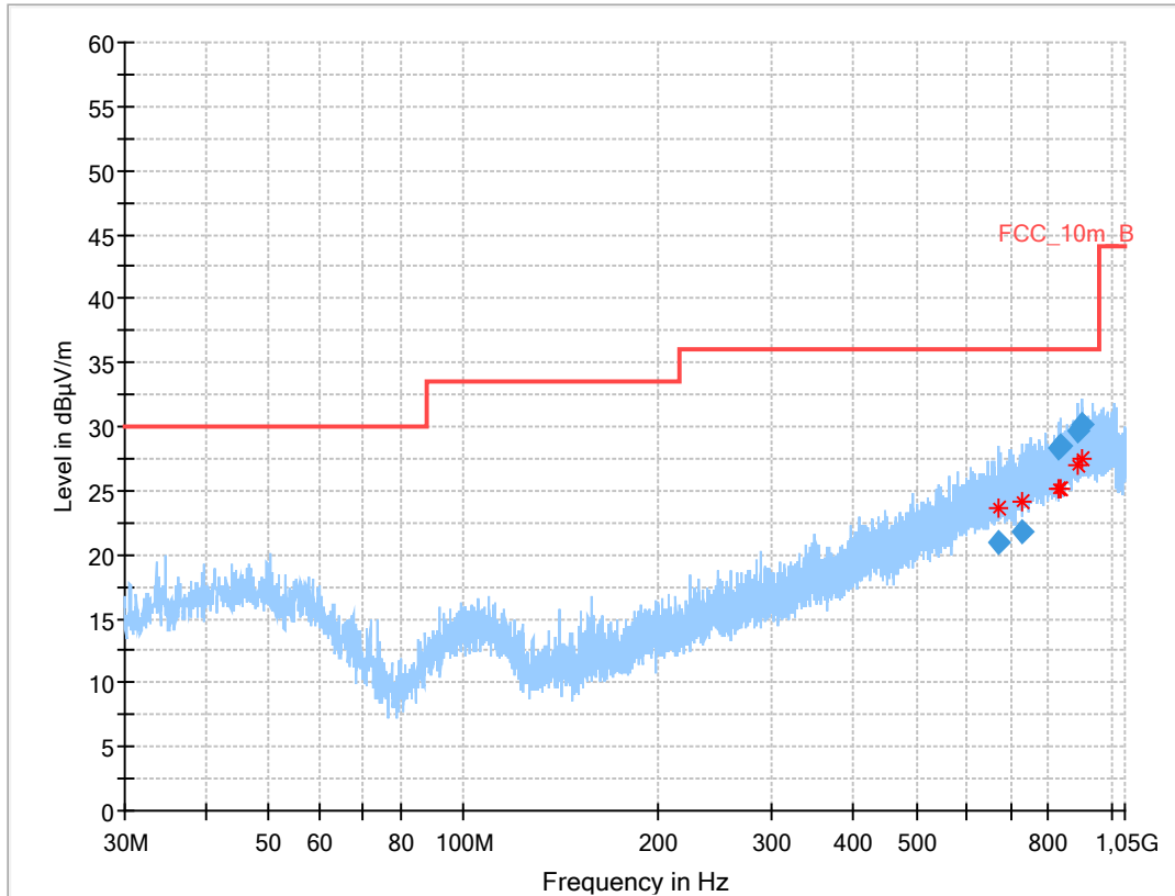
Plot 2: 30 MHz to 1 GHz, TX mode, vertical & horizontal polarization, valid for all channels of 2 Mbit/s
