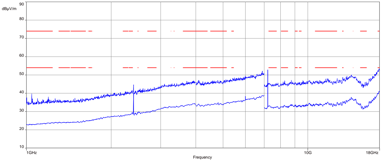
Plot 1: 1 GHz to 18 GHz, TX mode, 2402 MHz, vertical & horizontal polarization, 1 Mbit/s
