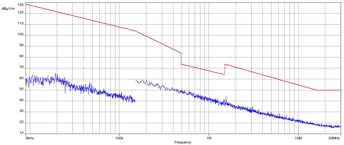
Plot 6: 9 kHz to 30 MHz, 2480 MHz, transmit mode, 2 Mbit/s
