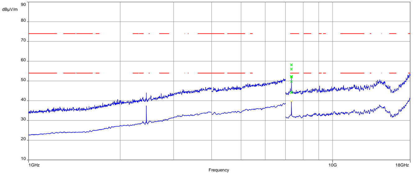
Plot 5: 1 GHz to 18 GHz, TX mode, 2440 MHz, vertical & horizontal polarization, 2 Mbit/s
