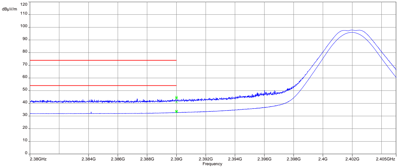
Plot 3: Lower restricted band, 2 Mbit/s
