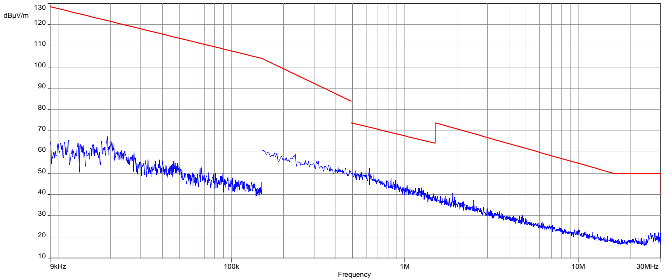
Plot 3: 9 kHz to 30 MHz, 2480 MHz, transmit mode, 1 Mbit/s
