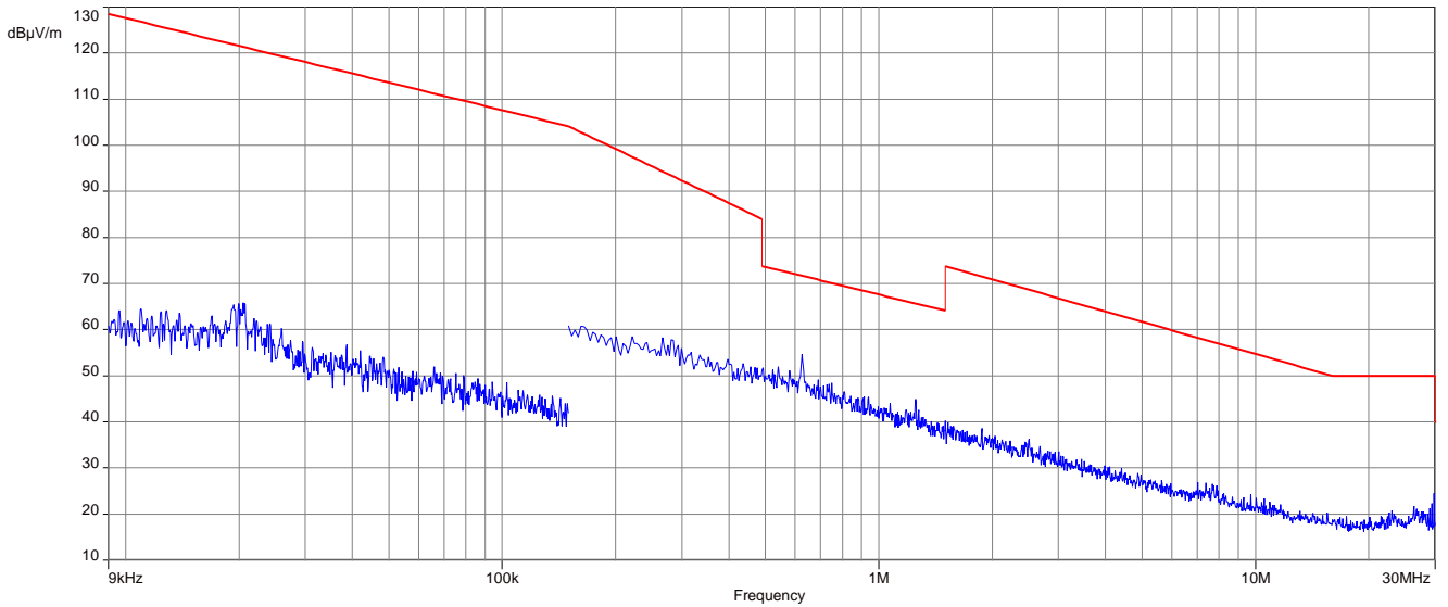
Plot 1: 9 kHz to 30 MHz, 2402 MHz, transmit mode, 1 Mbit/s
