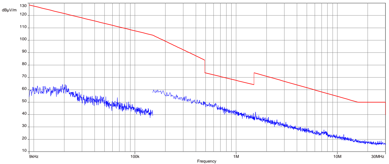
Plot 4: 9 kHz to 30 MHz, 2402 MHz, transmit mode, 2 Mbit/s
