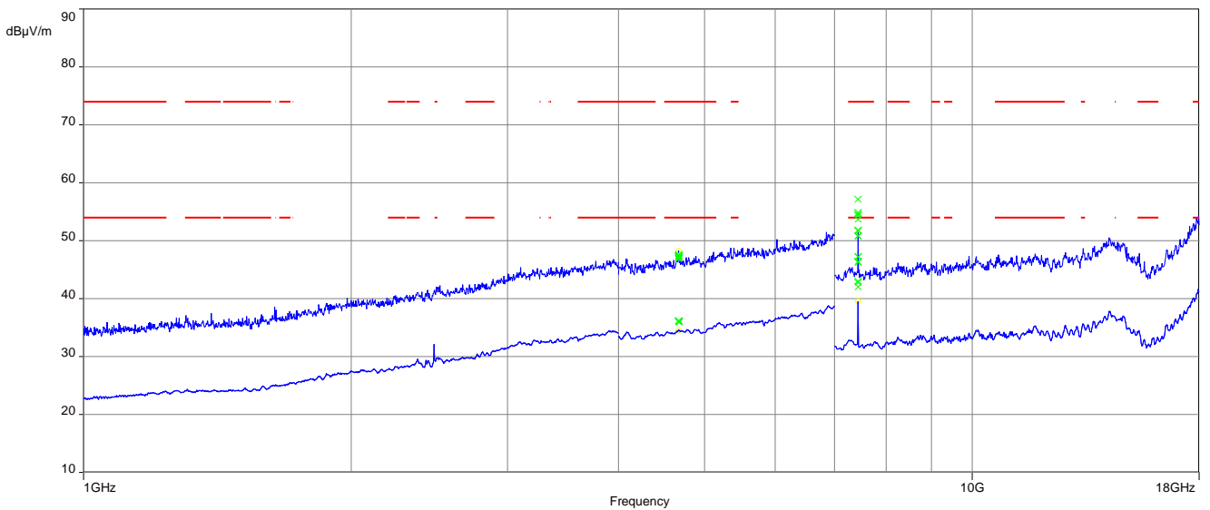
Plot 6: 1 GHz to 18 GHz, TX mode, 2480 MHz, vertical & horizontal polarization, 2 Mbit/s
