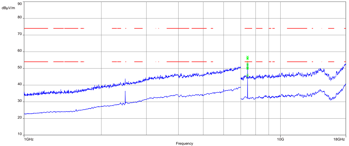
Plot 3: 1 GHz to 18 GHz, TX mode, 2480 MHz, vertical & horizontal polarization, 1 Mbit/s
