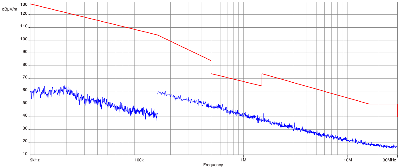
Plot 5: 9 kHz to 30 MHz, 2440 MHz, transmit mode, 2 Mbit/s
