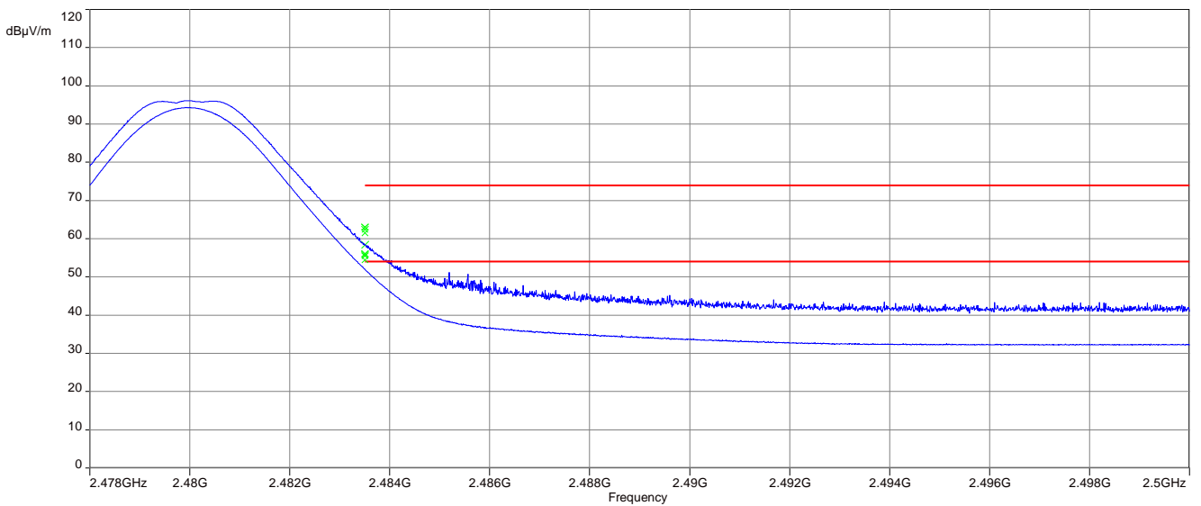
Plot 4: Upper restricted band, 2 Mbit/s
