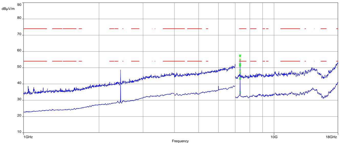
Plot 2: 1 GHz to 18 GHz, TX mode, 2440 MHz, vertical & horizontal polarization, 1 Mbit/s
