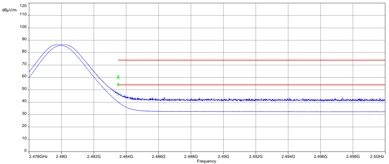
Plot 2: Upper restricted band, 1 Mbit/s
