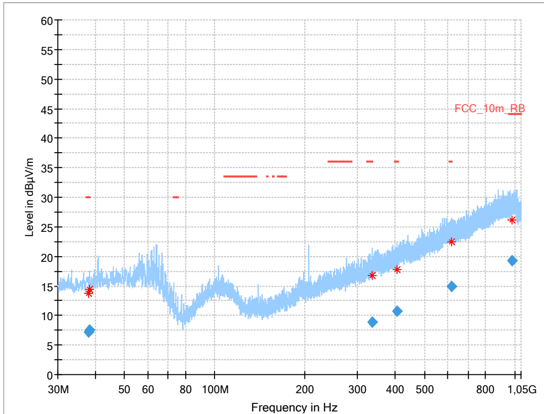
Plot 3: 30 MHz to 1 GHz, TX mode, vertical & horizontal polarization, 1 Msps, antenna 1 valid for all channels
