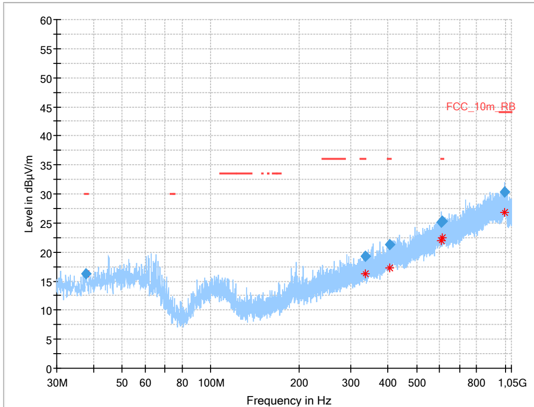
Plot 4: 30 MHz to 1 GHz, TX mode, vertical & horizontal polarization, 2 Msps, antenna 1 valid for all channels
