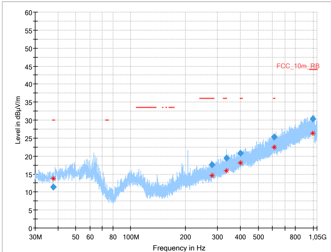
Plot 2: 30 MHz to 1 GHz, TX mode, vertical & horizontal polarization, 2 Msps, antenna 0 valid for all channels
