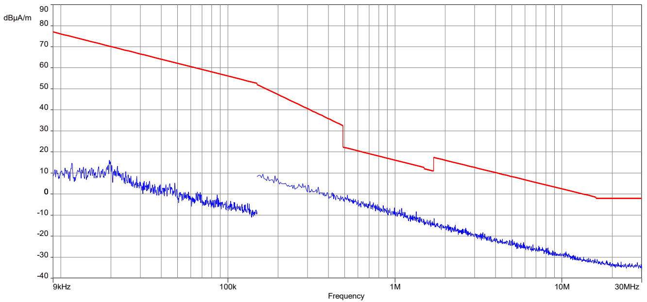
Plot 2: 9 kHz – 30 MHz, magnetic spurious emissions IC, MI e2eAudioHi mode
