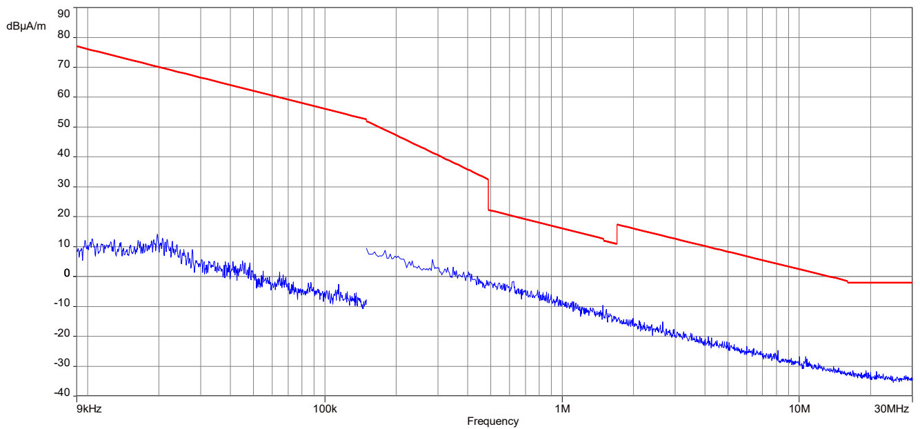
Plot 6: 9 kHz – 30 MHz, magnetic spurious emissions IC, MI e2eData mode
