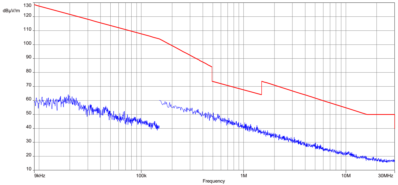
Plot 5: 9 kHz – 30 MHz, magnetic spurious emissions FCC, MI e2eData mode
