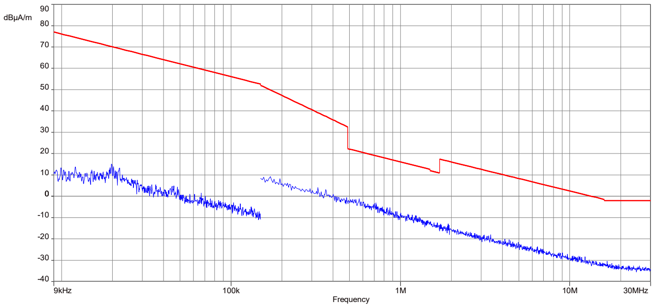
Plot 4: 9 kHz – 30 MHz, magnetic spurious emissions IC, MI e2eAudioLo mode
