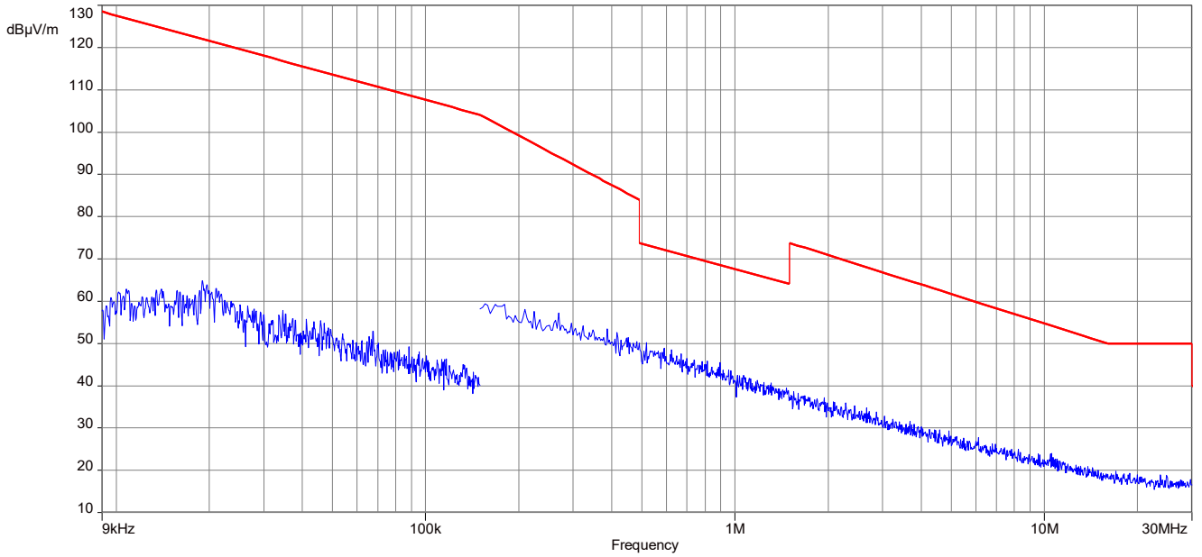
Plot 3: 9 kHz – 30 MHz, magnetic spurious emissions FCC, MI e2eAudioLo mode
