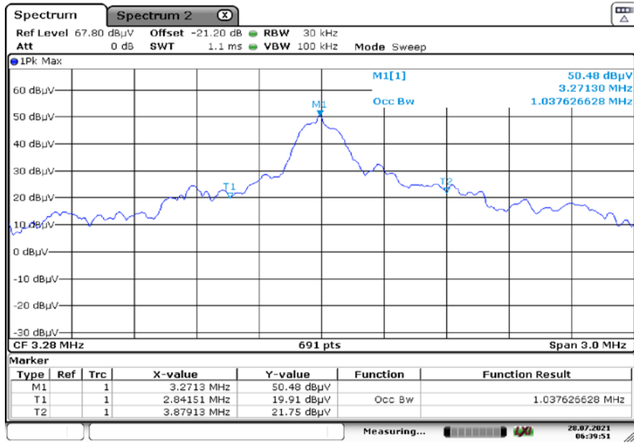
Plot 3: 99 % emission bandwidth MI e2eData mode
