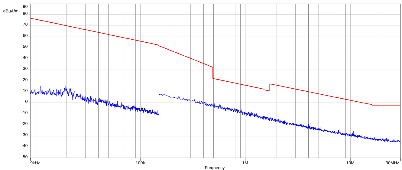
Plot 2: 9 kHz – 30 MHz, magnetic spurious emissions IC, MI e2eAudioHi mode
