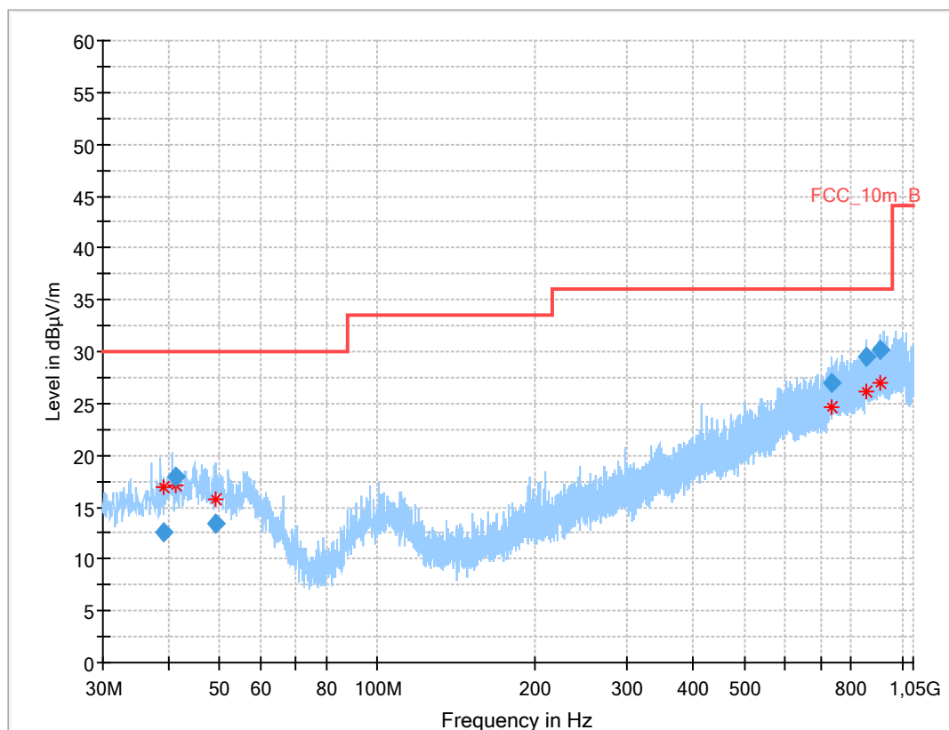
Plot 3: 30 MHz – 1 GHz, vertical and horizontal polarization MI e2eData mode
