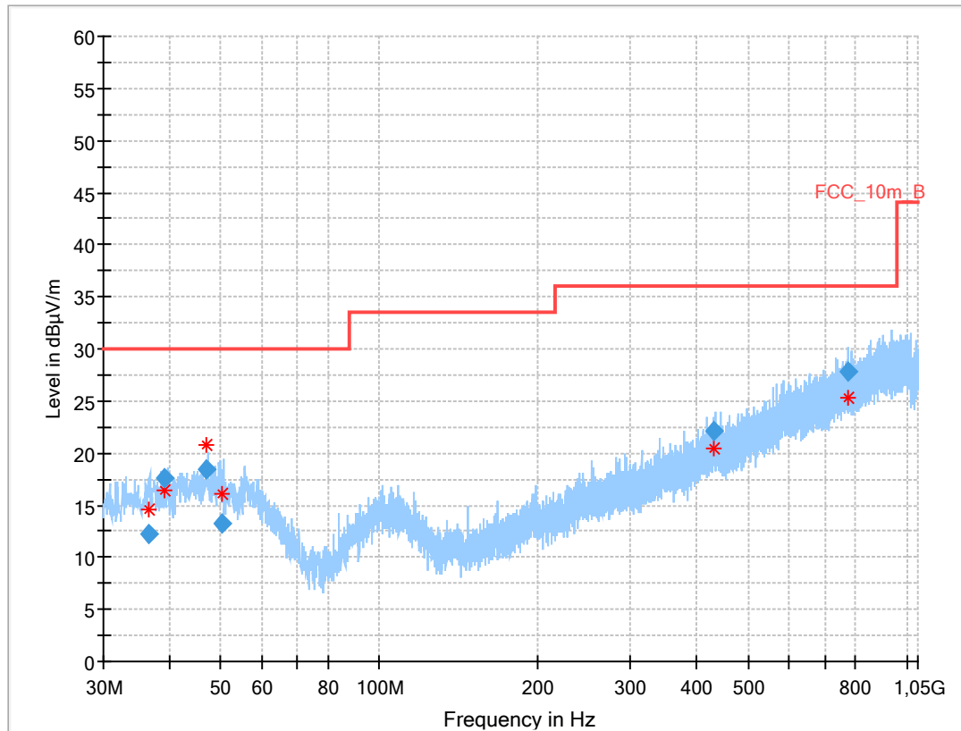
Plot 2: 30 MHz – 1 GHz, vertical and horizontal polarization MI e2eAudioLo mode
