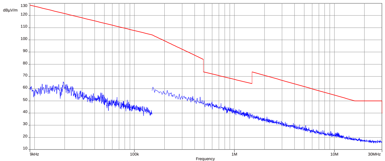
Plot 3: 9 kHz – 30 MHz, magnetic spurious emissions FCC, MI e2eAudioLo mode
