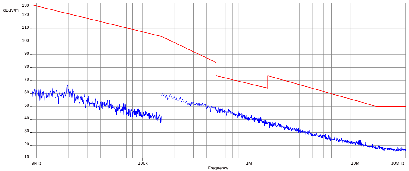
Plot 5: 9 kHz – 30 MHz, magnetic spurious emissions FCC, MI e2eData mode
