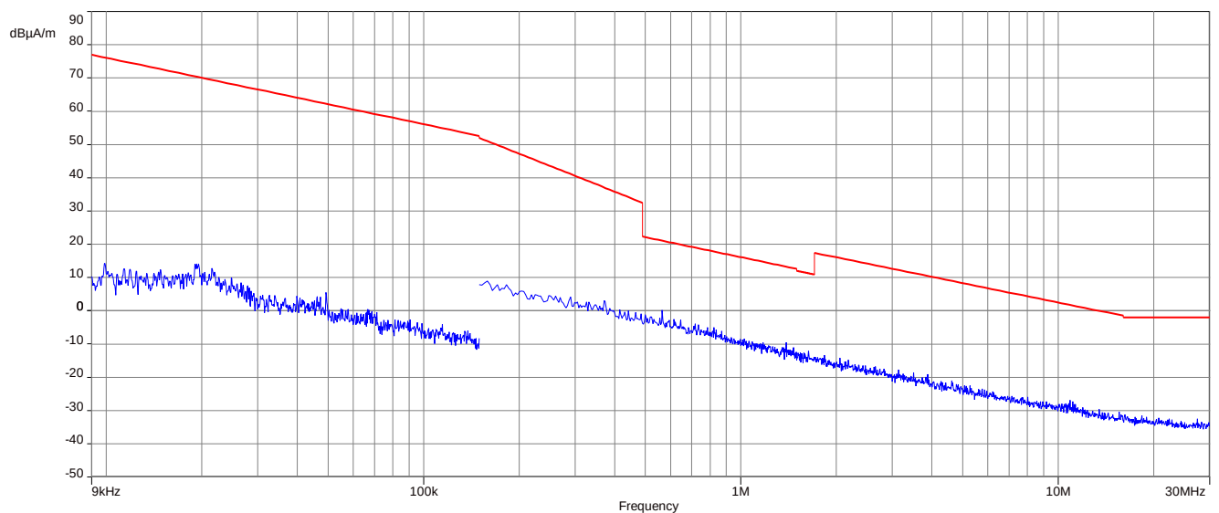
Plot 4: 9 kHz – 30 MHz, magnetic spurious emissions IC, MI e2eAudioLo mode
