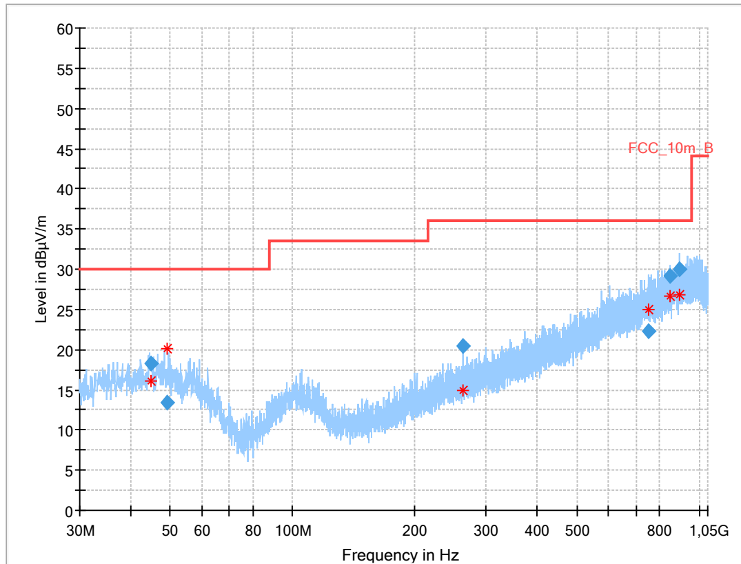
Plot 1: 30 MHz – 1 GHz, vertical and horizontal polarization MI e2eAudioHi mode
