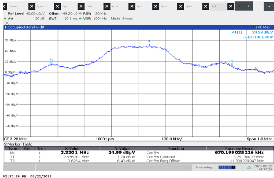
Plot 1: 99 % emission bandwidth MI e2eAudioHi mode
