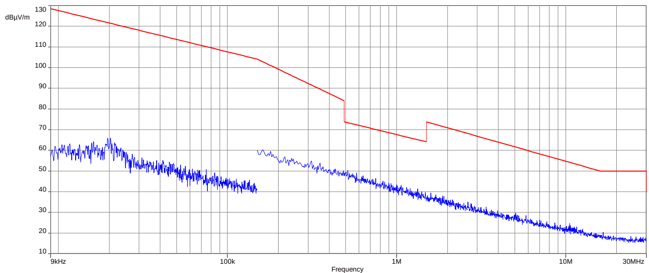
Plot 1: 9 kHz – 30 MHz, magnetic spurious emissions FCC, MI e2eAudioHi mode
