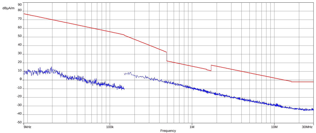
Plot 6: 9 kHz – 30 MHz, magnetic spurious emissions IC, MI e2eData mode
