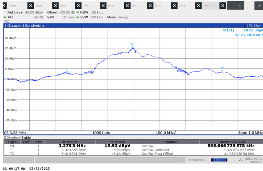
Plot 3: 99 % emission bandwidth MI e2eData mode
