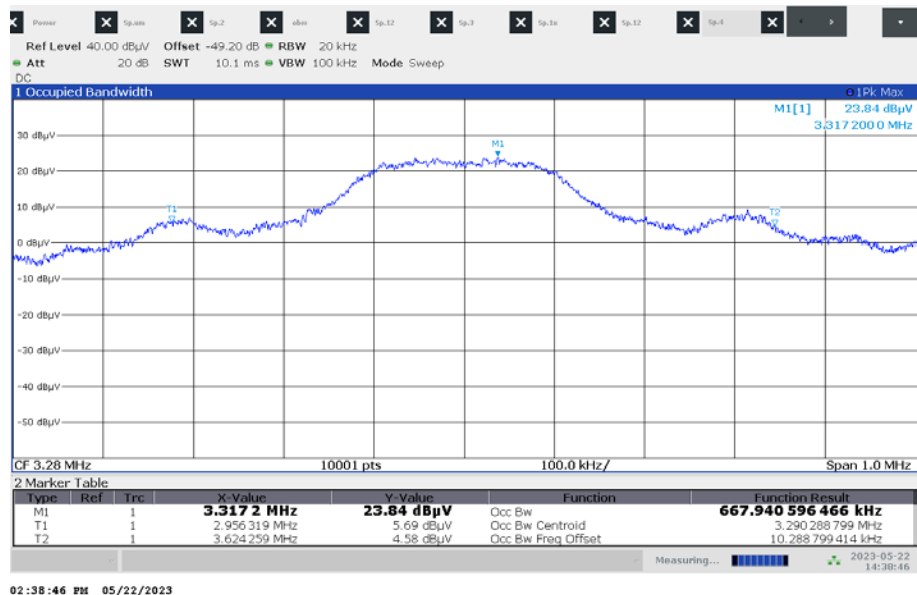
Plot 2: 99 % emission bandwidth MI e2eAudioLo mode
