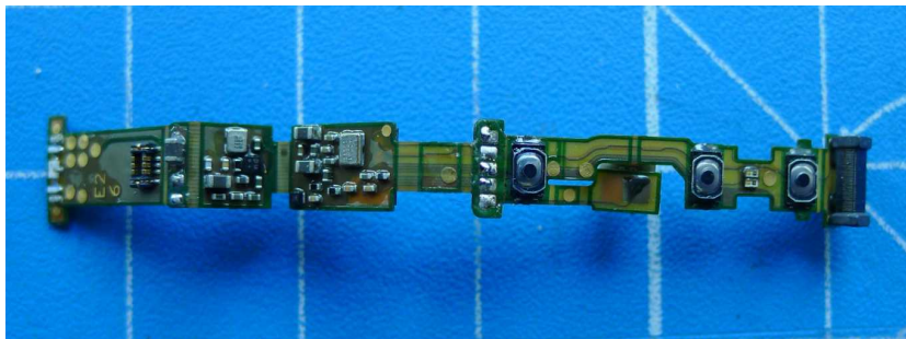
Photo 6: top FPC (flexPCB)
