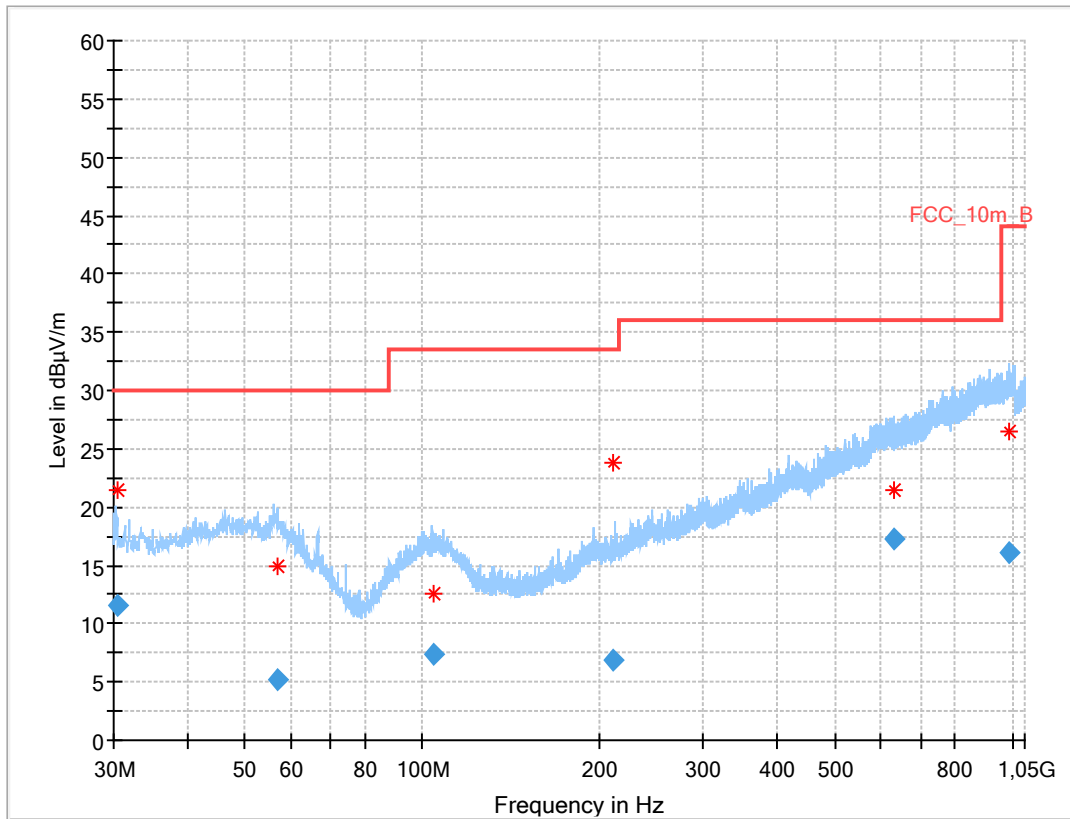
Plot 1: 30 MHz to 1 GHz, TX mode, 2402 MHz, vertical & horizontal polarization, 1 Msps
