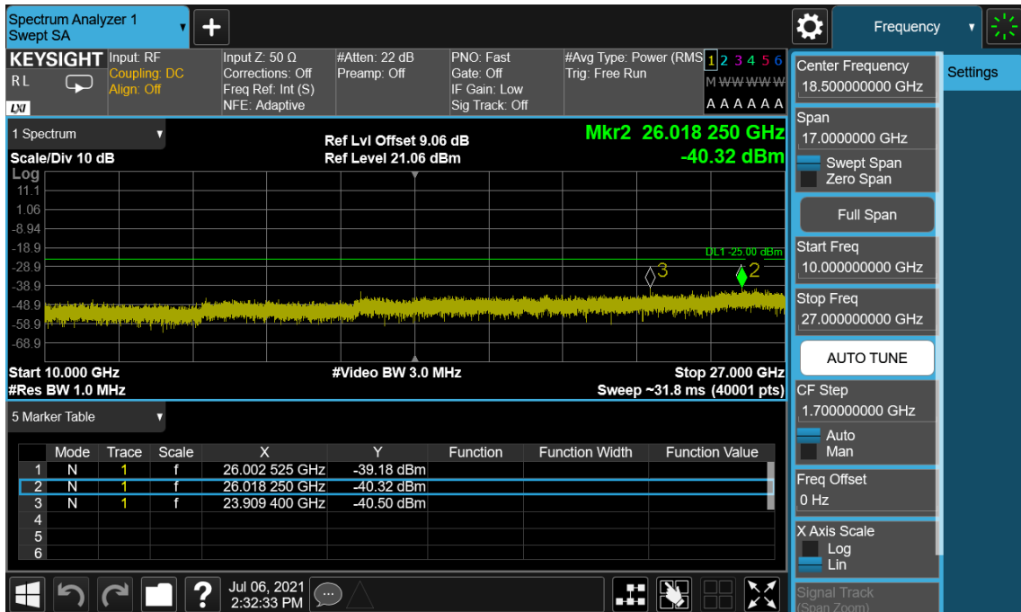
LTE Band 41 / 15 MHz / QPSK - RB Size/Offset (36/0)–Low Channel
