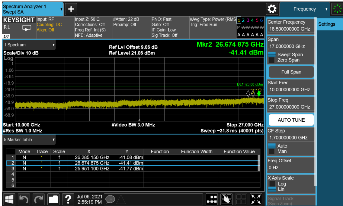
LTE Band 41 / 20 MHz / QPSK - RB Size/Offset (100/0)–Mid Channel
