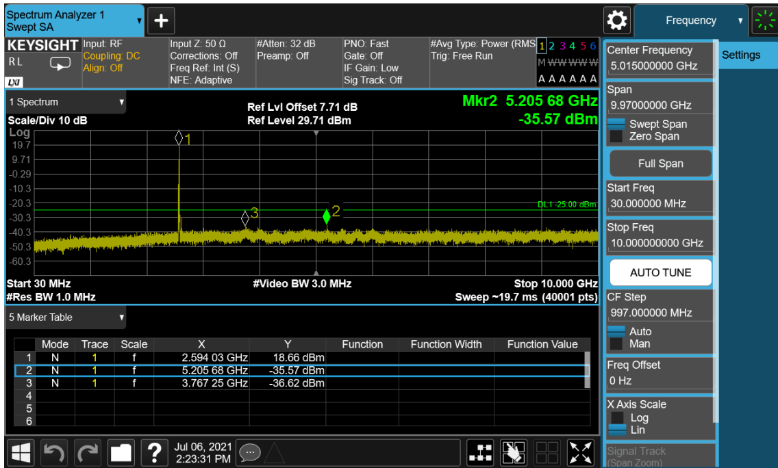
LTE Band 41 / 10 MHz / QPSK - RB Size/Offset (25/25) – Mid Channel
