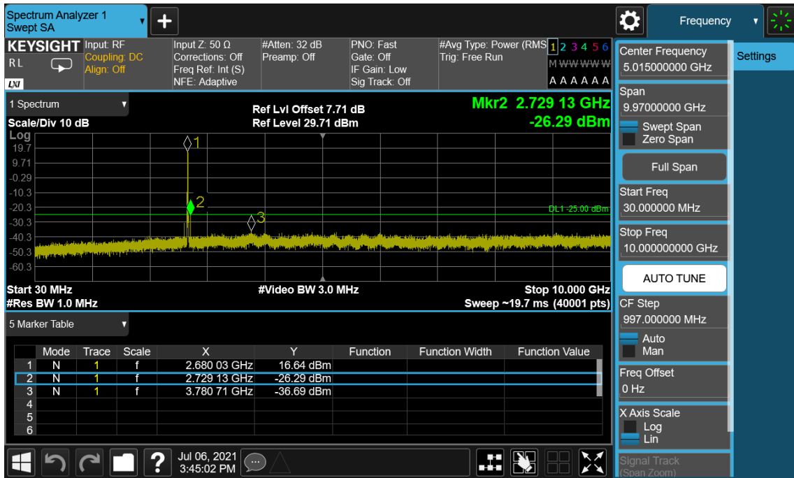
LTE Band 41 / 15 MHz / 16QAM - RB Size/Offset (36/0) – High Channel
