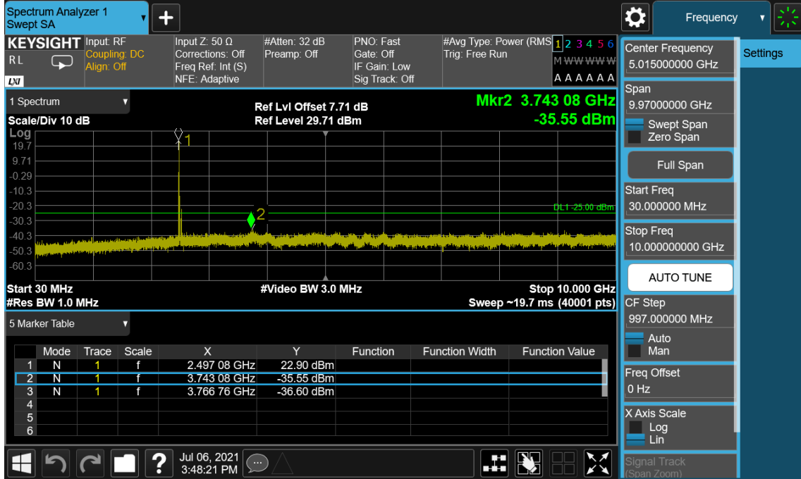
LTE Band 41 / 20 MHz / 16QAM - RB Size/Offset (1/0) –Low Channel
