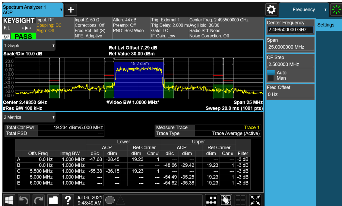
LTE Band 41 / 5 MHz / QPSK - RB Size/Offset (25/0)
