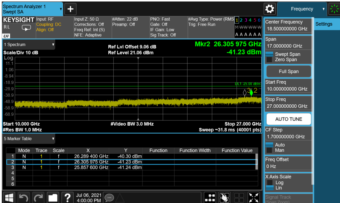
LTE Band 41 / 20 MHz / 16QAM - RB Size/Offset (1/99) – High Channel
