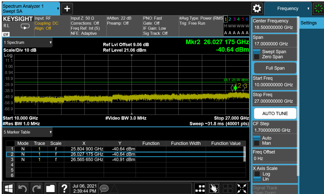
LTE Band 41 / 15 MHz / QPSK - RB Size/Offset (75/0) – Mid Channel
