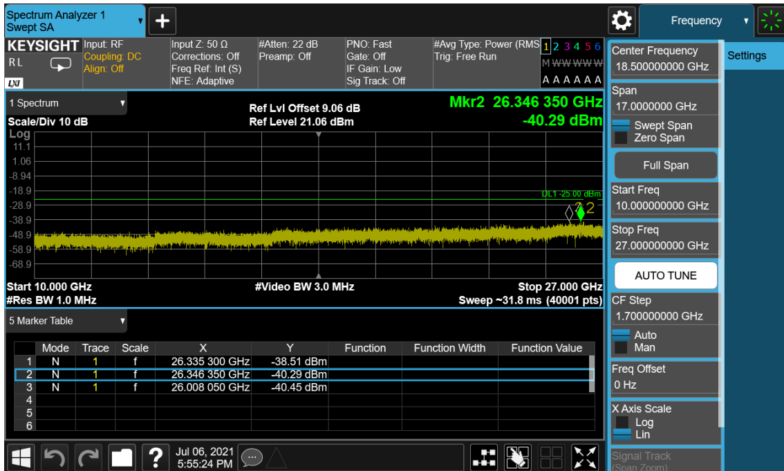
LTE Band 41 / 10 MHz / 16QAM - RB Size/Offset (25/12) – High Channel
