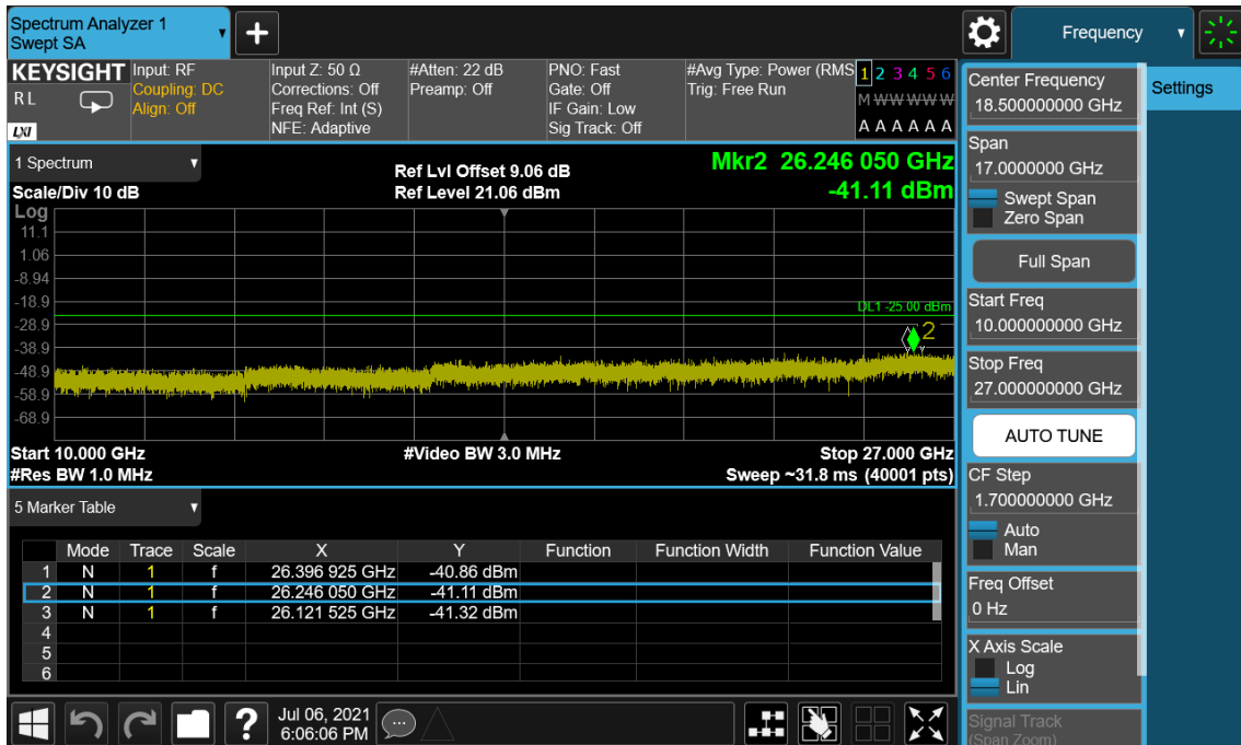
LTE Band 41 / 15 MHz / 16QAM - RB Size/Offset (1/36) – Mid Channel
