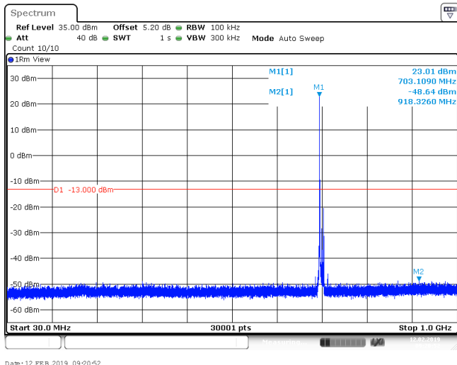
Band12_10MHz_16QAM_23095_1RB#0
