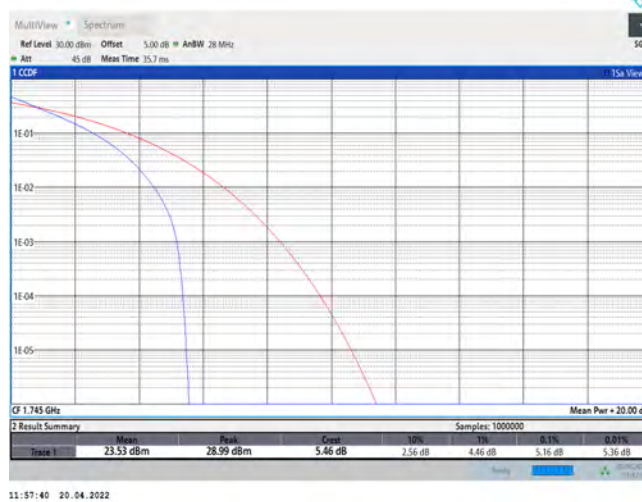
Band66-20MHz-QPSK-132322-100RB#0
