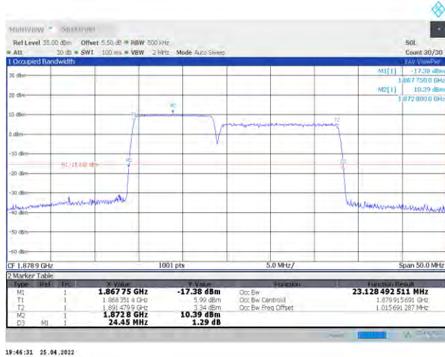
2-2-10MHz-15MHz-QPSK-QPSK-18829-18949-50RB#0-75RB#0
