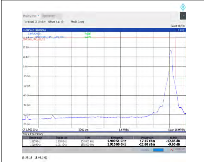
1-N2--15-15-H-5-CP-QPSK-Edge_1RB_Right-1@78-Ant1-seegraph-PASS-see graph
