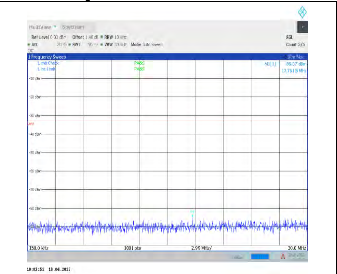
1-N2--15-20-H-1-DFT-PI2BPSK-Inner_1RB_Left-1@ 1-0.15-30-Ant1--85.37--33-PASS
