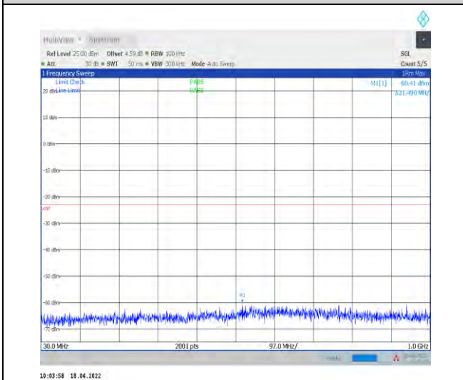
1-N2--15-20-H-1-DFT-PI2BPSK-Inner_1RB_Left-1@ 1-30-1000-Ant1--60.41--23-PASS
