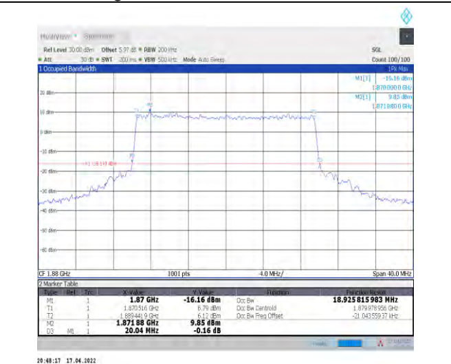
1-N2--15-20-M-8-CP-64QAM-Outer_Full-106@0-Ant 1-18.926-20.040-≤20-PASS
