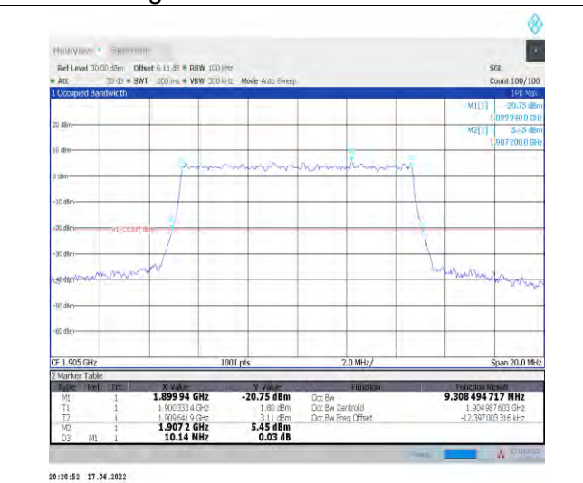
1-N2--15-10-H-9-CP-256QAM-Outer_Full-52@0-Ant1 1-9.308-10.140-≤10-PASS
