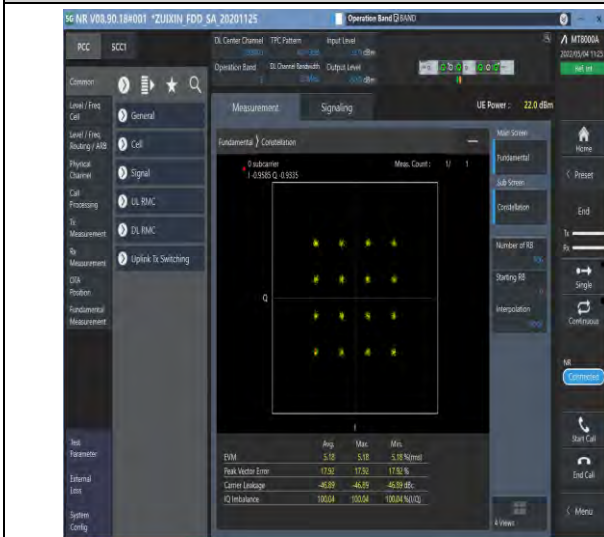
1-N2-PC3-15-20-M-7-CP-16QAM-Outer_Full-106@0-Ant1-see graph-PASS
