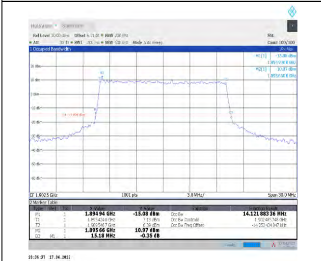
1-N2--15-15-H-7-CP-16QAM-Outer_Full-79@0-Ant1 -14.122-15.180-≤15-PASS
