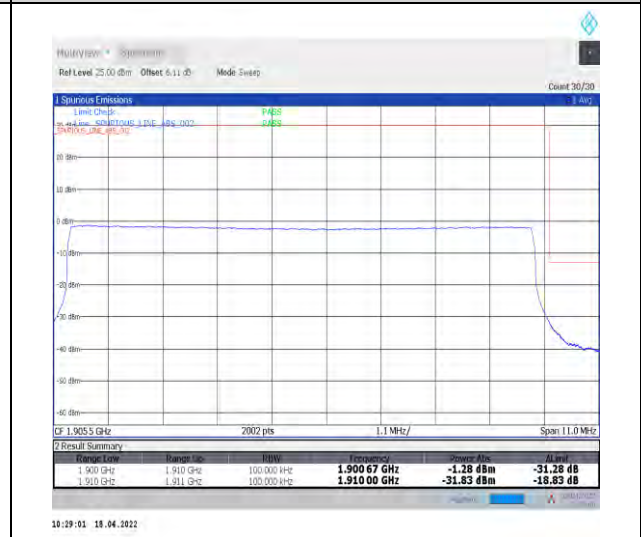
1-N2--15-10-H-6-CP-QPSK-Outer_Full-52@0-Ant1-seegraph-PASS-see graph
