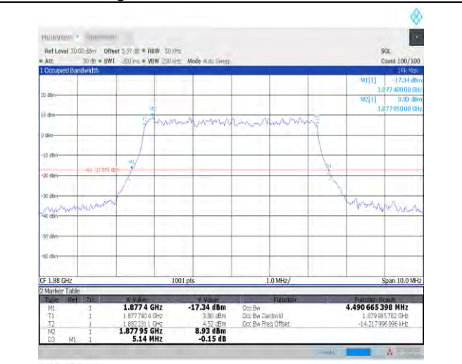
1-N2--15-5-M-5-DFT-256QAM-Outer_Full-25@0-Ant 1-4.491-5.140-≤5-PASS
