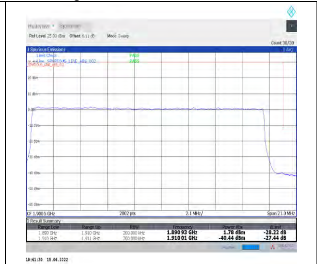
1-N2--15-20-H-3-DFT-PI2BPSK-Outer_Full-100@0-Ant1-seegraph-PASS-see graph
