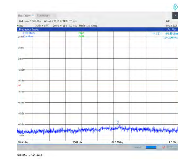
1-N2--15-20-M-1-DFT-PI2BPSK-Inner_1RB_Left-1 @1-30-1000-Ant1--60.49--23-PASS
