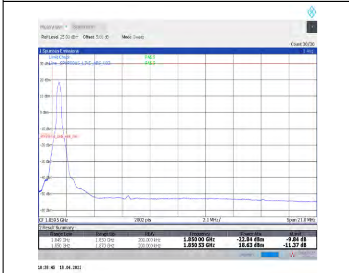
1-N2--15-20-L-4-CP-QPSK-Edge_1RB_Left-1@0-Ant1-seegraph-PASS-see graph
