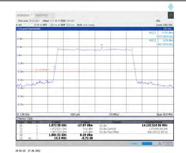
1-N2--15-15-M-9-CP-256QAM-Outer_Full-79@0-Ant1-14.153-15.300-≤15-PASS
