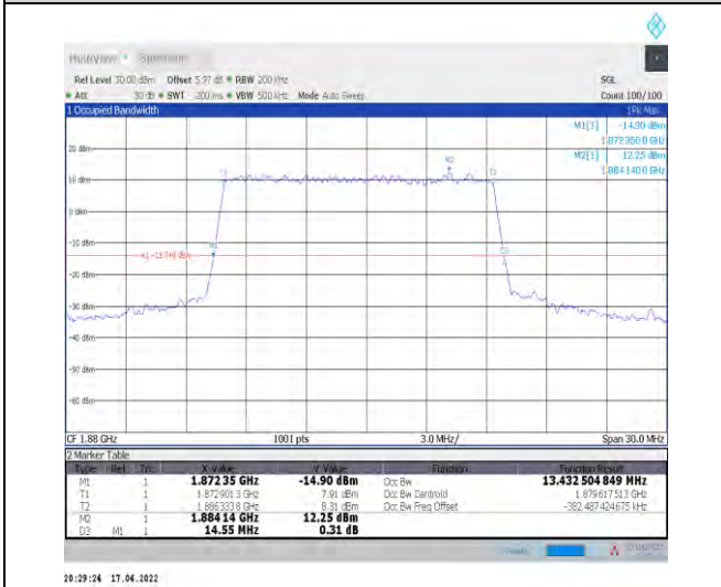
1-N2--15-15-M-4-DFT-64QAM-Outer_Full-75@0-Ant 1-13.433-14.550-≤15-PASS
