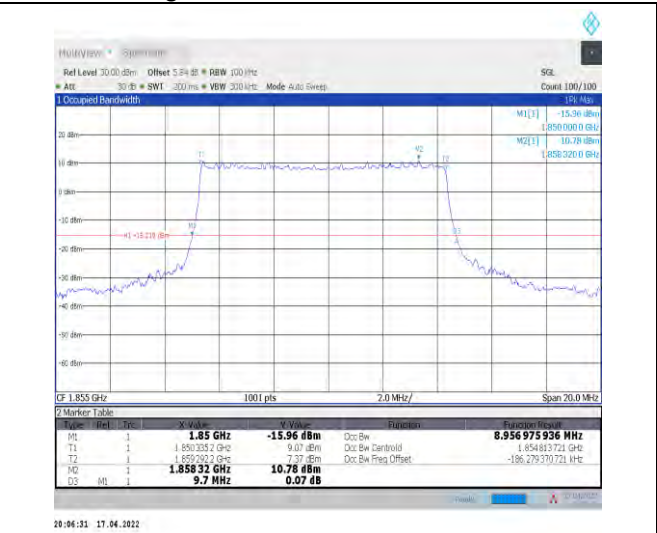
1-N2--15-10-L-3-DFT-16QAM-Outer_Full-50@0-Ant1 -8.957-9.700-≤10-PASS
