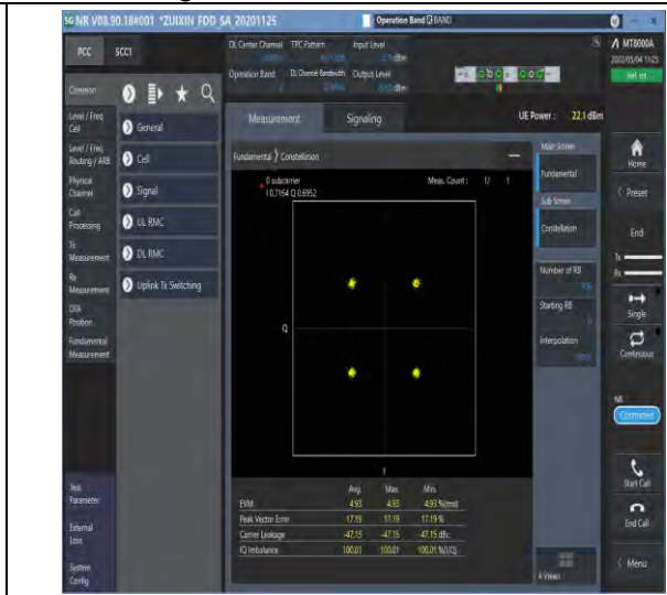
1-N2-PC3-15-20-M-6-CP-QPSK-Outer_Full-106@0-Ant1-see graph-PASS
