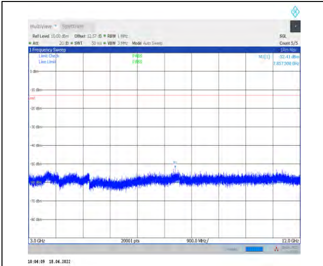
1-N2--15-20-H-1-DFT-PI2BPSK-Inner_1RB_Left-1@ 1-3000-12000-Ant1--52.41--13-PASS
