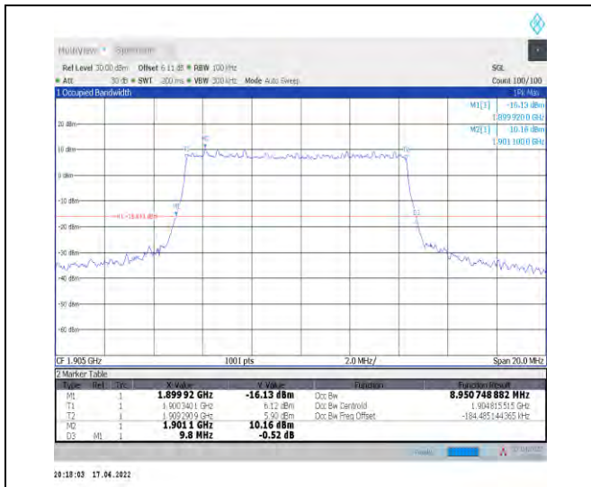
1-N2--15-10-H-4-DFT-64QAM-Outer_Full-50@0-Ant 1-8.951-9.800-≤10-PASS
