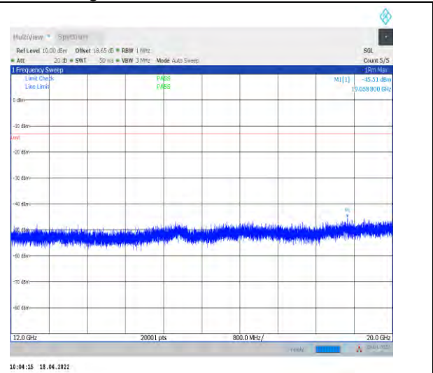
1-N2--15-20-H-1-DFT-PI2BPSK-Inner_1RB_Left-1@ 1-12000-20000-Ant1--45.51--13-PASS
