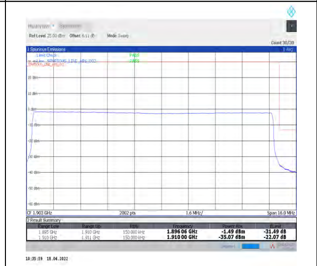
1-N2--15-15-H-6-CP-QPSK-Outer_Full-79@0-Ant1-seegraph-PASS-see graph
