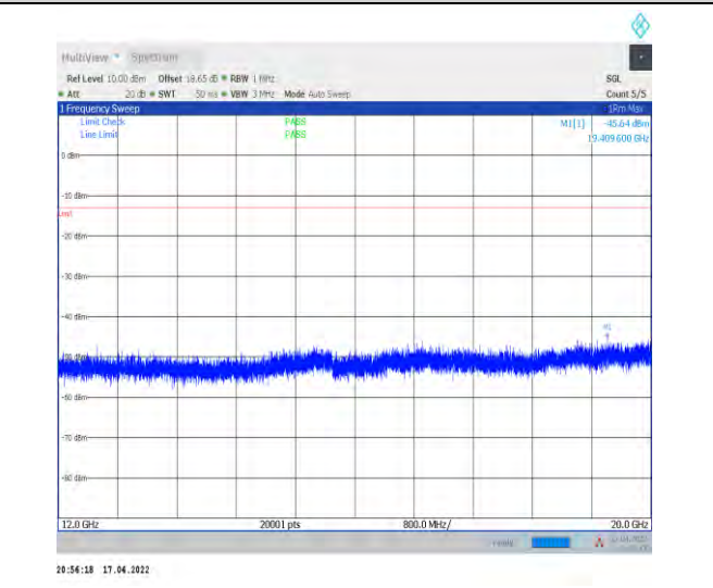
1-N2--15-20-M-1-DFT-PI2BPSK-Inner_1RB_Left-1@ 1-12000-20000-Ant1--45.64--13-PASS
