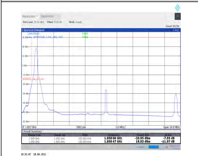
1-N2--15-15-L-4-CP-QPSK-Edge_1RB_Left-1@0-Ant1-seegraph-PASS-see graph
