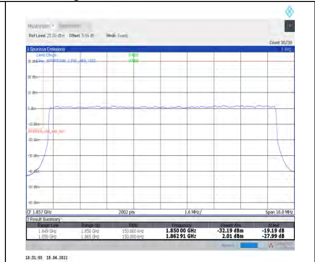
1-N2--15-15-L-3-DFT-PI2BPSK-Outer_Full-75@0-Ant1-seegraph-PASS-see graph
