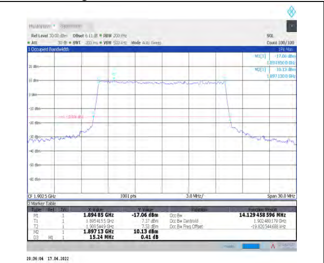
1-N2--15-15-H-6-CP-QPSK-Outer_Full-79@0-Ant1-1 4.129-15.240-≤15-PASS
