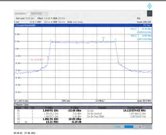
1-N2--15-15-L-6-CP-QPSK-Outer_Full-79@0-Ant1-1 4.126-15.210-≤15-PASS
