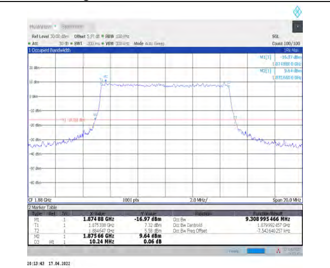
1-N2--15-10-M-6-CP-QPSK-Outer_Full-52@0-Ant1-9 .309-10.240-≤10-PASS
