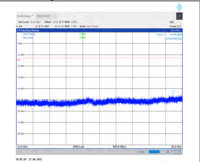
1-N2--15-20-L-1-DFT-PI2BPSK-Inner_1RB_Left-1@1 -12000-20000-Ant1--44.98--13-PASS
