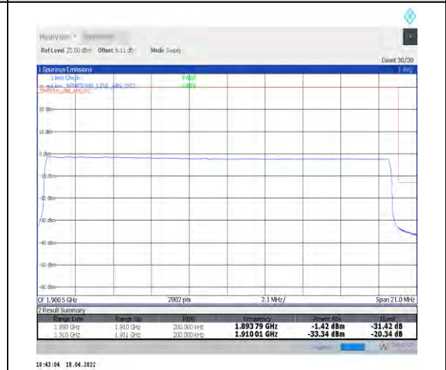
1-N2--15-20-H-6-CP-QPSK-Outer_Full-106@0-Ant1-seegraph-PASS-see graph
