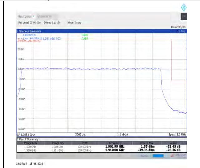
1-N2--15-10-H-3-DFT-PI2BPSK-Outer_Full-50@0-Ant1-seegraph-PASS-see graph
