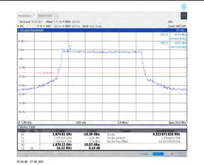
1-N2--15-10-M-8-CP-64QAM-Outer_Full-52@0-Ant1 -9.324-10.220-≤10-PASS
