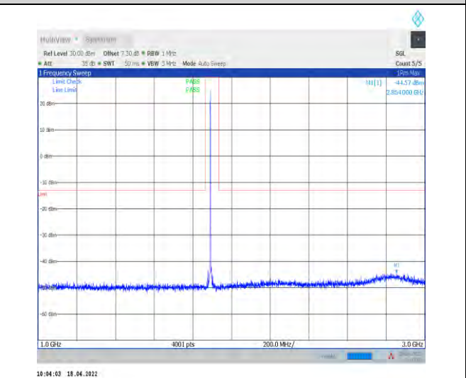
1-N2--15-20-H-1-DFT-PI2BPSK-Inner_1RB_Left-1@ 1-1000-3000-Ant1--44.57--13-PASS
