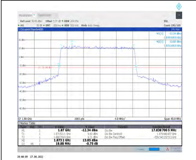
1-N2--15-20-M-1-DFT-QPSK-Outer_Full-100@0-Ant 1-17.839-18.880-≤20-PASS
