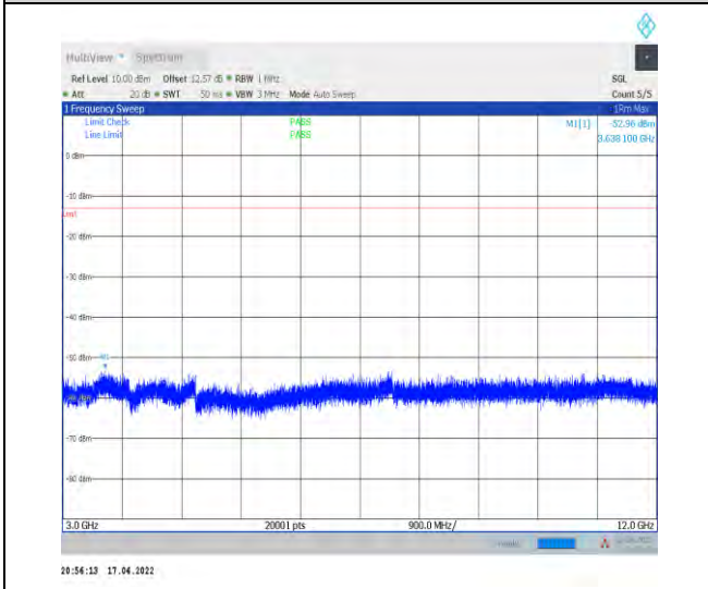
1-N2--15-20-M-1-DFT-PI2BPSK-Inner_1RB_Left-1 @1-3000-12000-Ant1--52.96--13-PASS
