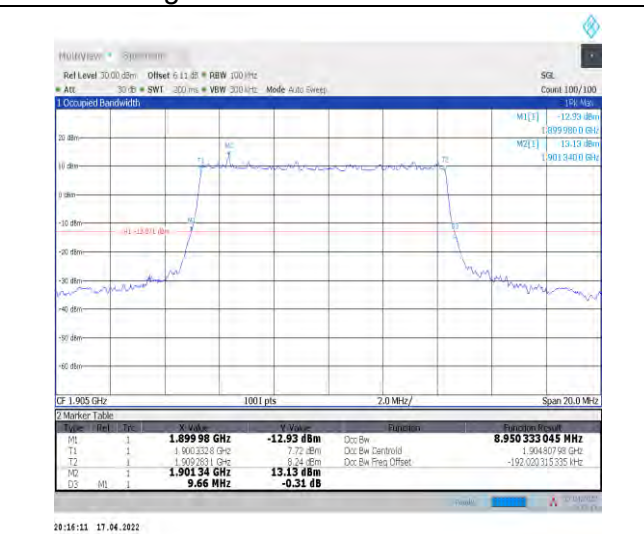
1-N2--15-10-H-1-DFT-QPSK-Outer_Full-50@0-Ant1- 8.95-9.660-≤10-PASS
