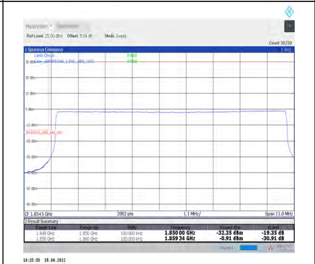
1-N2--15-10-L-6-CP-QPSK-Outer_Full-52@0-Ant1-seegraph-PASS-see graph
