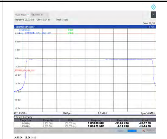
1-N2--15-15-L-6-CP-QPSK-Outer_Full-79@0-Ant1-seegraph-PASS-see graph
