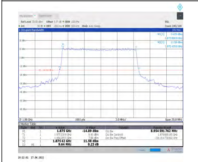
1-N2--15-10-M-3-DFT-16QAM-Outer_Full-50@0-Ant1 1-8.955-9.640-≤10-PASS
