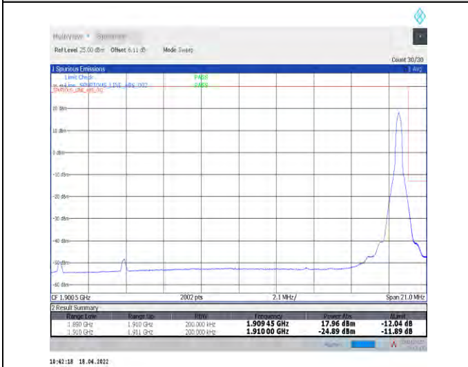
1-N2--15-20-H-5-CP-QPSK-Edge_1RB_Right-1@105-Ant1-seegraph-PASS-see graph
