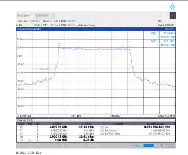
1-N2--15-10-H-3-DFT-16QAM-Outer_Full-50@0-Ant 1-8.962-9.680-≤10-PASS
