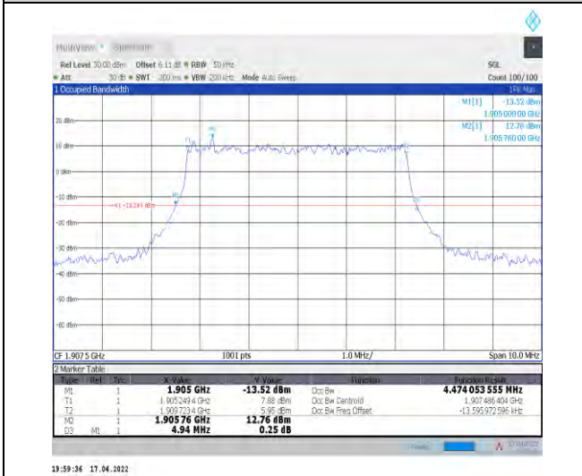
1-N2--15-5-H-1-DFT-QPSK-Outer_Full-25@0-Ant1-4.474-4.940-≤5-PASS
