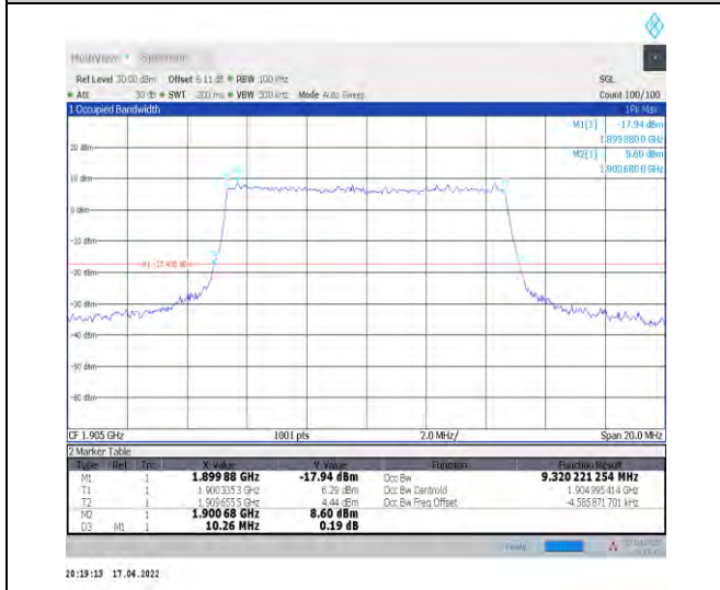
1-N2--15-10-H-6-CP-QPSK-Outer_Full-52@0-Ant1-9 .32-10.260-≤10-PASS
