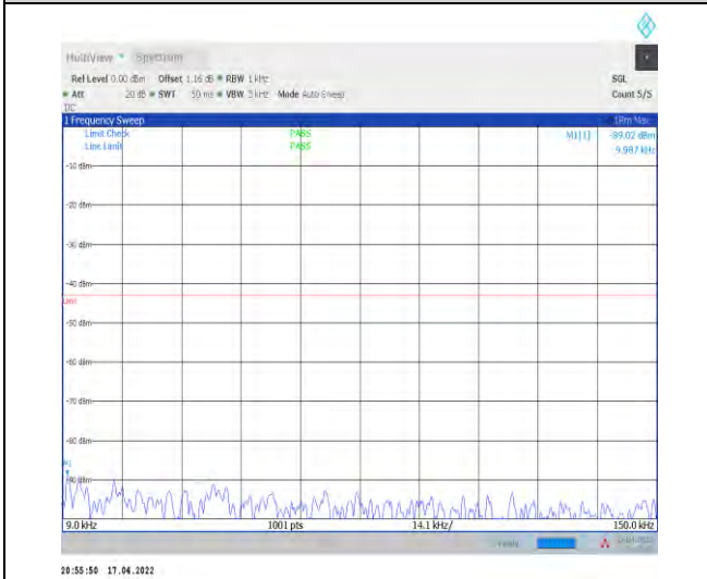
1-N2--15-20-M-1-DFT-PI2BPSK-Inner_1RB_Left-1 @1-0.009-0.15-Ant1--89.02--43-PASS
