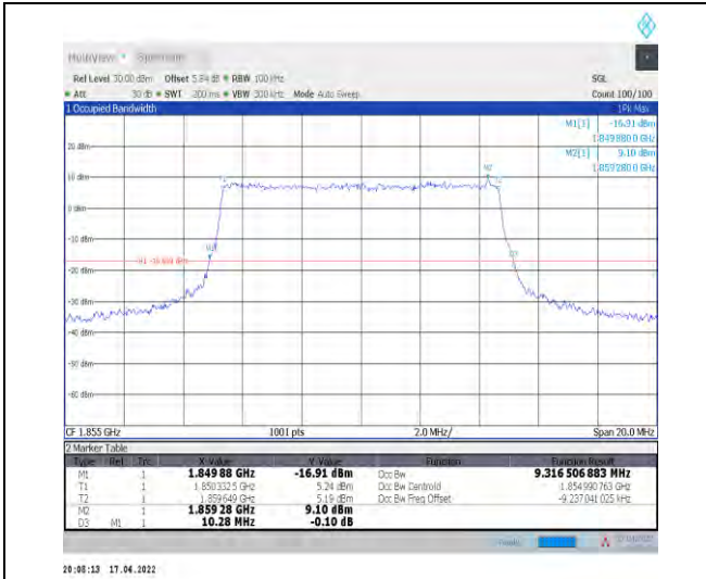
1-N2--15-10-L-6-CP-QPSK-Outer_Full-52@0-Ant1-9 .317-10.280-≤10-PASS
