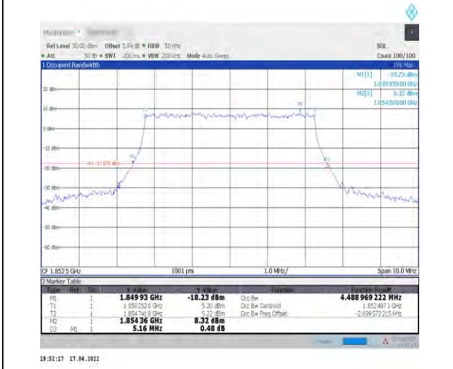
1-N2--15-5-L-7-CP-16QAM-Outer_Full-25@0-Ant1-4 .489-5.160-≤5-PASS
