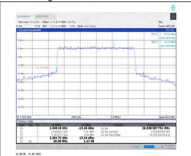
1-N7--15-30-H-1-DFT-QPSK-Outer_Full-160@0-Ant 1-28.539-29.580-≤30-PASS
