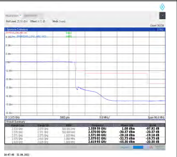
1-N7--15-40-H-6-CP-QPSK-Outer_Full-216@0-An t1-PASS-see graph
