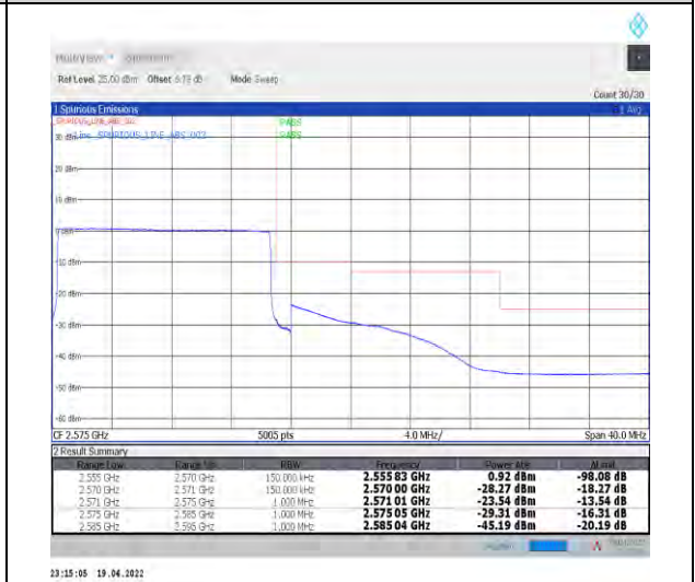
1-N7--15-15-H-6-CP-QPSK-Outer_Full-79@0-Ant 1-PASS-see graph
