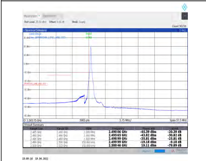
1-N7--15-15-L-4-CP-QPSK-Edge_1RB_Left-1@0-Ant1-PASS-see graph
