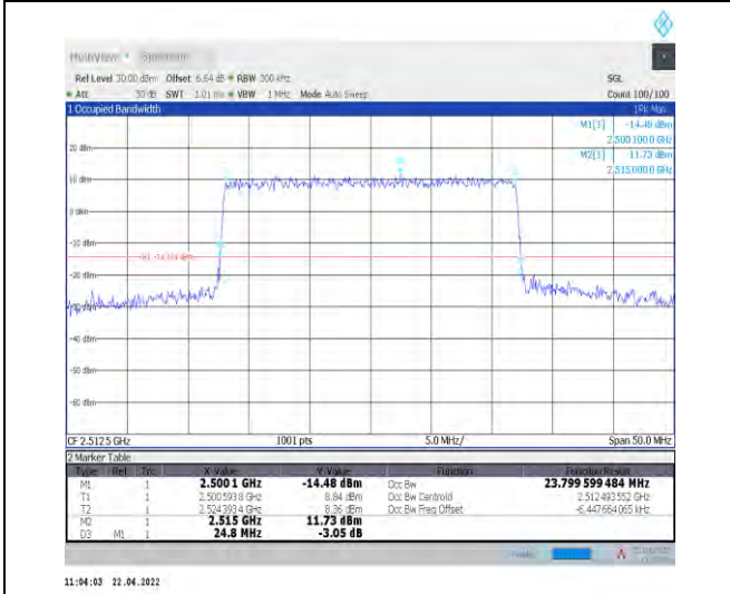
1-N7--15-25-L-7-CP-16QAM-Outer_Full-133@0-Ant 1-23.8-24.800-≤25-PASS
