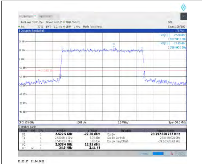
1-N7--15-25-M-8-CP-64QAM-Outer_Full-133@0-Ant 1-23.798-24.900-≤25-PASS
