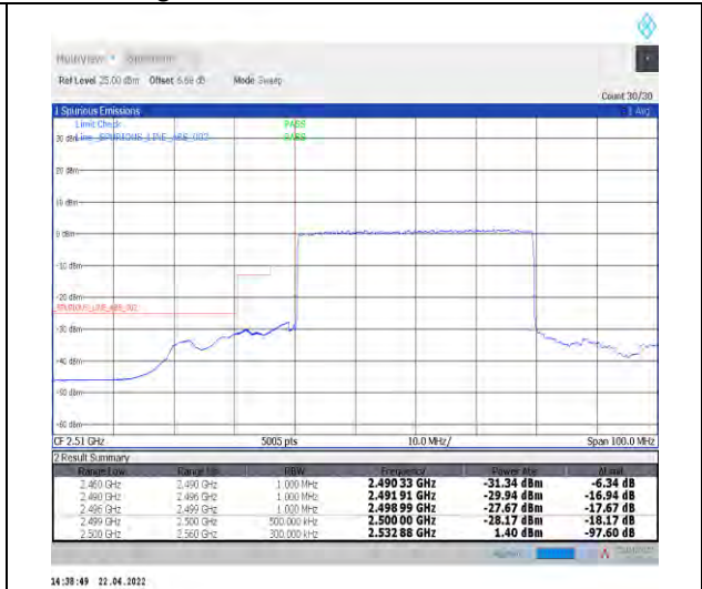
1-N7--15-40-L-3-DFT-PI2BPSK-Outer_Full-216@0-Ant1-PASS-see graph
