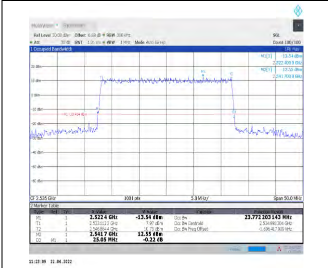
1-N7--15-25-M-6-CP-QPSK-Outer_Full-133@0-Ant1-23.772-25.050-<25-PASS
