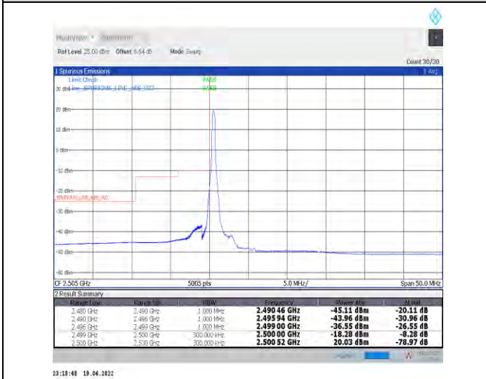
1-N7--15-20-L-4-CP-QPSK-Edge_1RB_Left-1@0-Ant1-PASS-see graph
