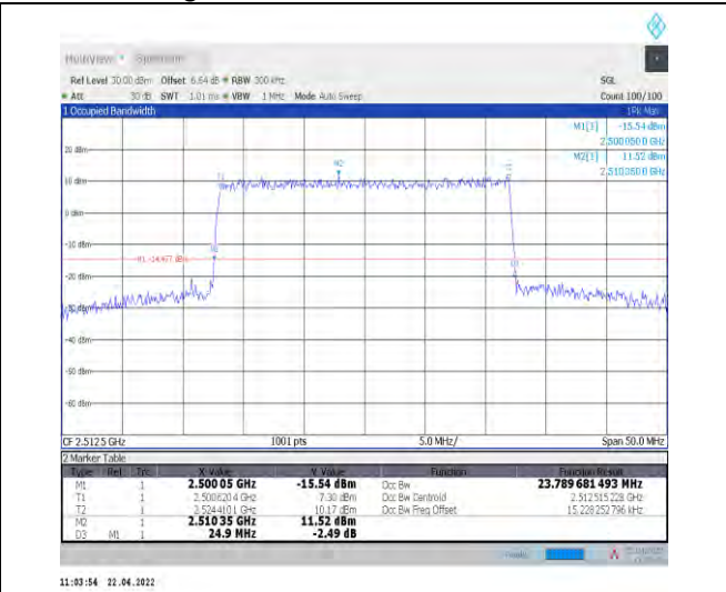
1-N7--15-25-L-6-CP-QPSK-Outer_Full-133@0-Ant1- 23.79-24.900-≤25-PASS
