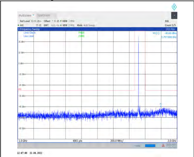
1-N7--15-40-M-1-DFT-PI2BPSK-Inner_1RB_Left-1 @1-1000-3000-Ant1--40.60--25-PASS
