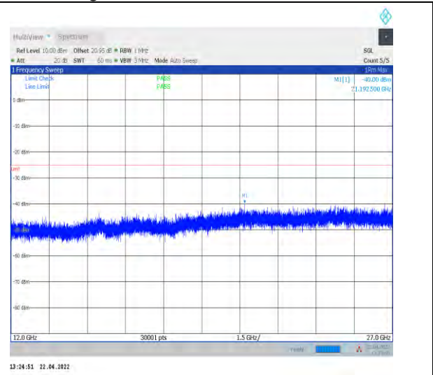
1-N7--15-40-H-1-DFT-PI2BPSK-Inner_1RB_Left-1@ 1-12000-27000-Ant1--40.00--25-PASS
