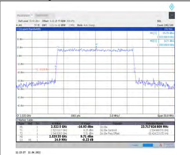
1-N7--15-25-M-9-CP-256QAM-Outer_Full-133@0-A nt1-23.718-24.900-≤25-PASS
