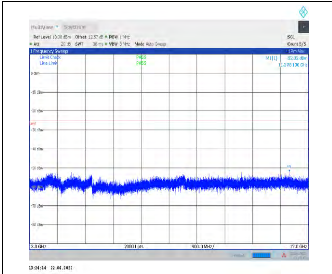
1-N7--15-40-H-1-DFT-PI2BPSK-Inner_1RB_Left-1@ 1-3000-12000-Ant1--52.32--25-PASS
