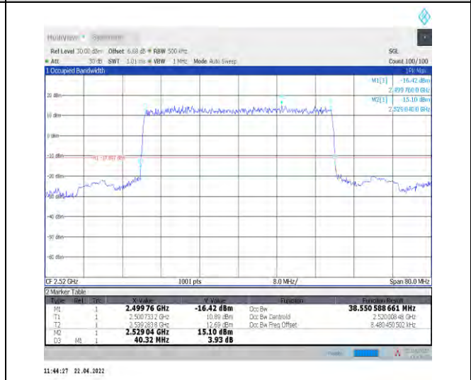
1-N7--15-40-L-2-DFT-PI2BPSK-Outer_Full-216@0-Ant1 -38.552-40.320-≤40-PASS
