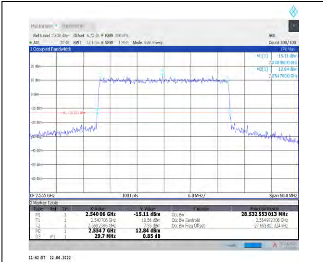
1-N7--15-30-H-4-DFT-64QAM-Outer_Full-160@0-An t1-28.533-29.700-<30-PASS
