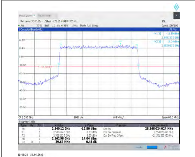
1-N7--15-30-H-2-DFT-PI2BPSK-Outer_Full-160@0-Ant1 1-28.568-29.640-≤30-PASS
