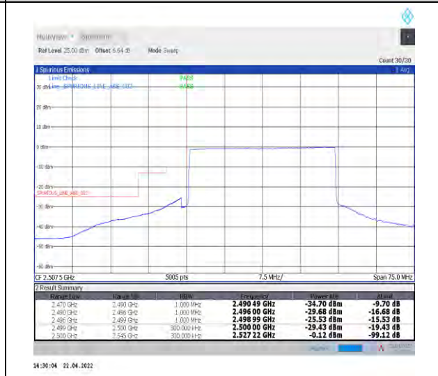
1-N7--15-30-L-6-CP-QPSK-Outer_Full-160@0-Ant1-PASS-see graph
