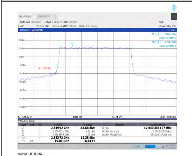
1-N7--15-20-H-4-DFT-64QAM-Outer_Full-100@0-Ant1-17.84-19.080-≤20-PASS
