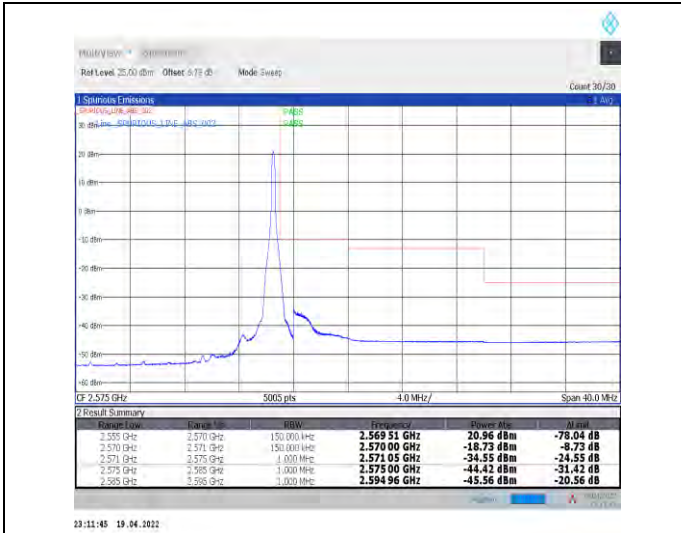
1-N7--15-15-H-2-DFT-PI2BPSK-Edge_1RB_Right-1@7 8-Ant1-PASS-see graph
