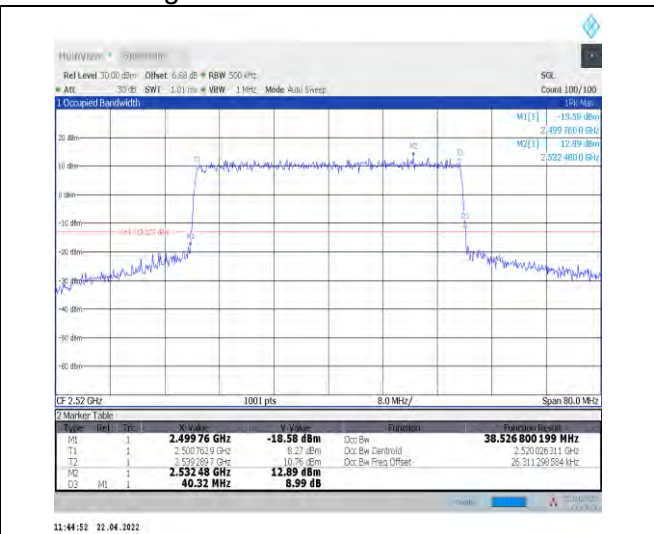
1-N7--15-40-L-4-DFT-64QAM-Outer_Full-216@0-Ant 1-38.533-40.320-≤40-PASS
