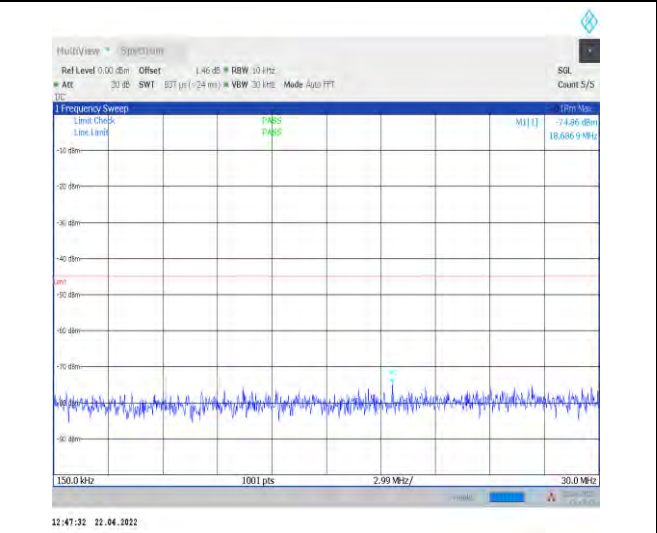
1-N7--15-40-M-1-DFT-PI2BPSK-Inner_1RB_Left-1@ 1-0.15-30-Ant1--74.86--45-PASS
