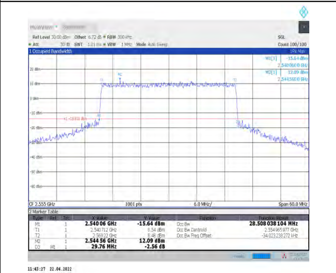
1-N7--15-30-H-7-CP-16QAM-Outer_Full-160@0-Ant 1-28.509-29.760-<30-PASS
