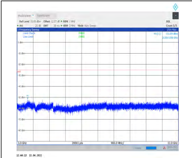
1-N7--15-40-L-1-DFT-PI2BPSK-Inner_1RB_Left-1@ 1-3000-12000-Ant1--51.69--25-PASS
