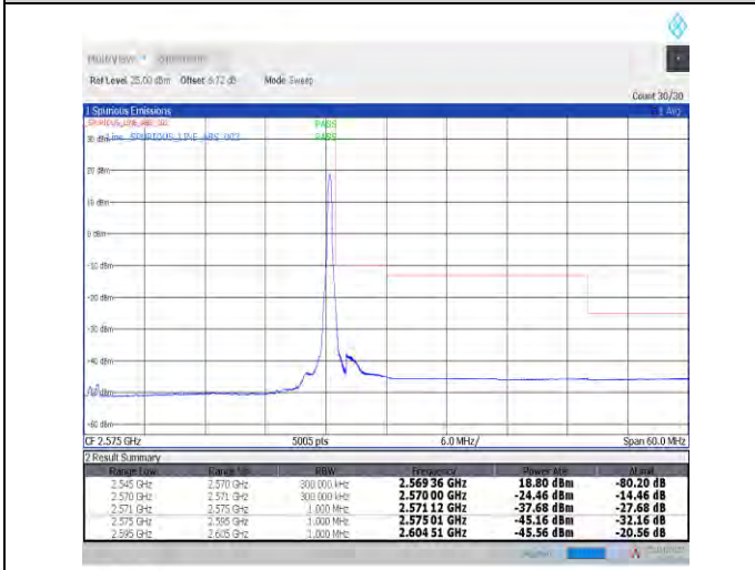
1-N7--15-25-H-2-DFT-PI2BPSK-Edge_1RB_Right-1@1 32-Ant1-PASS-see graph
