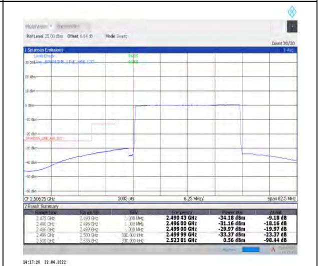
1-N7--15-25-L-6-CP-QPSK-Outer_Full-133@0-Ant1-PASS-see graph
