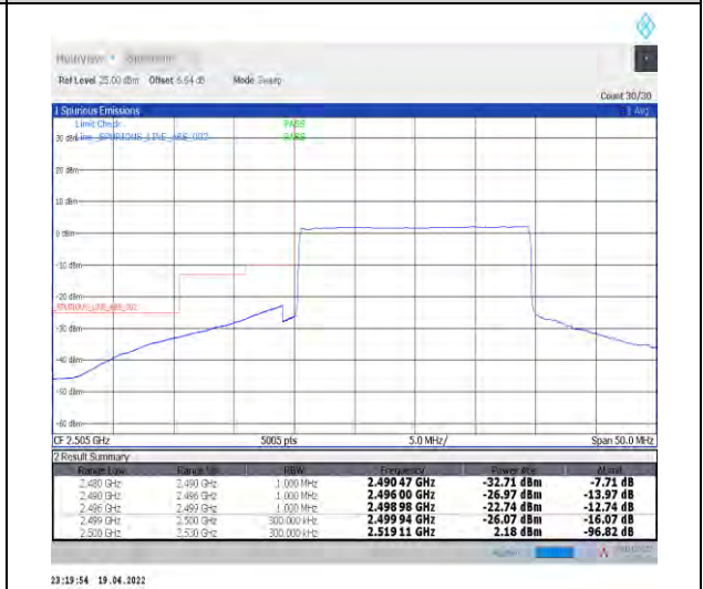
1-N7--15-20-L-6-CP-QPSK-Outer_Full-106@0-Ant1-PASS-see graph
