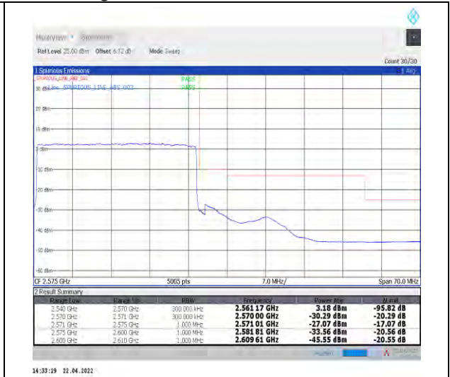
1-N7--15-30-H-3-DFT-PI2BPSK-Outer_Full-160@0-Ant1-PASS-see graph
