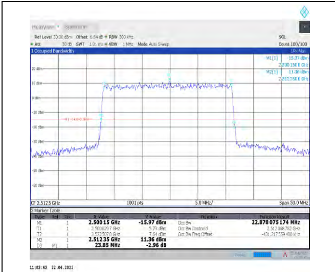
1-N7--15-25-L-5-DFT-256QAM-Outer_Full-128@0-A nt1-22.878-23.850-≤25-PASS
