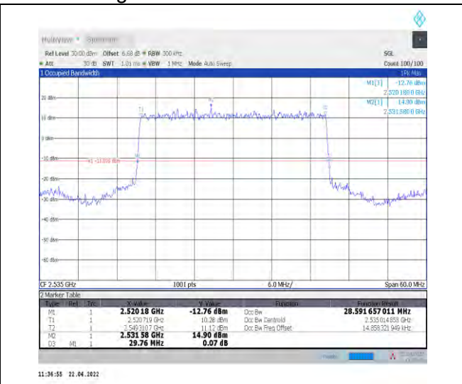
1-N7--15-30-M-2-DFT-PI2BPSK-Outer_Full-160@0-Ant1-28.592-29.760-≤30-PASS
