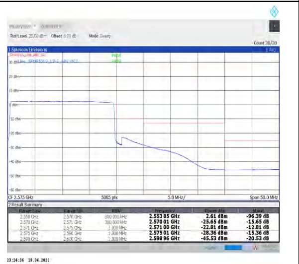
1-N7--15-20-H-6-CP-QPSK-Outer_Full-106@0-An t1-PASS-see graph
