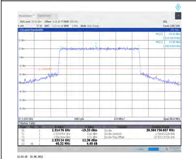
1-N7--15-40-M-8-CP-64QAM-Outer_Full-216@0-Ant 1-38.585-40.320-≤40-PASS
