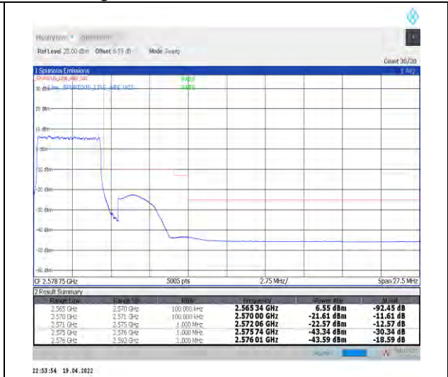
1-N7--15-5-H-3-DFT-PI2BPSK-Outer_Full-25@0-Ant1-PASS-see graph
