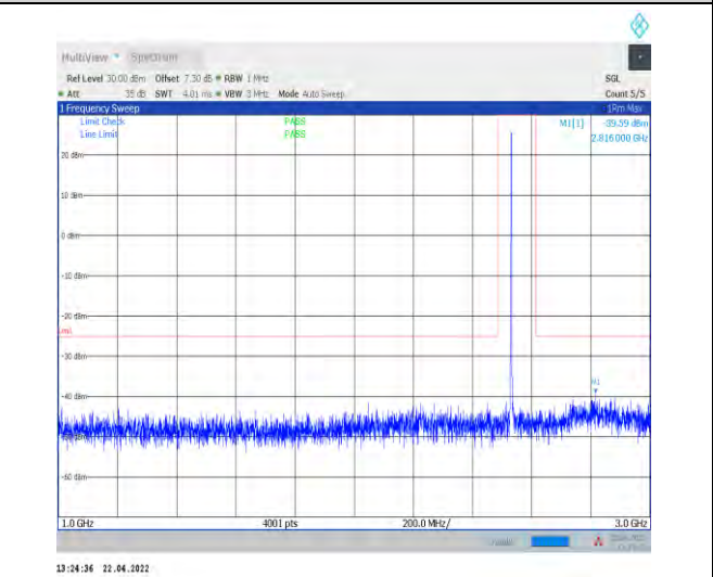
1-N7--15-40-H-1-DFT-PI2BPSK-Inner_1RB_Left-1@ 1-1000-3000-Ant1--39.59--25-PASS
