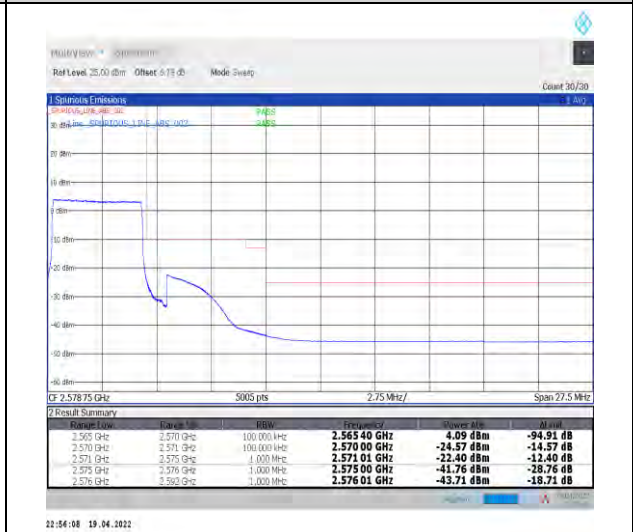
1-N7--15-5-H-6-CP-QPSK-Outer_Full-25@0-Ant1-PASS-see graph
