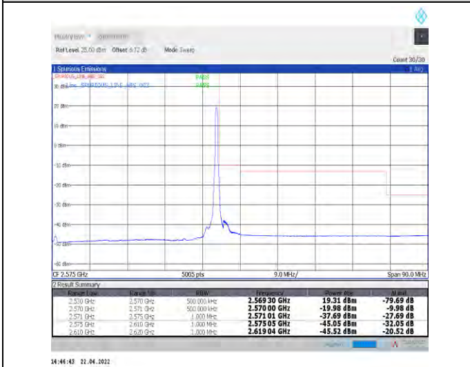
1-N7--15-40-H-5-CP-QPSK-Edge_1RB_Right-1@215- Ant1-PASS-see graph
