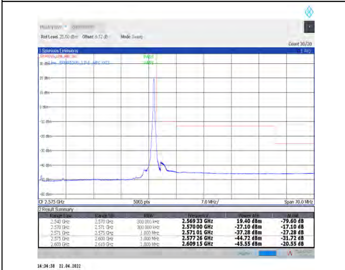
1-N7--15-30-H-5-CP-QPSK-Edge_1RB_Right-1@159-Ant1-PASS-see graph
