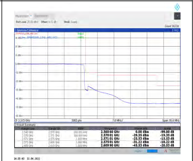
1-N7--15-30-H-6-CP-QPSK-Outer_Full-160@0-Ant1-PASS-see graph
