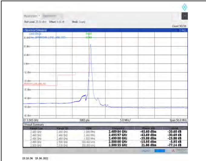
1-N7--15-20-L-1-DFT-PI2BPSK-Edge_1RB_Left-1@0-Ant1-PASS-see graph
