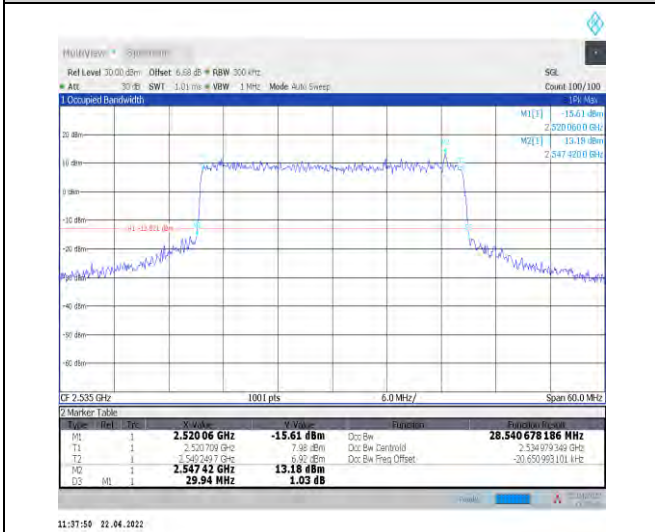
1-N7--15-30-M-7-CP-16QAM-Outer_Full-160@0-Ant 1-28.541-29.940-≤30-PASS
