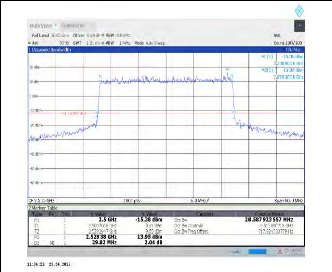
1-N7--15-30-L-1-DFT-QPSK-Outer_Full-160@0-Ant1 -28.589-29.820-≤30-PASS
