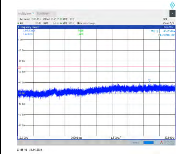
1-N7--15-40-M-1-DFT-PI2BPSK-Inner_1RB_Left-1 @1-12000-27000-Ant1--40.42--25-PASS
