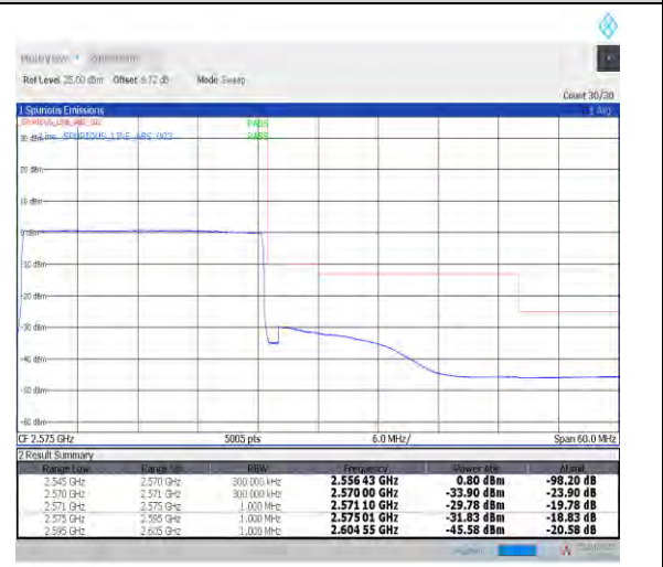
1-N7--15-25-H-3-DFT-PI2BPSK-Outer_Full-128@ 0-Ant1-PASS-see graph
