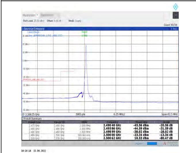
1-N7--15-25-L-4-CP-QPSK-Edge_1RB_Left-1@0-Ant1-PASS-see graph
