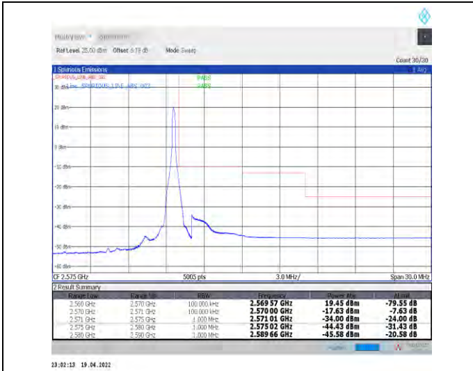
1-N7--15-10-H-2-DFT-PI2BPSK-Edge_1RB_Right-1@5 1-Ant1-PASS-see graph
