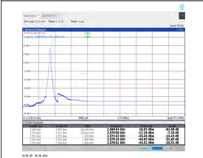
1-N7--15-5-H-5-CP-QPSK-Edge_1RB_Right-1@24-Ant1-PASS-see graph
