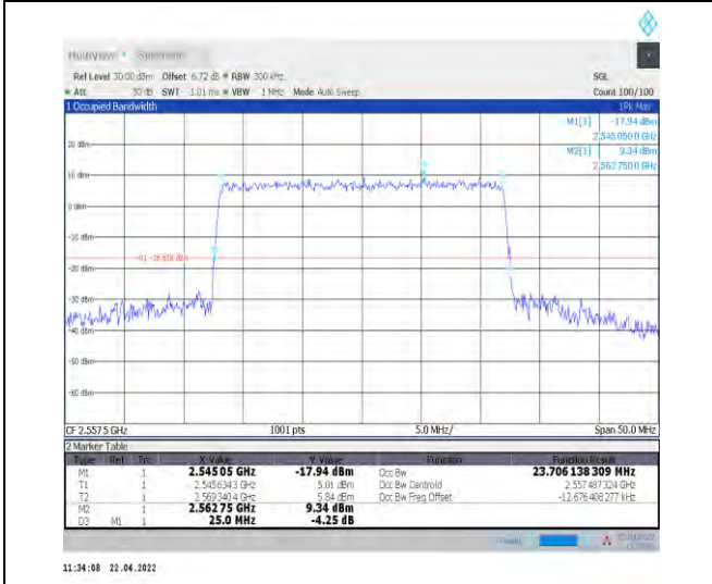
1-N7--15-25-H-9-CP-256QAM-Outer_Full-133@0-Ant t1-23.706-25.000-≤25-PASS
