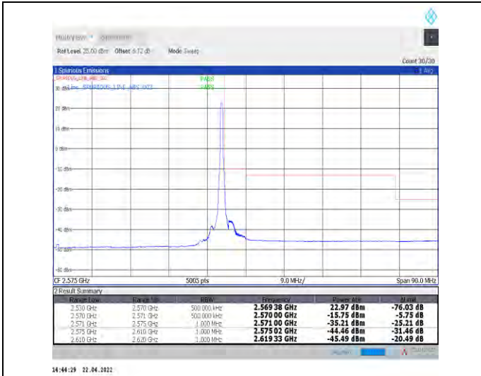
1-N7--15-40-H-2-DFT-PI2BPSK-Edge_1RB_Right-1@2 15-Ant1-PASS-see graph
