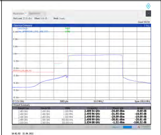
1-N7--15-40-L-6-CP-QPSK-Outer_Full-216@0-Ant1-PASS-see graph
