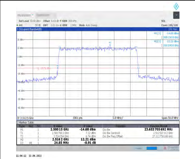
1-N7--15-25-L-8-CP-64QAM-Outer_Full-133@0-Ant 1-23.654-24.850-≤25-PASS
