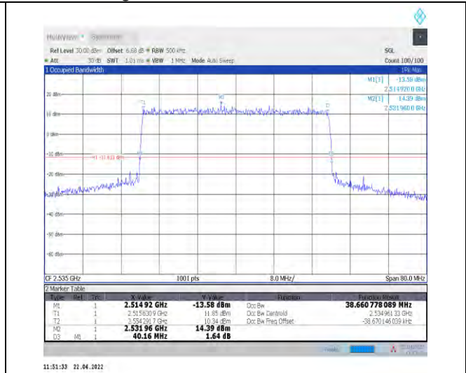
1-N7--15-40-M-3-DFT-16QAM-Outer_Full-216@0-Ant1-38.64-40.160-≤40-PASS
