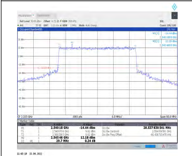
1-N7--15-30-H-6-CP-QPSK-Outer_Full-160@0-Ant1- 28.539-29.700-<30-PASS
