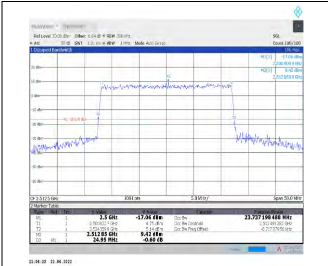
1-N7--15-25-L-9-CP-256QAM-Outer_Full-133@0-An t1-23.737-24.950-<=25-PASS
