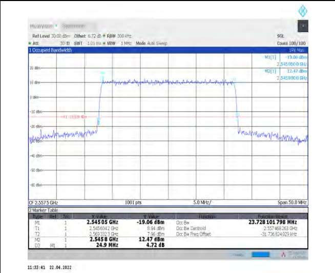
1-N7--15-25-H-6-CP-QPSK-Outer_Full-133@0-Ant1- 23.728-24.900-<math>\leq 25</math>-PASS
