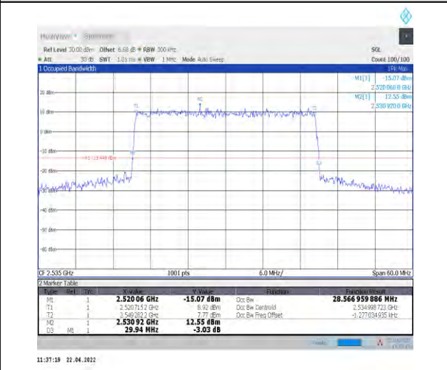
1-N7--15-30-M-4-DFT-64QAM-Outer_Full-160@0-Ant t1-28.567-29.940-≤30-PASS
