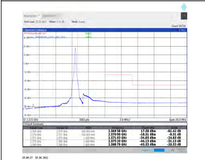
1-N7--15-10-H-5-CP-QPSK-Edge_1RB_Right-1@51-A nt1-PASS-see graph
