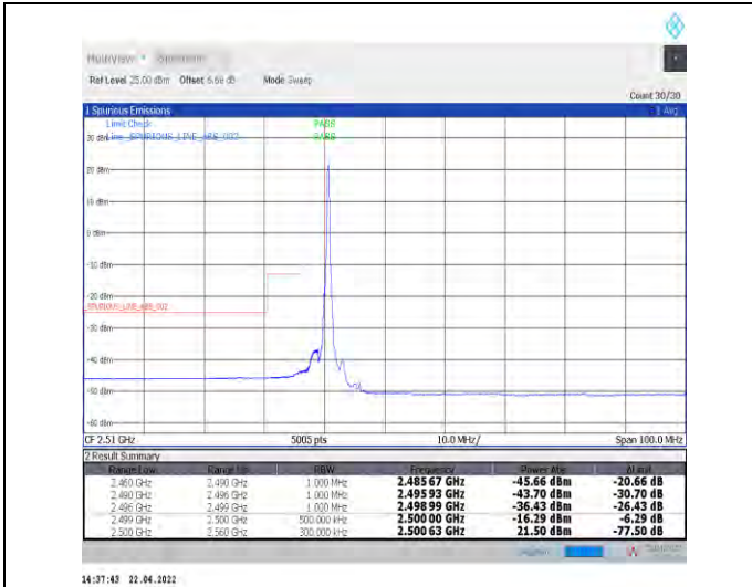
1-N7--15-40-L-1-DFT-PI2BPSK-Edge_1RB_Left-1@0-Ant1-PASS-see graph
