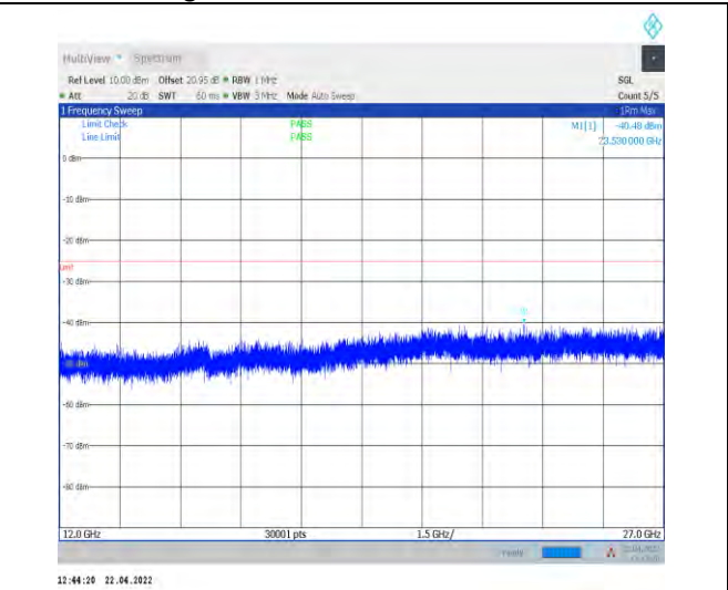
1-N7--15-40-L-1-DFT-PI2BPSK-Inner_1RB_Left-1@1 -12000-27000-Ant1--40.48--25-PASS
