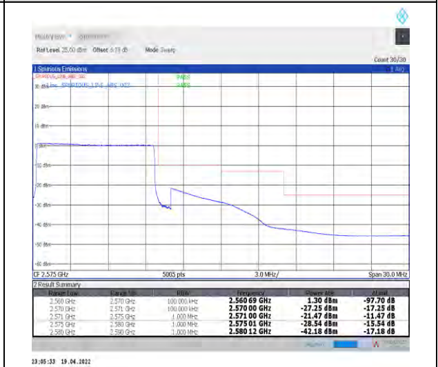
1-N7--15-10-H-6-CP-QPSK-Outer_Full-52@0-Ant 1-PASS-see graph
