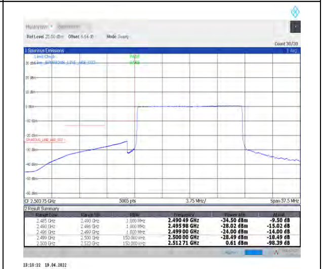
1-N7--15-15-L-6-CP-QPSK-Outer_Full-79@0-Ant1-PASS-see graph
