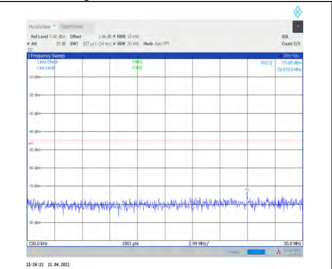
1-N7--15-40-H-1-DFT-PI2BPSK-Inner_1RB_Left-1@ 1-0.15-30-Ant1--75.05--45-PASS
