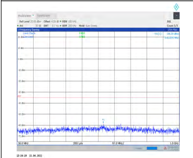
1-N7--15-40-H-1-DFT-PI2BPSK-Inner_1RB_Left-1@ 1-30-1000-Ant1--58.20--35-PASS
