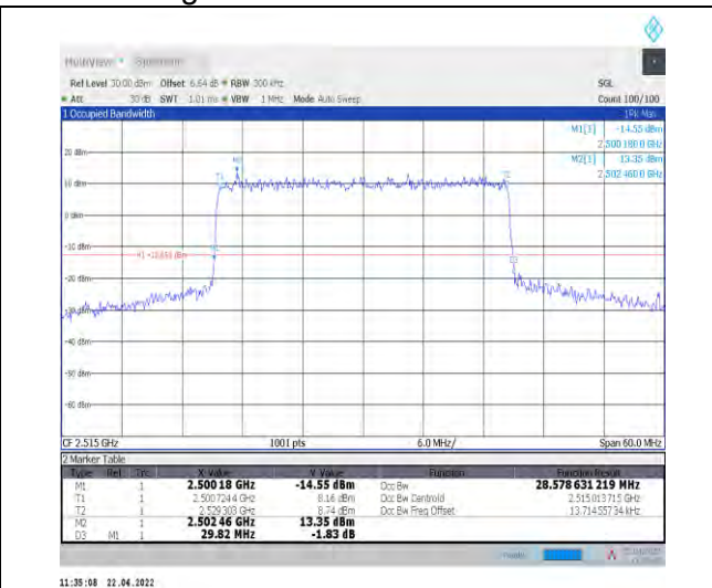
1-N7--15-30-L-3-DFT-16QAM-Outer_Full-160@0-Ant 1-28.579-29.820-≤30-PASS
