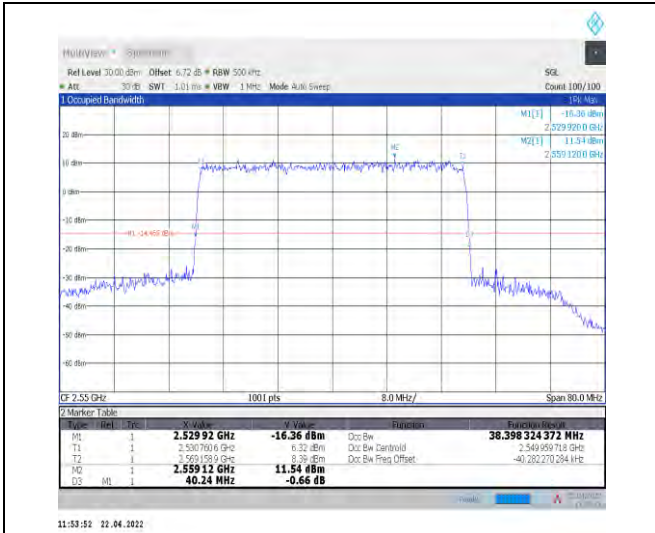
1-N7--15-40-H-5-DFT-256QAM-Outer_Full-216@0-A nt1-38.398-40.240-≤40-PASS
