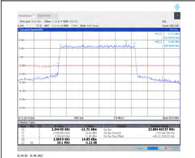
1-N7--15-25-H-1-DFT-QPSK-Outer_Full-128@0-Ant 1-22.884-24.100-≤25-PASS
