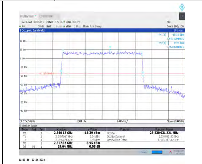
1-N7--15-30-H-9-CP-256QAM-Outer_Full-160@0-Ant 1-28.533-29.640-≤30-PASS
