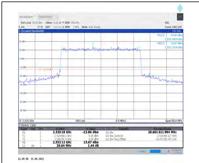
1-N7--15-30-M-1-DFT-QPSK-Outer_Full-160@0-Ant 1-28.602-29.640-≤30-PASS
