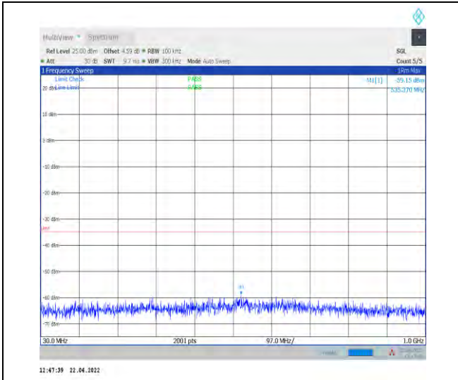
1-N7--15-40-M-1-DFT-PI2BPSK-Inner_1RB_Left-1 @1-30-1000-Ant1--59.15--35-PASS
