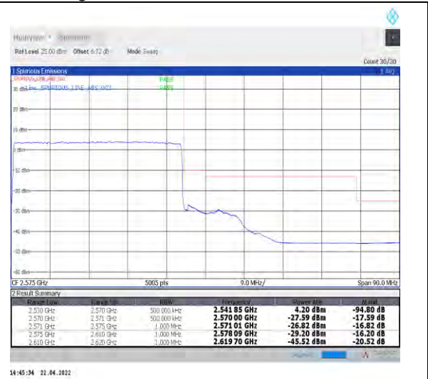
1-N7--15-40-H-3-DFT-PI2BPSK-Outer_Full-216@ 0-Ant1-PASS-see graph
