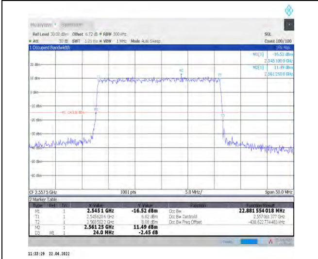
1-N7--15-25-H-5-DFT-256QAM-Outer_Full-128@0-A nt1-22.882-24.000-<math>\leq 25</math>-PASS
