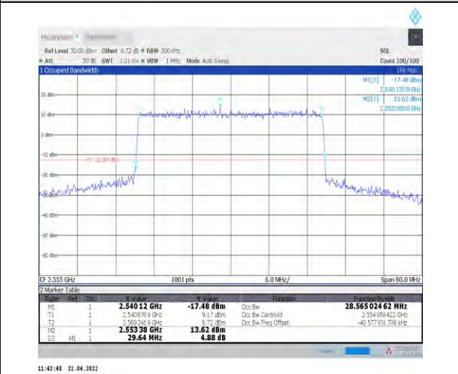
1-N7--15-30-H-3-DFT-16QAM-Outer_Full-160@0-Ant t1-28.565-29.640-≤30-PASS
