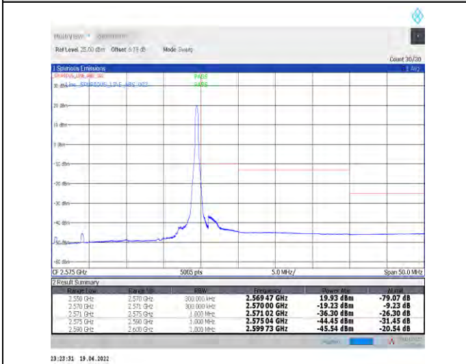
1-N7--15-20-H-5-CP-QPSK-Edge_1RB_Right-1@105- Ant1-PASS-see graph
