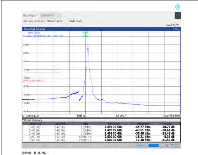
1-N7--15-10-L-4-CP-QPSK-Edge_1RB_Left-1@0-Ant1-PASS-see graph
