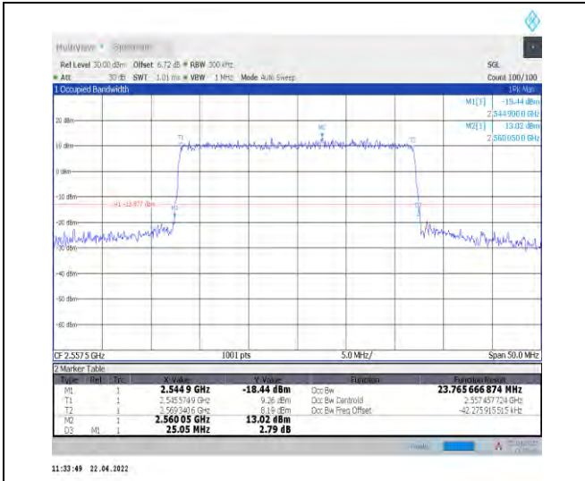
1-N7--15-25-H-7-CP-16QAM-Outer_Full-133@0-Ant 1-23.766-25.050-≤25-PASS
