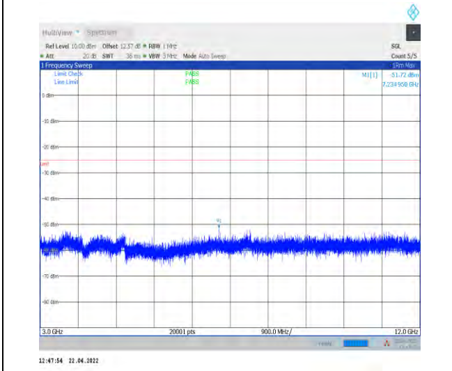
1-N7--15-40-M-1-DFT-PI2BPSK-Inner_1RB_Left-1 @1-3000-12000-Ant1--51.72--25-PASS
