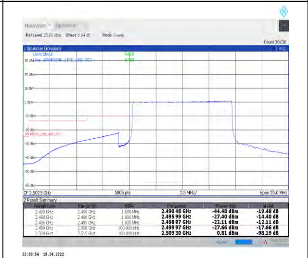
1-N7--15-10-L-6-CP-QPSK-Outer_Full-52@0-Ant1-PASS-see graph
