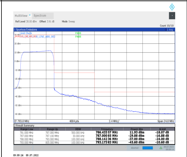
1-N13-PC3-15-5-H-6-CP-QPSK-Outer_Full-25@0-Ant1-PASS-see graph
