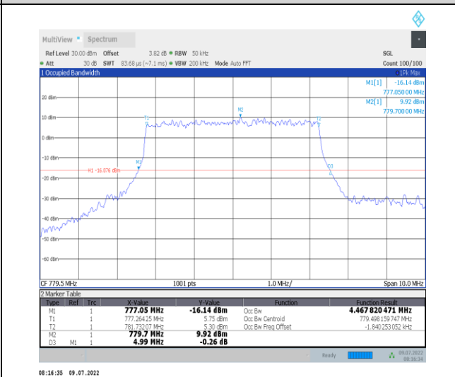
1-N13--15-5-L-8-CP-64QAM-Outer_Full-25@0-Ant1- 4.468-4.990-≤5-PASS
