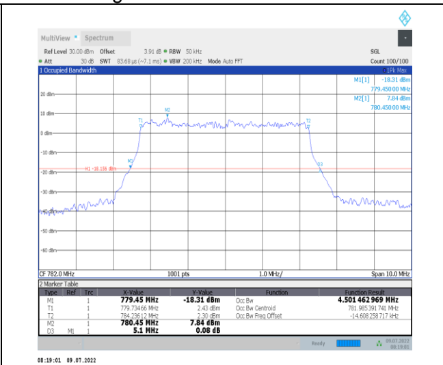
1-N13--15-5-M-9-CP-256QAM-Outer_Full-25@0-Ant 1-4.501-5.100-≤5-PASS
