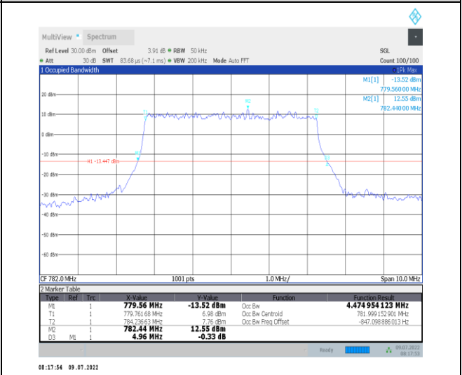
1-N13--15-5-M-3-DFT-16QAM-Outer_Full-25@0-Ant1 1-4.475-4.960≤5-PASS
