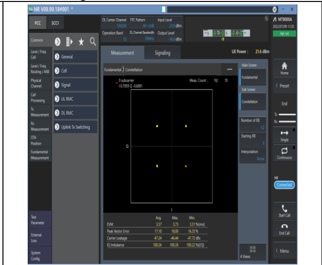
1-N13--15-10-M-6-CP-QPSK-Outer_Full-52@0-Ant 1-see graph-PASS
