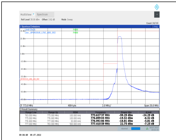
1-N13-PC3-15-5-L-1-DFT-PI2BPSK-Edge_1RB_Left-1 @0-Ant1-PASS-see graph
