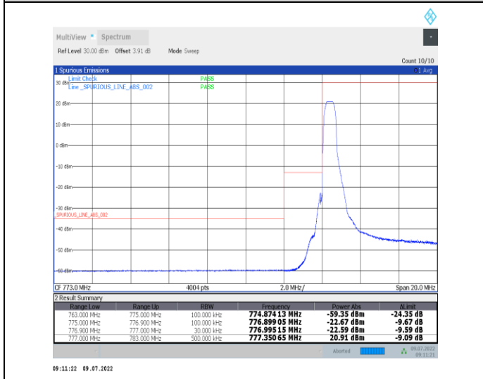
1-N13-PC3-15-10-L-4-CP-QPSK-Edge_1RB_Left-1@0-Ant1-PASS-see graph
