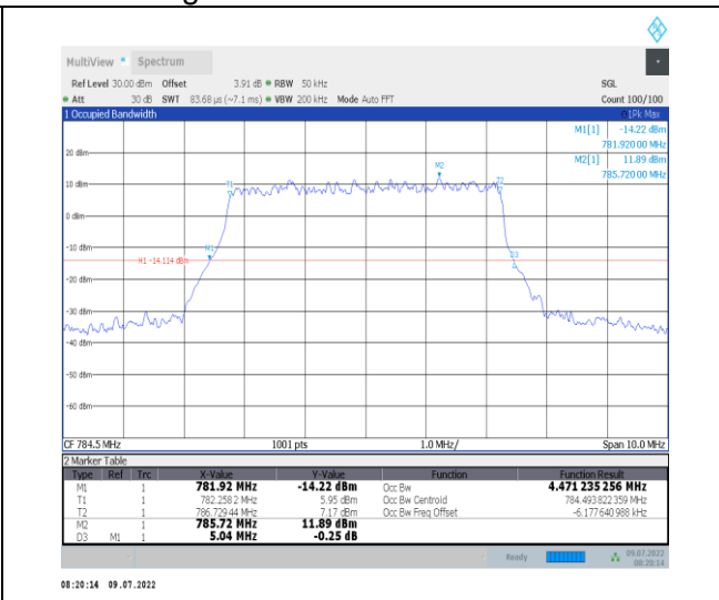
1-N13--15-5-H-4-DFT-64QAM-Outer_Full-25@0-Ant 1-4.471-5.040-≤5-PASS
