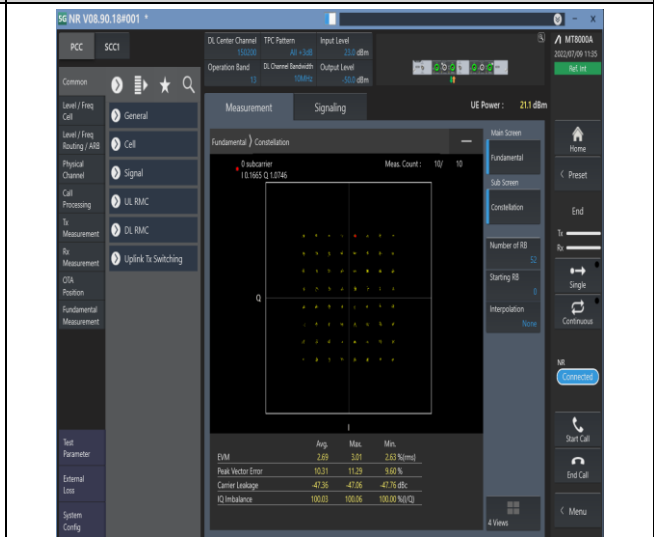
1-N13--15-10-M-8-CP-64QAM-Outer_Full-52@0-Ant1 -see graph-PASS
