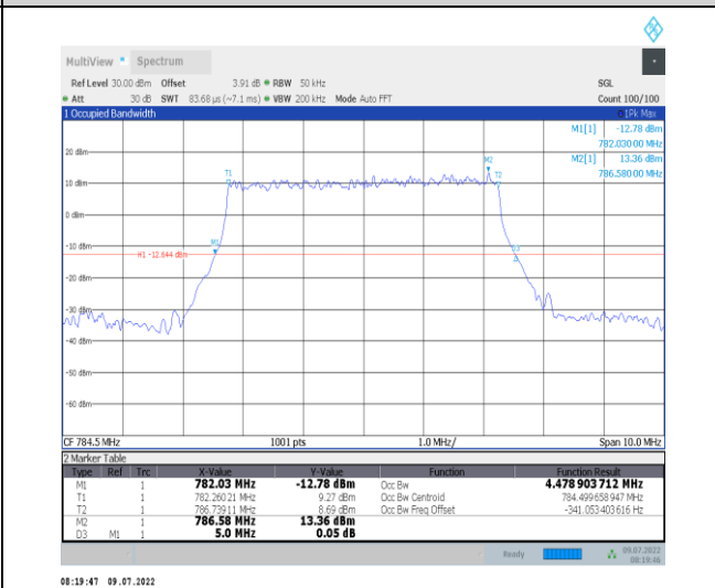
1-N13--15-5-H-2-DFT-PI2BPSK-Outer_Full-25@0-A nt1-4.479-5.000-≤5-PASS
