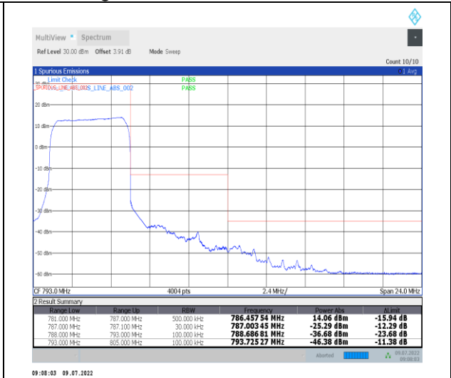
1-N13-PC3-15-5-H-3-DFT-PI2BPSK-Outer_Full-25@0-Ant1-PASS-see graph
