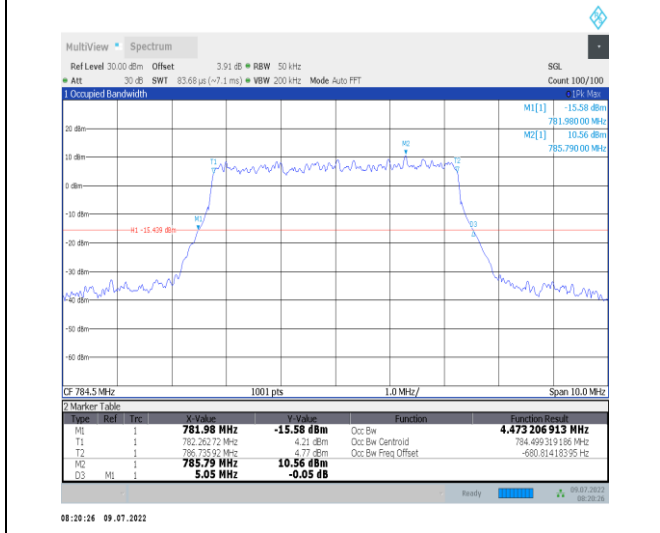
1-N13--15-5-H-5-DFT-256QAM-Outer_Full-25@0-Ant t1-4.473-5.050-≤5-PASS
