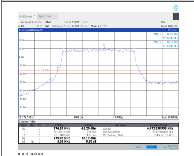
1-N13--15-5-L-7-CP-16QAM-Outer_Full-25@0-Ant1- 4.473-5.080-≤5-PASS
