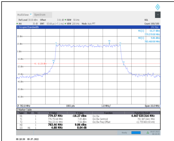
1-N13--15-5-M-8-CP-64QAM-Outer_Full-25@0-Ant1 -4.468-4.880-≤5-PASS
