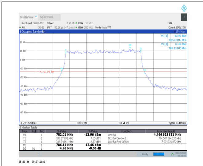
1-N13--15-5-H-3-DFT-16QAM-Outer_Full-25@0-Ant 1-4.467-4.960-≤5-PASS
