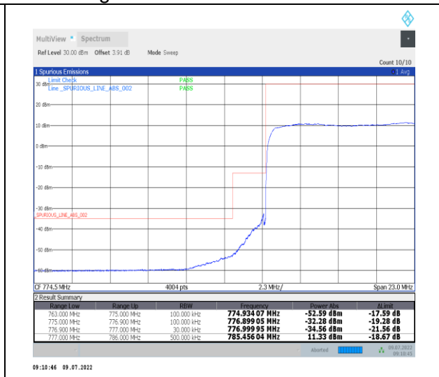
1-N13-PC3-15-10-L-3-DFT-PI2BPSK-Outer_Full-50@0-Ant1-PASS-see graph
