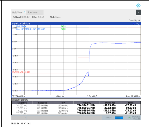
1-N13-PC3-15-10-L-6-CP-QPSK-Outer_Full-52@0-Ant1-PASS-see graph
