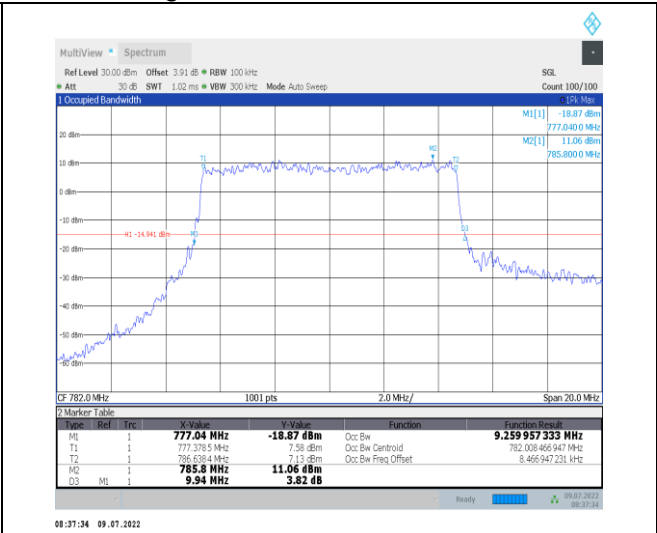
1-N13--15-10-M-7-CP-16QAM-Outer_Full-52@0-Ant 1-9.26-9.940-≤10-PASS
