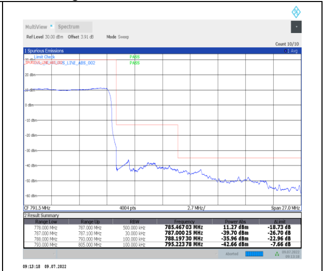
1-N13-PC3-15-10-H-3-DFT-PI2BPSK-Outer_Full-5 0@0-Ant1-PASS-see graph
