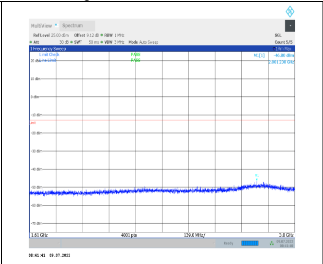
1-N13--15-10-M-1-DFT-PI2BPSK-Inner_1RB_Left-1 @ 1-1610-3000-Ant1--46.80--13-PASS
