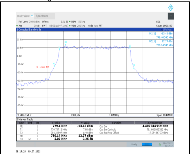
1-N13--15-5-M-1-DFT-QPSK-Outer_Full-25@0-Ant1 -4.49-5.070≤5-PASS
