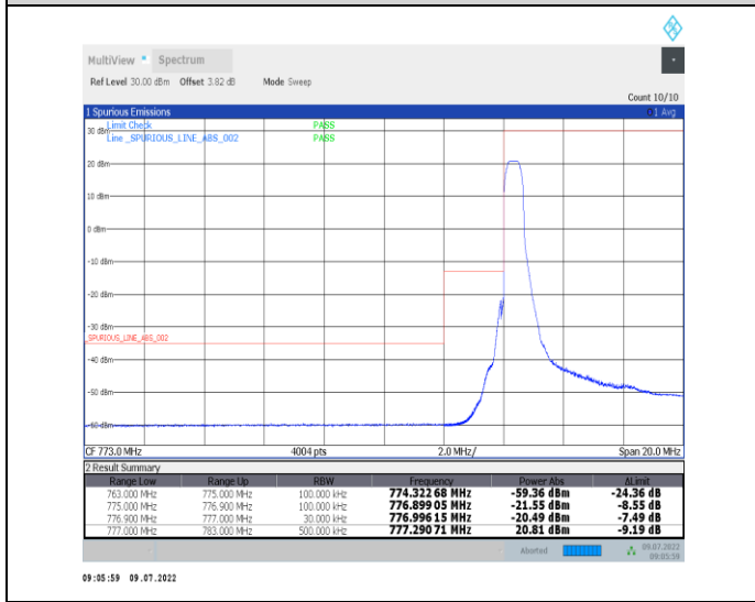
1-N13-PC3-15-5-L-4-CP-QPSK-Edge_1RB_Left-1 @0- Ant1-PASS-see graph
