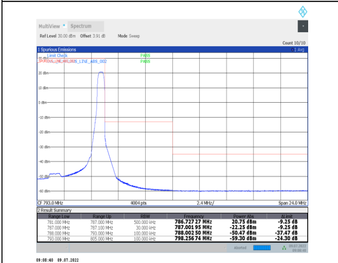
1-N13-PC3-15-5-H-5-CP-QPSK-Edge_1RB_Right-1@24-Ant1-PASS-see graph
