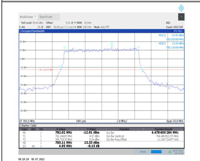
1-N13--15-5-H-1-DFT-QPSK-Outer_Full-25@0-Ant1- 4.479-4.950-≤5-PASS
