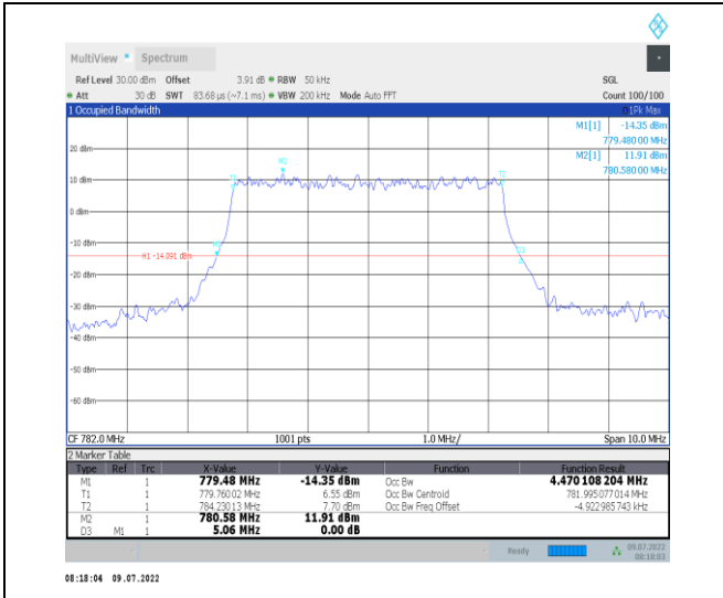
1-N13--15-5-M-4-DFT-64QAM-Outer_Full-25@0-Ant 1-4.47-5.060-≤5-PASS
