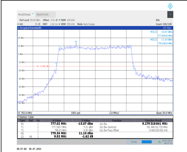
1-N13--15-10-M-8-CP-64QAM-Outer_Full-52@0-Ant 1-9.279-9.920-≤10-PASS
