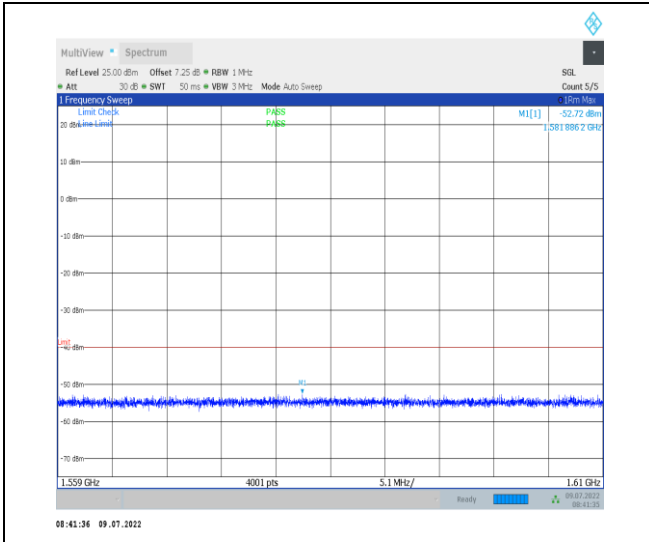
1-N13--15-10-M-1-DFT-PI2BPSK-Inner_1RB_Left-1 @ 1-1559-1610-Ant1--52.72--40-PASS
