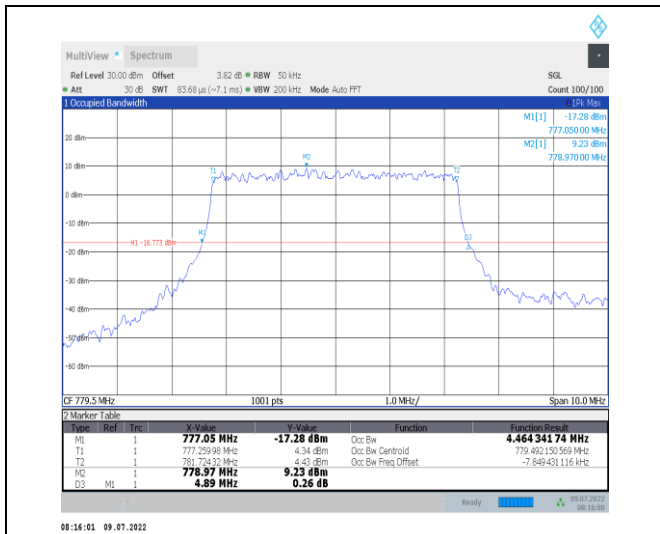
1-N13--15-5-L-5-DFT-256QAM-Outer_Full-25@0-Ant 1-4.464-4.890-≤5-PASS
