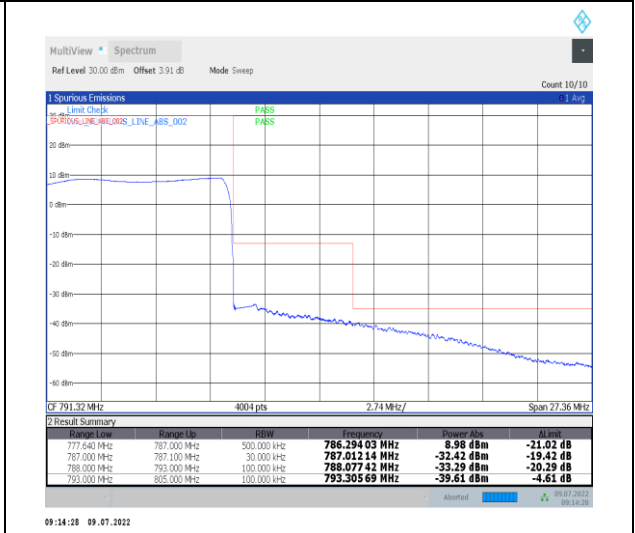
1-N13-PC3-15-10-H-6-CP-QPSK-Outer_Full-52@ 0-Ant1-PASS-see graph
