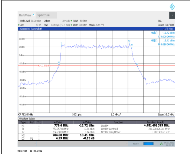
1-N13--15-5-M-2-DFT-PI2BPSK-Outer_Full-25@0-Ant1 -4.481-4.990≤5-PASS
