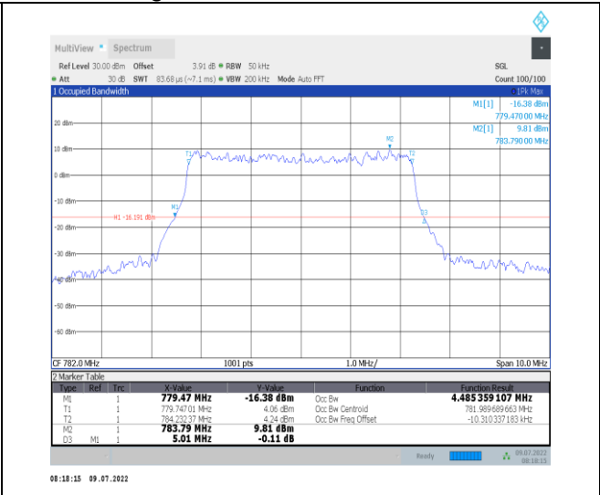
1-N13--15-5-M-5-DFT-256QAM-Outer_Full-25@0-A nt1-4.485-5.010-≤5-PASS
