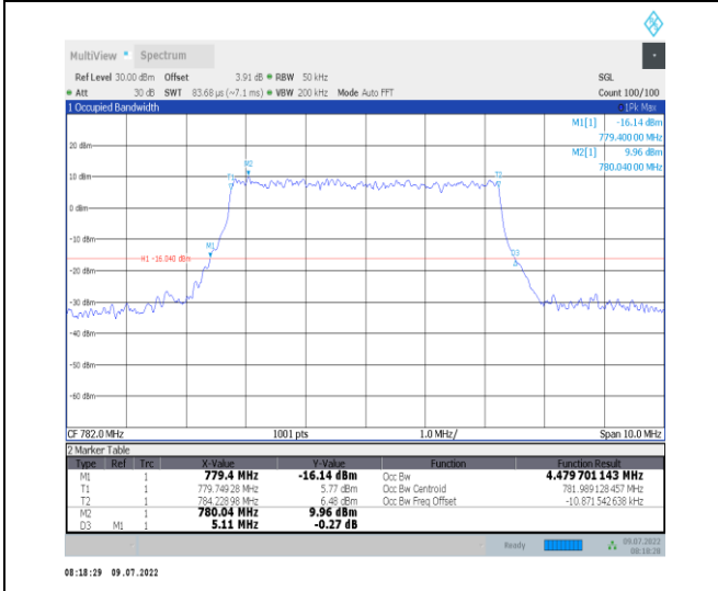
1-N13--15-5-M-6-CP-QPSK-Outer_Full-25@0-Ant1-4 .48-5.110-≤5-PASS
