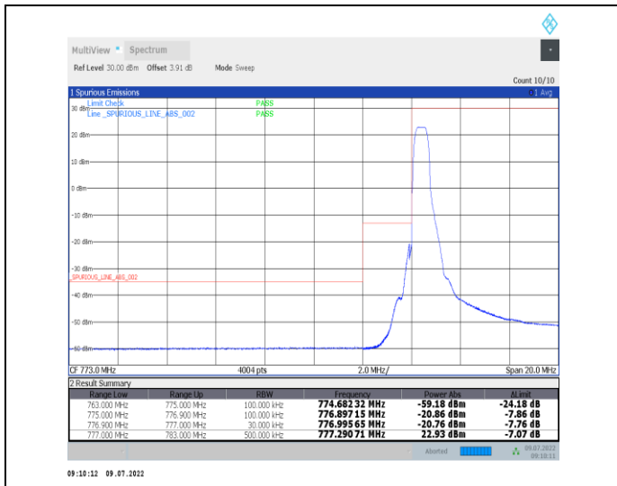
1-N13-PC3-15-10-L-1-DFT-PI2BPSK-Edge_1RB_Left-1@0-Ant1-PASS-see graph
