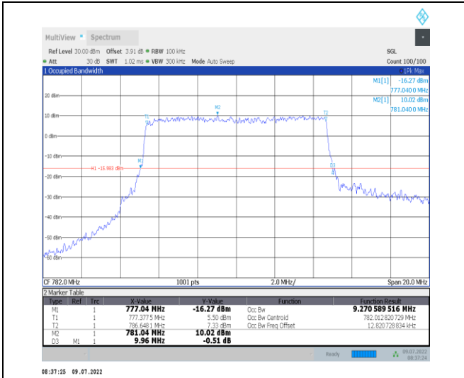
1-N13--15-10-M-6-CP-QPSK-Outer_Full-52@0-Ant-1-9.271-9.960-≤10-PASS
