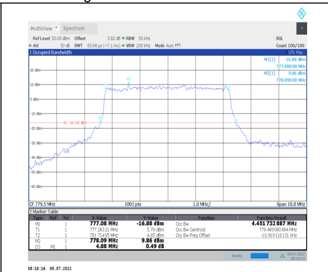
1-N13--15-5-L-6-CP-QPSK-Outer_Full-25@0-Ant1-4 .452-4.880-≤5-PASS
