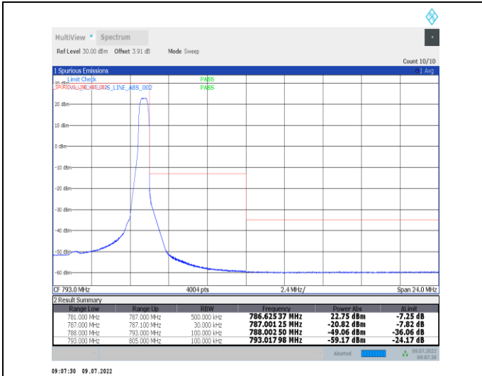
1-N13-PC3-15-5-H-2-DFT-PI2BPSK-Edge_1RB_Right-1@24-Ant1-PASS-see graph
