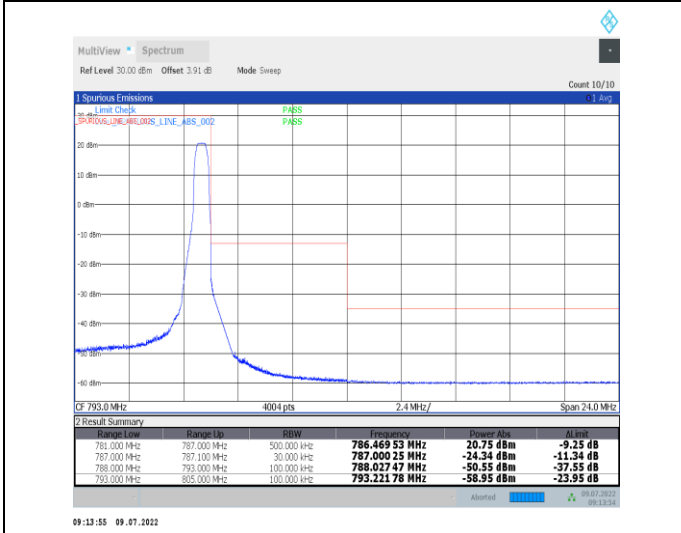
1-N13-PC3-15-10-H-5-CP-QPSK-Edge_1RB_Right-1 @51-Ant1-PASS-see graph
