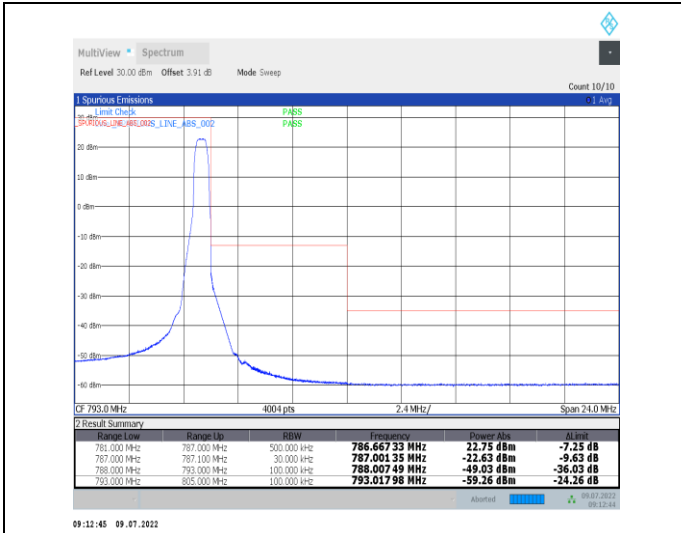
1-N13-PC3-15-10-H-2-DFT-PI2BPSK-Edge_1RB_Right -1@51-Ant1-PASS-see graph
