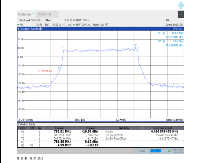
1-N13--15-5-H-6-CP-QPSK-Outer_Full-25@0-Ant1-4 .457-4.990-≤5-PASS
