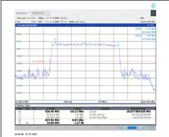
1-N26-824-849--15-20-M-9-CP-256QAM-Outer_Full-1 106@0-Ant1-18.878-19.960-≤20-PASS
