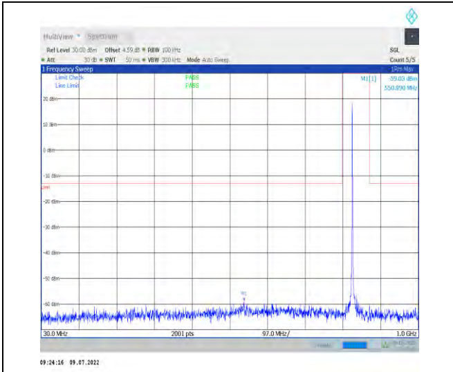
1-N26-824-849-PC3-15-20-H-1-DFT-PI2BPSK-Inner _1RB_Left-1@1-30-1000-Ant1--59.03--23-PASS
