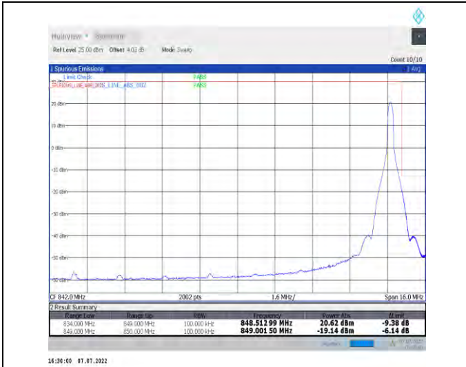
1-N26-824-849--15-15-H-2-DFT-PI2BPSK-Edge_1RB_Right-1@78-Ant1-seegraph-PASS-see graph
