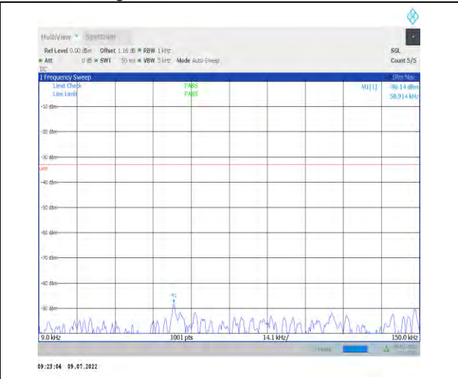
1-N26-824-849-PC3-15-20-M-1-DFT-PI2BPSK-Inner _1RB_Left-1@1-0.009-0.15-Ant1--88.14--43-PASS
