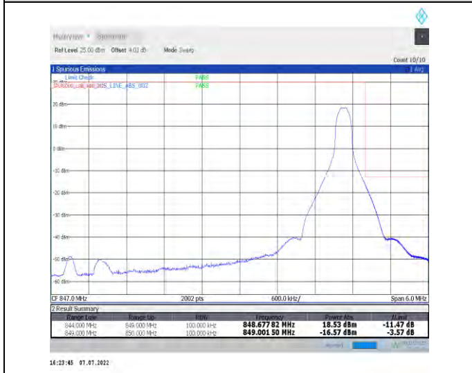
1-N26-824-849--15-5-H-5-CP-QPSK-Edge_1RB_Right-1@24-Ant1-seegraph-PASS-see graph
