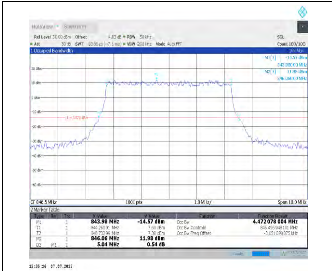
1-N26-824-849--15-5-H-3-DFT-16QAM-Outer_Full-2 5@0-Ant1-4.472-5.040-≤5-PASS
