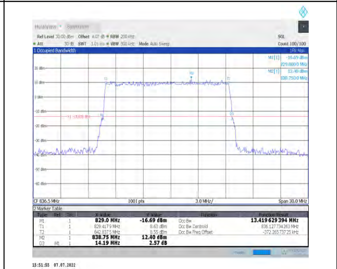
1-N26-824-849--15-15-M-5-DFT-256QAM-Outer_Full-75@0-Ant1-13.42-14.190-≤15-PASS
