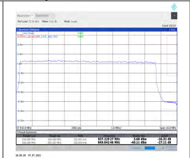
1-N26-824-849--15-15-H-3-DFT-PI2BPSK-Outer_Full-75@0-Ant1-seegraph-PASS-see graph
