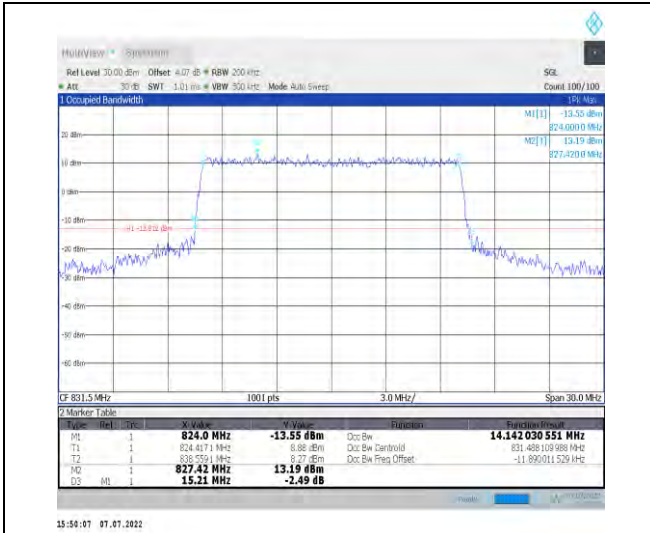
1-N26-824-849--15-15-L-7-CP-16QAM-Outer_Full-7 9@0-Ant1-14.142-15.210-≤15-PASS
