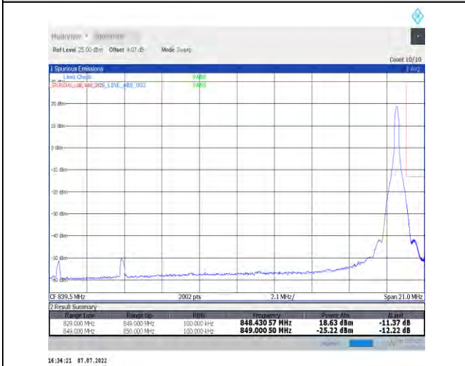
1-N26-824-849--15-20-H-5-CP-QPSK-Edge_1RB_Right-1@105-Ant1-seegraph-PASS-see graph
