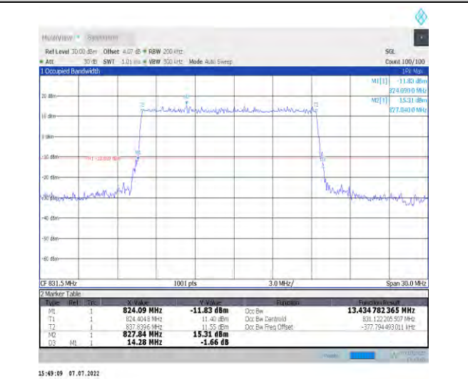
1-N26-824-849--15-15-L-2-DFT-PI2BPSK-Outer_Full 75@0-Ant1-13.435-14.280-<=15-PASS
