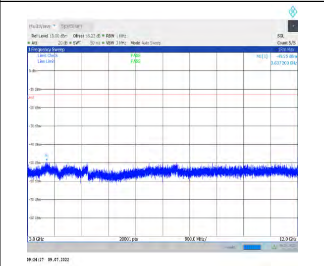
1-N26-824-849-PC3-15-20-H-1-DFT-PI2BPSK-Inner _1RB_Left-1@1-3000-12000-Ant1--49.25--13-PASS
