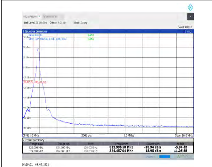
1-N26-824-849--15-15-L-4-CP-QPSK-Edge_1RB_Left-1@0-Ant1-seegraph-PASS-see graph
