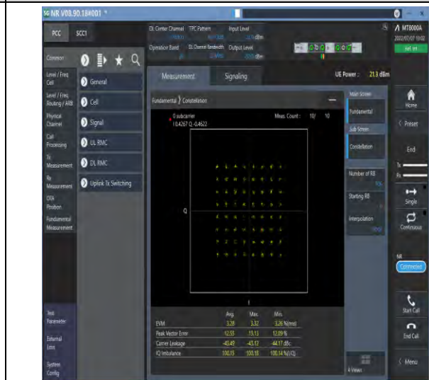
1-N26-824-849--15-20-M-8-CP-64QAM-Outer_Full-106@0-Ant1-see graph-PASS
