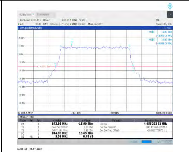
1-N26-824-849--15-5-H-6-CP-QPSK-Outer_Full-2 @0-Ant1-4.455-5.010-≤5-PASS
