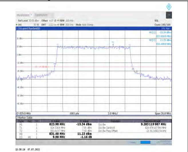
1-N26-824-849--15-10-L-7-CP-16QAM-Outer_Full-5 2@0-Ant1-9.283-9.980-≤10-PASS
