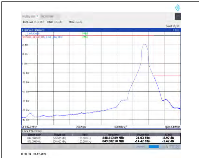
1-N26-824-849--15-5-H-2-DFT-PI2BPSK-Edge_1RB_Right-1@24-Ant1-seegraph-PASS-see graph
