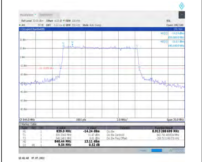
1-N26-824-849--15-10-H-3-DFT-16QAM-Outer_Full-50@0-Ant1-8.913-9.540-≤10-PASS
