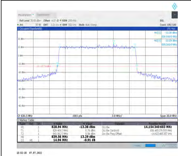
1-N26-824-849--15-15-M-8-CP-64QAM-Outer_Full-7 9@0-Ant1-14.154-14.940-≤15-PASS
