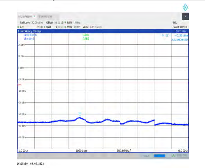
1-N26-824-849-PC3-15-20-H-1-DFT-PI2BPSK-Inner _1RB_Left-1@1-1000-6000-Ant1--42.36--13-PASS
