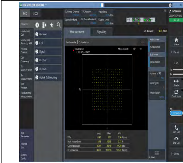
1-N26-824-849--15-20-M-9-CP-256QAM-Outer_Full-106@0-Ant1-see graph-PASS
