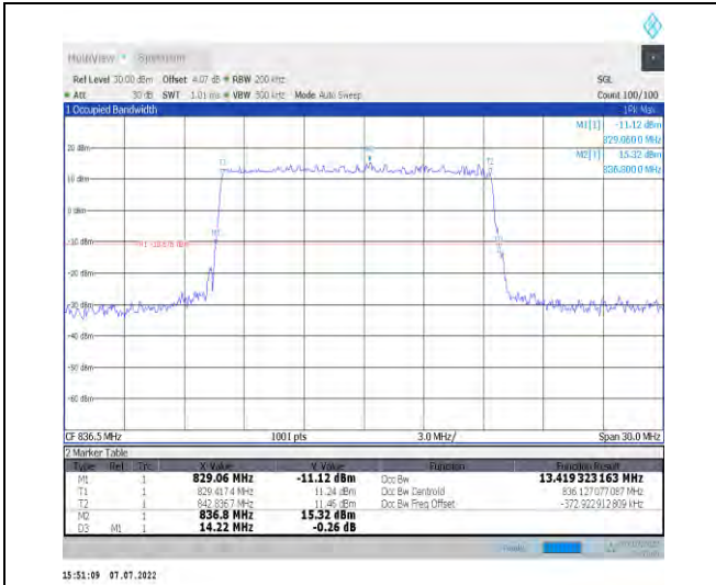
1-N26-824-849--15-15-M-2-DFT-PI2BPSK-Outer_Fu II-75@0-Ant1-13.419-14.220-≤15-PASS
