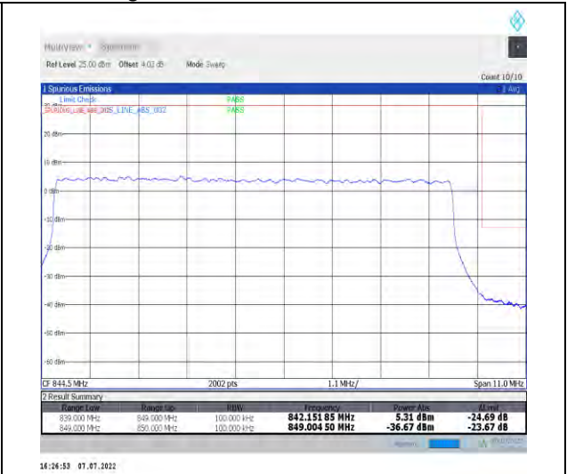
1-N26-824-849--15-10-H-3-DFT-PI2BPSK-Outer_Full-50@0-Ant1-seegraph-PASS-see graph
