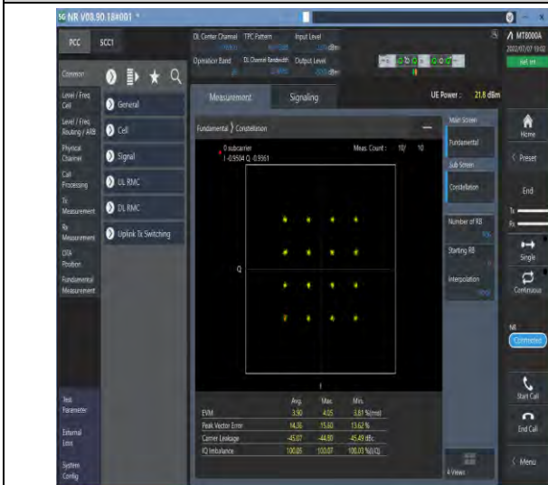
1-N26-824-849--15-20-M-7-CP-16QAM-Outer_Full-106@0-Ant1-see graph-PASS
