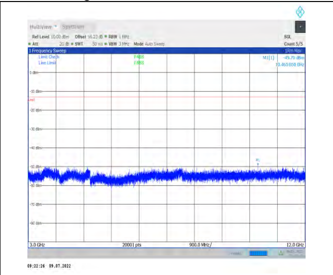
1-N26-824-849-PC3-15-20-L-1-DFT-PI2BPSK-Inner _1RB_Left-1@1-3000-12000-Ant1--49.70--13-PASS
