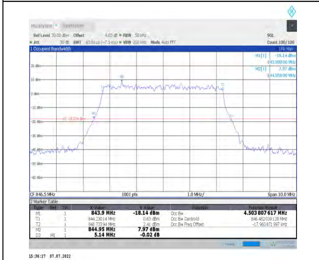
1-N26-824-849--15-5-H-9-CP-256QAM-Outer_Full-2 5@0-Ant1-4.504-5.140-<math>\leq</math>5-PASS
