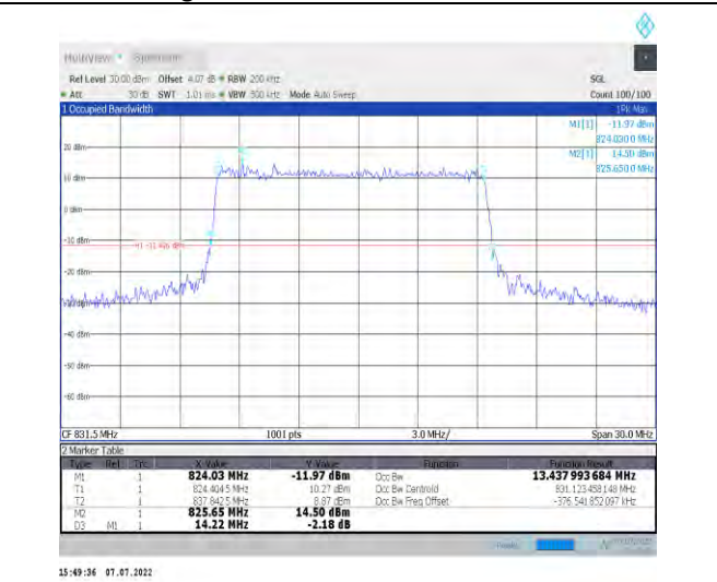
1-N26-824-849--15-15-L-4-DFT-64QAM-Outer_Full-75@0-Ant1-13.438-14.220-≤15-PASS
