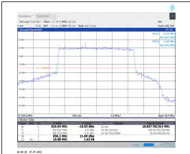
1-N26-824-849--15-20-H-6-CP-QPSK-Outer_Full-10 6@0-Ant1-18.858-19.880-≤20-PASS
