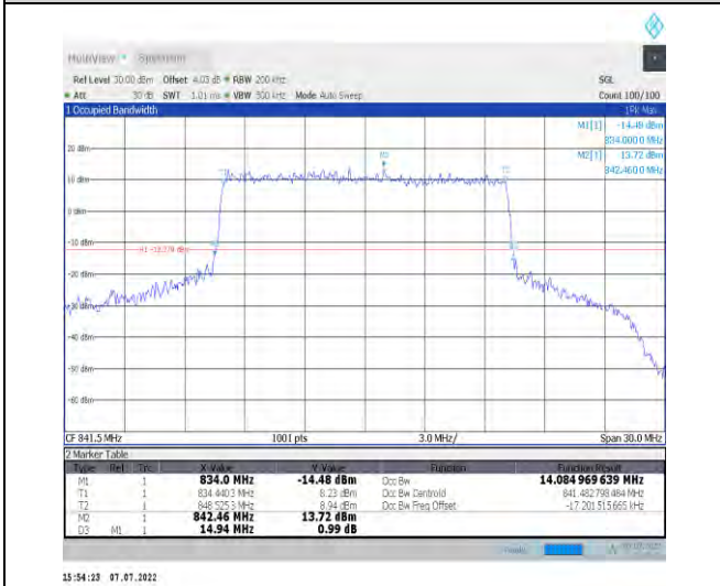
1-N26-824-849--15-15-H-7-CP-16QAM-Outer_Full-7 9@0-Ant1-14.085-14.940≤15-PASS
