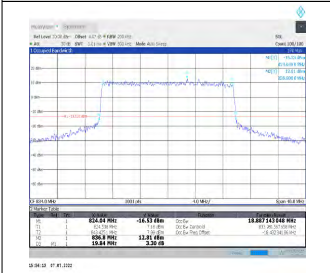
1-N26-824-849--15-20-L-6-CP-QPSK-Outer_Full-106@0-Ant1-18.887-19.840-<math>\leq 20</math>-PASS
