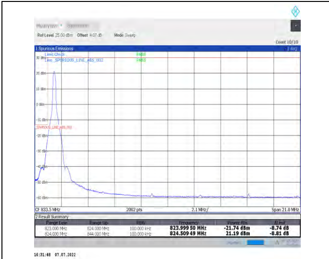
1-N26-824-849--15-20-L-1-DFT-PI2BPSK-Edge_1RB_Left-1@0-Ant1-seegraph-PASS-see graph
