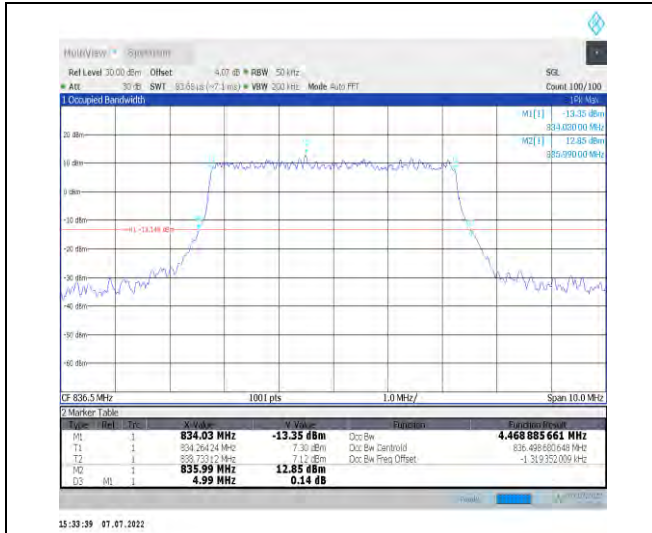
1-N26-824-849--15-5-M-4-DFT-64QAM-Outer_Full-25@0-Ant1-4.469-4.990-≤5-PASS
