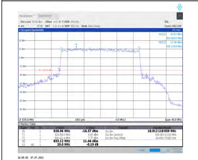
1-N26-824-849--15-20-H-8-CP-64QAM-Outer_Full-1 06@0-Ant1-18.912-20.000-≤20-PASS
