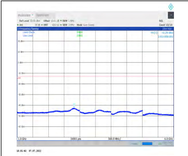
1-N26-824-849-PC3-15-20-L-1-DFT-PI2BPSK-Inner _1RB_Left-1@1-1000-6000-Ant1--42.20--13-PASS
