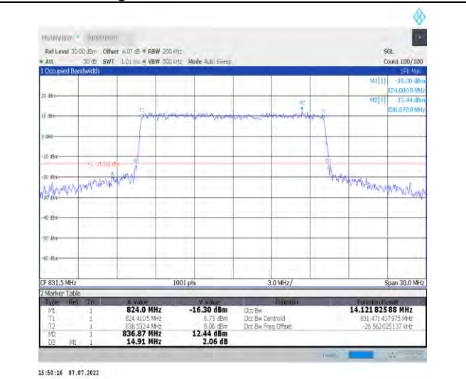
1-N26-824-849--15-15-L-8-CP-64QAM-Outer_Full-7 9@0-Ant1-14.122-14.910-≤15-PASS
