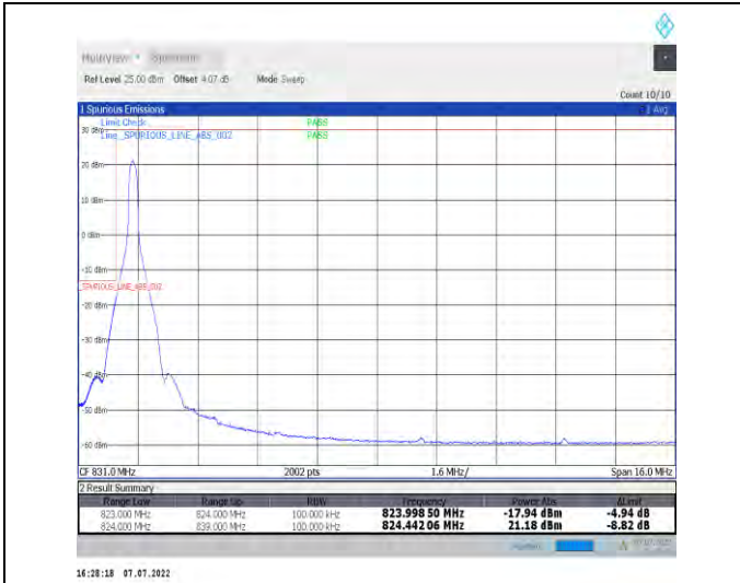
1-N26-824-849--15-15-L-1-DFT-PI2BPSK-Edge_1RB_Left-1@0-Ant1-seegraph-PASS-see graph
