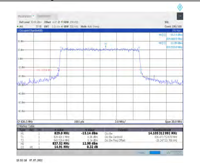
1-N26-824-849--15-15-M-7-CP-16QAM-Outer_Full-7 9@0-Ant1-14.105-14.910-≤15-PASS
