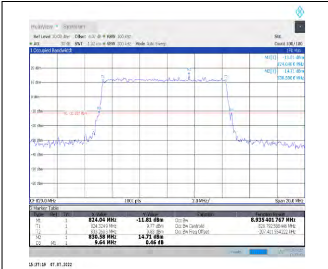
1-N26-824-849--15-10-L-2-DFT-PI2BPSK-Outer_Full-50@0-Ant1-8.935-9.640-≤10-PASS
