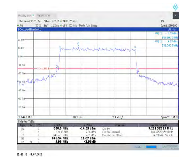
1-N26-824-849--15-10-H-8-CP-64QAM-Outer_Full-5 2@0-Ant1-9.291-9.980-<=10-PASS
