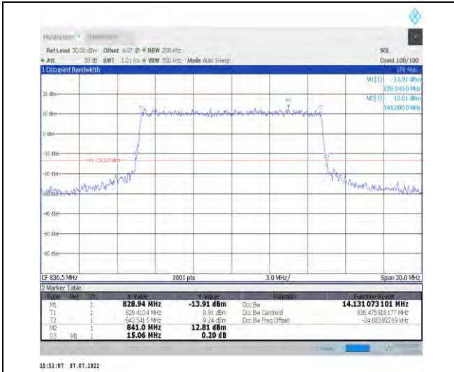
1-N26-824-849--15-15-M-6-CP-QPSK-Outer_Full-79 @0-Ant1-14.131-15.060-≤15-PASS
