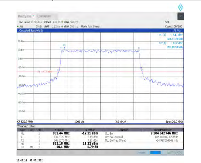
1-N26-824-849--15-10-M-6-CP-QPSK-Outer_Full-52 @0-Ant1-9.305-10.100-≤10-PASS
