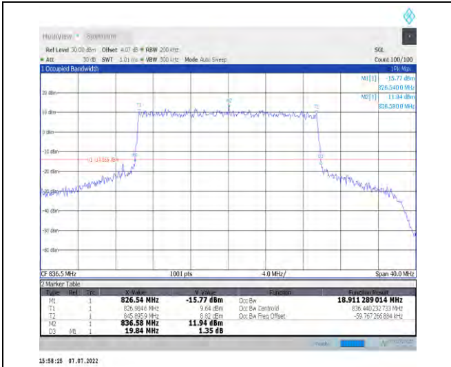
1-N26-824-849--15-20-M-7-CP-16QAM-Outer_Full-1 06@0-Ant1-18.911-19.840-≤20-PASS
