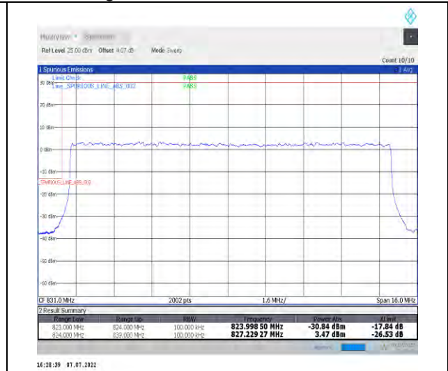
1-N26-824-849--15-15-L-3-DFT-PI2BPSK-Outer_Full-75@0-Ant1-seegraph-PASS-see graph
