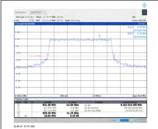
1-N26-824-849--15-10-M-7-CP-16QAM-Outer_Full-5 2@0-Ant1-9.262-10.040-≤10-PASS
