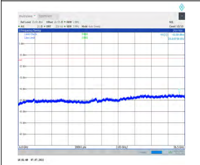
1-N26-824-849-PC3-15-20-L-1-DFT-PI2BPSK-Inner _1RB_Left-1@1-6000-26500-Ant1--43.88--13-PASS
