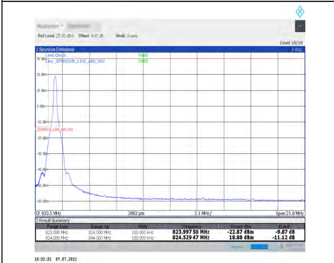
1-N26-824-849--15-20-L-4-CP-QPSK-Edge_1RB_Left-1@0-Ant1-seegraph-PASS-see graph
