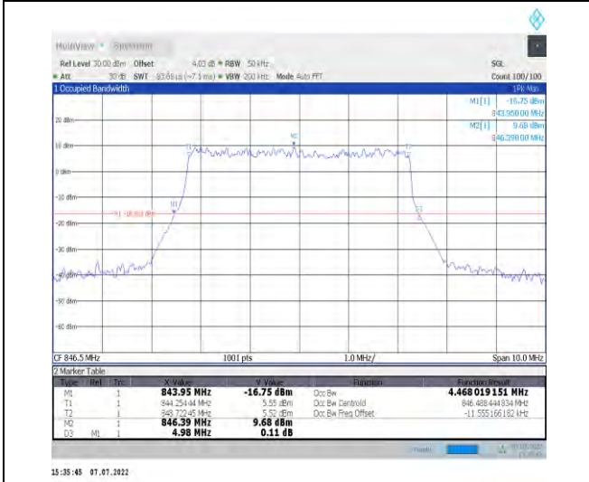
1-N26-824-849--15-5-H-5-DFT-256QAM-Outer_Full-2 25@0-Ant1-4.468-4.980-≤5-PASS
