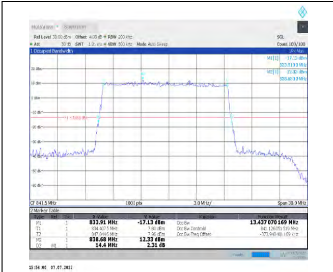
1-N26-824-849--15-15-H-5-DFT-256QAM-Outer_Full -75@0-Ant1-13.437-14.400≤15-PASS
