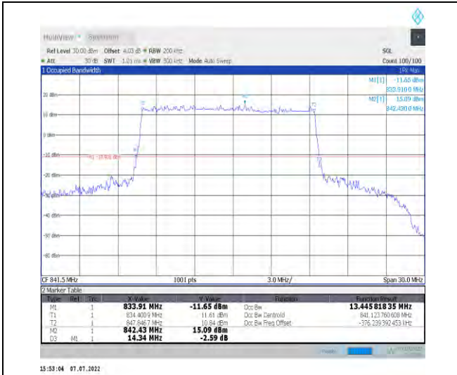
1-N26-824-849--15-15-H-1-DFT-QPSK-Outer_Full-75@0-Ant1-13.446-14.340-≤15-PASS
