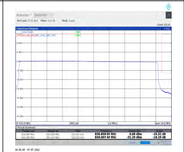
1-N26-824-849--15-15-H-6-CP-QPSK-Outer_Full-79@0-Ant1-seegraph-PASS-see graph
