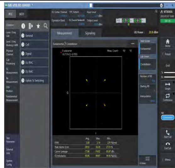
1-N26-824-849--15-20-M-2-DFT-QPSK-Outer_Full-1 00@0-Ant1-see graph-PASS
