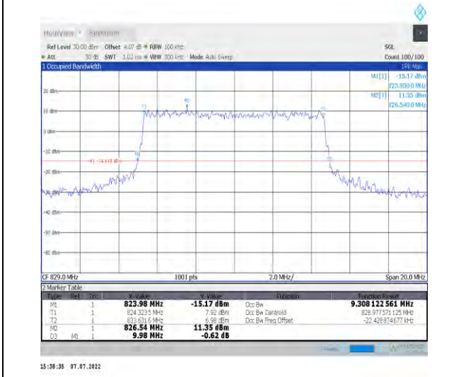
1-N26-824-849--15-10-L-8-CP-64QAM-Outer_Full-5 2@0-Ant1-9.308-9.980-≤10-PASS
