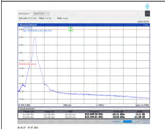
1-N26-824-849--15-10-L-4-CP-QPSK-Edge_1RB_Left-1@0-Ant1-seegraph-PASS-see graph
