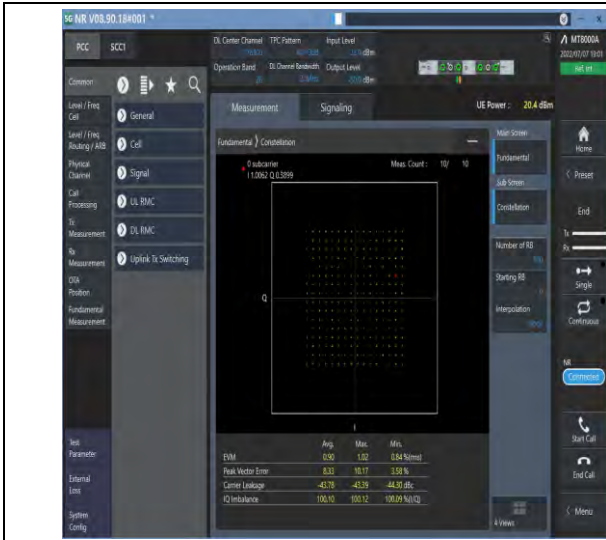
1-N26-824-849--15-20-M-5-DFT-256QAM-Outer_Full-100@0-Ant1-see graph-PASS
