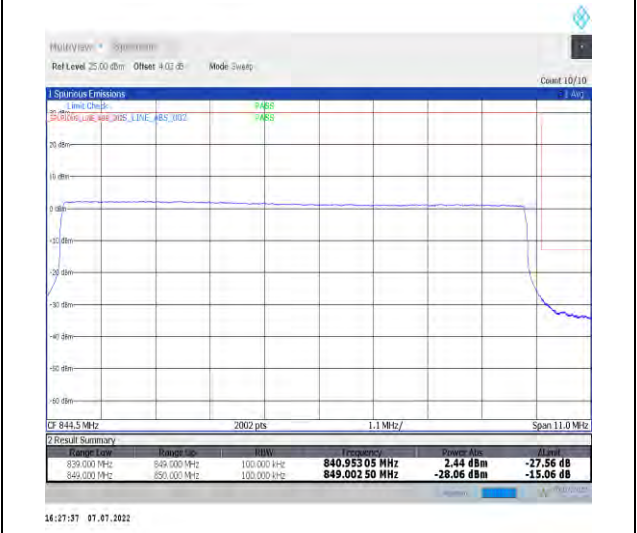
1-N26-824-849--15-10-H-6-CP-QPSK-Outer_Full-5 2@0-Ant1-seegraph-PASS-see graph
