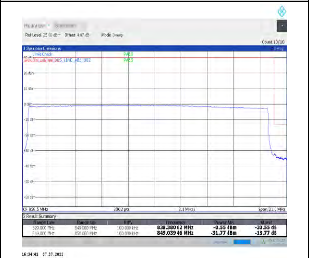
1-N26-824-849--15-20-H-6-CP-QPSK-Outer_Full-106@0-Ant1-seegraph-PASS-see graph
