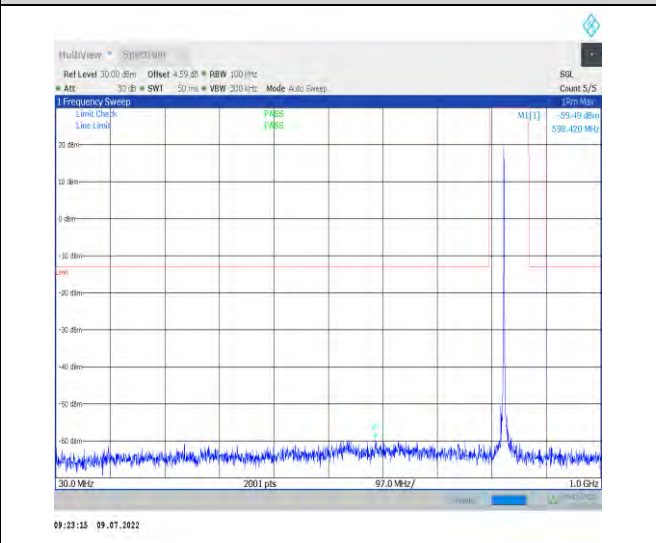
1-N26-824-849-PC3-15-20-M-1-DFT-PI2BPSK-Inner _1RB_Left-1@1-30-1000-Ant1--59.49--23-PASS
