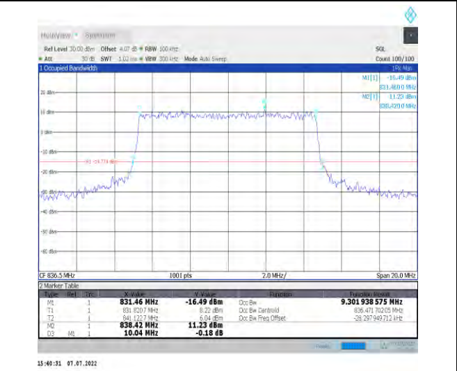
1-N26-824-849--15-10-M-8-CP-64QAM-Outer_Full-5 2@0-Ant1-9.302-10.040-≤10-PASS
