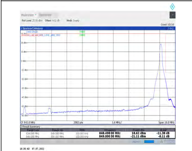
1-N26-824-849--15-15-H-5-CP-QPSK-Edge_1RB_Right-1@78-Ant1-seegraph-PASS-see graph
