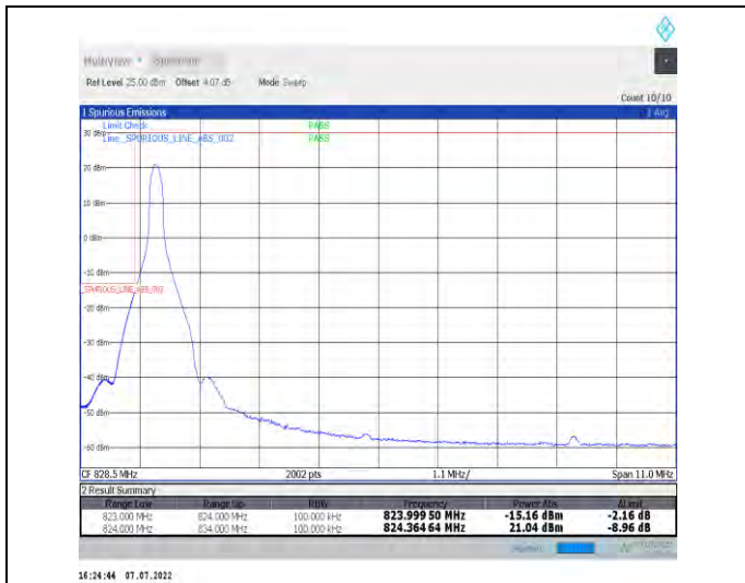
1-N26-824-849--15-10-L-1-DFT-PI2BPSK-Edge_1RB_Left-1@0-Ant1-seegraph-PASS-see graph
