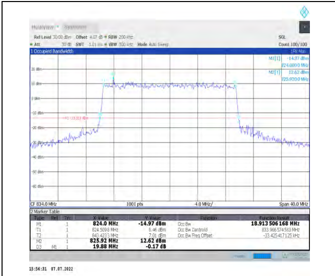
1-N26-824-849--15-20-L-8-CP-64QAM-Outer_Full-1 06@0-Ant1-18.914-19.880-≤20-PASS
