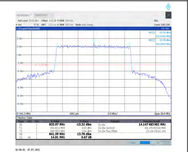
1-N26-824-849--15-15-H-8-CP-64QAM-Outer_Full-7 9@0-Ant1-14.147-14.910≤15-PASS
