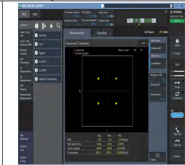
1-N26-824-849--15-20-M-6-CP-QPSK-Outer_Full-106@0-Ant1-see graph-PASS
