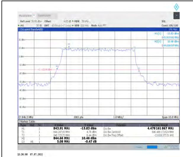
1-N26-824-849--15-5-H-7-CP-16QAM-Outer_Full-25 @0-Ant1-4.478-5.080-<math>\leq</math>5-PASS
