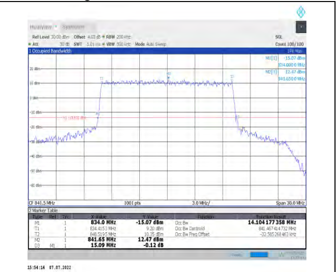
1-N26-824-849--15-15-H-6-CP-QPSK-Outer_Full-79 @0-Ant1-14.104-15.090≤15-PASS
