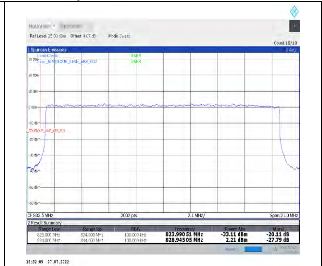
1-N26-824-849--15-20-L-3-DFT-PI2BPSK-Outer_Full-100@0-Ant1-seegraph-PASS-see graph
