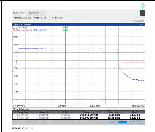
1-N26-824-849--15-5-H-6-CP-QPSK-Outer_Full-25@0-Ant1-seegraph-PASS-see graph
