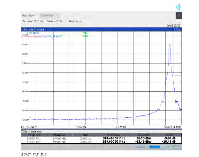
1-N26-824-849--15-20-H-2-DFT-PI2BPSK-Edge_1RB_Right-1@105-Ant1-seegraph-PASS-see graph
