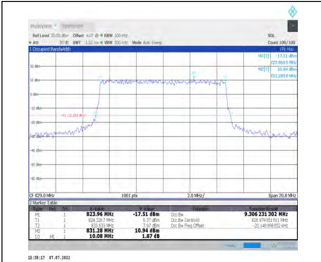
1-N26-824-849--15-10-L-6-CP-QPSK-Outer_Full-52 @0-Ant1-9.306-10.080-≤10-PASS
