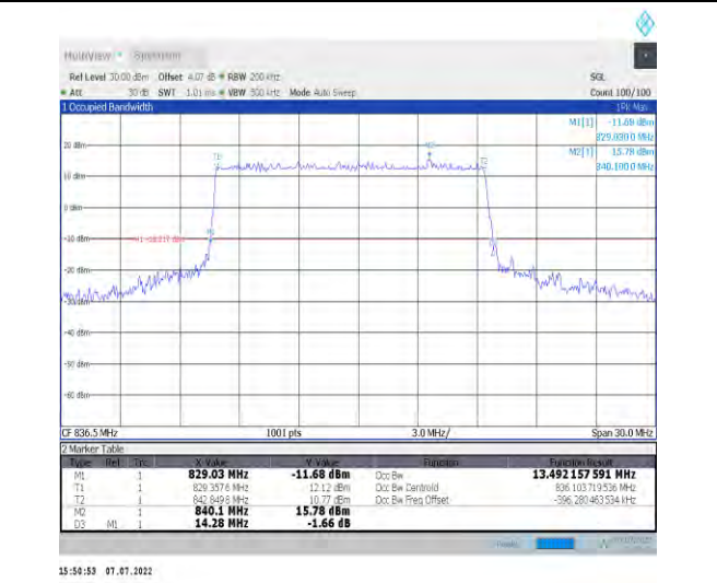
1-N26-824-849--15-15-M-1-DFT-QPSK-Outer_Full-7 5@0-Ant1-13.492-14.280-≤15-PASS
