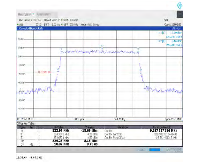
1-N26-824-849--15-10-L-9-CP-256QAM-Outer_Full- 52@0-Ant1-9.298-10.020-≤10-PASS
