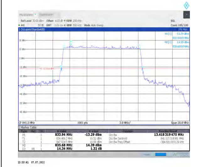
1-N26-824-849--15-15-H-3-DFT-16QAM-Outer_Full-75@0-Ant1-13.418-14.340-≤15-PASS
