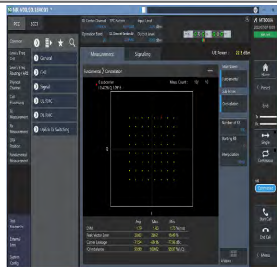
1-N26-824-849--15-20-M-4-DFT-64QAM-Outer_Full -100@0-Ant1-see graph-PASS
