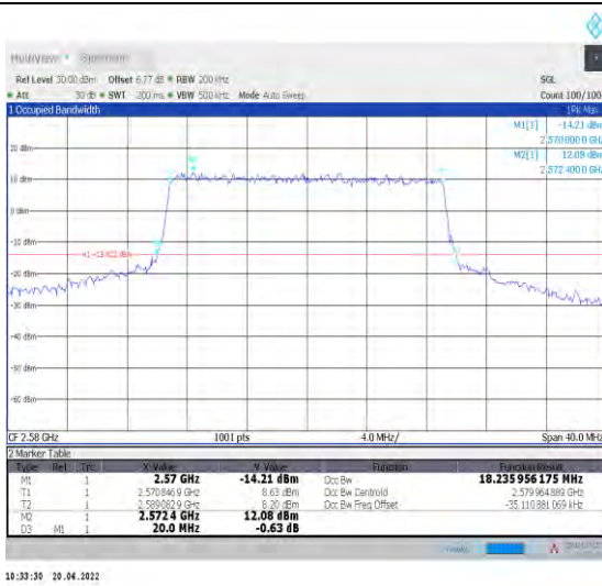
1-N38--30-20-L-7-CP-16QAM-Outer_Full-51@0-Ant1 -18.236-20.000-≤20-PASS
