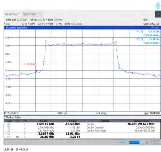
1-N38--30-30-H-3-DFT-16QAM-Outer_Full-75@0-An t1-26.862-28.860-<=30-PASS
