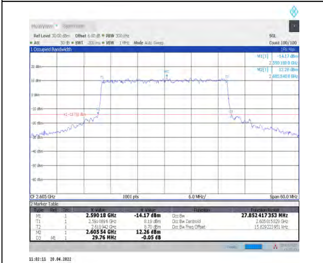
1-N38--30-30-H-8-CP-64QAM-Outer_Full-78@0-Ant1 1-27.852-29.760-≤30-PASS
