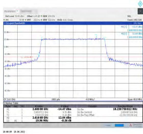
1-N38--30-20-H-6-CP-QPSK-Outer_Full-51@0-Ant1- 18.231-19.960-≤20-PASS
