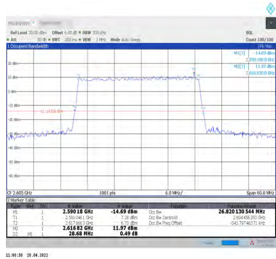
1-N38--30-30-H-5-DFT-256QAM-Outer_Full-75@0-A nt1-26.82-28.680-<=30-PASS
