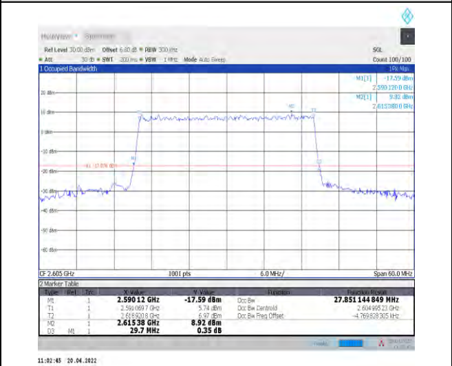
1-N38--30-30-H-9-CP-256QAM-Outer_Full-78@0-Ant1 1-27.851-29.700-≤30-PASS
