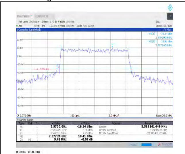
1-N38--30-10-L-6-CP-QPSK-Outer_Full-24@0-Ant1- 8.565-9.480-<=10-PASS
