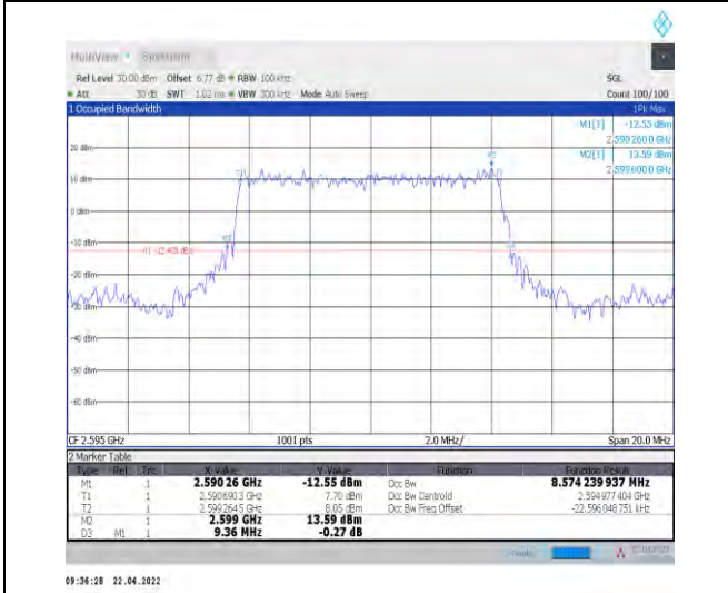
1-N38--30-10-M-2-DFT-PI2BPSK-Outer_Full-24@0-Ant Ant1-8.574-9.360-≤10-PASS
