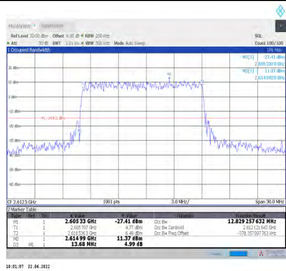
1-N38--30-15-H-5-DFT-256QAM-Outer_Full-36@0-Ant nt1-12.829-13.680-≤15-PASS
