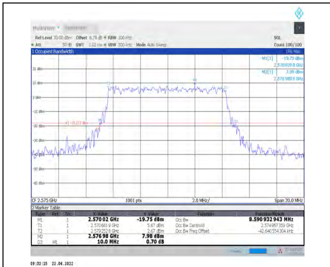
1-N38--30-10-L-5-DFT-256QAM-Outer_Full-24@0-A nt1-8.591-10.000-<=10-PASS
