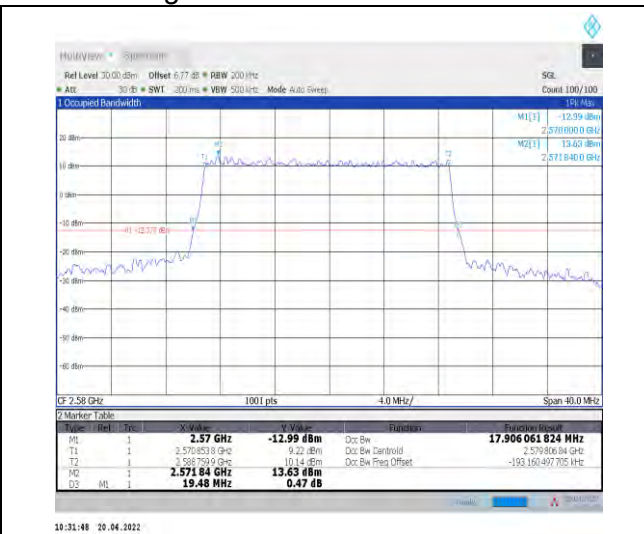
1-N38--30-20-L-4-DFT-64QAM-Outer_Full-50@0-An t1-17.906-19.480-≤20-PASS
