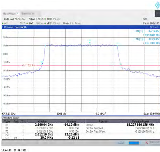
1-N38--30-20-H-7-CP-16QAM-Outer_Full-51@0-Ant 1-18.228-20.000-≤20-PASS
