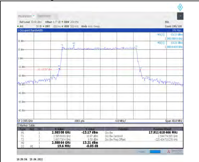
1-N38--30-20-M-3-DFT-16QAM-Outer_Full-50@0-Ant1-17.912-19.600-<=20-PASS
