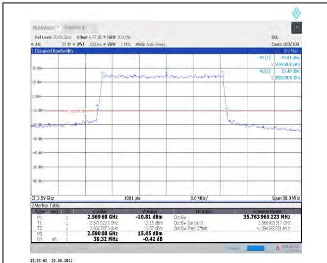
1-N38--30-40-L-1-DFT-QPSK-Outer_Full-100@0-Ant 1-35.764-38.320-≤40-PASS
