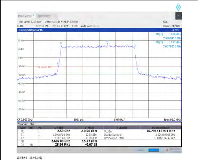
1-N38--30-30-H-1-DFT-QPSK-Outer_Full-75@0-Ant 1-26.796-28.860-≤30-PASS
