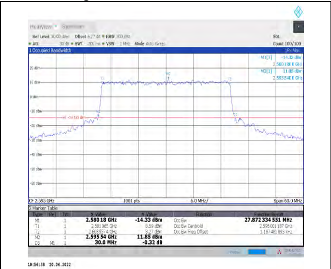
1-N38--30-30-M-8-CP-64QAM-Outer_Full-78@0-Ant 1-27.872-30.000-≤30-PASS
