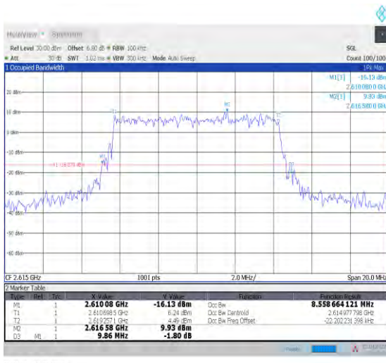
1-N38--30-10-H-5-DFT-256QAM-Outer_Full-24@0-A nt1-8.559-9.860-≤10-PASS
