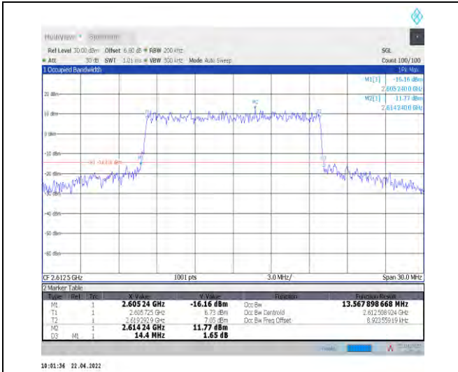
1-N38--30-15-H-8-CP-64QAM-Outer_Full-38@0-Ant 1-13.568-14.400-≤15-PASS
