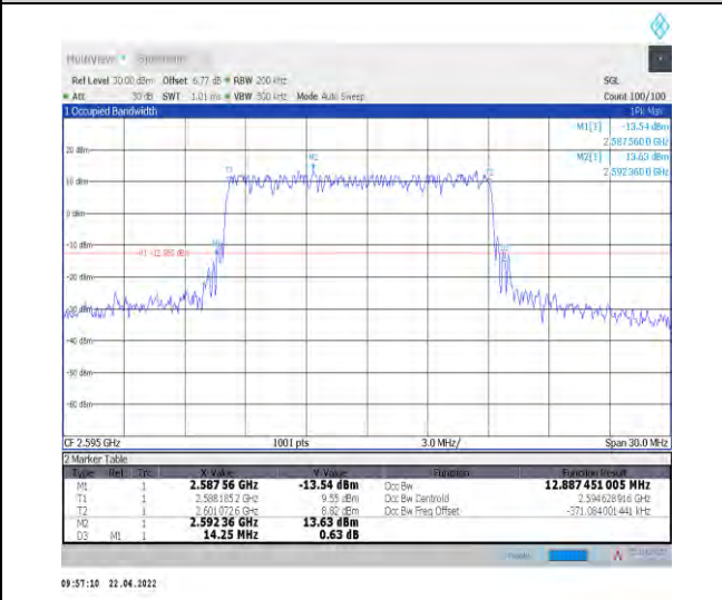
1-N38--30-15-M-4-DFT-64QAM-Outer_Full-36@0-Ant 1-12.887-14.250-≤15-PASS
