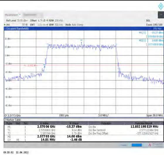
1-N38--30-15-L-3-DFT-16QAM-Outer_Full-36@0-An t1-12.852-14.010-≤15-PASS
