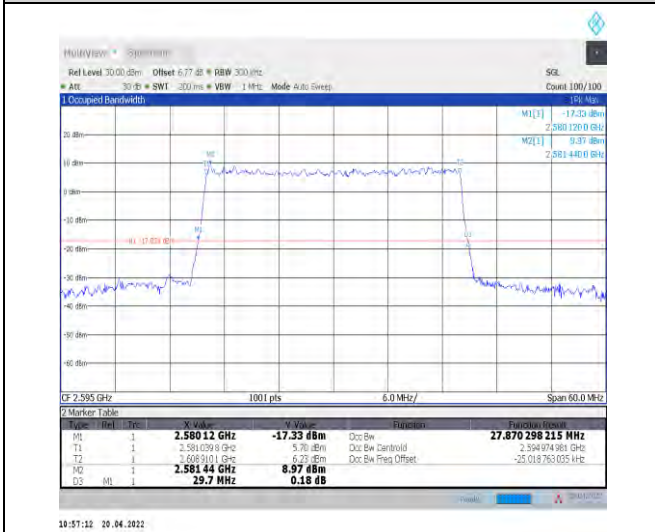
1-N38--30-30-M-9-CP-256QAM-Outer_Full-78@0-Ant t1-27.87-29.700-≤30-PASS
