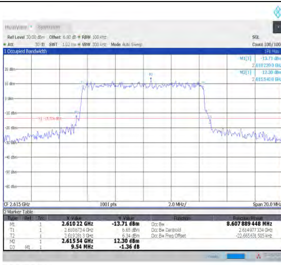
1-N38--30-10-H-3-DFT-16QAM-Outer_Full-24@0-An t1-8.608-9.540-≤10-PASS
