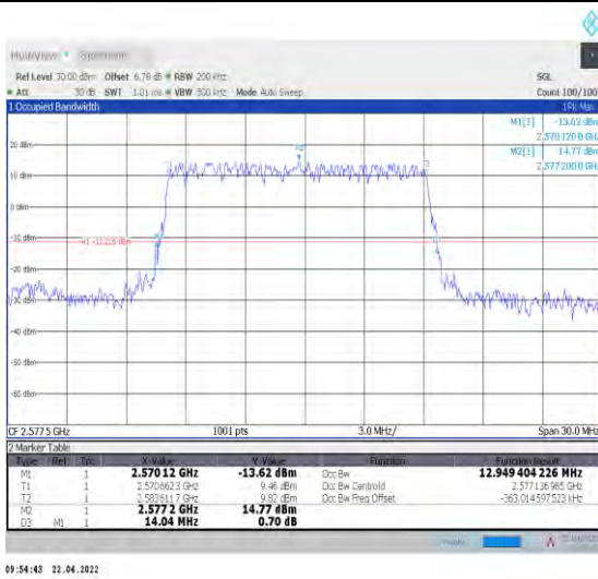
1-N38--30-15-L-2-DFT-PI2BPSK-Outer_Full-36@0-A nt1-12.949-14.040-≤15-PASS
