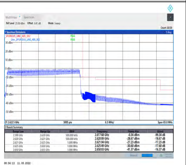
1-N38-PC2-30-30-H-6-CP-QPSK-Outer_Full-78@0-Ant1-PASS-see graph
