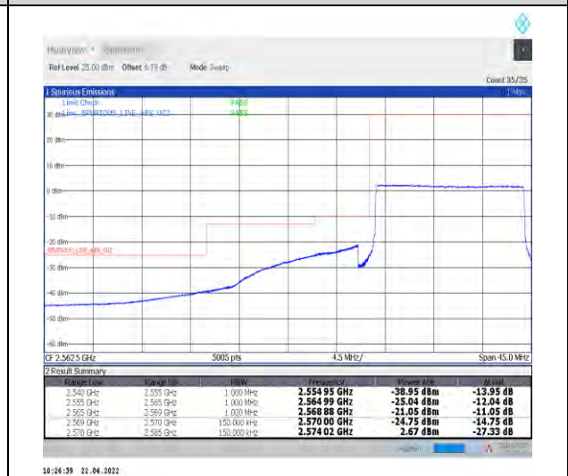
1-N38--30-15-L-6-CP-QPSK-Outer_Full-38@0-Ant 1-PASS-see graph
