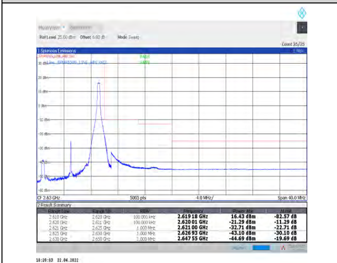
1-N38--30-10-H-5-CP-QPSK-Edge_1RB_Right-1@23- Ant1-PASS-see graph
