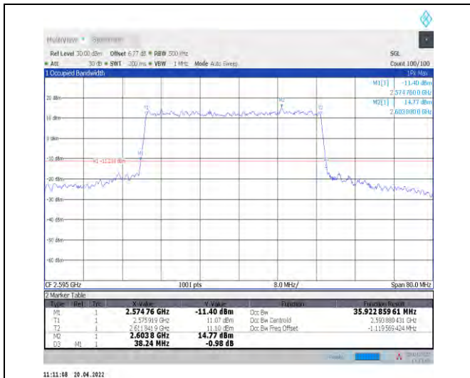
1-N38--30-40-M-4-DFT-64QAM-Outer_Full-100@0-A nt1-35.923-38.240-≤40-PASS
