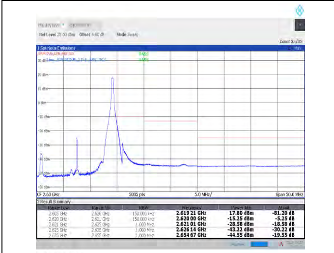
1-N38--30-15-H-2-DFT-PI2BPSK-Edge_1RB_Right-1@37-Ant1-PASS-see graph
