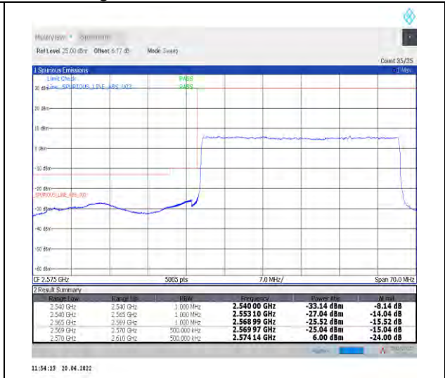
1-N38--30-40-L-3-DFT-PI2BPSK-Outer_Full-100@0-Ant1-PASS-see graph
