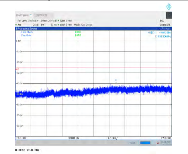
1-N38--30-40-H-1-DFT-PI2BPSK-Inner_1RB_Left-1 @1-12000-27000-Ant1--40.00--25-PASS
