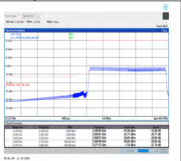
1-N38-PC2-30-30-L-6-CP-QPSK-Outer_Full-78@0-Ant1-PASS-see graph
