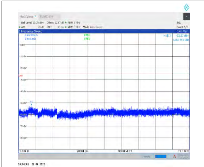
1-N38--30-40-L-1-DFT-PI2BPSK-Inner_1RB_Left-1 @1-3000-12000-Ant1--52.27--25-PASS
