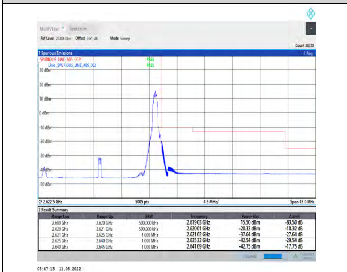
1-N38-PC2-30-20-H-5-CP-QPSK-Edge_1RB_Right-1@50-Ant1-PASS-see graph
