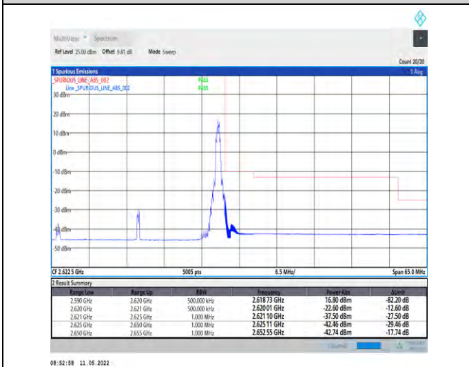
1-N38-PC2-30-30-H-5-CP-QPSK-Edge_1RB_Right-1@77-Ant1-PASS-see graph
