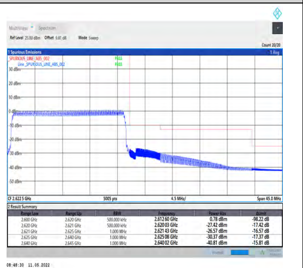
1-N38-PC2-30-20-H-6-CP-QPSK-Outer_Full-51@0-Ant1-PASS-see graph
