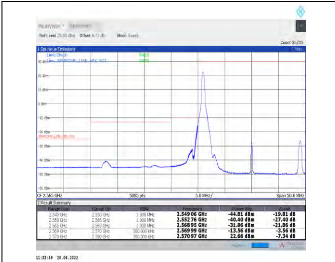
1-N38--30-20-L-1-DFT-PI2BPSK-Edge_1RB_Left-1@0-Ant1-PASS-see graph
