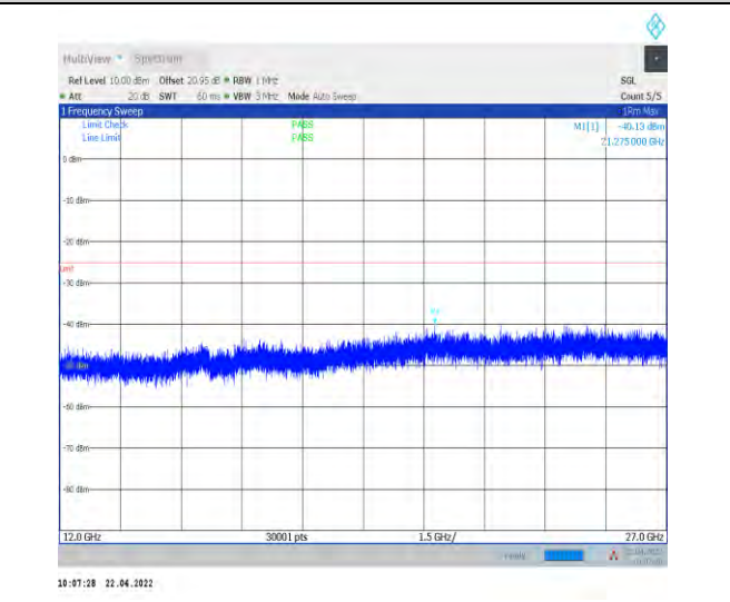
1-N38--30-40-M-1-DFT-PI2BPSK-Inner_1RB_Left-1 @1-12000-27000-Ant1--40.13--25-PASS
