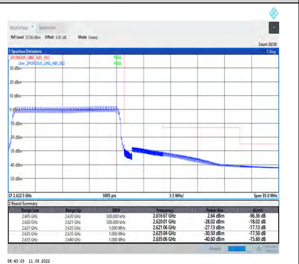
1-N38-PC2-30-15-H-6-CP-QPSK-Outer_Full-38@0-Ant1-PASS-see graph
