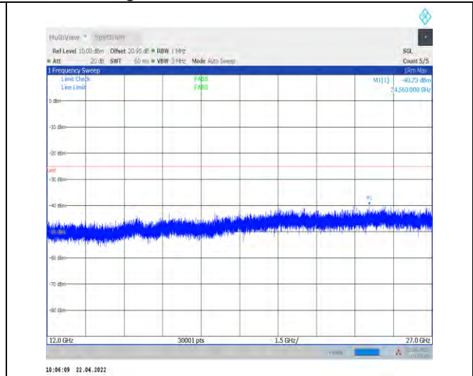
1-N38--30-40-L-1-DFT-PI2BPSK-Inner_1RB_Left-1@ 1-12000-27000-Ant1--40.23--25-PASS
