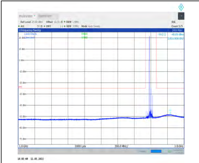
1-N38-PC2-30-40-H-1-DFT-QPSK-Edge_1RB_Left-1 @0-1000-3000-Ant1--48.09--25-PASS
