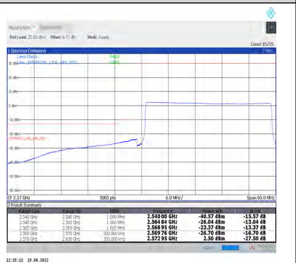
1-N38--30-30-L-6-CP-QPSK-Outer_Full-78@0-Ant 1-PASS-see graph
