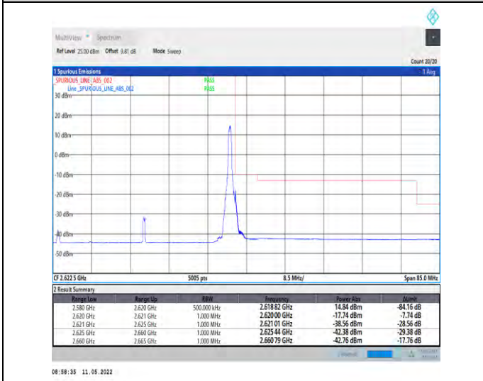
1-N38-PC2-30-40-H-5-CP-QPSK-Edge_1RB_Right-1@ 105-Ant1-PASS-see graph
