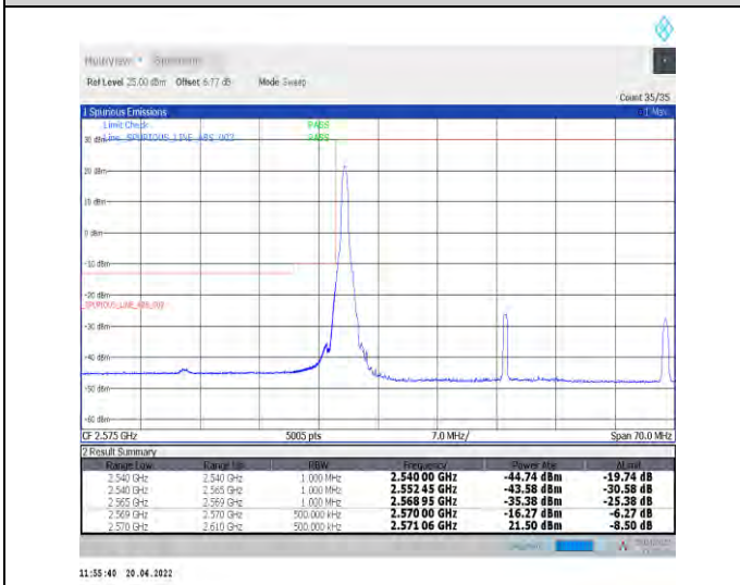
1-N38--30-40-L-4-CP-QPSK-Edge_1RB_Left-1@0-Ant1-PASS-see graph
