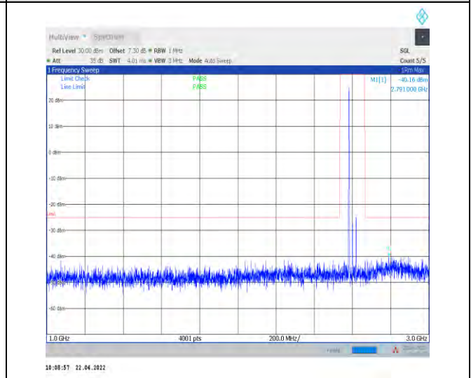
1-N38--30-40-H-1-DFT-PI2BPSK-Inner_1RB_Left-1 @1-1000-3000-Ant1--40.16--25-PASS
