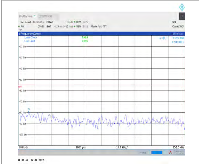
1-N38--30-40-M-1-DFT-PI2BPSK-Inner_1RB_Left-1 @1-0.009-0.15-Ant1--79.96--55-PASS
