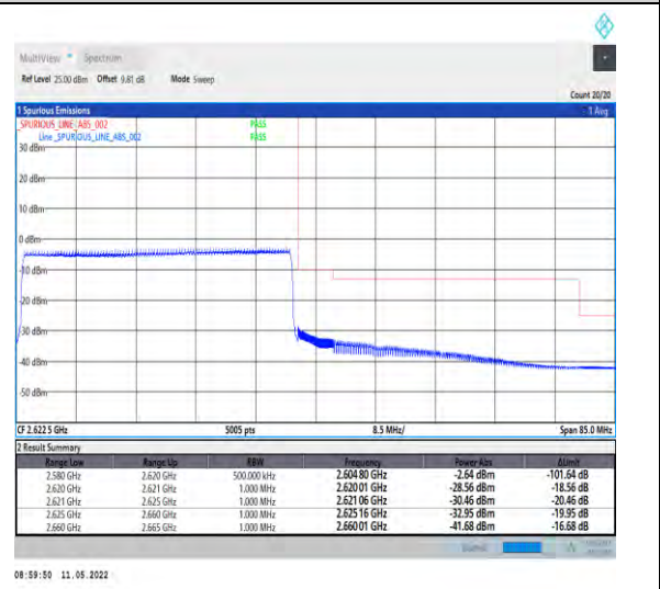
1-N38-PC2-30-40-H-6-CP-QPSK-Outer_Full-106 @0-Ant1-PASS-see graph
