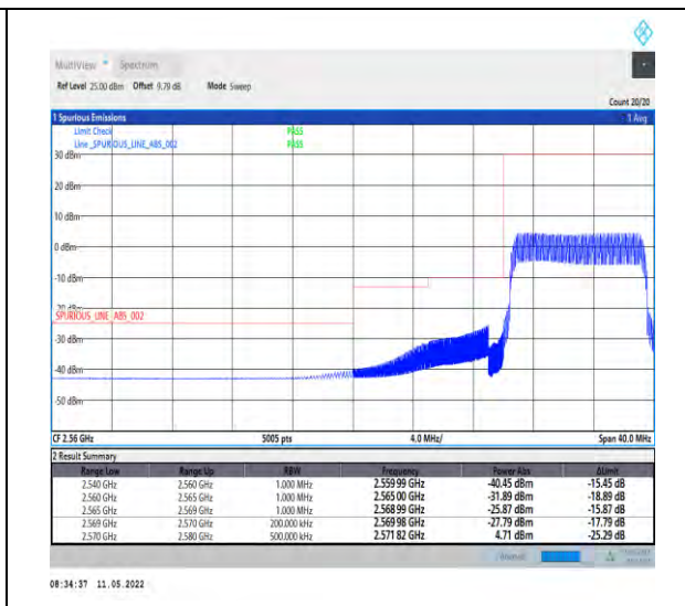
1-N38-PC2-30-10-L-6-CP-QPSK-Outer_Full-24@0 -Ant1-PASS-see graph
