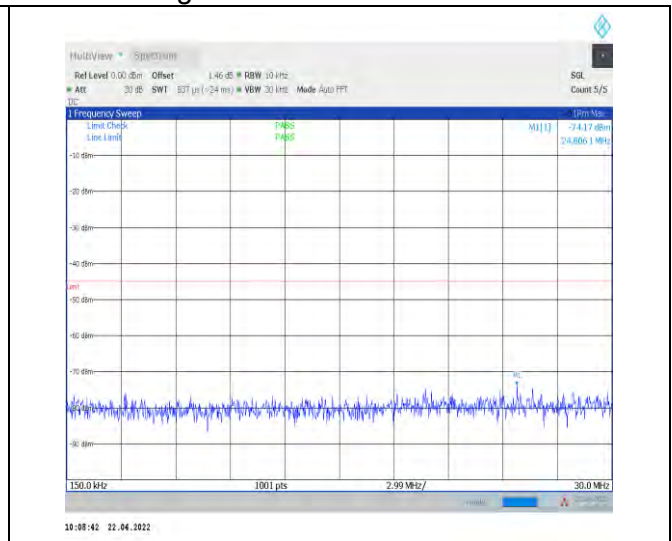
1-N38--30-40-H-1-DFT-PI2BPSK-Inner_1RB_Left-1 @1-0.15-30-Ant1--74.17--45-PASS
