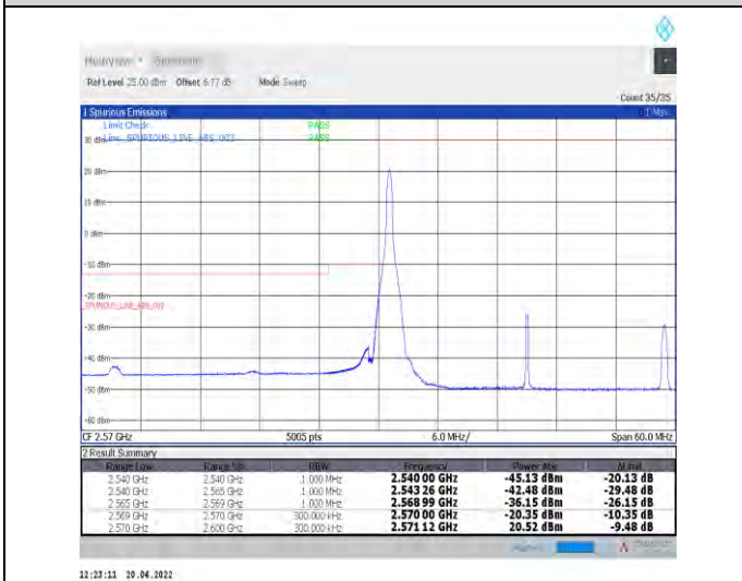
1-N38--30-30-L-4-CP-QPSK-Edge_1RB_Left-1@0-Ant 1-PASS-see graph
