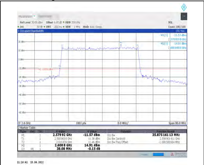
1-N38--30-40-H-4-DFT-64QAM-Outer_Full-100@0-A nt1-35.875-38.080-≤40-PASS
