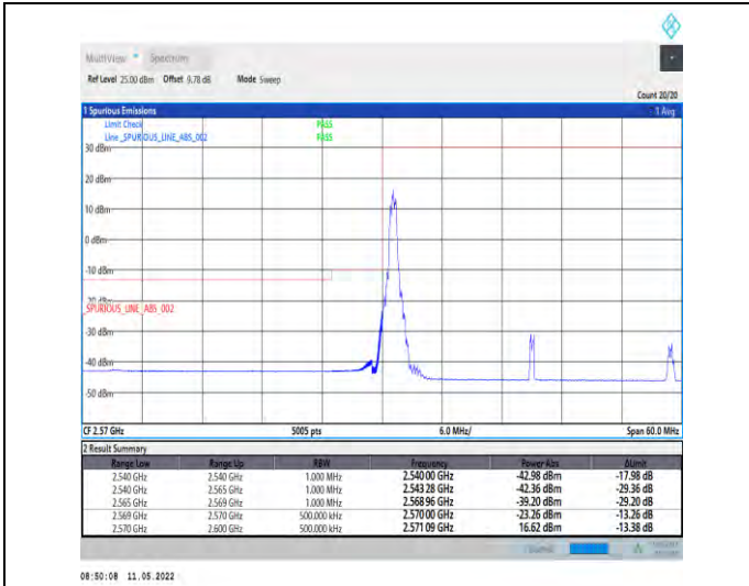
1-N38-PC2-30-30-L-4-CP-QPSK-Edge_1RB_Left-1@0 -Ant1-PASS-see graph
