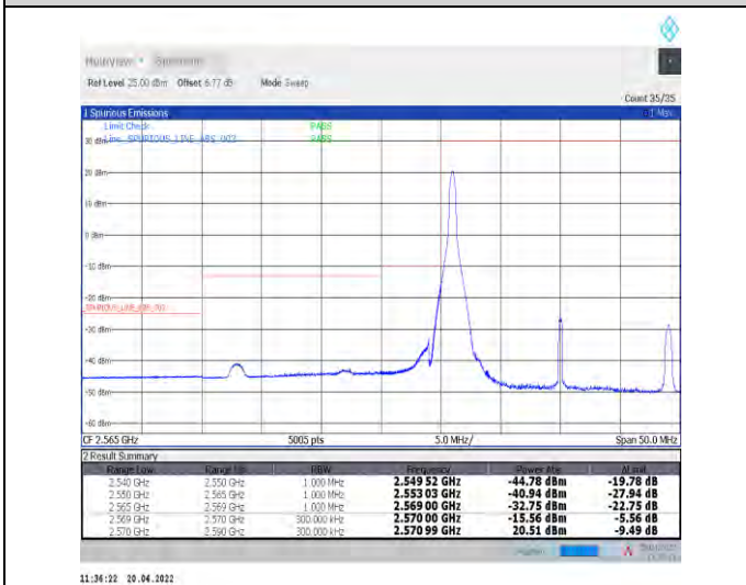
1-N38--30-20-L-4-CP-QPSK-Edge_1RB_Left-1@0-Ant 1-PASS-see graph
