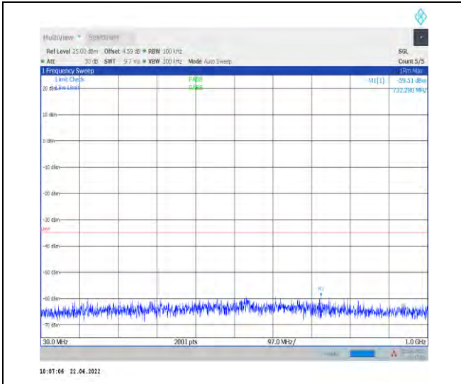
1-N38--30-40-M-1-DFT-PI2BPSK-Inner_1RB_Left-1 @1-30-1000-Ant1--59.51--35-PASS
