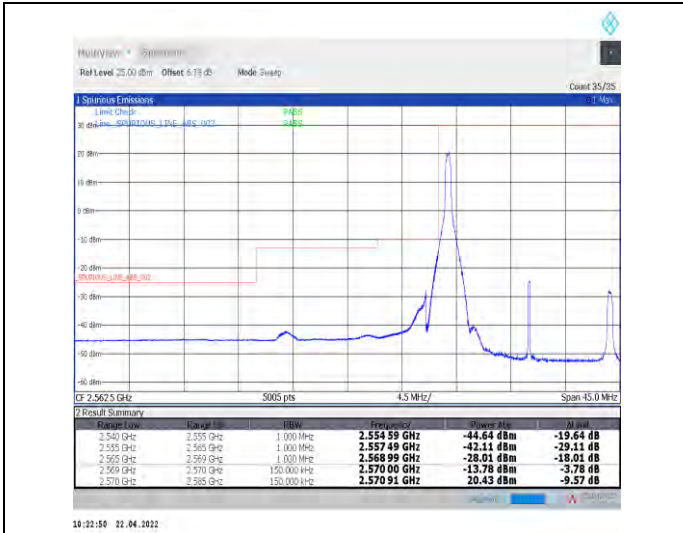
1-N38--30-15-L-1-DFT-PI2BPSK-Edge_1RB_Left-1@0-Ant1-PASS-see graph
