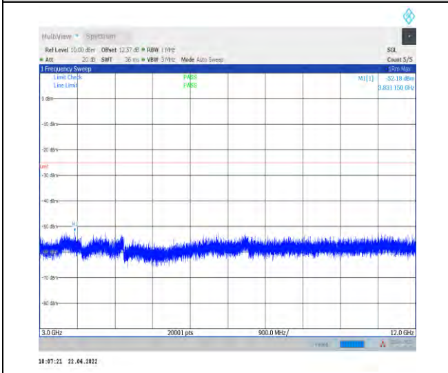
1-N38--30-40-M-1-DFT-PI2BPSK-Inner_1RB_Left-1 @1-3000-12000-Ant1--52.18--25-PASS
