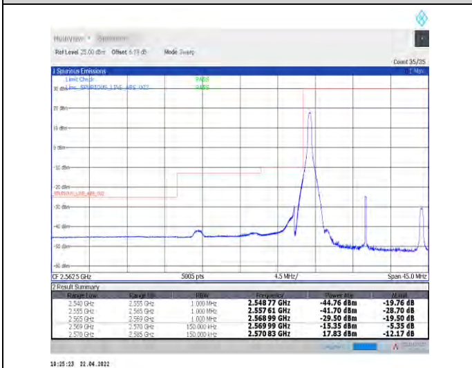
1-N38--30-15-L-4-CP-QPSK-Edge_1RB_Left-1@0-Ant 1-PASS-see graph
