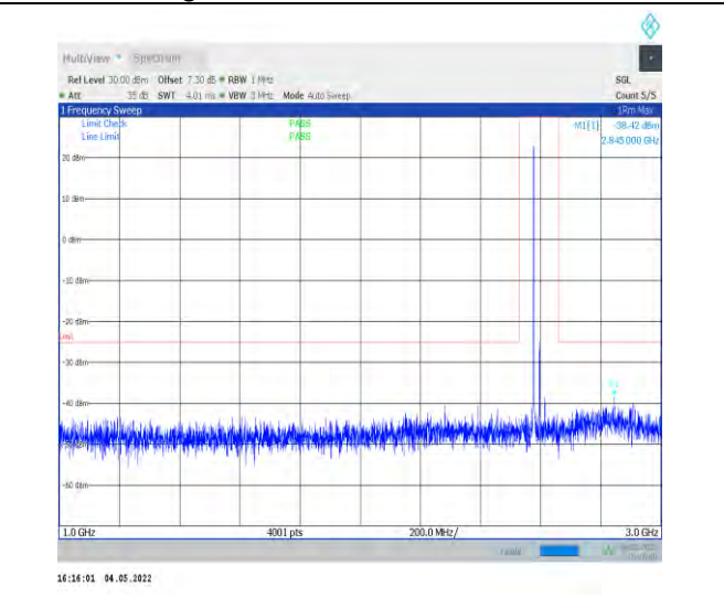
1-N38--30-40-M-1-DFT-PI2BPSK-Inner_1RB_Left-1 @1-1000-3000-Ant1--39.82--25-PASS
