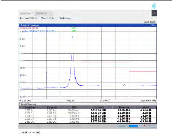
1-N38--30-40-H-2-DFT-PI2BPSK-Edge_1RB_Right-1@105-Ant1-PASS-see graph
