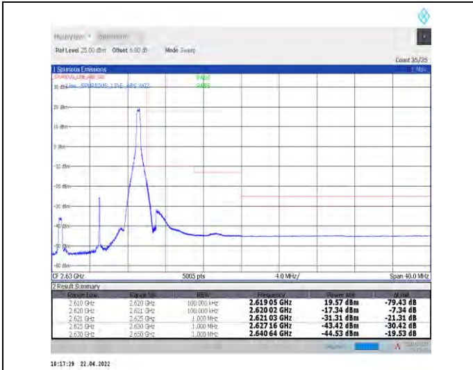
1-N38--30-10-H-2-DFT-PI2BPSK-Edge_1RB_Right-1@ 23-Ant1-PASS-see graph
