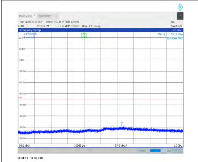
1-N38-PC2-30-40-M-1-DFT-QPSK-Edge_1RB_Left-1 @0-30-1000-Ant1--59.12--35-PASS
