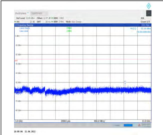
1-N38--30-40-H-1-DFT-PI2BPSK-Inner_1RB_Left-1 @1-3000-12000-Ant1--52.16--25-PASS
