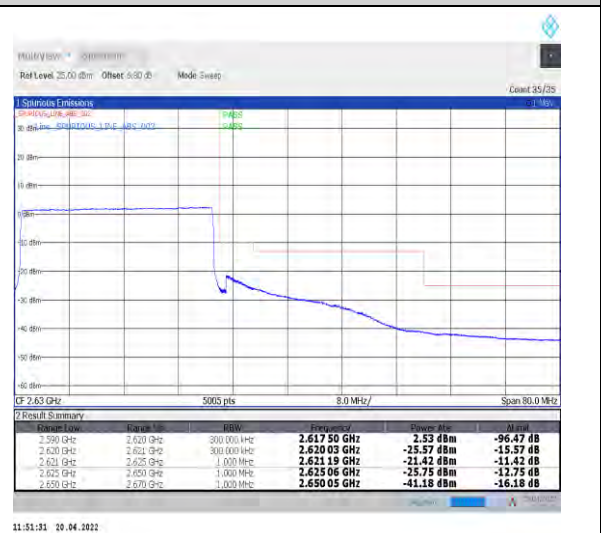
1-N38--30-30-H-6-CP-QPSK-Outer_Full-78@0-Ant1-PASS-see graph
