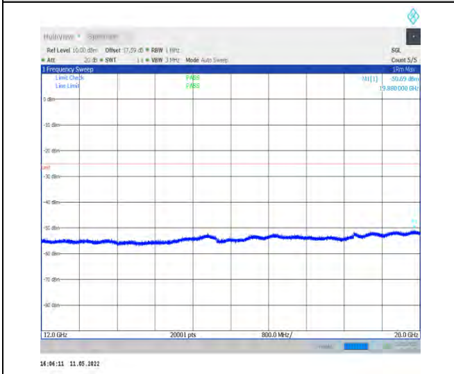
1-N38-PC2-30-40-H-1-DFT-QPSK-Edge_1RB_Left-1 @0-12000-20000-Ant1--50.69--25-PASS
