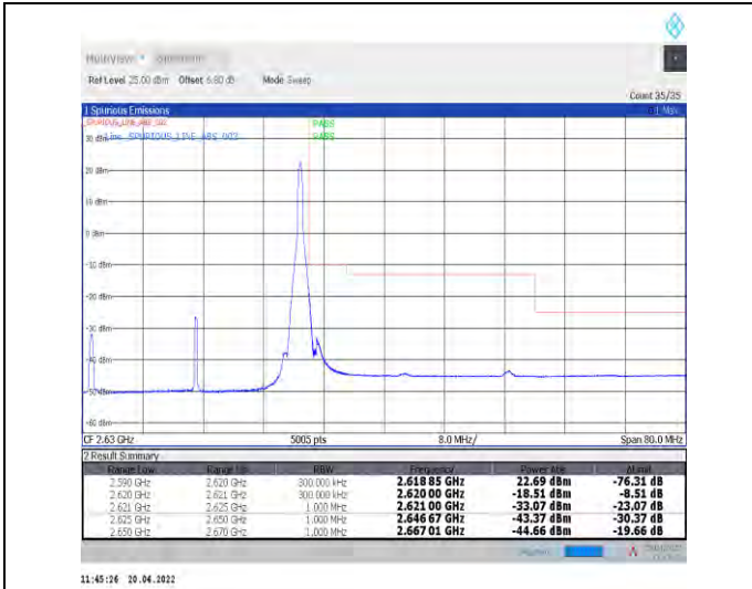
1-N38--30-30-H-2-DFT-PI2BPSK-Edge_1RB_Right-1@77-Ant1-PASS-see graph
