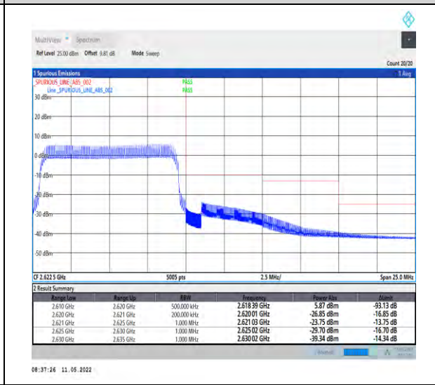
1-N38-PC2-30-10-H-6-CP-QPSK-Outer_Full-24@0 -Ant1-PASS-see graph
