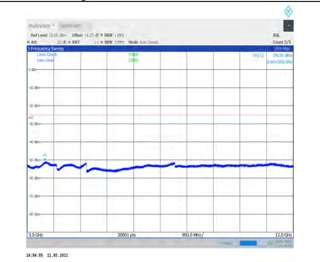
1-N38-PC2-30-40-H-1-DFT-QPSK-Edge_1RB_Left-1 @0-3000-12000-Ant1--50.50--25-PASS
