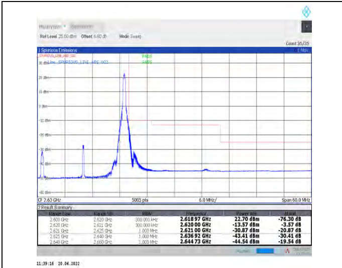
1-N38--30-20-H-2-DFT-PI2BPSK-Edge_1RB_Right-1@ 50-Ant1-PASS-see graph
