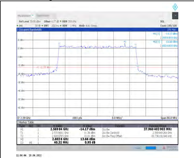
1-N38--30-40-L-6-CP-QPSK-Outer_Full-106@0-Ant 1-37.96-40.320-≤40-PASS
