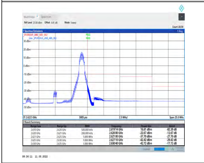
1-N38-PC2-30-10-H-5-CP-QPSK-Edge_1RB_Right-1@23 -Ant1-PASS-see graph
