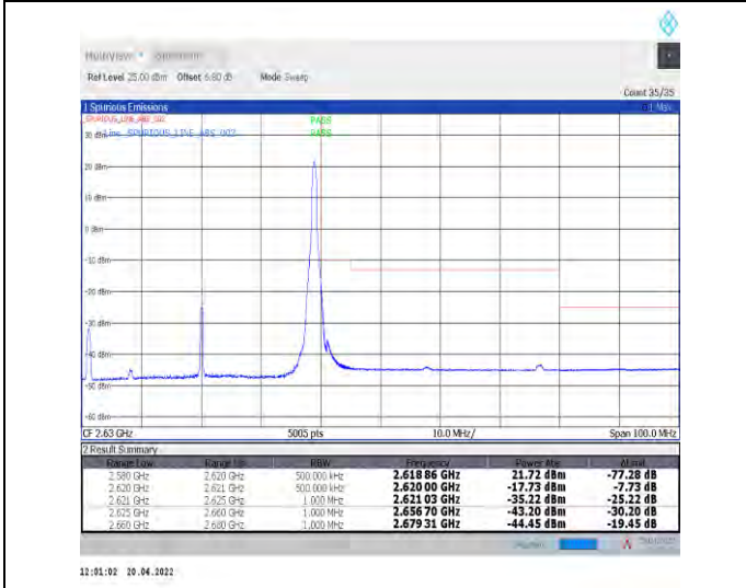
1-N38--30-40-H-5-CP-QPSK-Edge_1RB_Right-1@105-Ant1-PASS-see graph
