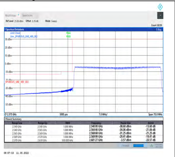
1-N38-PC2-30-40-L-6-CP-QPSK-Outer_Full-106 @0-Ant1-PASS-see graph
