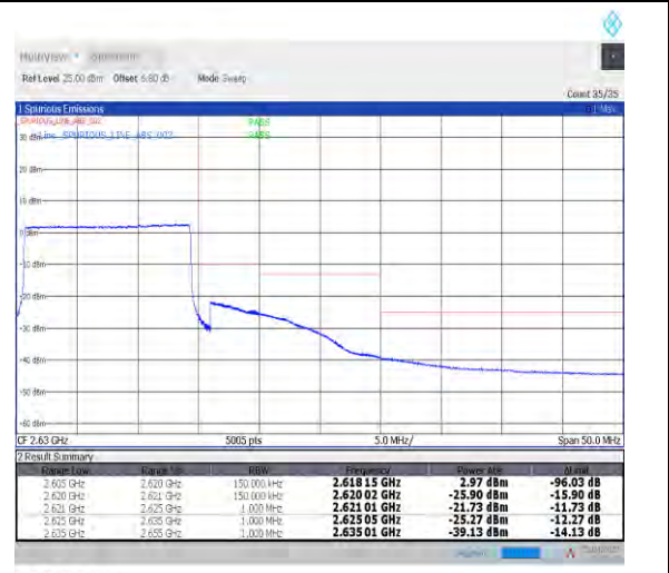
1-N38--30-15-H-3-DFT-PI2BPSK-Outer_Full-36@0-Ant1-PASS-see graph
