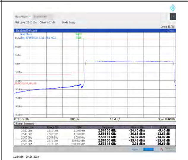
1-N38--30-40-L-6-CP-QPSK-Outer_Full-106@0-Ant1-PASS-see graph
