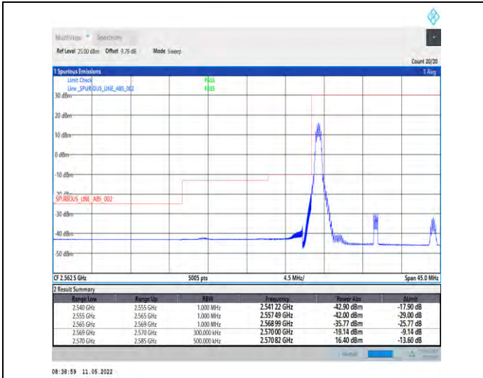
1-N38-PC2-30-15-L-4-CP-QPSK-Edge_1RB_Left-1@0 -Ant1-PASS-see graph
