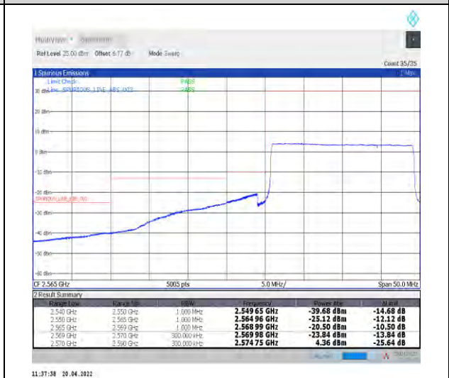
1-N38--30-20-L-6-CP-QPSK-Outer_Full-51@0-Ant 1-PASS-see graph
