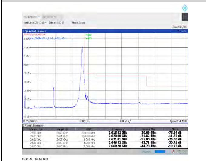
1-N38--30-30-H-5-CP-QPSK-Edge_1RB_Right-1@77-Ant1-PASS-see graph
