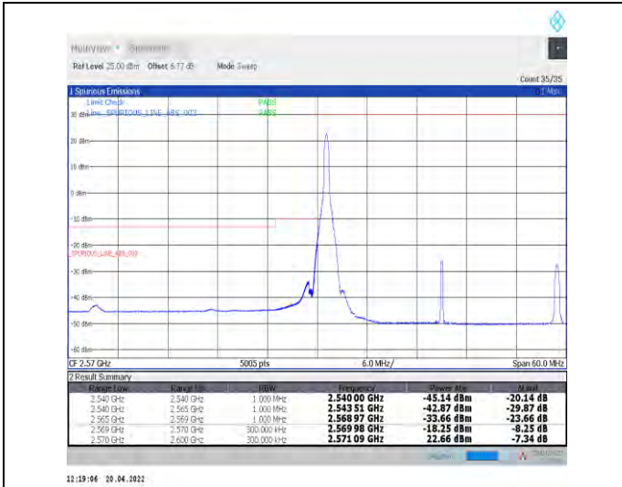
1-N38--30-30-L-1-DFT-PI2BPSK-Edge_1RB_Left-1@0-Ant1-PASS-see graph
