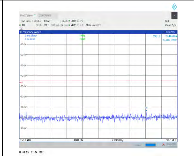
1-N38--30-40-M-1-DFT-PI2BPSK-Inner_1RB_Left-1 @1-0.15-30-Ant1--74.16--45-PASS
