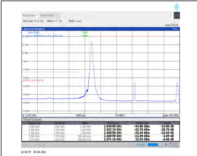
1-N38--30-40-L-1-DFT-PI2BPSK-Edge_1RB_Left-1@0-Ant1-PASS-see graph
