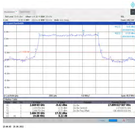
1-N41--30-20-H-2-DFT-PI2BPSK-Outer_Full-50@0-Ant 1-17.899-19.880-≤20-PASS
