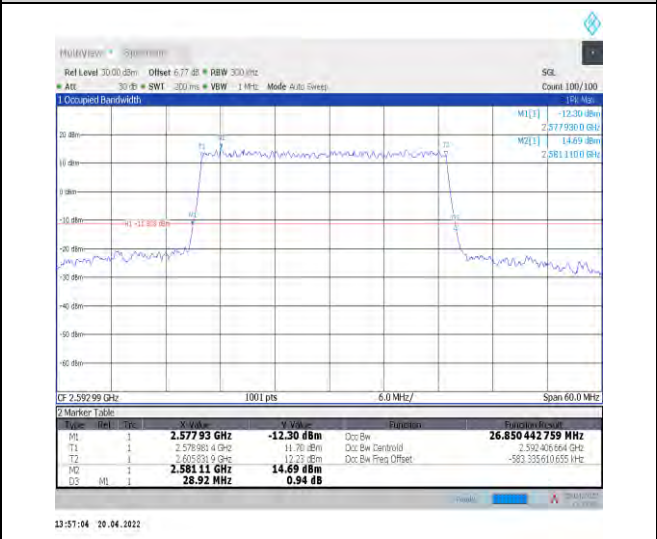
1-N41--30-30-M-4-DFT-64QAM-Outer_Full-75@0-Ant nt1-26.85-28.920-≤30-PASS
