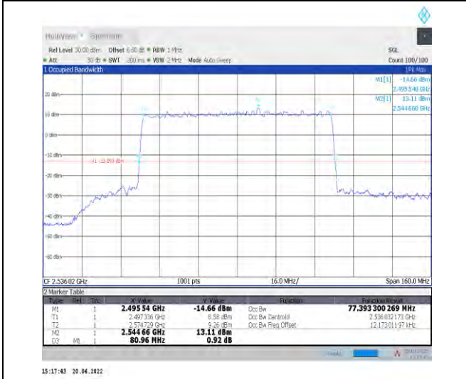
1-N41--30-80-L-9-CP-256QAM-Outer_Full-217@0-A nt1-77.393-80.960-≤80-PASS
