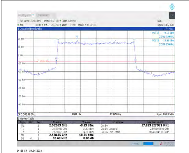
1-N41--30-60-M-2-DFT-PI2BPSK-Outer_Full-162@0 -Ant1-57.914-60.480-≤60-PASS
