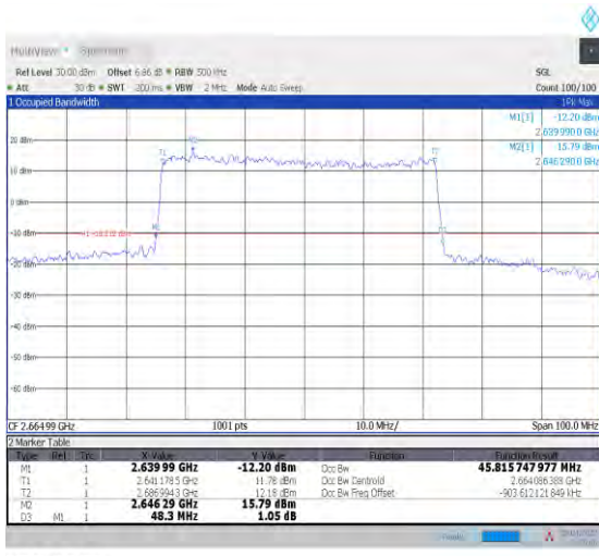
1-N41--30-50-H-4-DFT-64QAM-Outer_Full-128@0-Ant1-45.816-48.300-≤50-PASS
