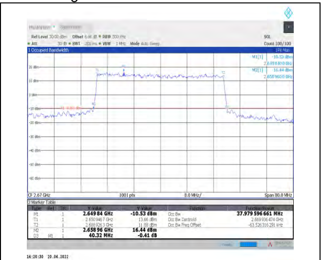
1-N41--30-40-H-6-CP-QPSK-Outer_Full-106@0-Ant 1-37.98-40.320-<=40-PASS
