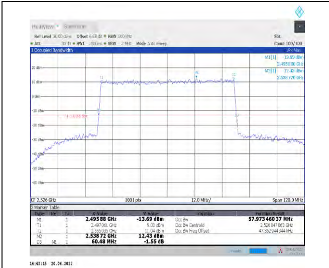
1-N41--30-60-L-5-DFT-256QAM-Outer_Full-162@0-Ant1-57.973-60.480-≤60-PASS
