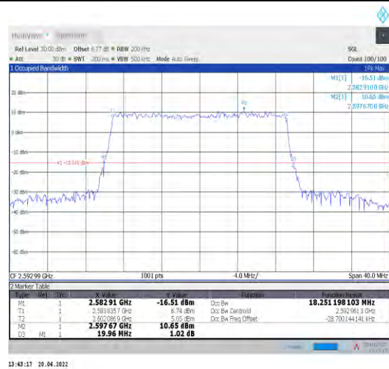
1-N41--30-20-M-9-CP-256QAM-Outer_Full-51@0-Ant 1-18.251-19.960-≤20-PASS
