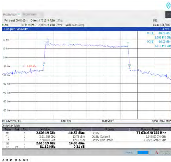
1-N41--30-80-H-7-CP-16QAM-Outer_Full-217@0-Ant t1-77.635-81.120-<math>\leq 80</math>-PASS
