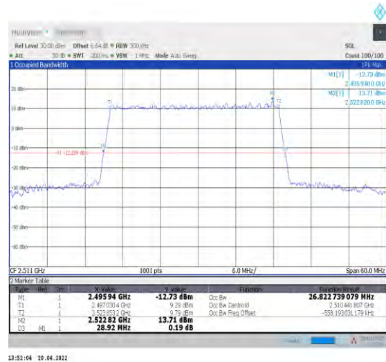
1-N41--30-30-L-5-DFT-256QAM-Outer_Full-75@0-A nt1-26.823-28.920-≤30-PASS
