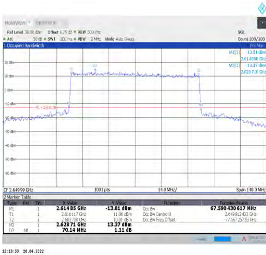
1-N41--30-70-H-6-CP-QPSK-Outer_Full-189@0-Ant 1-67.59-70.140-≤70-PASS
