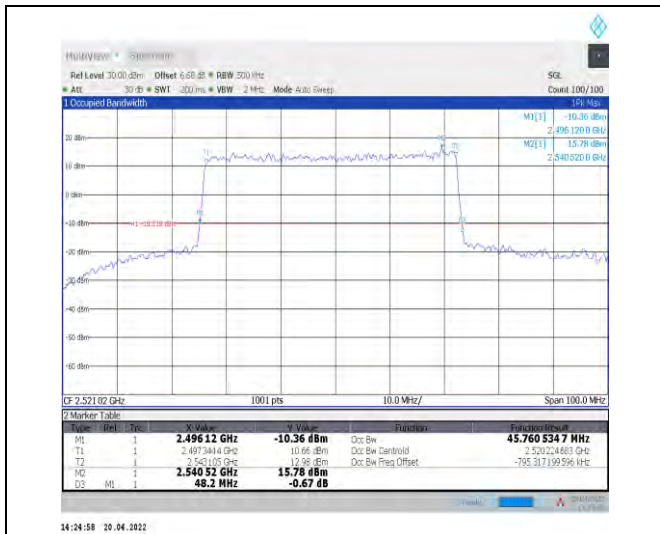
1-N41--30-50-L-4-DFT-64QAM-Outer_Full-128@0-A nt1-45.761-48.200-≤50-PASS
