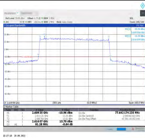
1-N41--30-80-H-6-CP-QPSK-Outer_Full-217@0-Ant 1-77.642-81.280-<math>\leq 80</math>-PASS
