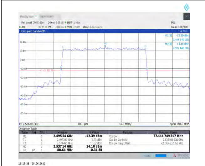
1-N41--30-80-L-5-DFT-256QAM-Outer_Full-216@0-A Ant1-77.112-80.640-<=80-PASS
