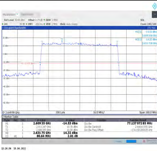
1-N41--30-80-H-5-DFT-256QAM-Outer_Full-216@0-Ant1-77.138-80.640-<math>\leq 80</math>-PASS
