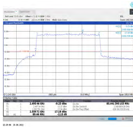
1-N41--30-90-L-1-DFT-QPSK-Outer_Full-240@0-Ant 1-85.441-89.460-≤90-PASS
