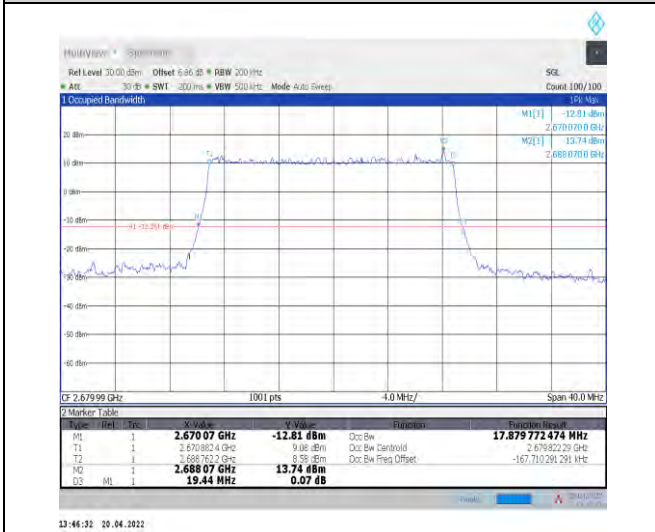
1-N41--30-20-H-5-DFT-256QAM-Outer_Full-50@0-A nt1-17.88-19.440-<=20-PASS
