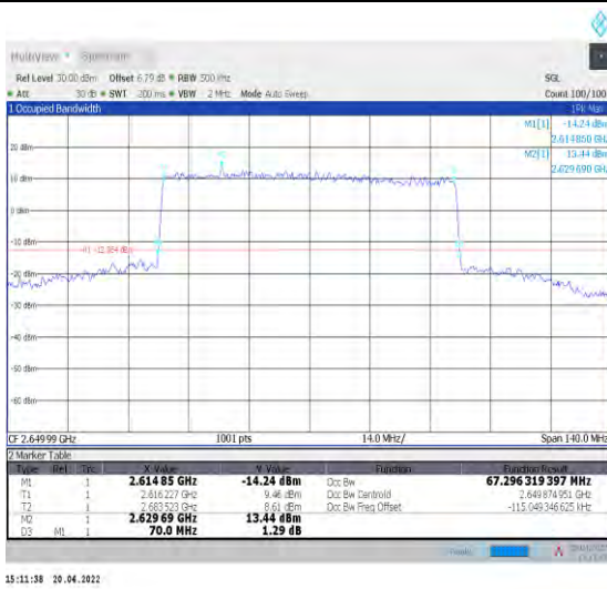
1-N41--30-70-H-8-CP-64QAM-Outer_Full-189@0-Ant t1-67.296-70.000-≤70-PASS
