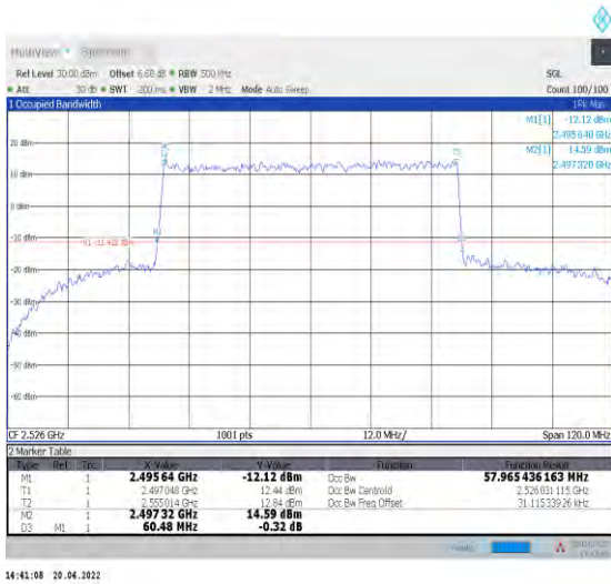
1-N41--30-60-L-3-DFT-16QAM-Outer_Full-162@0-Ant 1-57.965-60.480-≤60-PASS
