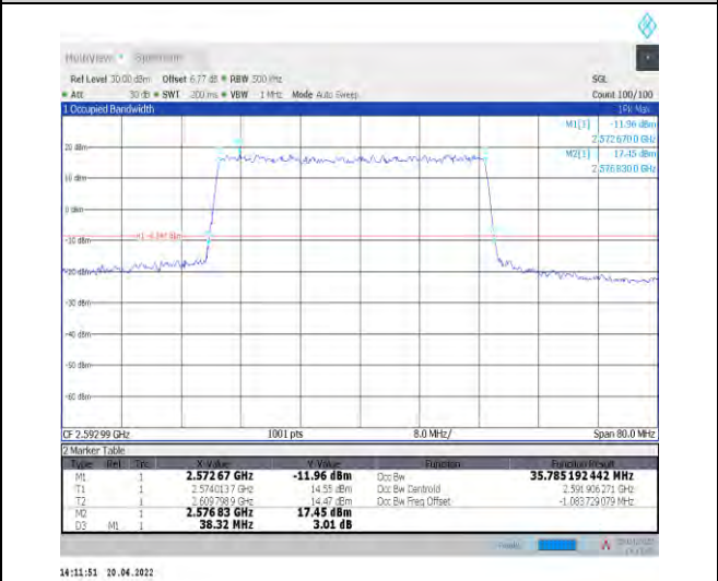
1-N41--30-40-M-1-DFT-QPSK-Outer_Full-100@0-An t1-35.785-38.320-≤40-PASS
