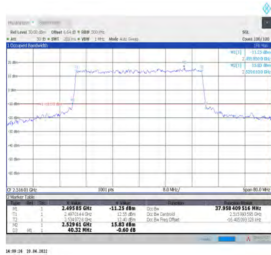
1-N41--30-40-L-6-CP-QPSK-Outer_Full-106@0-Ant 1-37.958-40.320-<40-PASS
