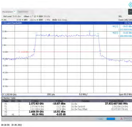
1-N41--30-40-M-6-CP-QPSK-Outer_Full-106@0-Ant 1-37.933-40.240-<40-PASS
