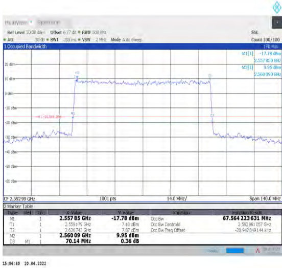
1-N41--30-70-M-9-CP-256QAM-Outer_Full-189@0-A nt1-67.564-70.140-<=70-PASS
