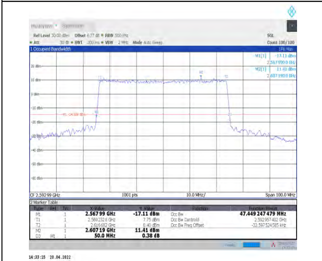
1-N41--30-50-M-9-CP-256QAM-Outer_Full-133@0-A nt1-47.449-50.000-<=50-PASS
