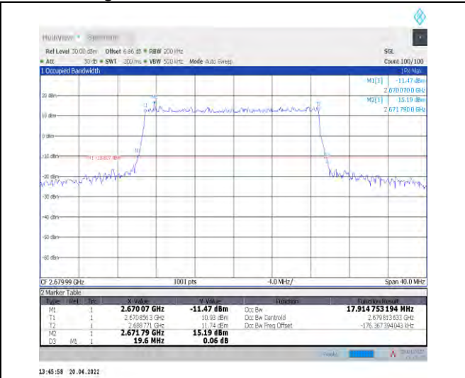
1-N41--30-20-H-4-DFT-64QAM-Outer_Full-50@0-An t1-17.915-19.600-<=20-PASS
