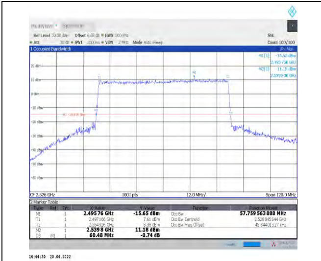
1-N41--30-60-L-9-CP-256QAM-Outer_Full-162@0-A nt1-57.76-60.480-≤60-PASS
