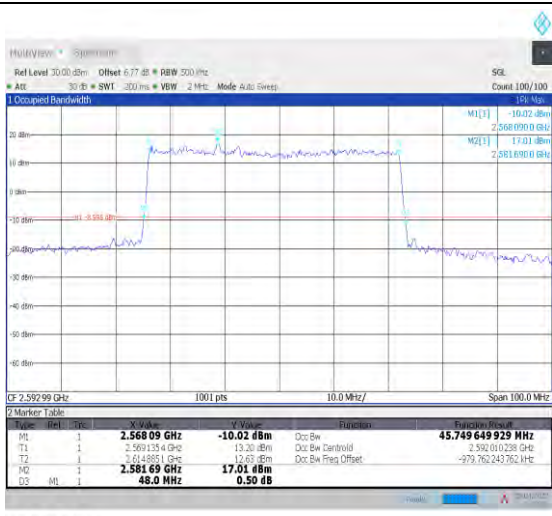
1-N41--30-50-M-3-DFT-16QAM-Outer_Full-128@0-A Ant1-45.75-48.000-≤50-PASS
