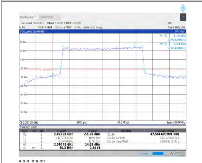
1-N41--30-50-L-6-CP-QPSK-Outer_Full-133@0-Ant1 -47.505-50.200-≤50-PASS
