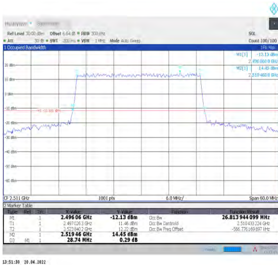
1-N41--30-30-L-4-DFT-64QAM-Outer_Full-75@0-Ant 1-26.814-28.740-≤30-PASS
