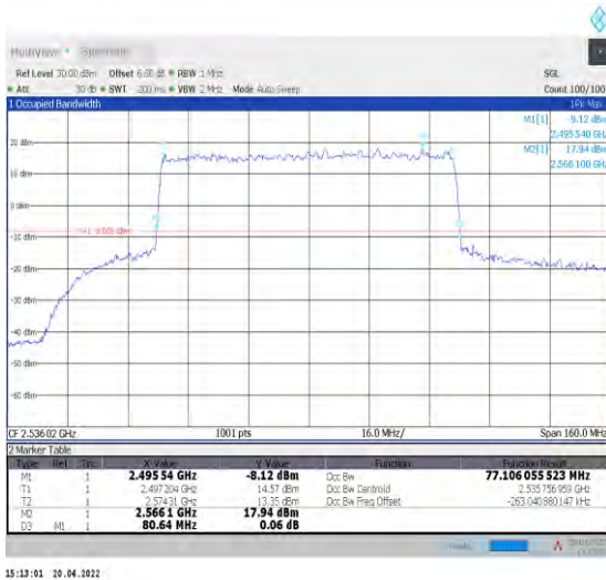
1-N41--30-80-L-1-DFT-QPSK-Outer_Full-216@0-Ant 1-77.106-80.640-≤80-PASS
