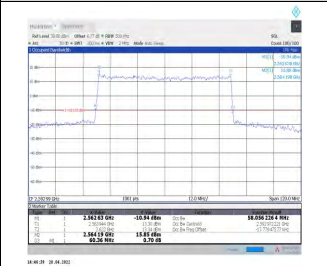
1-N41--30-60-M-3-DFT-16QAM-Outer_Full-162@0-0 Ant1-58.056-60.360-≤60-PASS
