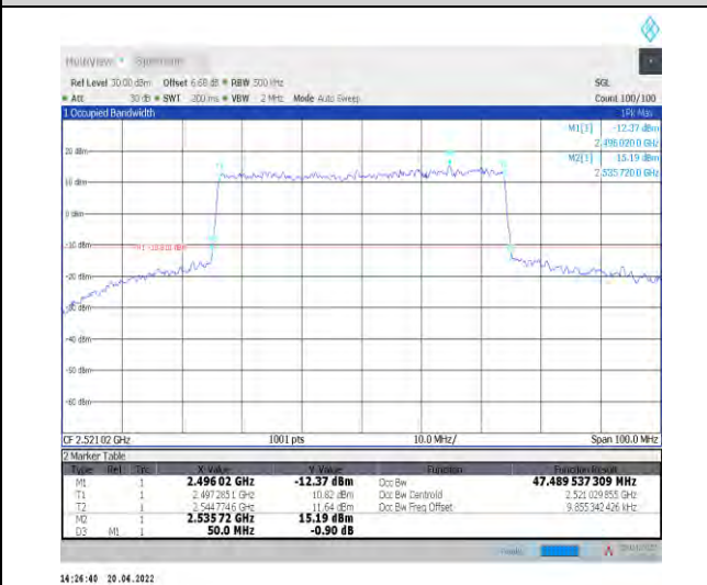
1-N41--30-50-L-7-CP-16QAM-Outer_Full-133@0-Ant1 t1-47.49-50.000-≤50-PASS
