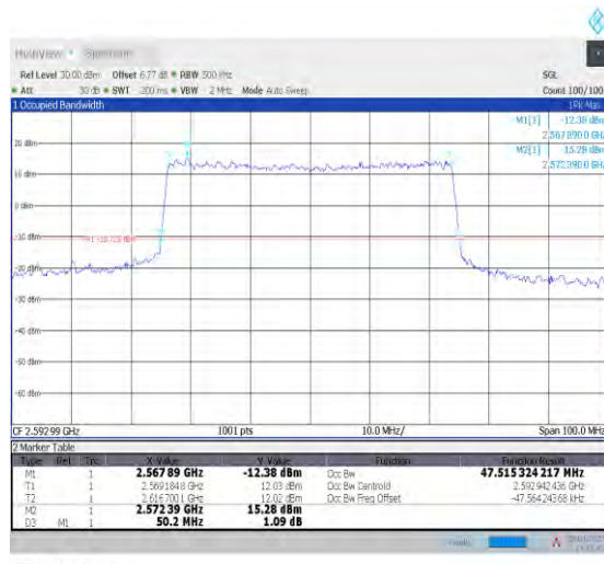
1-N41--30-50-M-6-CP-QPSK-Outer_Full-133@0-Ant1-47.515-50.200-≤50-PASS
