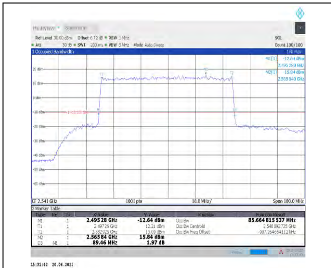
1-N41--30-90-L-4-DFT-64QAM-Outer_Full-240@0-A nt1-85.665-89.460-≤90-PASS
