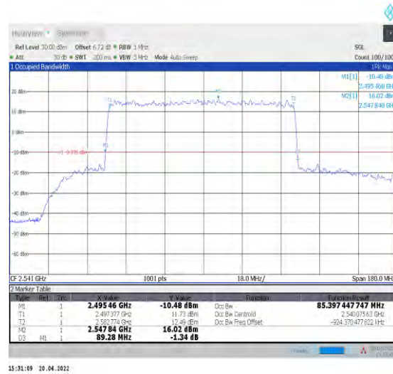
1-N41--30-90-L-3-DFT-16QAM-Outer_Full-240@0-A nt1-85.397-89.280-≤90-PASS
