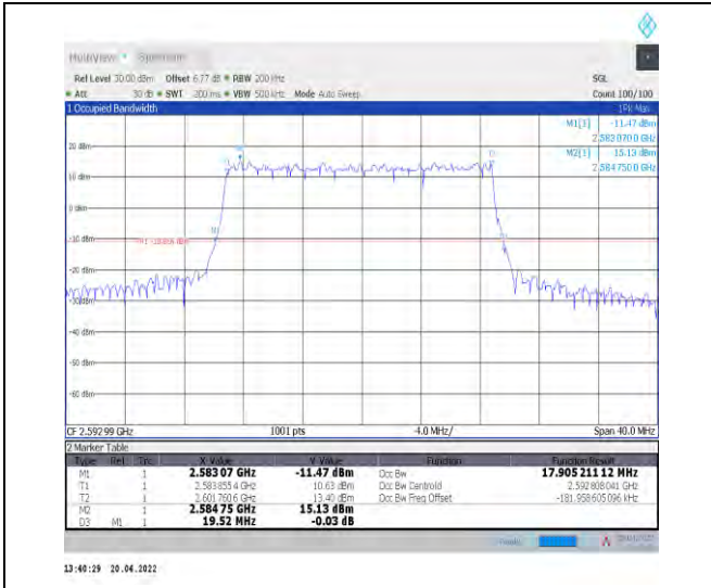
1-N41--30-20-M-4-DFT-64QAM-Outer_Full-50@0-Ant t1-17.905-19.520-<=20-PASS
