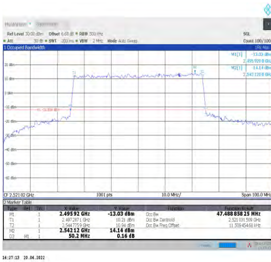
1-N41--30-50-L-8-CP-64QAM-Outer_Full-133@0-Ant 1-47.489-50.200-≤50-PASS
