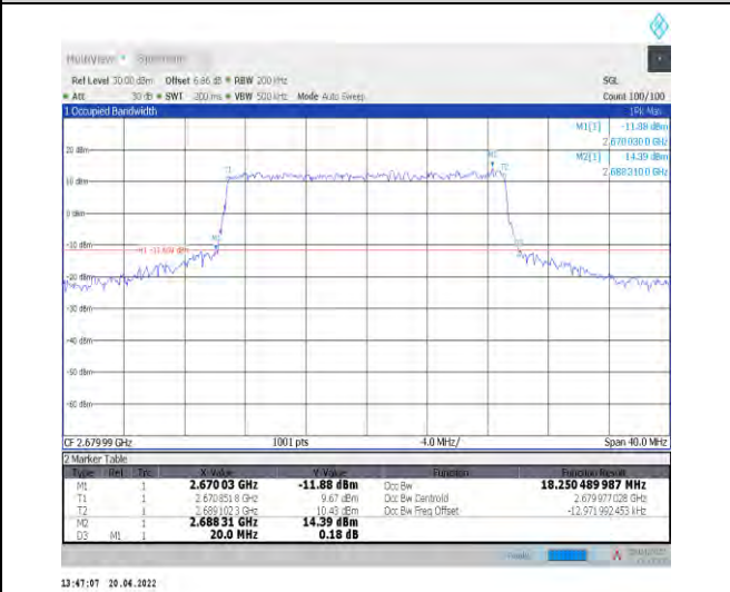
1-N41--30-20-H-6-CP-QPSK-Outer_Full-51@0-Ant1- 18.25-20.000-<=20-PASS
