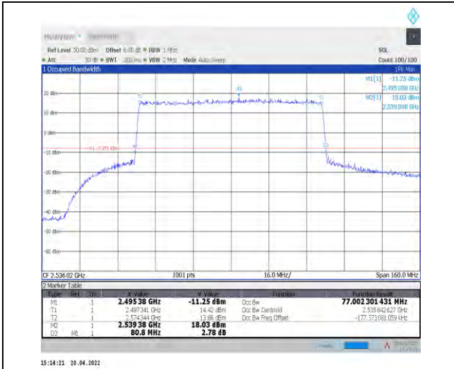
1-N41--30-80-L-3-DFT-16QAM-Outer_Full-216@0-A nt1-77.002-80.800-<=80-PASS
