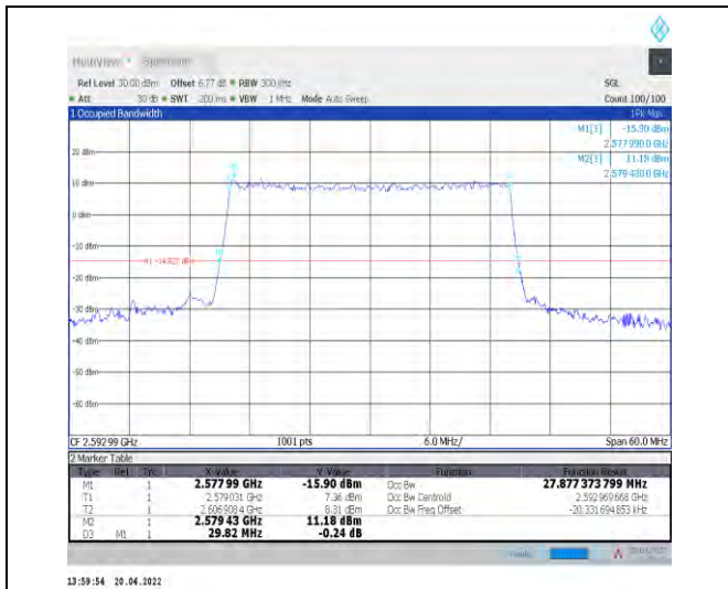
1-N41--30-30-M-9-CP-256QAM-Outer_Full-78@0-An t1-27.877-29.820-<30-PASS
