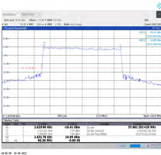
1-N41--30-60-H-9-CP-256QAM-Outer_Full-162@0-A nt1-57.861-60.360-≤60-PASS
