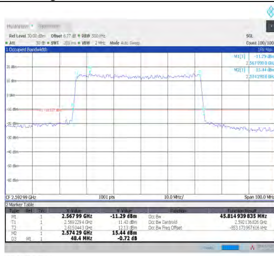
1-N41--30-50-M-4-DFT-64QAM-Outer_Full-128@0-Ant1-45.815-48.400-≤50-PASS
