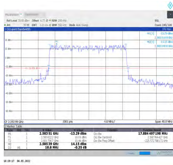
1-N41--30-20-M-3-DFT-16QAM-Outer_Full-50@0-Ant1-17.884-18.800-≤20-PASS
