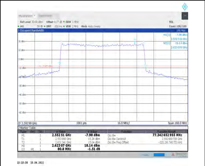
1-N41--30-80-M-1-DFT-QPSK-Outer_Full-216@0-An t1-77.343-80.800-≤80-PASS
