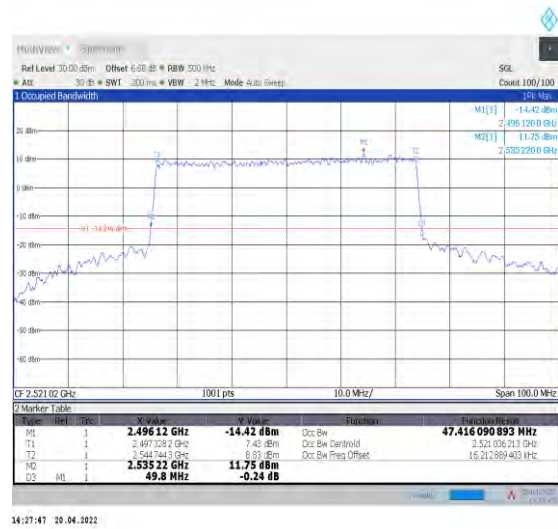
1-N41--30-50-L-9-CP-256QAM-Outer_Full-133@0-Ant 1-47.416-49.800-≤50-PASS
