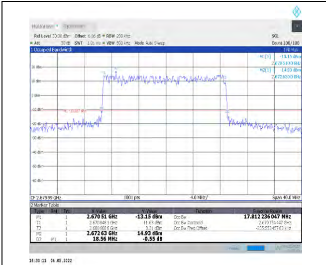
1-N41--30-20-H-3-DFT-16QAM-Outer_Full-50@0-An t1-17.812-18.560-<=20-PASS
