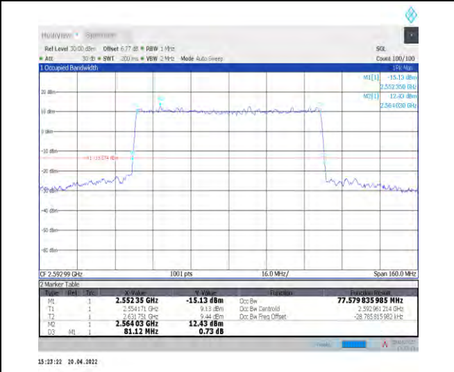
1-N41--30-80-M-9-CP-256QAM-Outer_Full-217@0-Ant 1-77.58-81.120-<80-PASS
