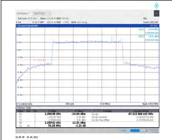
1-N41--30-70-L-8-CP-64QAM-Outer_Full-189@0-Ant1 1-67.323-70.280-≤70-PASS
