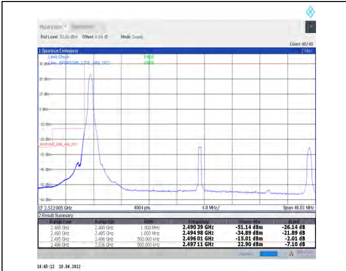
1-N41--30-40-L-1-DFT-PI2BPSK-Edge_1RB_Left-1@0-Ant1-PASS-see graph
