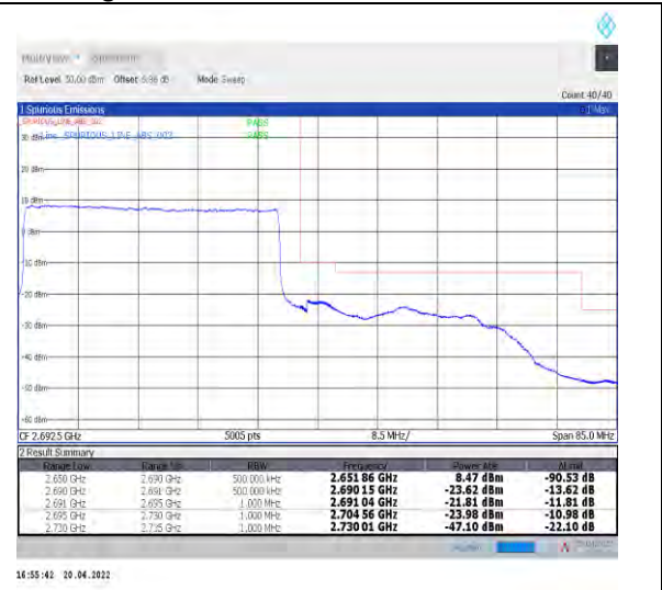
1-N41--30-40-H-3-DFT-PI2BPSK-Outer_Full-100@0-Ant1-PASS-see graph
