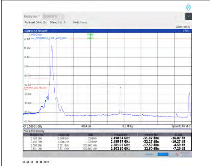
1-N41--30-70-L-4-CP-QPSK-Edge_1RB_Left-1@0-Ant1-PASS-see graph
