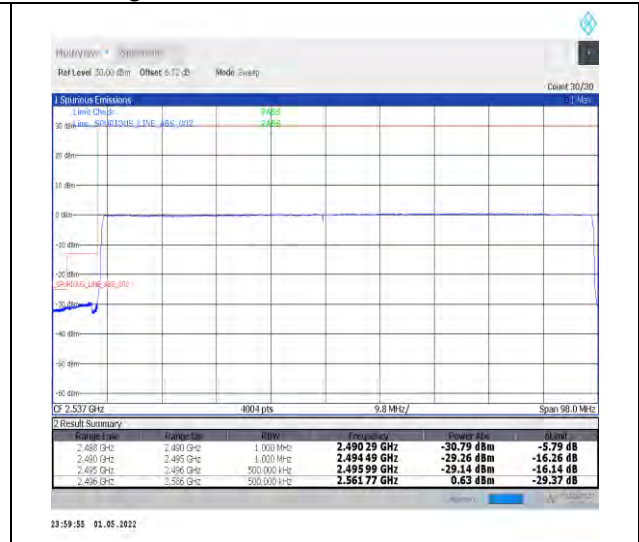
1-N41-PC2-30-90-L-6-CP-QPSK-Outer_Full-245 @0-Ant2-PASS-see graph
