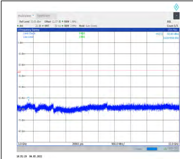
1-N41--30-100-L-1-DFT-PI2BPSK-Inner_1RB_Left-1 @1-3000-12000-Ant1--52.85--25-PASS
