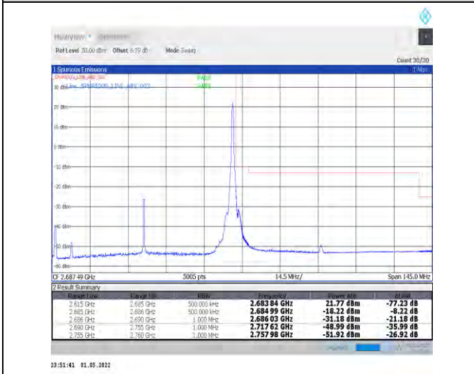
1-N41-PC2-30-70-H-5-CP-QPSK-Edge_1RB_Right-1@ 188-Ant2-PASS-see graph
