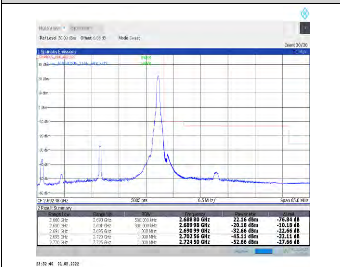
1-N41-PC2-30-30-H-5-CP-QPSK-Edge_1RB_Right-1@77 -Ant2-PASS-see graph
