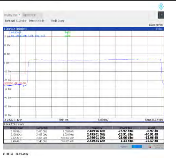
1-N41--30-50-L-6-CP-QPSK-Outer_Full-133@0-Ant1-PASS-see graph
