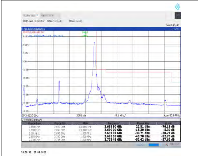
1-N41--30-40-H-5-CP-QPSK-Edge_1RB_Right-1@105-Ant1-PASS-see graph
