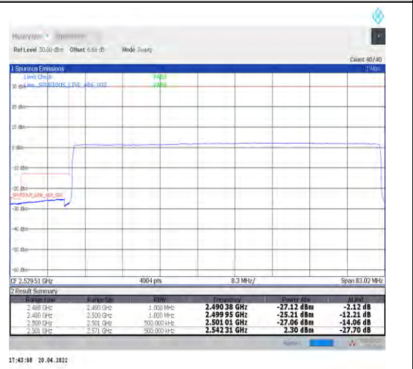
1-N41--30-70-L-6-CP-QPSK-Outer_Full-189@0-Ant1-PASS-see graph
