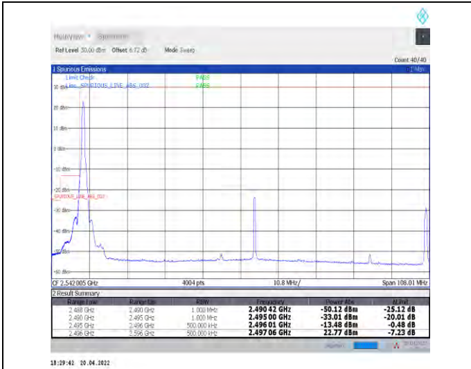
1-N41--30-100-L-1-DFT-PI2BPSK-Edge_1RB_Left-1@0-Ant1-PASS-see graph
