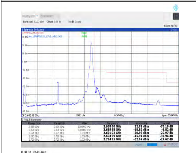
1-N41--30-30-H-5-CP-QPSK-Edge_1RB_Right-1@77-Ant1-PASS-see graph
