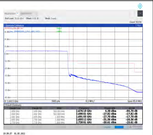
1-N41-PC2-30-40-H-6-CP-QPSK-Outer_Full-106 @0-Ant2-PASS-see graph
