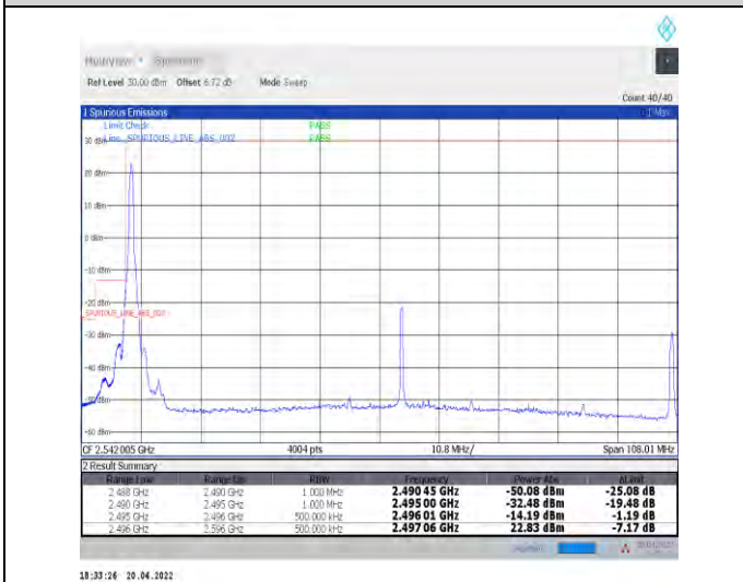
1-N41--30-100-L-4-CP-QPSK-Edge_1RB_Left-1@0-Ant1-PASS-see graph
