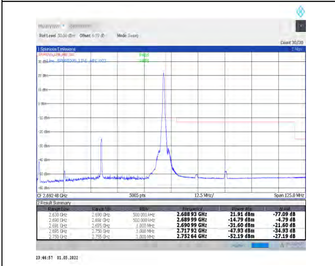
1-N41-PC2-30-60-H-5-CP-QPSK-Edge_1RB_Right-1@ 161-Ant2-PASS-see graph
