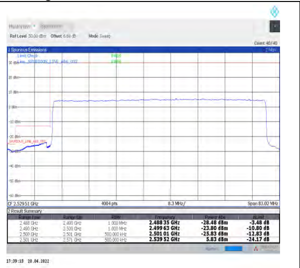
1-N41--30-70-L-3-DFT-PI2BPSK-Outer_Full-180@0-Ant1-PASS-see graph
