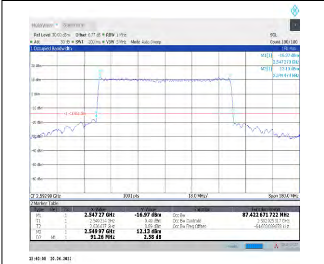
1-N41--30-90-M-9-CP-256QAM-Outer_Full-245@0-A nt1-87.423-91.260-<=90-PASS
