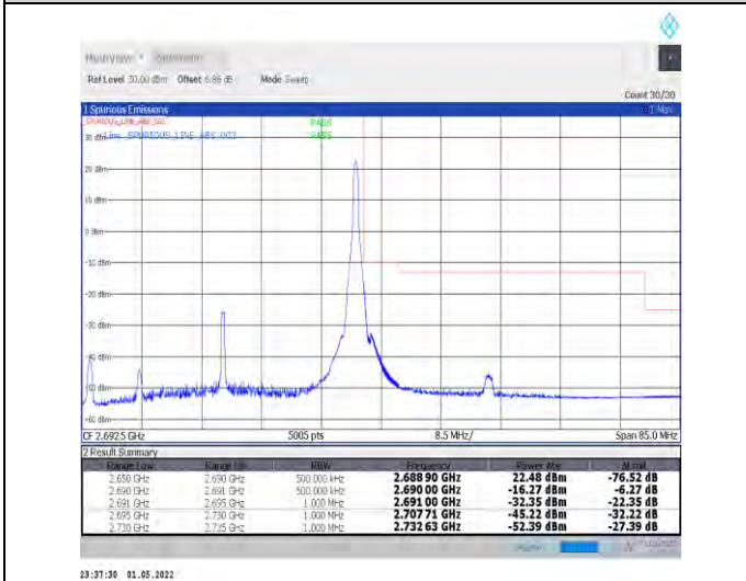
1-N41-PC2-30-40-H-5-CP-QPSK-Edge_1RB_Right-1@ 105-Ant2-PASS-see graph
