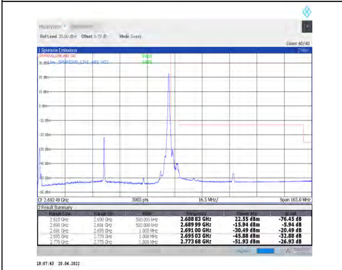
1-N41--30-80-H-5-CP-QPSK-Edge_1RB_Right-1@216-Ant1-PASS-see graph
