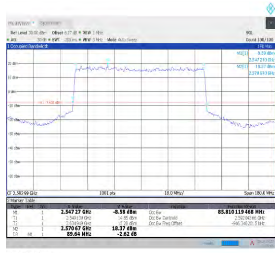
1-N41--30-90-M-2-DFT-PI2BPSK-Outer_Full-240@0-Ant 1-85.81-89.640-≤90-PASS
