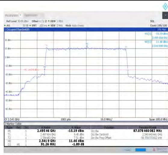
1-N41--30-90-L-9-CP-256QAM-Outer_Full-245@0-Ant 1-87.078-91.260-≤90-PASS
