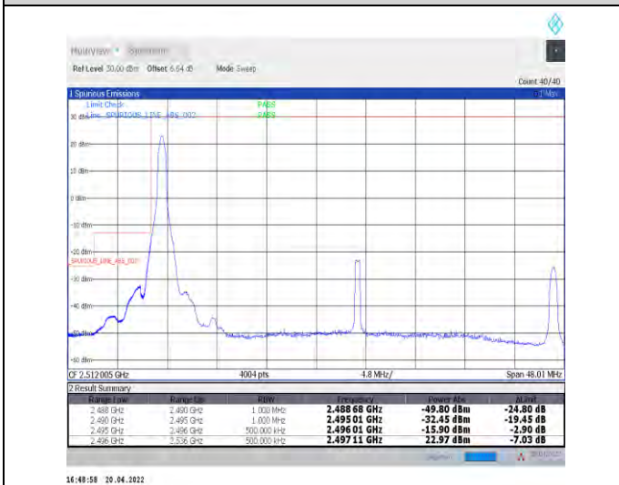
1-N41--30-40-L-4-CP-QPSK-Edge_1RB_Left-1@0-Ant1-PASS-see graph
