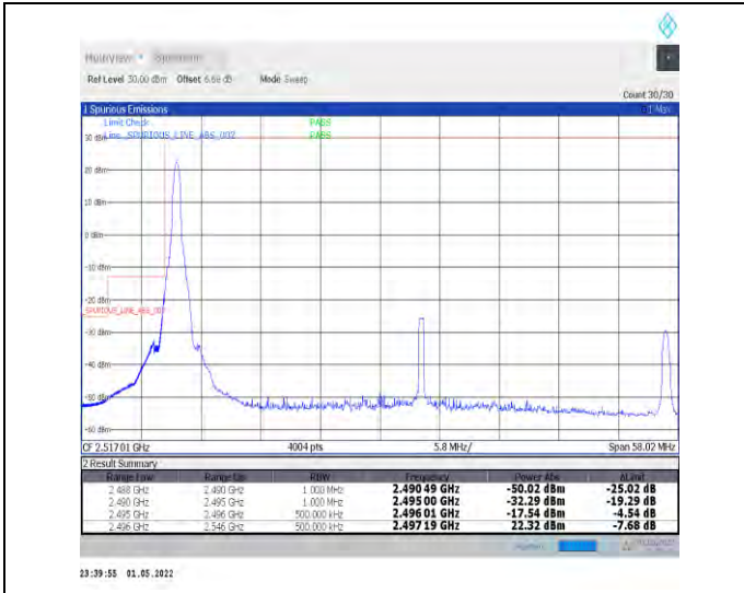
1-N41-PC2-30-50-L-4-CP-QPSK-Edge_1RB_Left-1@0 -Ant2-PASS-see graph
