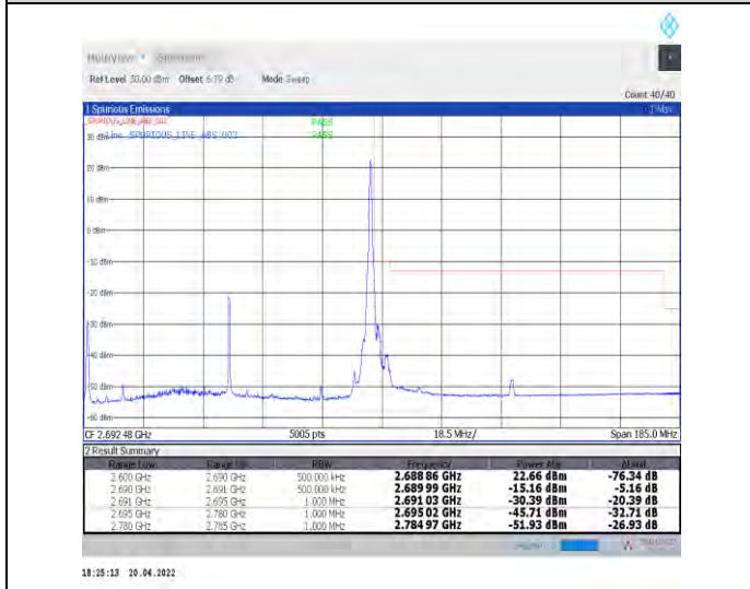
1-N41--30-90-H-5-CP-QPSK-Edge_1RB_Right-1@244-Ant1-PASS-see graph
