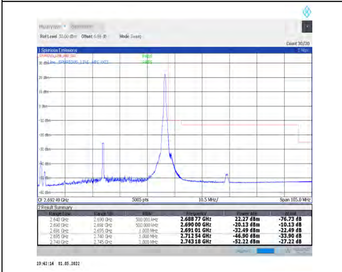
1-N41-PC2-30-50-H-5-CP-QPSK-Edge_1RB_Right-1@ 132-Ant2-PASS-see graph
