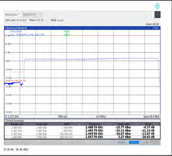
1-N41--30-60-L-6-CP-QPSK-Outer_Full-162@0-Ant1-PASS-see graph
