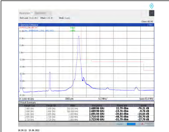
1-N41--30-30-H-2-DFT-PI2BPSK-Edge_1RB_Right-1@77-Ant1-PASS-see graph
