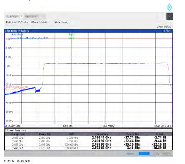
1-N41-PC2-30-30-L-6-CP-QPSK-Outer_Full-78@0 -Ant2-PASS-see graph
