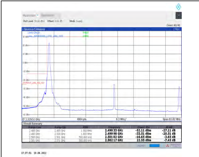
1-N41--30-70-L-1-DFT-PI2BPSK-Edge_1RB_Left-1@0-Ant1-PASS-see graph
