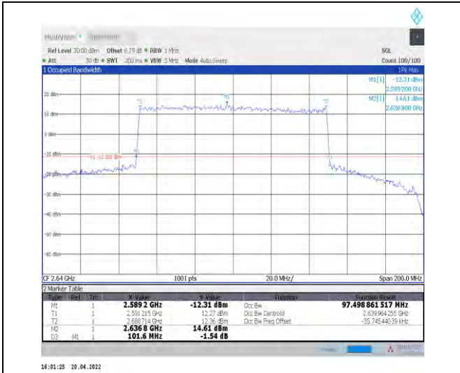
1-N41--30-100-H-7-CP-16QAM-Outer_Full-273@0-A nt1-97.499-101.600-≤100-PASS
