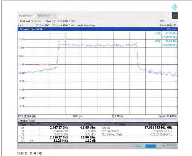
1-N41--30-90-M-7-CP-16QAM-Outer_Full-245@0-An t1-87.532-91.260-<=90-PASS
