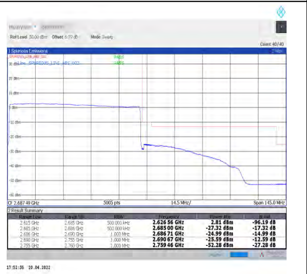
1-N41--30-70-H-6-CP-QPSK-Outer_Full-189@0-Ant1-PASS-see graph
