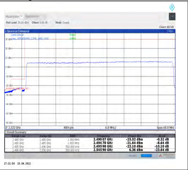
1-N41--30-60-L-3-DFT-PI2BPSK-Outer_Full-162@0-Ant1-PASS-see graph
