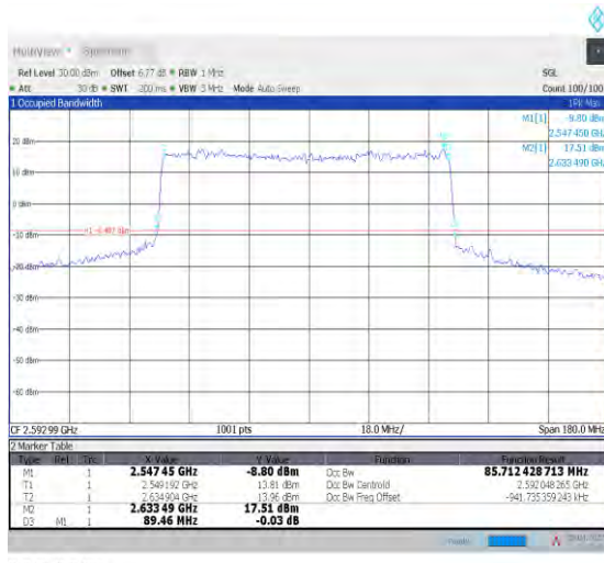
1-N41--30-90-M-1-DFT-QPSK-Outer_Full-240@0-Ant 1-85.712-89.460-≤90-PASS
