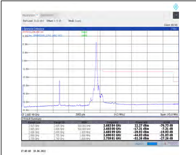
1-N41--30-70-H-2-DFT-PI2BPSK-Edge_1RB_Right-1@188-Ant1-PASS-see graph
