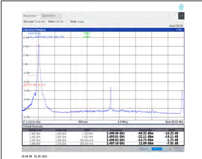
1-N41-PC2-30-80-L-4-CP-QPSK-Edge_1RB_Left-1@0 -Ant2-PASS-see graph
