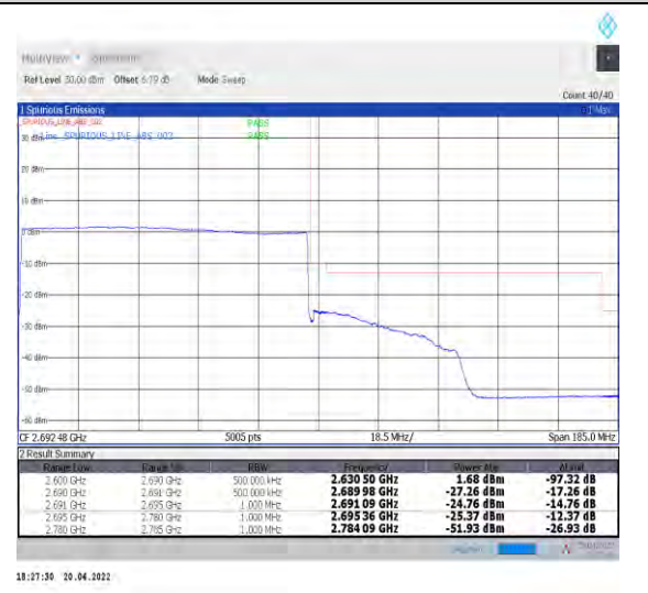
1-N41--30-90-H-6-CP-QPSK-Outer_Full-245@0-Ant1-PASS-see graph
