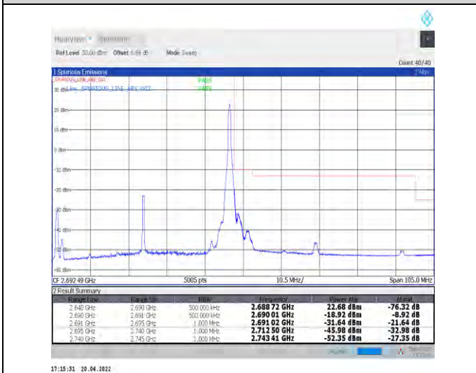
1-N41--30-50-H-5-CP-QPSK-Edge_1RB_Right-1@132-Ant1-PASS-see graph
