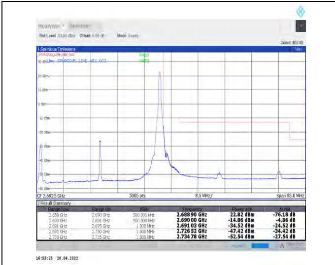
1-N41--30-40-H-2-DFT-PI2BPSK-Edge_1RB_Right-1@105-Ant1-PASS-see graph
