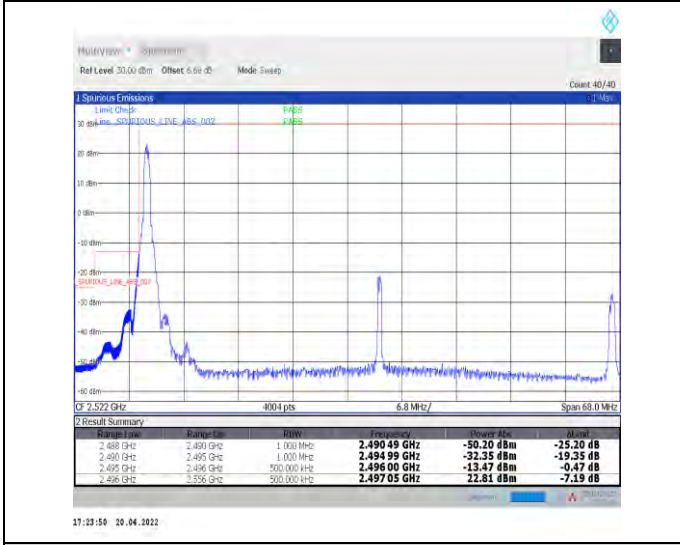
1-N41--30-60-L-4-CP-QPSK-Edge_1RB_Left-1@0-Ant1-PASS-see graph
