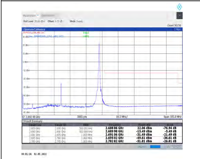
1-N41-PC2-30-90-H-5-CP-QPSK-Edge_1RB_Right-1@ 244-Ant2-PASS-see graph
