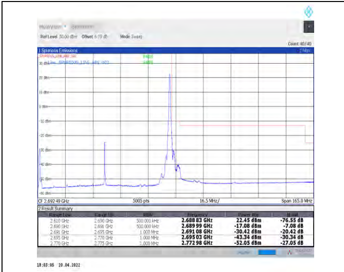
1-N41--30-80-H-2-DFT-PI2BPSK-Edge_1RB_Right-1@216-Ant1-PASS-see graph
