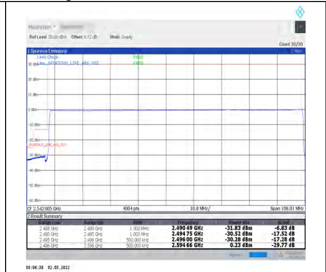
1-N41-PC2-30-100-L-6-CP-QPSK-Outer_Full-273 @0-Ant2-PASS-see graph
