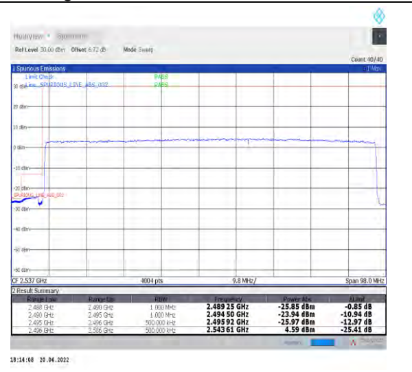
1-N41--30-90-L-3-DFT-PI2BPSK-Outer_Full-240@0-Ant1-PASS-see graph
