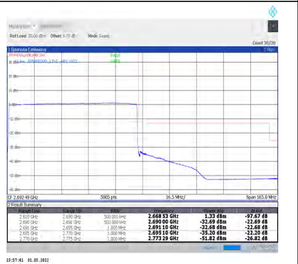
1-N41-PC2-30-80-H-6-CP-QPSK-Outer_Full-217 @0-Ant2-PASS-see graph
