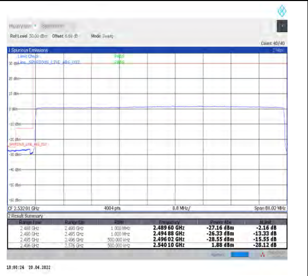
1-N41--30-80-L-6-CP-QPSK-Outer_Full-217@0-Ant1-PASS-see graph
