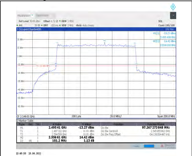
1-N41--30-100-L-6-CP-QPSK-Outer_Full-273@0-An t1-97.267-101.200-≤100-PASS
