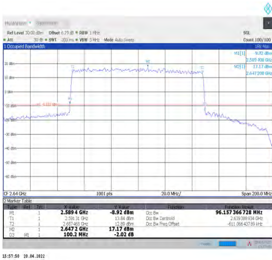
1-N41--30-100-H-1-DFT-QPSK-Outer_Full-270@0-A nt1-96.157-100.200-≤100-PASS
