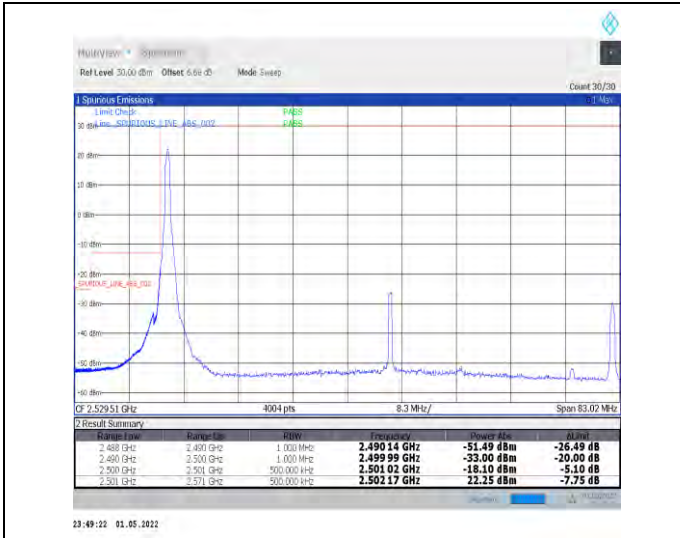
1-N41-PC2-30-70-L-4-CP-QPSK-Edge_1RB_Left-1@0 -Ant2-PASS-see graph
