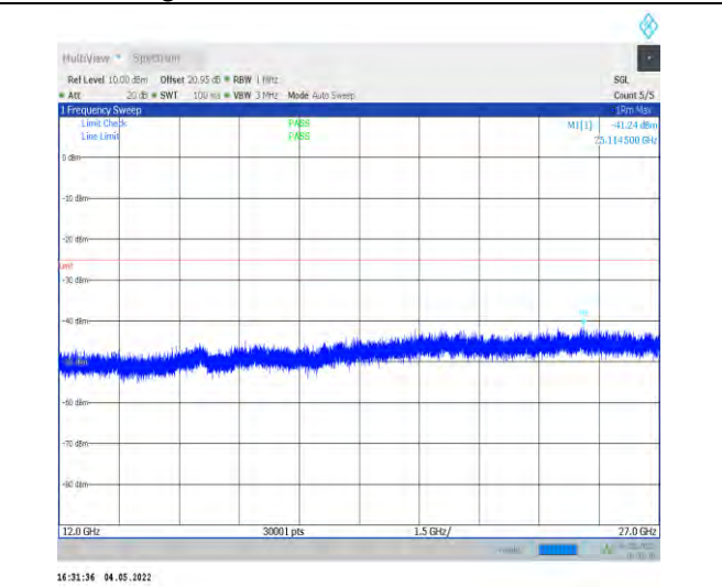
1-N41--30-100-L-1-DFT-PI2BPSK-Inner_1RB_Left-1 @1-12000-27000-Ant1--41.24--25-PASS
