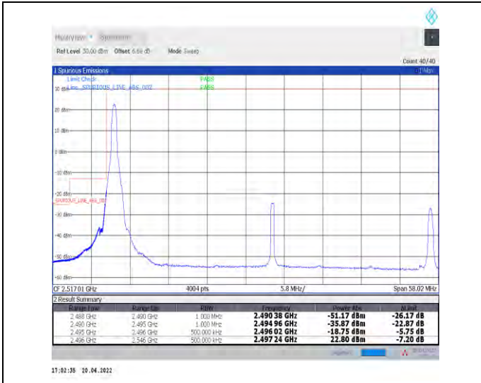
1-N41--30-50-L-1-DFT-PI2BPSK-Edge_1RB_Left-1@0-Ant1-PASS-see graph
