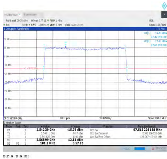
1-N41--30-100-M-9-CP-256QAM-Outer_Full-273@0-A Ant1-97.512-101.200-≤100-PASS
