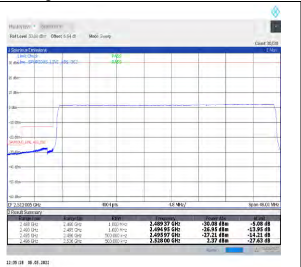
1-N41-PC2-30-40-L-6-CP-QPSK-Outer_Full-106 @0-Ant2-PASS-see graph
