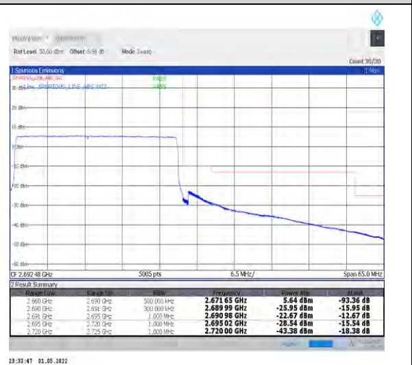
1-N41-PC2-30-30-H-6-CP-QPSK-Outer_Full-78@0 -Ant2-PASS-see graph
