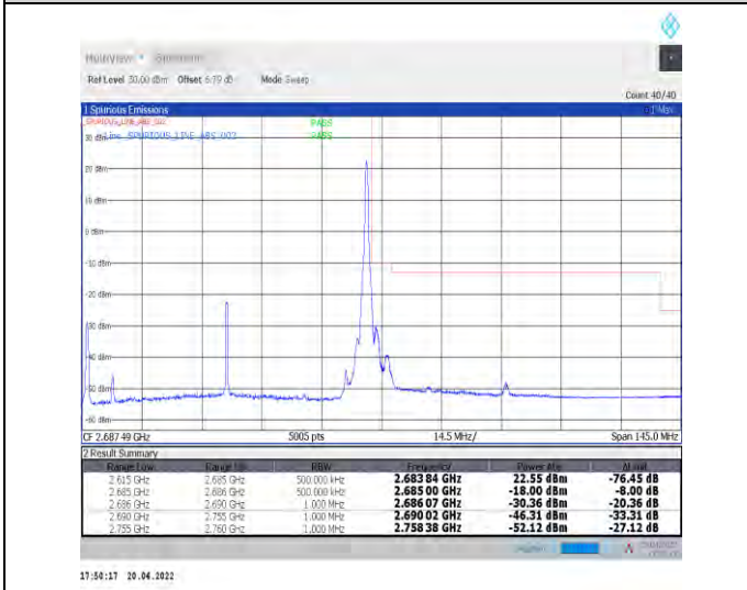
1-N41--30-70-H-5-CP-QPSK-Edge_1RB_Right-1@188-Ant1-PASS-see graph
