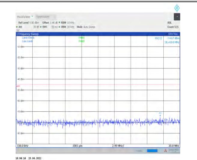
1-N41--30-100-M-1-DFT-PI2BPSK-Inner_1RB_Left-1 @1-0.15-30-Ant1--74.67--45-PASS
