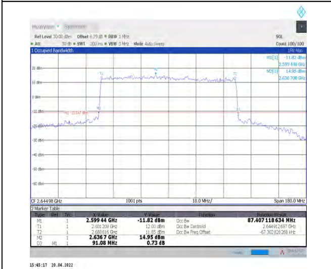
1-N41--30-90-H-8-CP-64QAM-Outer_Full-245@0-An t1-87.407-91.080-≤90-PASS
