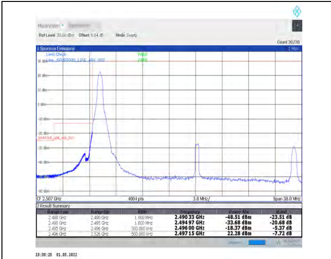
1-N41-PC2-30-30-L-4-CP-QPSK-Edge_1RB_Left-1@0 -Ant2-PASS-see graph
