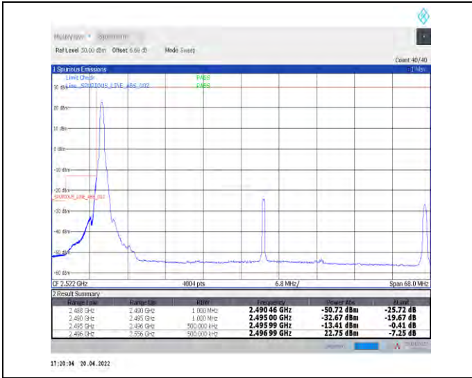
1-N41--30-60-L-1-DFT-PI2BPSK-Edge_1RB_Left-1@0-Ant1-PASS-see graph
