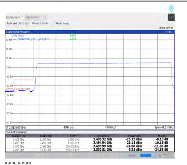
1-N41--30-40-L-6-CP-QPSK-Outer_Full-106@0-Ant1-PASS-see graph
