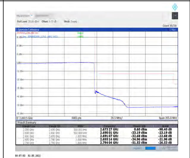
1-N41-PC2-30-100-H-6-CP-QPSK-Outer_Full-273 @0-Ant2-PASS-see graph
