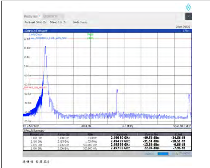
1-N41-PC2-30-60-L-4-CP-QPSK-Edge_1RB_Left-1@0 -Ant2-PASS-see graph
