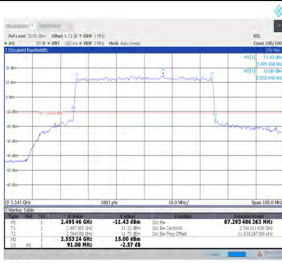
1-N41--30-90-L-8-CP-64QAM-Outer_Full-245@0-Ant 1-87.293-91.080-≤90-PASS
