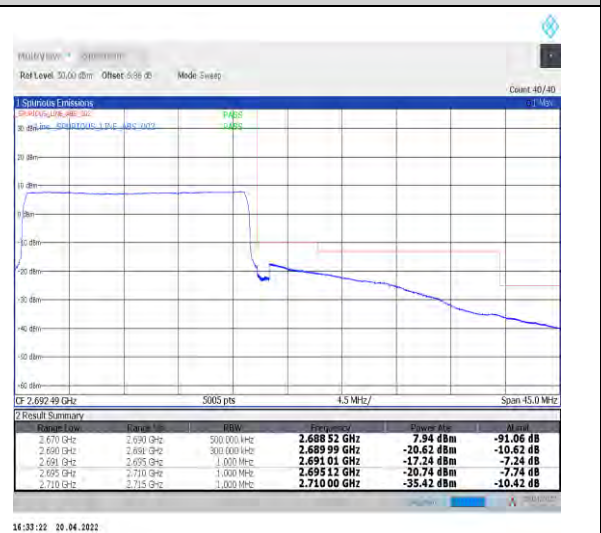
1-N41--30-20-H-6-CP-QPSK-Outer_Full-51@0-Ant1-PASS-see graph
