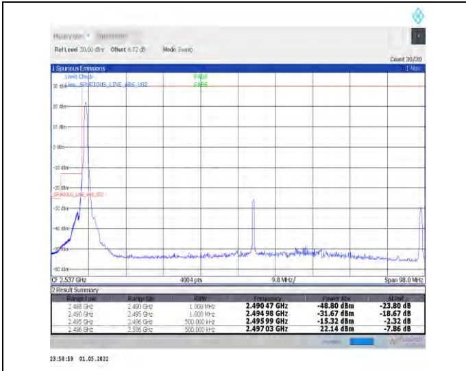
1-N41-PC2-30-90-L-4-CP-QPSK-Edge_1RB_Left-1@0 -Ant2-PASS-see graph
