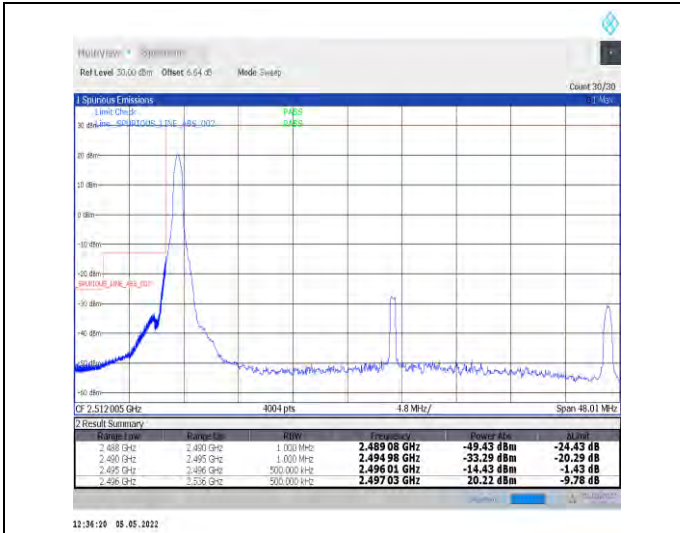
1-N41-PC2-30-40-L-4-CP-QPSK-Edge_1RB_Left-1@0 -Ant2-PASS-see graph
