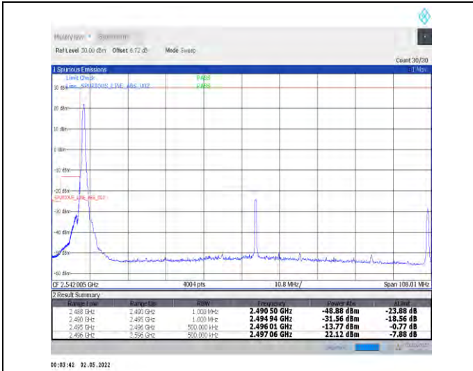
1-N41-PC2-30-100-L-4-CP-QPSK-Edge_1RB_Left-1@ 0-Ant2-PASS-see graph
