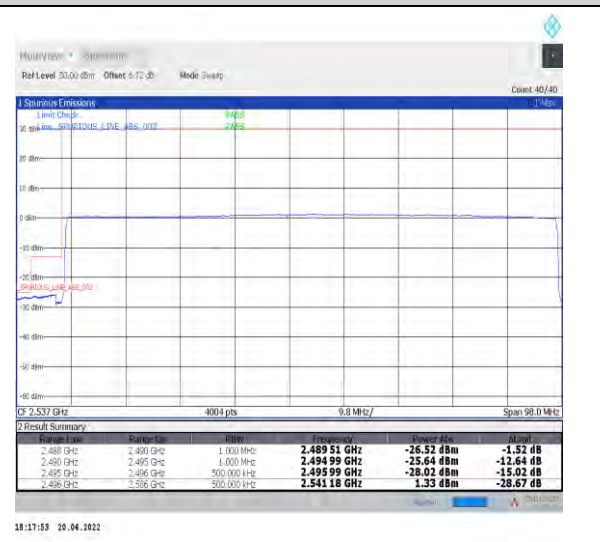
1-N41--30-90-L-6-CP-QPSK-Outer_Full-245@0-Ant1-PASS-see graph
