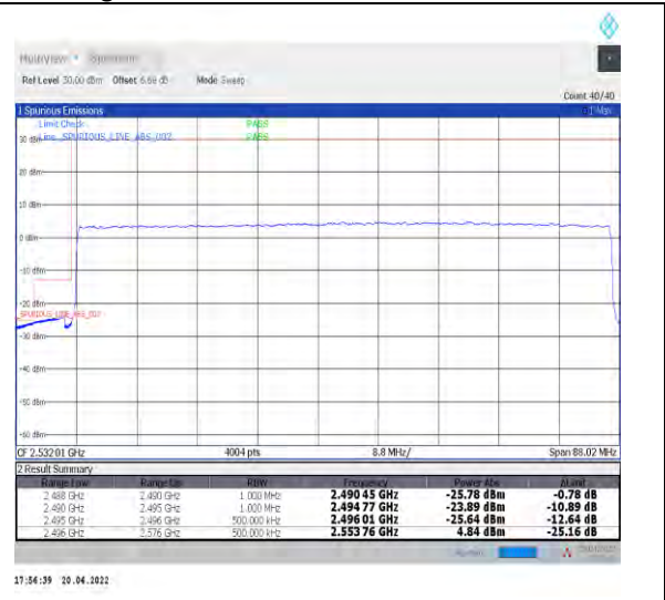
1-N41--30-80-L-3-DFT-PI2BPSK-Outer_Full-216@0-Ant1-PASS-see graph
