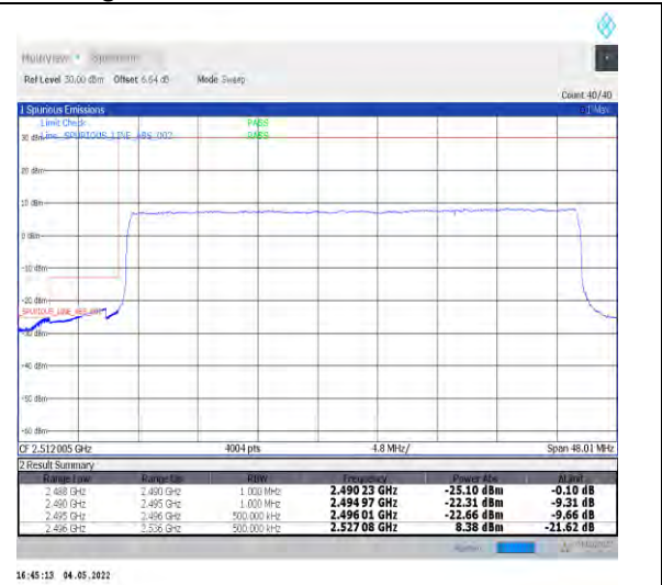
1-N41--30-40-L-3-DFT-PI2BPSK-Outer_Full-100@0-Ant1-PASS-see graph
