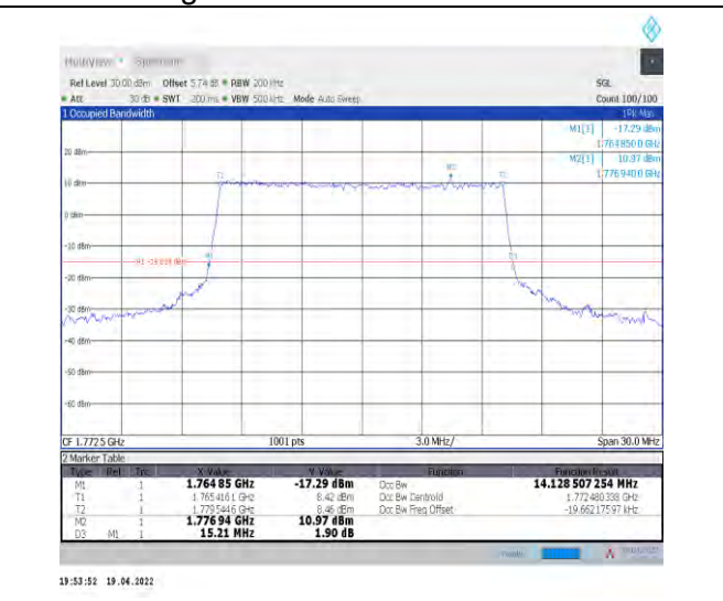
1-N66-PC3-15-15-H-6-CP-QPSK-Outer_Full-79@0-Ant1-14.129-15.210-≤15-PASS
