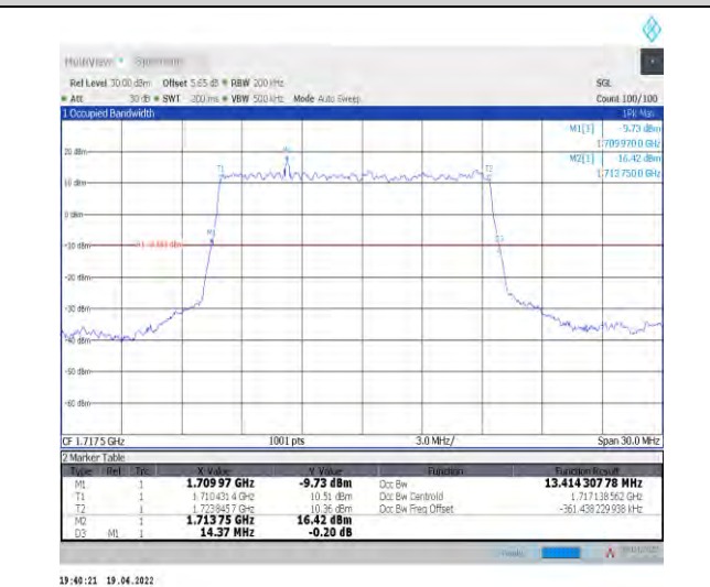
1-N66-PC3-15-15-L-2-DFT-PI2BPSK-Outer_Full-75@0- Ant1-13.414-14.370-≤15-PASS
