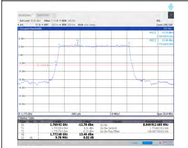
1-N66-PC3-15-10-H-2-DFT-PI2BPSK-Outer_Full-50 @0-Ant1-8.95-9.780-≤10-PASS
