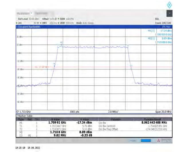
1-N66-PC3-15-10-L-5-DFT-256QAM-Outer_Full-50 @0-Ant1-8.962-9.820-≤10-PASS
