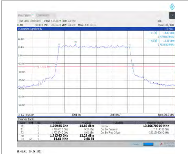
1-N66-PC3-15-15-L-3-DFT-16QAM-Outer_Full-75@ 0-Ant1-13.467-14.610-≤15-PASS
