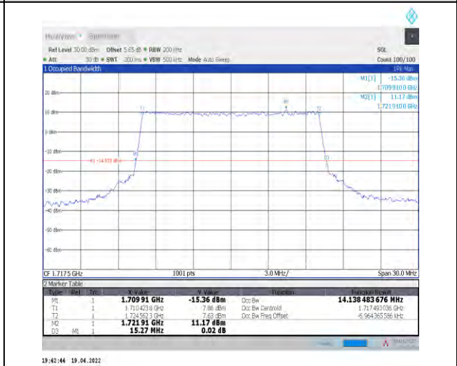
1-N66-PC3-15-15-L-6-CP-QPSK-Outer_Full-79@0-A nt1-14.138-15.270-≤15-PASS
