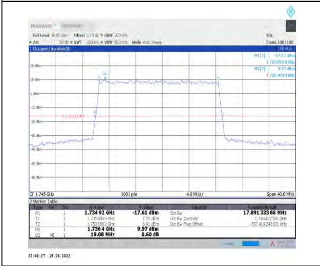
1-N66-PC3-15-20-M-5-DFT-256QAM-Outer_Full-100 @0-Ant1-17.891-19.080-≤20-PASS
