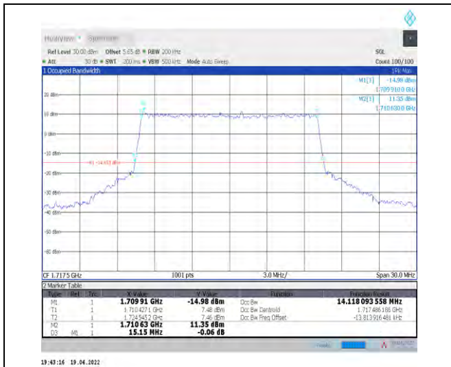
1-N66-PC3-15-15-L-7-CP-16QAM-Outer_Full-79@0-Ant1-14.118-15.150-≤15-PASS
