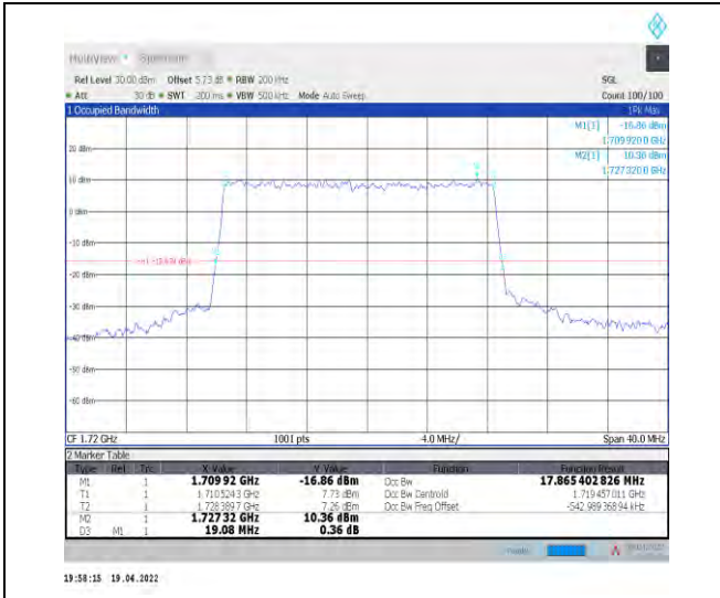
1-N66-PC3-15-20-L-4-DFT-64QAM-Outer_Full-100 @0-Ant1-17.865-19.080-≤20-PASS
