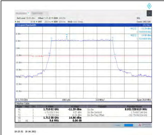
1-N66-PC3-15-10-L-2-DFT-PI2BPSK-Outer_Full-50 @0-Ant1-8.952-9.600-≤10-PASS
