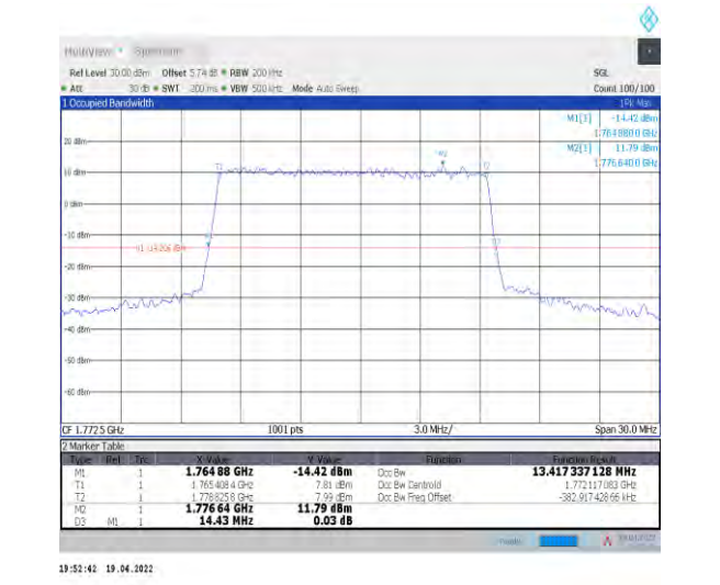
1-N66-PC3-15-15-H-4-DFT-64QAM-Outer_Full-75@0-Ant1-13.417-14.430-≤15-PASS
