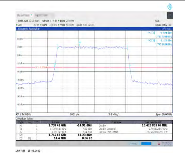
1-N66-PC3-15-15-M-5-DFT-256QAM-Outer_Full-75 @0-Ant1-13.429-14.400-≤15-PASS
