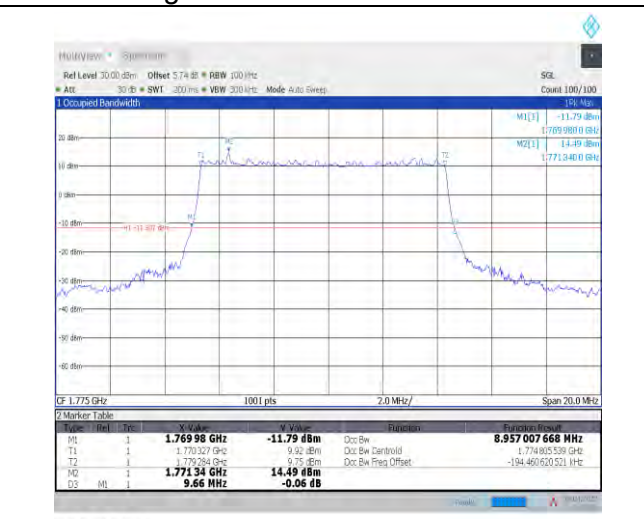
1-N66-PC3-15-10-H-1-DFT-QPSK-Outer_Full-50@0- Ant1-8.957-9.660-≤10-PASS
