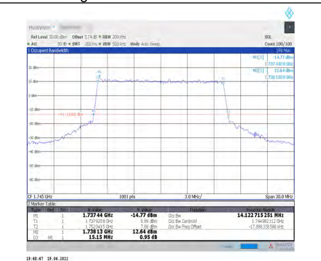
1-N66-PC3-15-15-M-7-CP-16QAM-Outer_Full-79@0-Ant1-14.123-15.150-≤15-PASS
