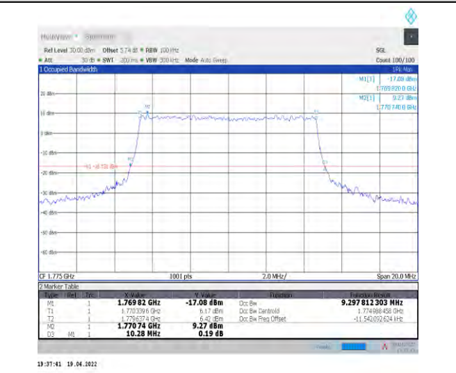
1-N66-PC3-15-10-H-7-CP-16QAM-Outer_Full-52@0 -Ant1-9.298-10.280-≤10-PASS
