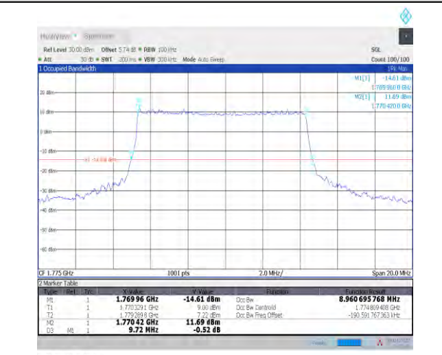
1-N66-PC3-15-10-H-3-DFT-16QAM-Outer_Full-50@ 0-Ant1-8.961-9.720-≤10-PASS
