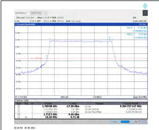
1-N66-PC3-15-10-L-6-CP-QPSK-Outer_Full-52@0-Ant1-9.305-10.260-≤10-PASS
