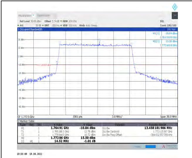
1-N66-PC3-15-15-H-1-DFT-QPSK-Outer_Full-75@0-Ant1-13.458-14.520-≤15-PASS
