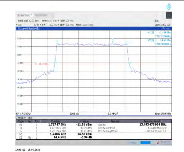
1-N66-PC3-15-15-M-1-DFT-QPSK-Outer_Full-75@0-Ant1-13.493-14.400-≤15-PASS
