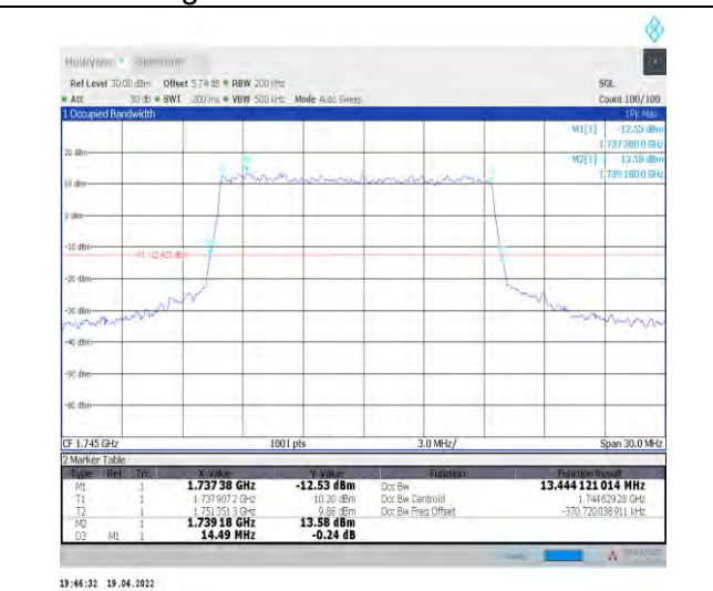
1-N66-PC3-15-15-M-3-DFT-16QAM-Outer_Full-75 @0-Ant1-13.444-14.490-≤15-PASS
