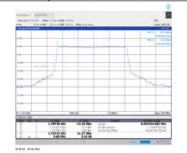
1-N66-PC3-15-10-L-3-DFT-16QAM-Outer_Full-50 @0-Ant1-8.955-9.680-≤10-PASS
