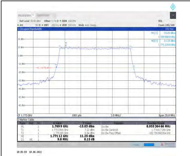
1-N66-PC3-15-10-H-4-DFT-64QAM-Outer_Full-50@ 0-Ant1-8.955-9.800-≤10-PASS
