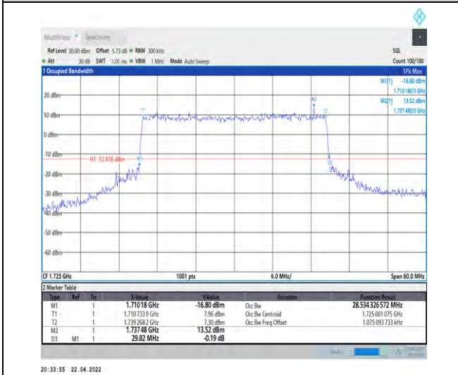
1-N66-PC3-15-30-L-7-CP-16QAM-Outer_Full-160@0-Ant1-28.534-29.820-≤30-PASS
