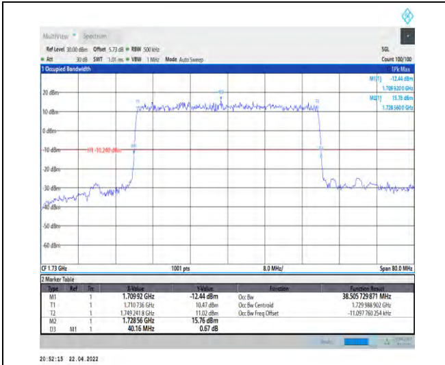
1-N66-PC3-15-40-L-2-DFT-PI2BPSK-Outer_Full-216 @0-Ant1-38.506-40.160-≤40-PASS
