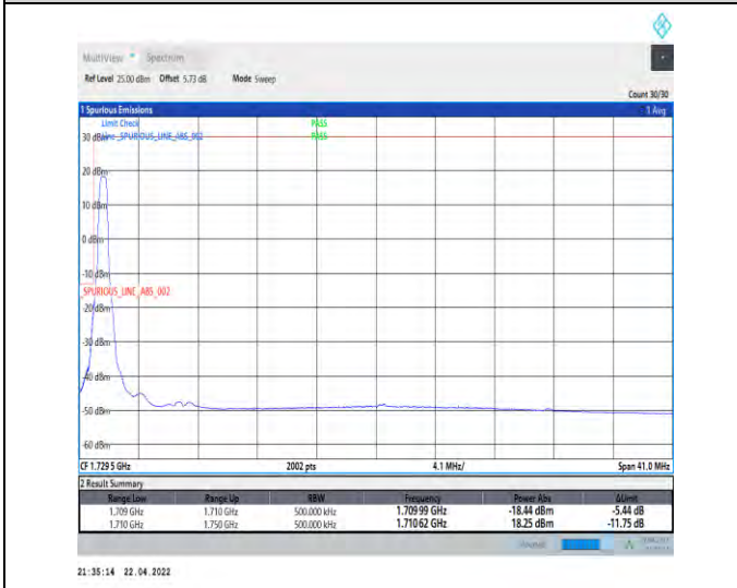
1-N66-PC3-15-40-L-4-CP-QPSK-Edge_1RB_Left-1@0-Ant1-seegraph-PASS-see graph
