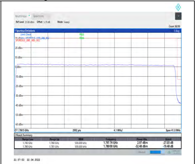
1-N66-PC3-15-40-H-3-DFT-PI2BPSK-Outer_Full-216@0-Ant1-seegraph-PASS-see graph
