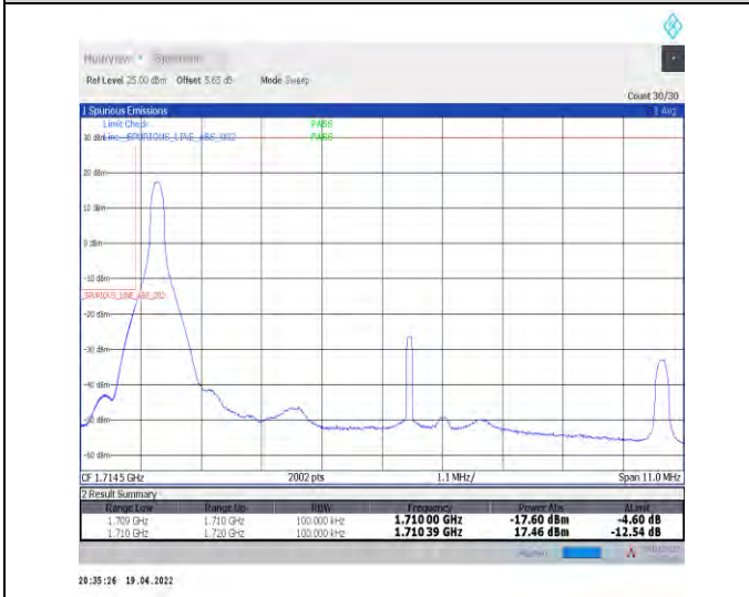
1-N66-PC3-15-10-L-4-CP-QPSK-Edge_1RB_Left-1@0-Ant1-seegraph-PASS-see graph
