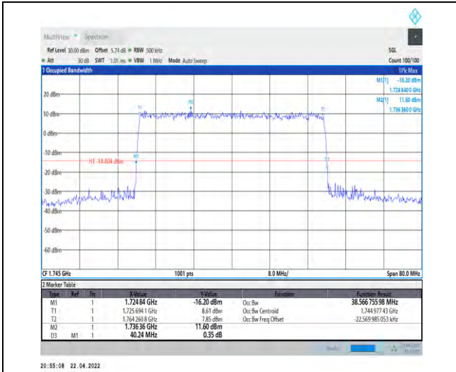
1-N66-PC3-15-40-M-5-DFT-256QAM-Outer_Full-216 @0-Ant1-38.567-40.240-≤40-PASS
