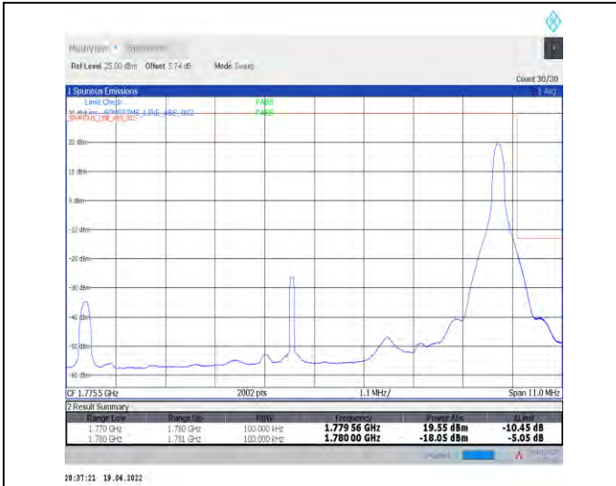
1-N66-PC3-15-10-H-2-DFT-PI2BPSK-Edge_1RB_Right-t-1@51-Ant1-seegraph-PASS-see graph
