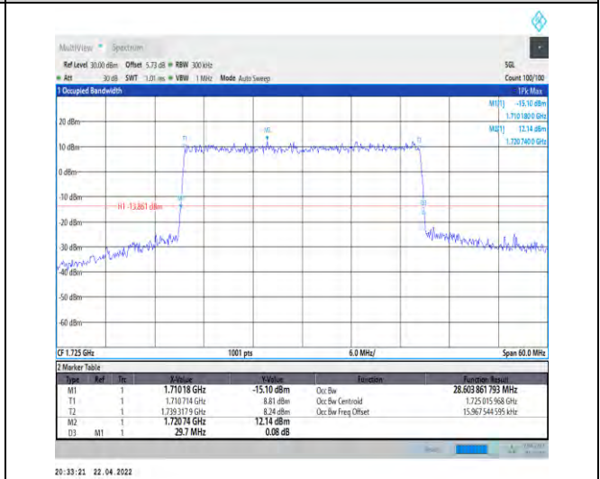
1-N66-PC3-15-30-L-4-DFT-64QAM-Outer_Full-160 @0-Ant1-28.604-29.700-≤30-PASS
