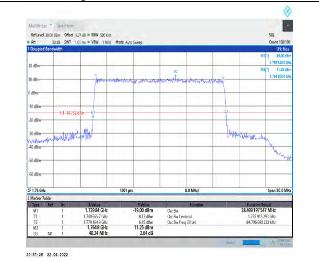
1-N66-PC3-15-40-H-5-DFT-256QAM-Outer_Full-216 @0-Ant1-38.499-40.240-≤40-PASS
