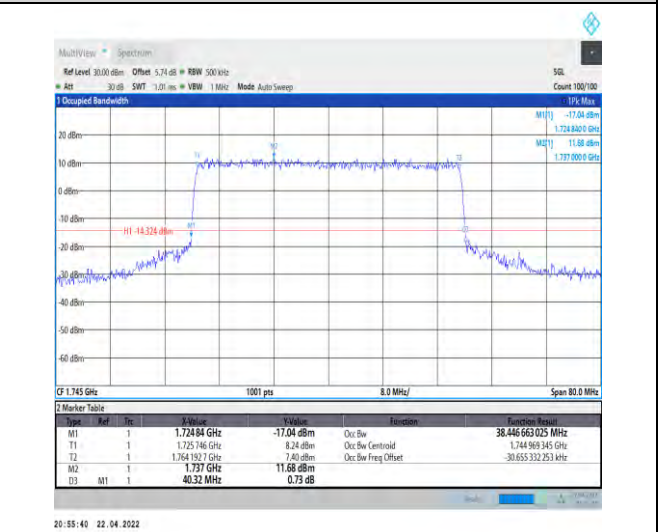
1-N66-PC3-15-40-M-8-CP-64QAM-Outer_Full-216 @0-Ant1-38.447-40.320-≤40-PASS
