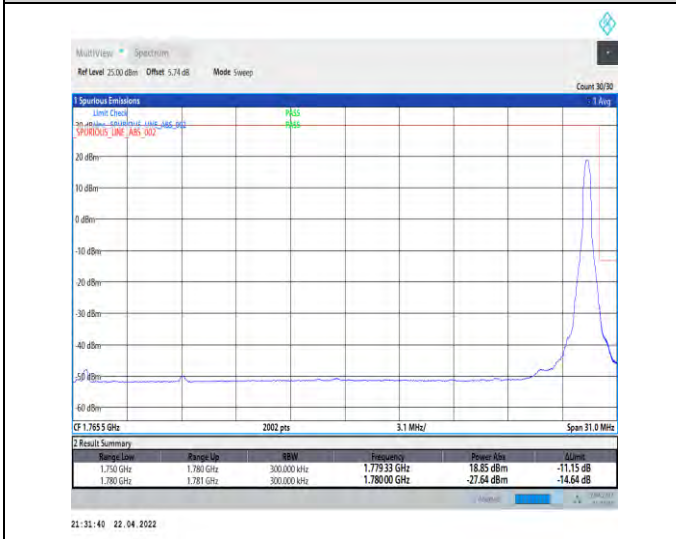
1-N66-PC3-15-30-H-5-CP-QPSK-Edge_1RB_Right-1@159-Ant1-seegraph-PASS-see graph
