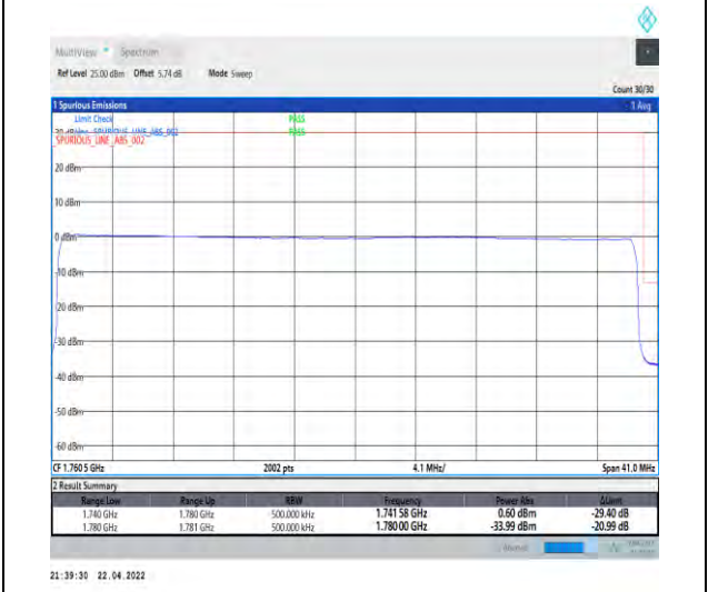
1-N66-PC3-15-40-H-6-CP-QPSK-Outer_Full-216@0-Ant1-seegraph-PASS-see graph
