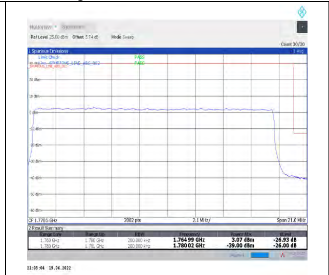
1-N66-PC3-15-20-H-3-DFT-PI2BPSK-Outer_Full-100@0-Ant1-seegraph-PASS-see graph
