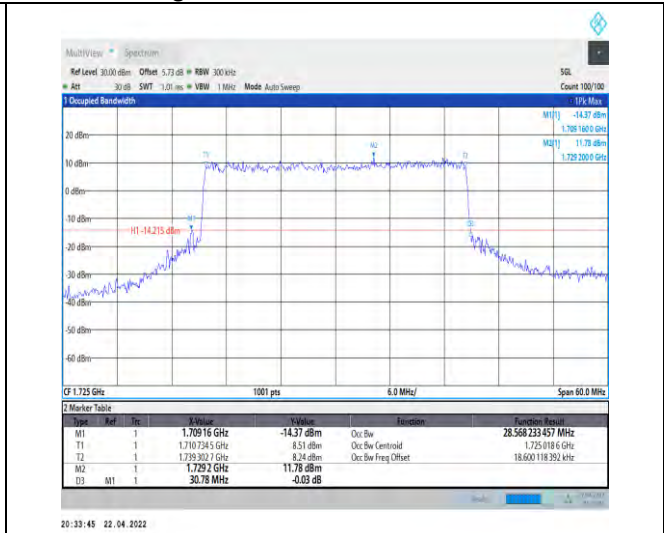
1-N66-PC3-15-30-L-6-CP-QPSK-Outer_Full-160@0-Ant1-28.568-30.780-≤30-PASS
