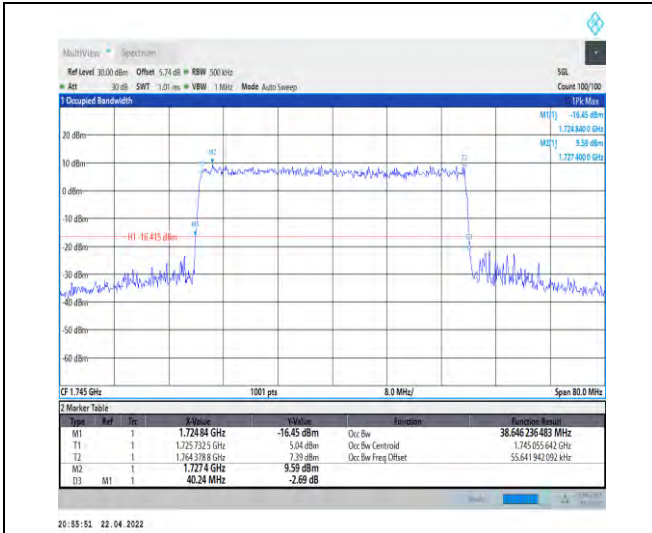
1-N66-PC3-15-40-M-9-CP-256QAM-Outer_Full-216 @0-Ant1-38.646-40.240-≤40-PASS
