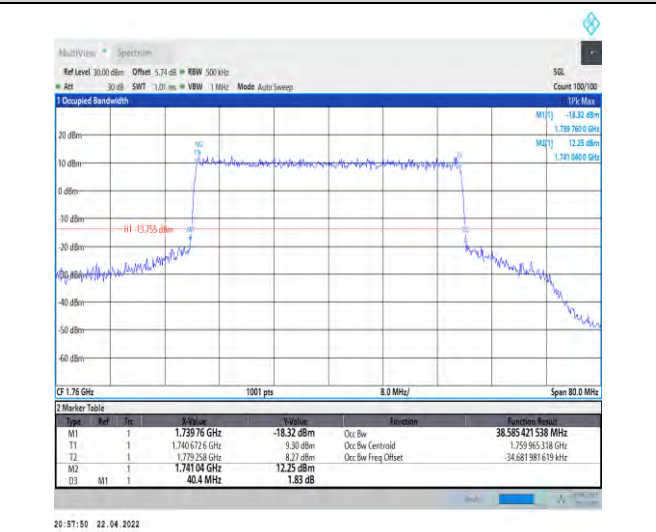
1-N66-PC3-15-40-H-7-CP-16QAM-Outer_Full-216@0-Ant1-38.585-40.400-≤40-PASS
