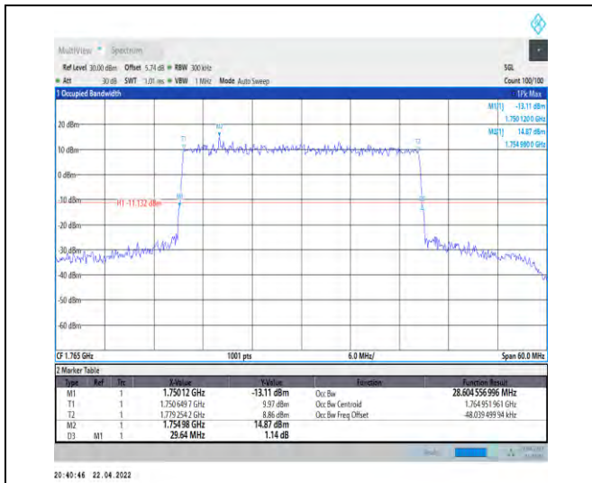
1-N66-PC3-15-30-H-3-DFT-16QAM-Outer_Full-160 @0-Ant1-28.605-29.640-≤30-PASS
