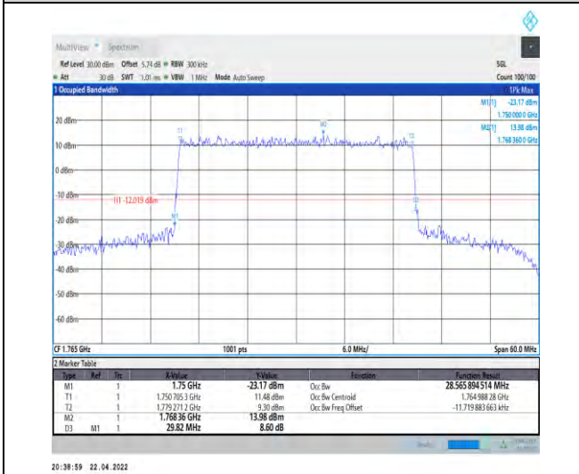
1-N66-PC3-15-30-H-1-DFT-QPSK-Outer_Full-160@ 0-Ant1-28.566-29.820-≤30-PASS
