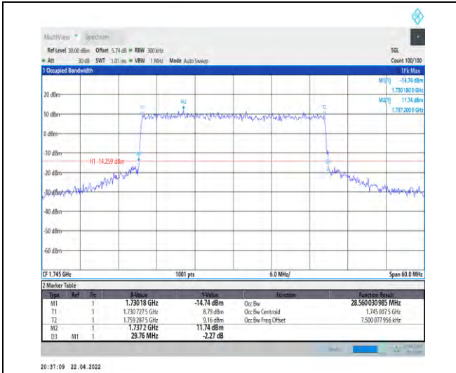
1-N66-PC3-15-30-M-8-CP-64QAM-Outer_Full-160@ 0-Ant1-28.56-29.760-≤30-PASS
