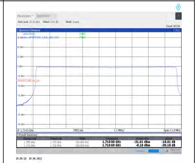
1-N66-PC3-15-10-L-6-CP-QPSK-Outer_Full-52@0-Ant1-seegraph-PASS-see graph
