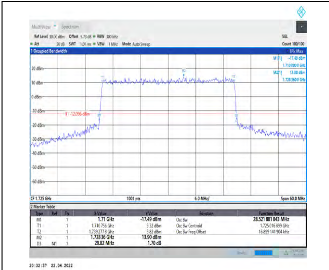
1-N66-PC3-15-30-L-1-DFT-QPSK-Outer_Full-160@ 0-Ant1-28.522-29.820-≤30-PASS
