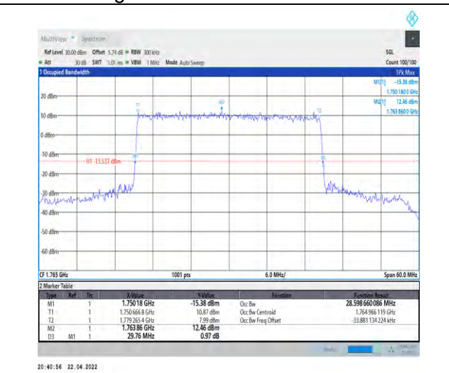
1-N66-PC3-15-30-H-4-DFT-64QAM-Outer_Full-160 @0-Ant1-28.599-29.760-≤30-PASS
