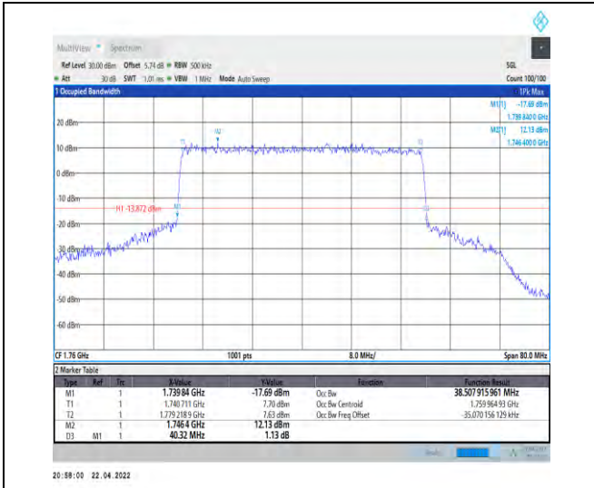
1-N66-PC3-15-40-H-8-CP-64QAM-Outer_Full-216@ 0-Ant1-38.508-40.320-≤40-PASS
