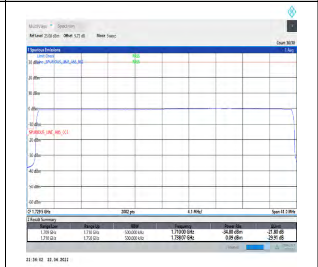
1-N66-PC3-15-40-L-6-CP-QPSK-Outer_Full-216@0-Ant1-seegraph-PASS-see graph
