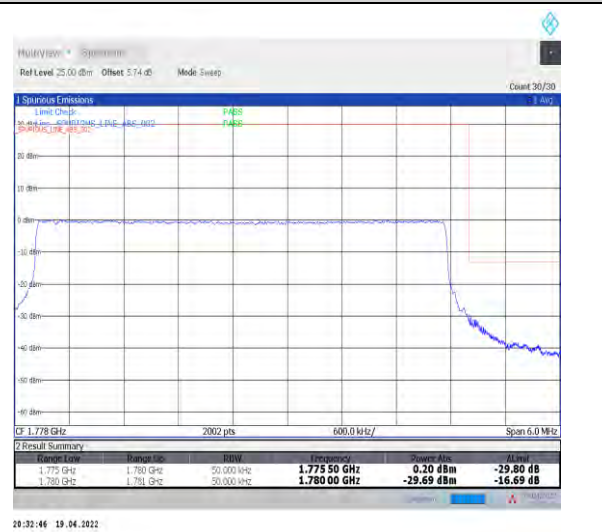
1-N66-PC3-15-5-H-6-CP-QPSK-Outer_Full-25@0-Ant1-seegraph-PASS-see graph
