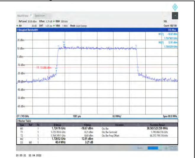
1-N66-PC3-15-40-M-6-CP-QPSK-Outer_Full-216 @0-Ant1-38.566-40.400-≤40-PASS
