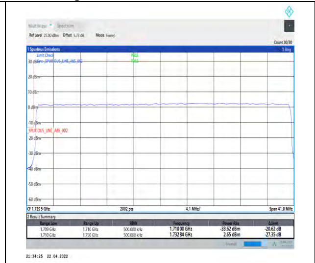
1-N66-PC3-15-40-L-3-DFT-PI2BPSK-Outer_Full-216@0-Ant1-seegraph-PASS-see graph
