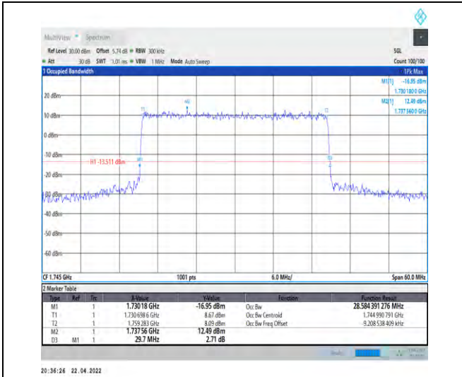
1-N66-PC3-15-30-M-4-DFT-64QAM-Outer_Full-160 @0-Ant1-28.584-29.700-≤30-PASS
