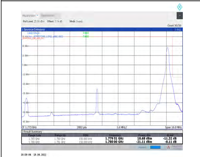
1-N66-PC3-15-15-H-5-CP-QPSK-Edge_1RB_Right-1@78-Ant1-seegraph-PASS-see graph
