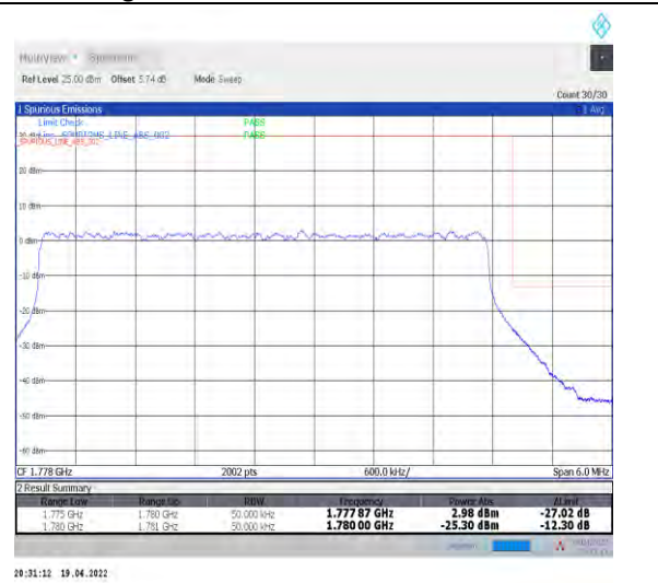
1-N66-PC3-15-5-H-3-DFT-PI2BPSK-Outer_Full-25@0-Ant1-seegraph-PASS-see graph
