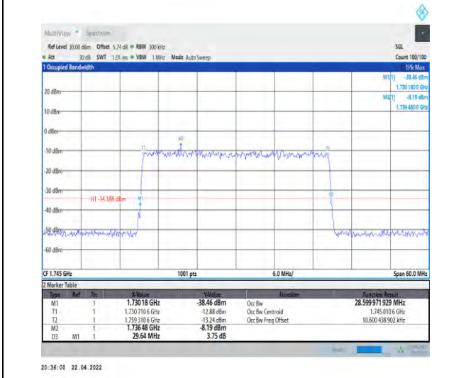
1-N66-PC3-15-30-M-2-DFT-PI2BPSK-Outer_Full-160 @0-Ant1-28.6-29.640-≤30-PASS
