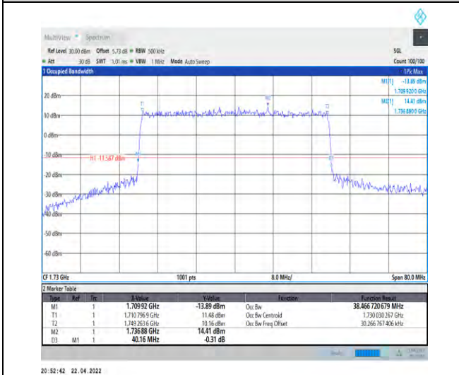
1-N66-PC3-15-40-L-4-DFT-64QAM-Outer_Full-216 @0-Ant1-38.467-40.160-≤40-PASS
