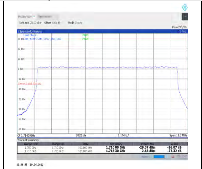
1-N66-PC3-15-10-L-3-DFT-PI2BPSK-Outer_Full-50@0-Ant1-seegraph-PASS-see graph
