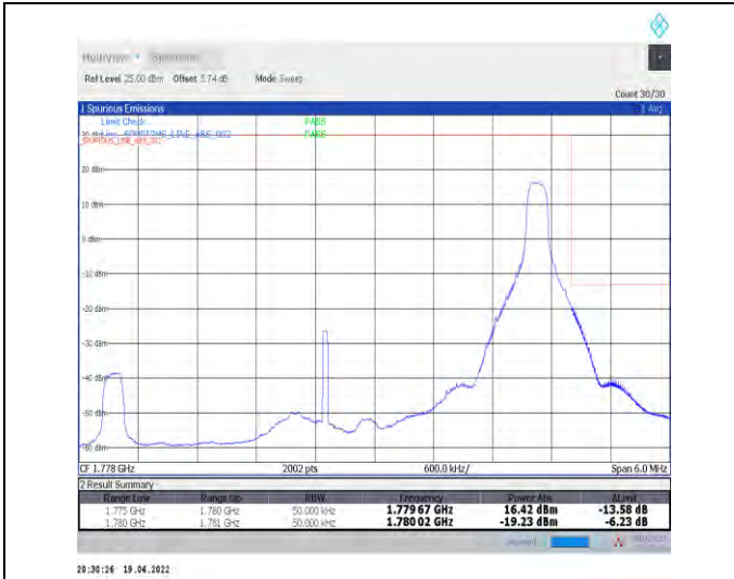
1-N66-PC3-15-5-H-2-DFT-PI2BPSK-Edge_1RB_Right-1@24-Ant1-seegraph-PASS-see graph
