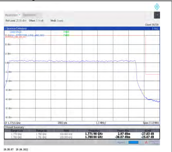
1-N66-PC3-15-10-H-3-DFT-PI2BPSK-Outer_Full-50@0-Ant1-seegraph-PASS-see graph
