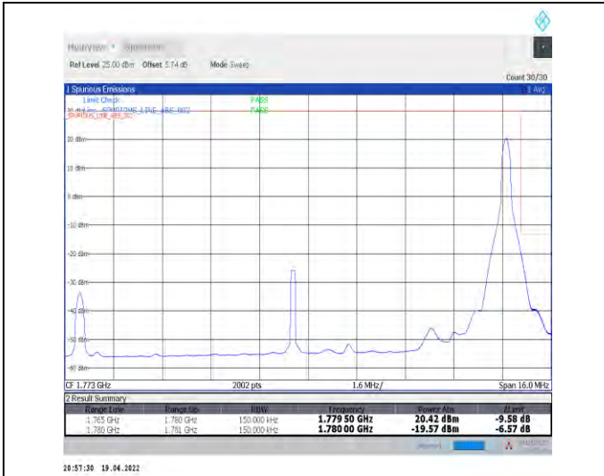
1-N66-PC3-15-15-H-2-DFT-PI2BPSK-Edge_1RB_Right-t-1@78-Ant1-seegraph-PASS-see graph
