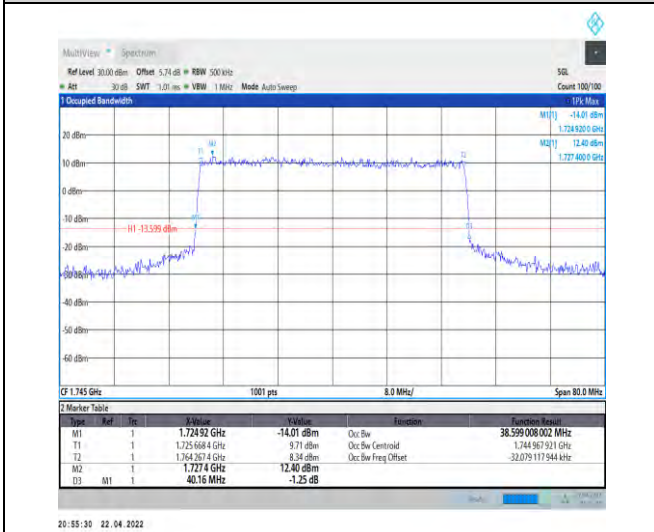
1-N66-PC3-15-40-M-7-CP-16QAM-Outer_Full-216 @0-Ant1-38.599-40.160-≤40-PASS
