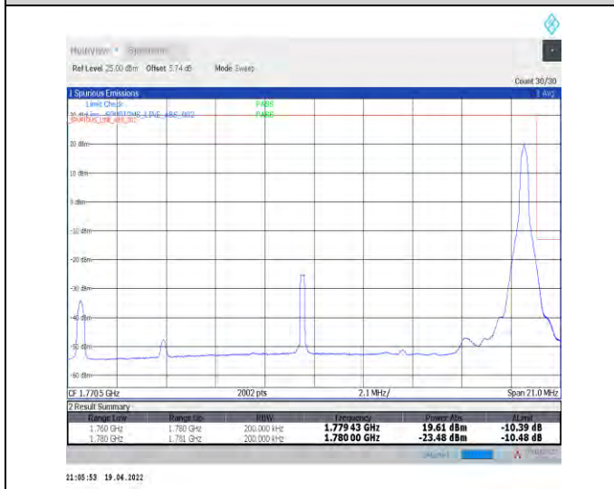
1-N66-PC3-15-20-H-5-CP-QPSK-Edge_1RB_Right-1@105-Ant1-seegraph-PASS-see graph
