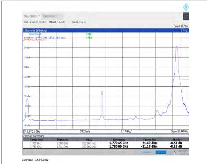
1-N66-PC3-15-20-H-2-DFT-PI2BPSK-Edge_1RB_Right-t-1@105-Ant1-seegraph-PASS-see graph
