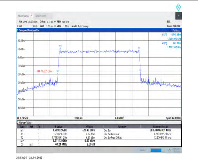
1-N66-PC3-15-40-L-9-CP-256QAM-Outer_Full-216@0-Ant1-38.633-40.240-≤40-PASS
