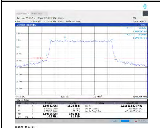
1-N70--15-10-L-8-CP-64QAM-Outer_Full-52@0-Ant1-9.312-10.300-≤10-PASS
