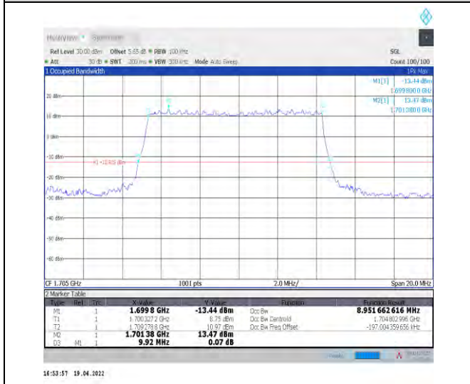
1-N70--15-10-H-2-DFT-PI2BPSK-Outer_Full-50@0-Ant Ant1-8.952-9.920-≤10-PASS
