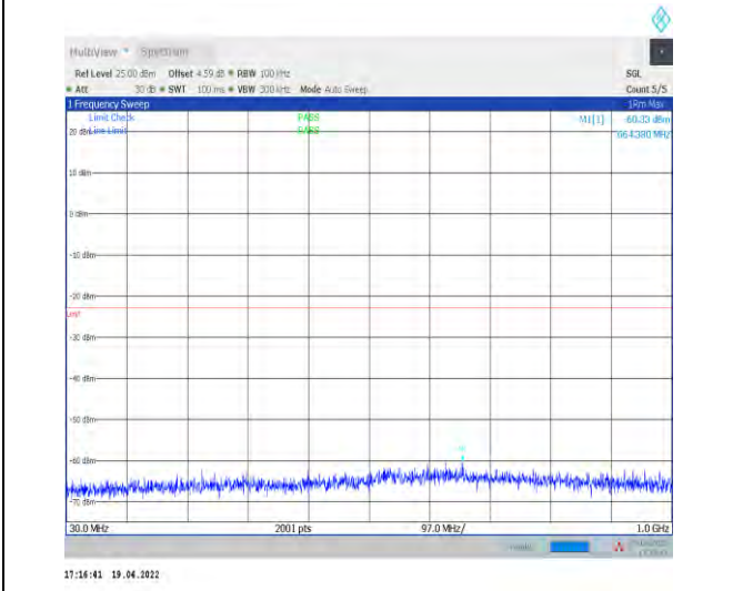
1-N70--15-15-M-1-DFT-PI2BPSK-Inner_1RB_Left-1 @1-30-1000-Ant1--60.33--23-PASS
