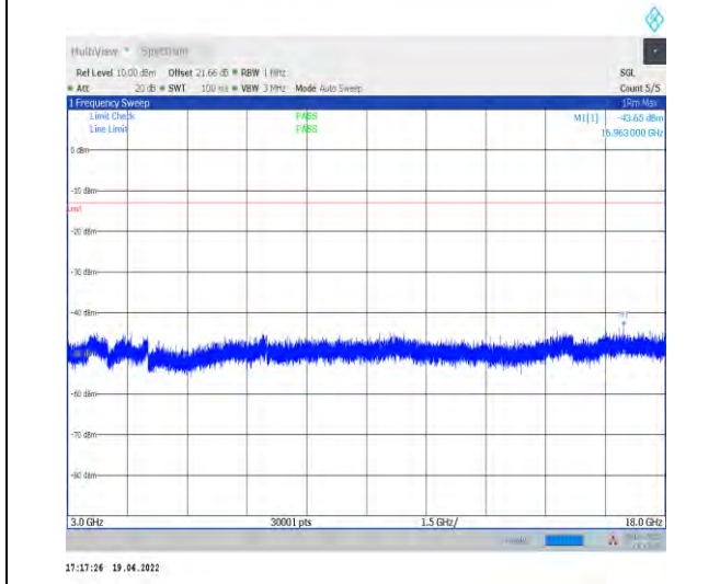
1-N70--15-15-H-1-DFT-PI2BPSK-Inner_1RB_Left-1 @1-3000-18000-Ant1--43.65--13-PASS
