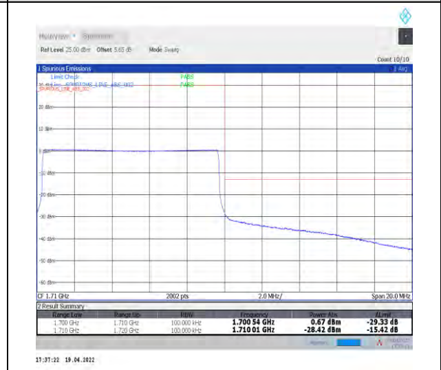
1-N70--15-10-H-6-CP-QPSK-Outer_Full-52@0-Ant1-seegraph-PASS-see graph
