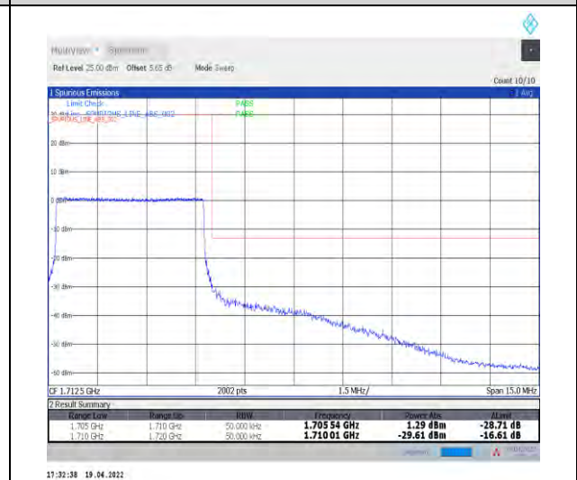
1-N70--15-5-H-6-CP-QPSK-Outer_Full-25@0-Ant1-seegraph-PASS-see graph
