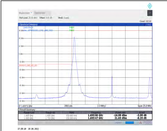
1-N70--15-15-L-1-DFT-PI2BPSK-Edge_1RB_Left-1@0-Ant1-seegraph-PASS-see graph
