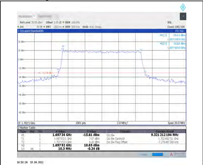
1-N70--15-10-M-6-CP-QPSK-Outer_Full-52@0-Ant1 -9.321-10.300-≤10-PASS
