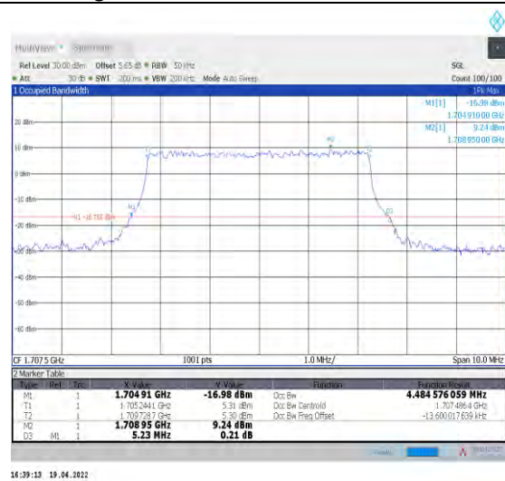
1-N70--15-5-H-8-CP-64QAM-Outer_Full-25@0-Ant1 -4.485-5.230-≤5-PASS
