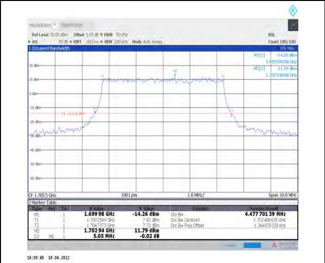
1-N70--15-5-M-3-DFT-16QAM-Outer_Full-25@0-Ant1 -4.478-5.050-≤5-PASS
