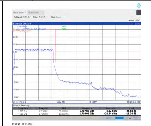
1-N70--15-5-H-3-DFT-PI2BPSK-Outer_Full-25@0-Ant1-seegraph-PASS-see graph
