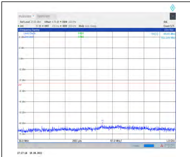
1-N70--15-15-H-1-DFT-PI2BPSK-Inner_1RB_Left-1 @1-30-1000-Ant1--60.82--23-PASS
