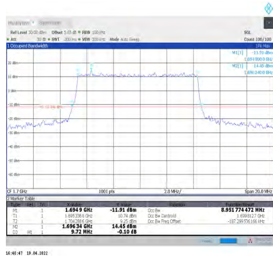
1-N70--15-10-L-1-DFT-QPSK-Outer_Full-50@0-Ant1 -8.952-9.720-≤10-PASS
