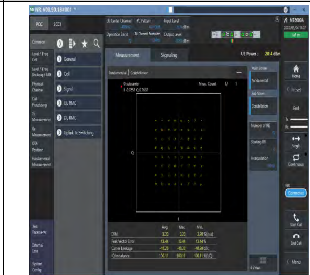
1-N70-PC3-15-15-M-8-CP-64QAM-Outer_Full-79@0-Ant1-see graph-PASS
