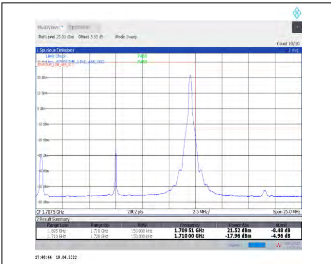
1-N70--15-15-H-2-DFT-PI2BPSK-Edge_1RB_Right-1@78-Ant1-seegraph-PASS-see graph
