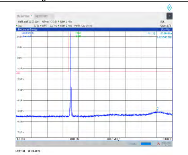
1-N70--15-15-H-1-DFT-PI2BPSK-Inner_1RB_Left-1 @1-1000-3000-Ant1--50.10--13-PASS
