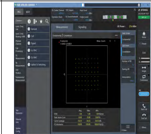
1-N70-PC3-15-15-M-4-DFT-64QAM-Outer_Full-75 @0-Ant1-see graph-PASS
