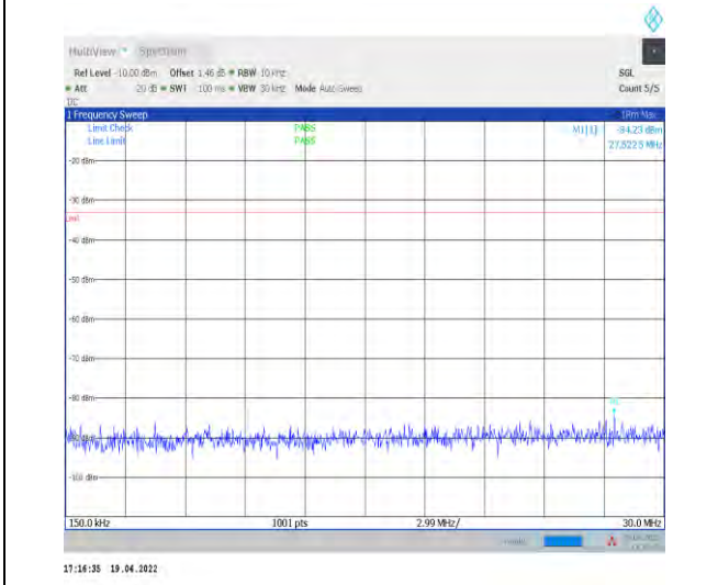
1-N70--15-15-M-1-DFT-PI2BPSK-Inner_1RB_Left-1 @1-0.15-30-Ant1--84.23--33-PASS
