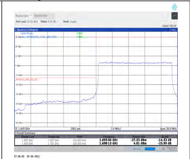
1-N70--15-10-L-3-DFT-PI2BPSK-Outer_Full-50@0-Ant1-seegraph-PASS-see graph
