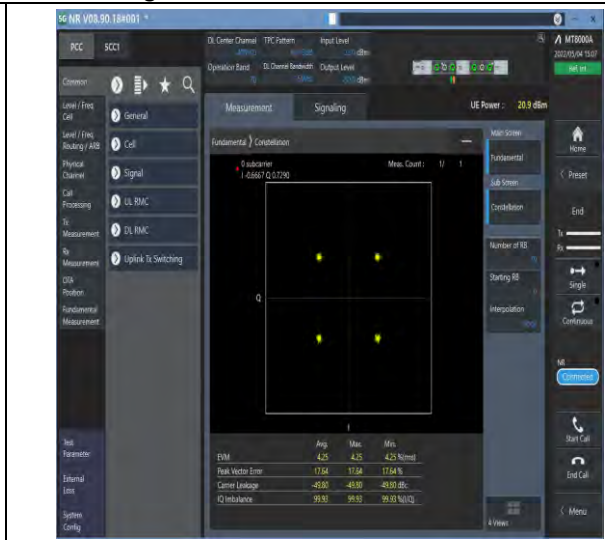
1-N70-PC3-15-15-M-6-CP-QPSK-Outer_Full-79@0-Ant1-see graph-PASS
