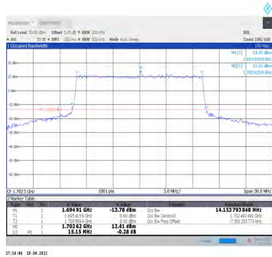
1-N70--15-15-H-8-CP-64QAM-Outer_Full-79@0-Ant 1-14.154-15.150-≤15-PASS
