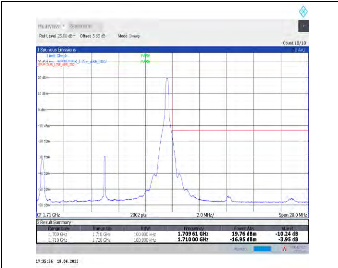
1-N70--15-10-H-2-DFT-PI2BPSK-Edge_1RB_Right-1@51-Ant1-seegraph-PASS-see graph
