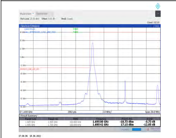
1-N70--15-10-L-4-CP-QPSK-Edge_1RB_Left-1@0-Ant1-seegraph-PASS-see graph
