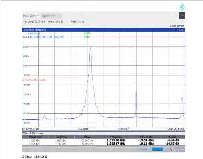
1-N70--15-15-L-4-CP-QPSK-Edge_1RB_Left-1@0-Ant1-seegraph-PASS-see graph
