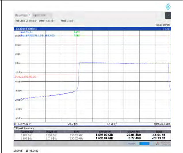
1-N70--15-15-L-6-CP-QPSK-Outer_Full-79@0-Ant1-seegraph-PASS-see graph
