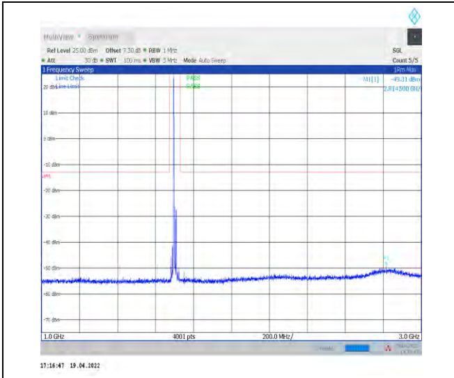
1-N70--15-15-M-1-DFT-PI2BPSK-Inner_1RB_Left-1 @1-1000-3000-Ant1--49.31--13-PASS
