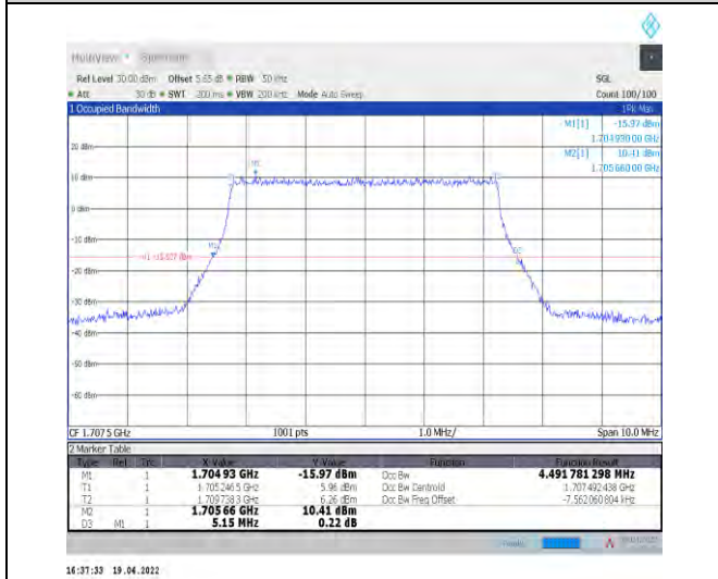
1-N70--15-5-H-5-DFT-256QAM-Outer_Full-25@0-Ant t1-4.492-5.150-≤5-PASS
