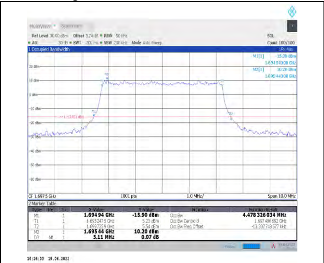
1-N70--15-5-L-6-CP-QPSK-Outer_Full-25@0-Ant1-4 .478-5.110-≤5-PASS
