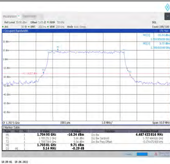
1-N70--15-5-H-7-CP-16QAM-Outer_Full-25@0-Ant1 4.487-5.140-≤5-PASS
