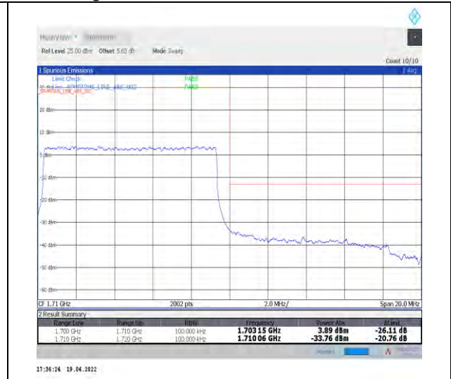
1-N70--15-10-H-3-DFT-PI2BPSK-Outer_Full-50@0-Ant1-seegraph-PASS-see graph
