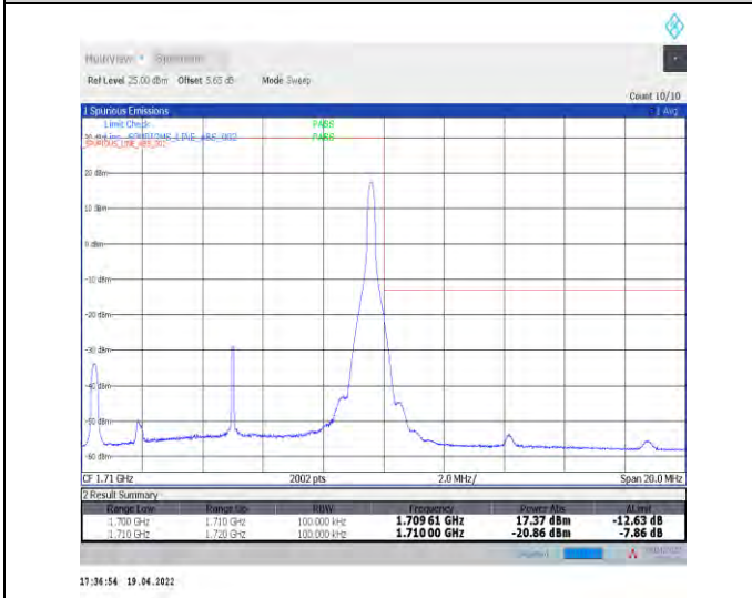
1-N70--15-10-H-5-CP-QPSK-Edge_1RB_Right-1@51-Ant1-seegraph-PASS-see graph
