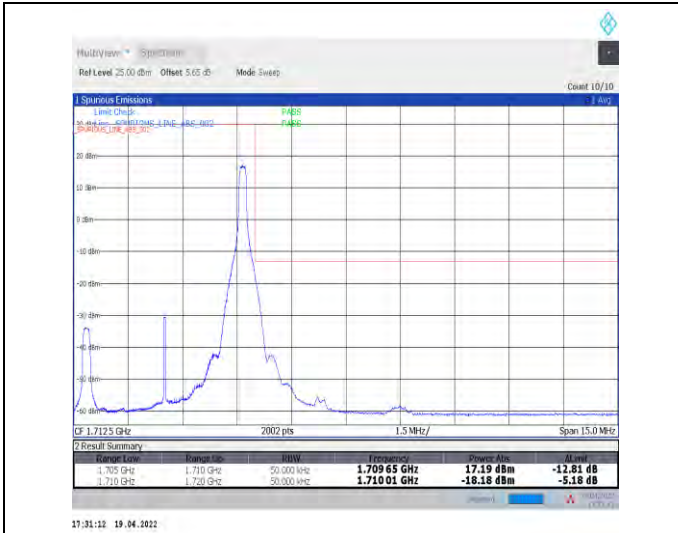
1-N70--15-5-H-2-DFT-PI2BPSK-Edge_1RB_Right-1@24-Ant1-seegraph-PASS-see graph
