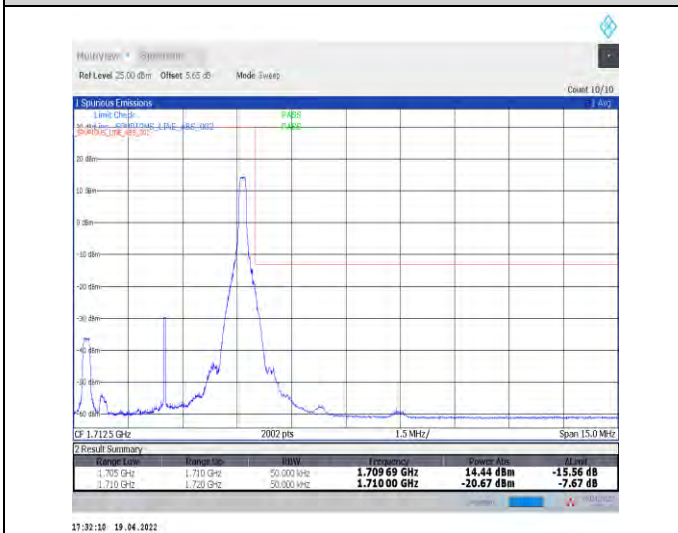
1-N70--15-5-H-5-CP-QPSK-Edge_1RB_Right-1@24-Ant1-seegraph-PASS-see graph
