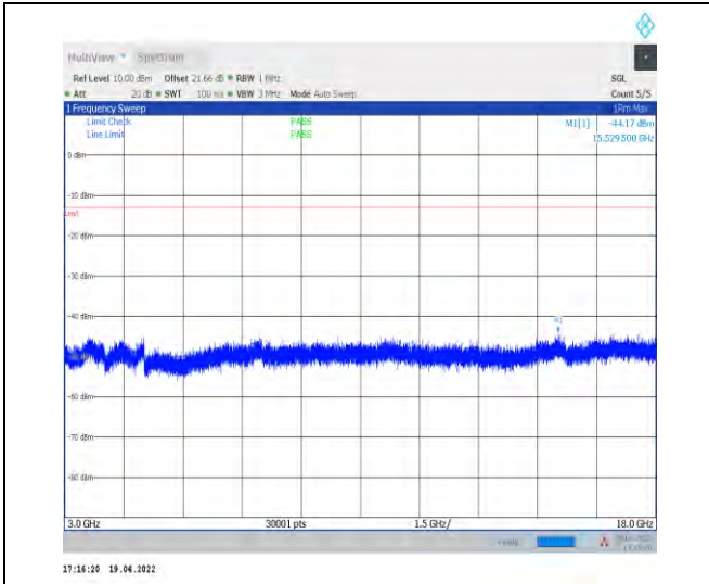
1-N70--15-15-L-1-DFT-PI2BPSK-Inner_1RB_Left-1 @1-3000-18000-Ant1--44.17--13-PASS
