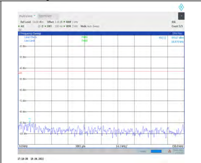
1-N70--15-15-M-1-DFT-PI2BPSK-Inner_1RB_Left-1 @1-0.009-0.15-Ant1--89.67--43-PASS
