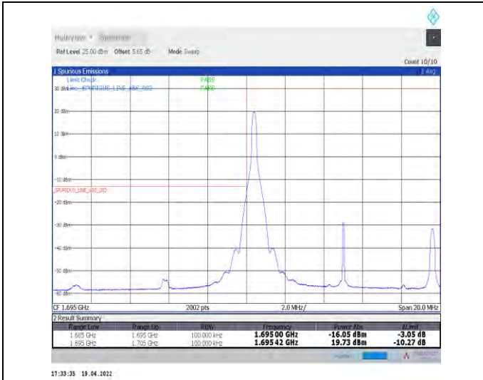
1-N70--15-10-L-1-DFT-PI2BPSK-Edge_1RB_Left-1@0-Ant1-seegraph-PASS-see graph
