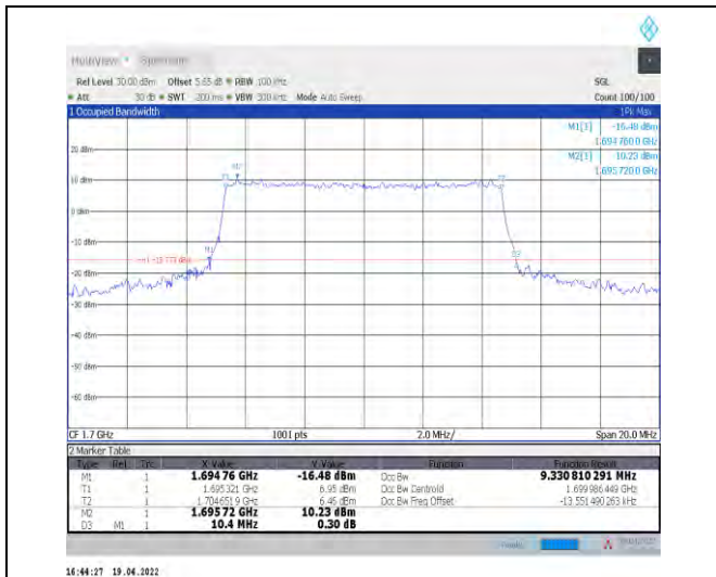
1-N70--15-10-L-6-CP-QPSK-Outer_Full-52@0-Ant1-9.331-10.400-≤10-PASS
