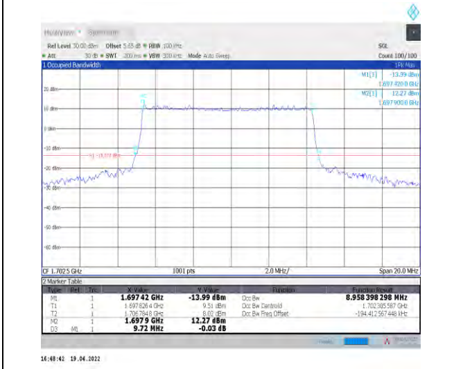
1-N70--15-10-M-3-DFT-16QAM-Outer_Full-50@0-Ant t1-8.958-9.720-≤10-PASS
