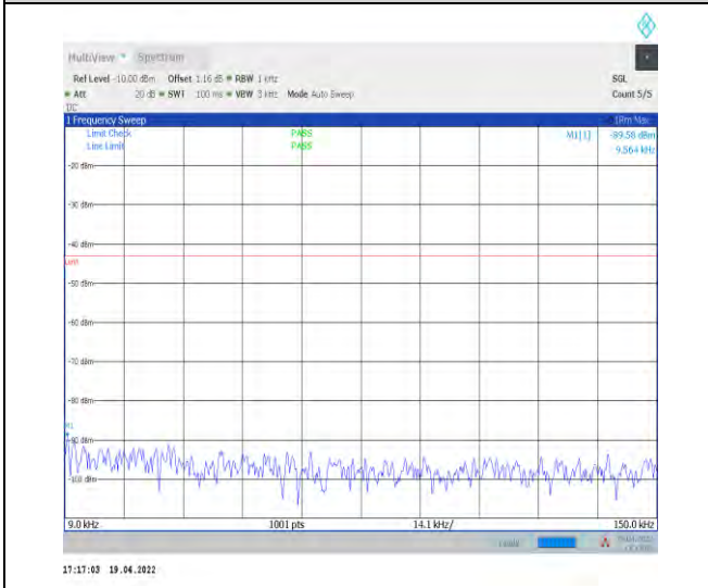
1-N70--15-15-H-1-DFT-PI2BPSK-Inner_1RB_Left-1 @1-0.009-0.15-Ant1--89.58--43-PASS
