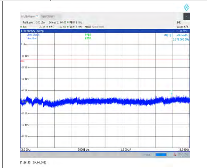
1-N70--15-15-M-1-DFT-PI2BPSK-Inner_1RB_Left-1 @1-3000-18000-Ant1--43.64--13-PASS
