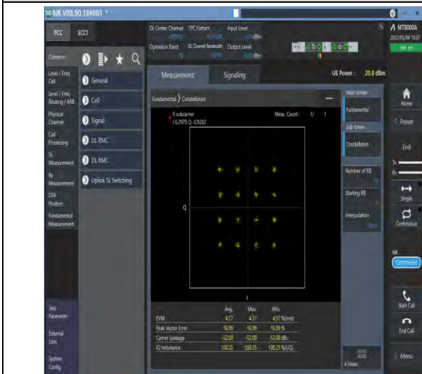
1-N70-PC3-15-15-M-7-CP-16QAM-Outer_Full-79@0-Ant1-see graph-PASS
