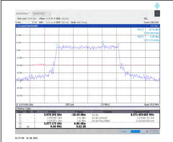
1-N77-3700-3980--30-10-H-9-CP-256QAM-Outer_F ull-24@0-Ant1-8.571-9.460-≤10-PASS
