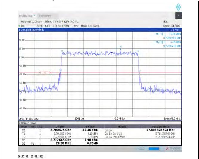
1-N77-3700-3980--30-30-L-9-CP-256QAM-Outer_Ful I-78@0-Ant1-27.852-28.980-<30-PASS
