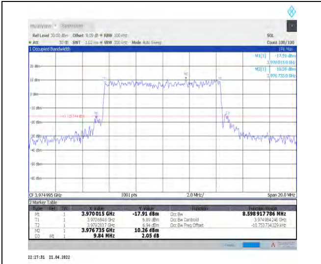
1-N77-3700-3980--30-10-H-7-CP-16QAM-Outer_Full -24@0-Ant1-8.599-9.840-≤10-PASS
