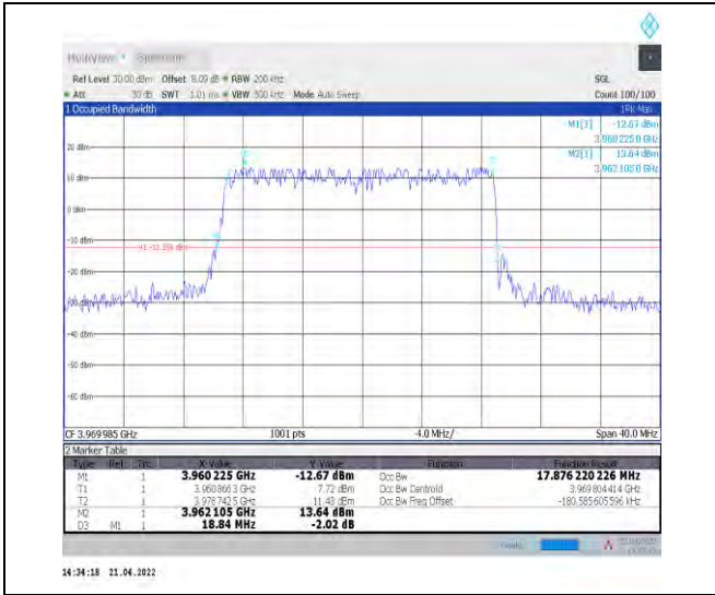
1-N77-3700-3980--30-20-H-1-DFT-QPSK-Outer_Full -50@0-Ant1-17.876-18.840-≤20-PASS
