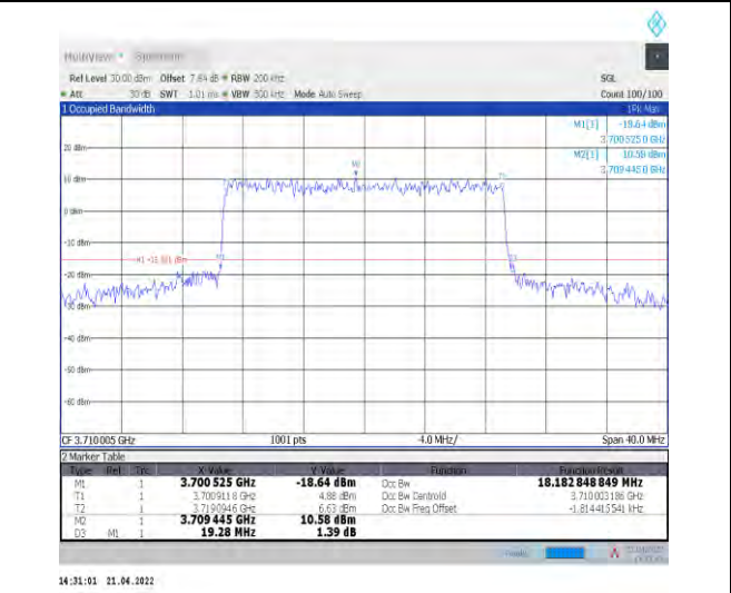
1-N77-3700-3980--30-20-L-6-CP-QPSK-Outer_Full-5 @0-Ant1-18.183-19.280-≤20-PASS
