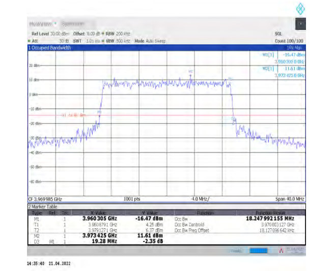
1-N77-3700-3980--30-20-H-8-CP-64QAM-Outer_Full-51@0-Ant1-18.248-19.280-<=20-PASS
