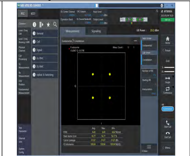
1-N77-3700-3980-PC2-30-100-M-6-CP-QPSK-Outer_Full-273@0-Ant1-see graph-PASS
