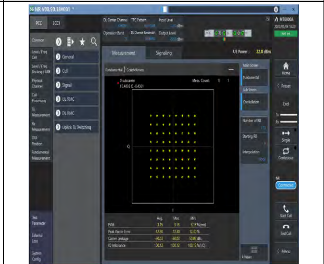
1-N77-3700-3980-PC2-30-100-M-8-CP-64QAM-Outer_Full-273@0-Ant1-see graph-PASS
