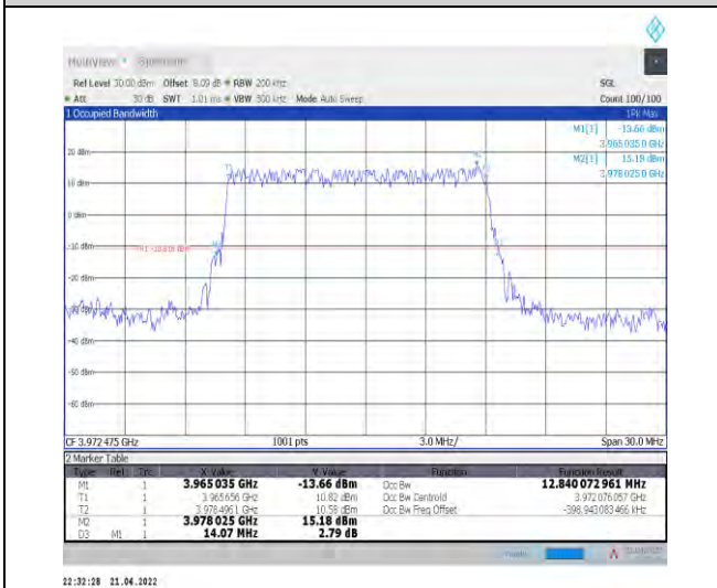
1-N77-3700-3980--30-15-H-2-DFT-PI2BPSK-Outer_Full-36@0-Ant1-12.84-14.070-≤15-PASS
