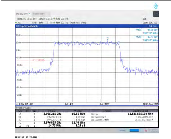
1-N77-3700-3980--30-15-H-6-CP-QPSK-Outer_Full-38@0-Ant1-13.532-14.730-≤15-PASS
