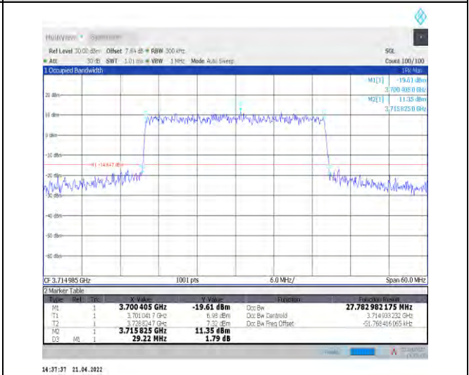
1-N77-3700-3980--30-30-L-7-CP-16QAM-Outer_Full-78@0-Ant1-27.782-29.220-≤30-PASS
