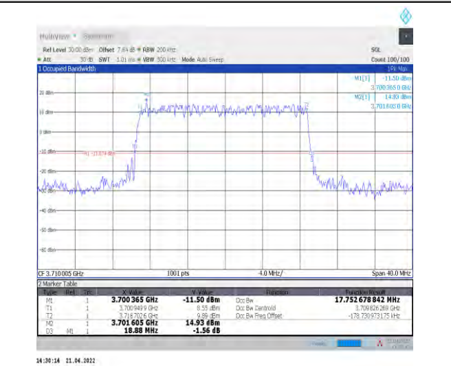
1-N77-3700-3980--30-20-L-2-DFT-PI2BPSK-Outer_Full ull-50@0-Ant1-17.753-18.880-≤20-PASS
