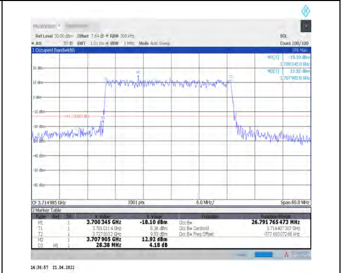
1-N77-3700-3980--30-30-L-3-DFT-16QAM-Outer_Full-75@0-Ant1-26.795-28.380-≤30-PASS
