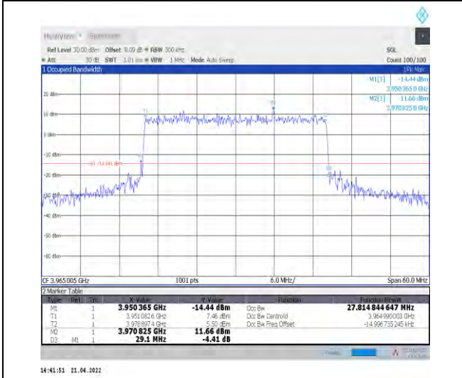
1-N77-3700-3980--30-30-H-8-CP-64QAM-Outer_Full-78@0-Ant1-27.794-29.100-≤30-PASS
