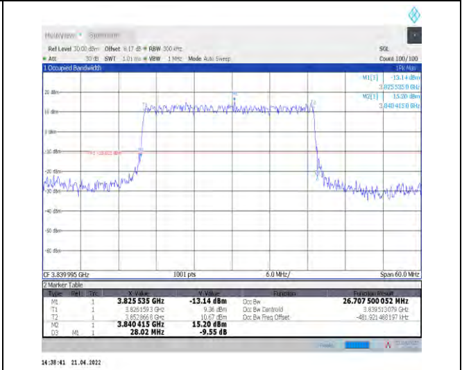
1-N77-3700-3980--30-30-M-2-DFT-PI2BPSK-Outer_Full Full-75@0-Ant1-26.71-28.020-<30-PASS
