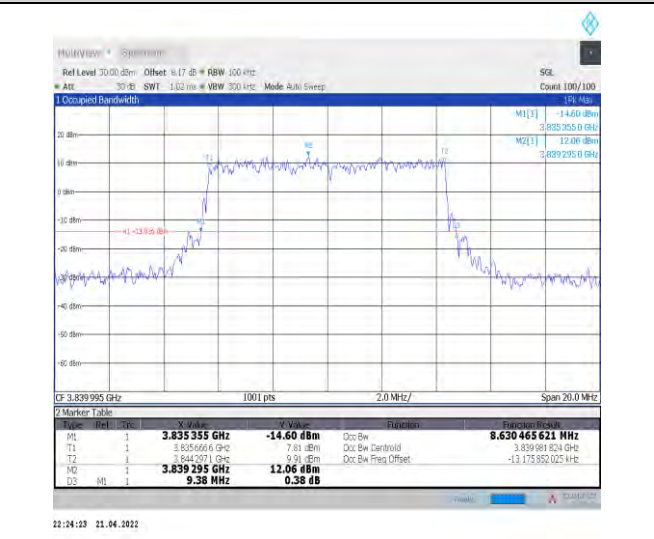
1-N77-3700-3980--30-10-M-3-DFT-16QAM-Outer_Fu Il-24@0-Ant1-8.63-9.380-≤10-PASS
