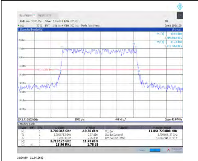
1-N77-3700-3980--30-20-L-5-DFT-256QAM-Outer_F ull-50@0-Ant1-17.852-18.960-≤20-PASS
