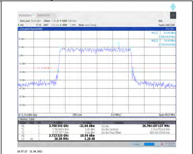
1-N77-3700-3980--30-30-L-5-DFT-256QAM-Outer_F ull-75@0-Ant1-26.784-28.380-≤30-PASS
