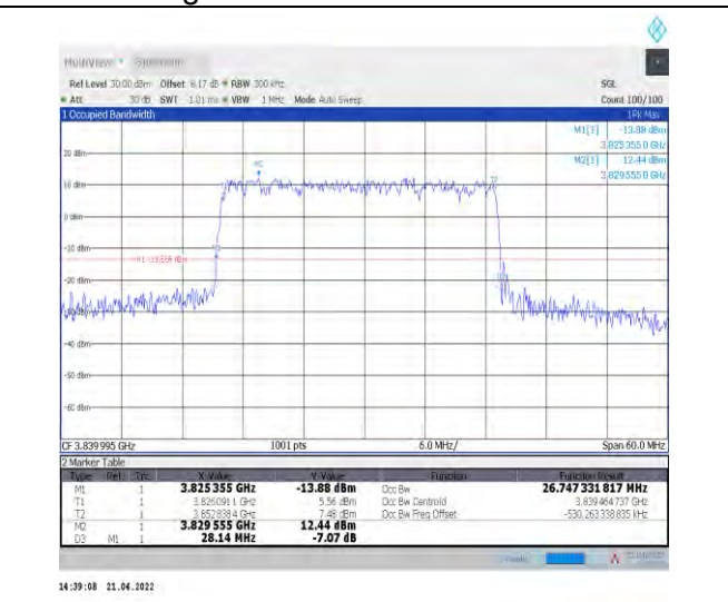
1-N77-3700-3980--30-30-M-4-DFT-64QAM-Outer_Full-75@0-Ant1-26.747-28.140-≤30-PASS
