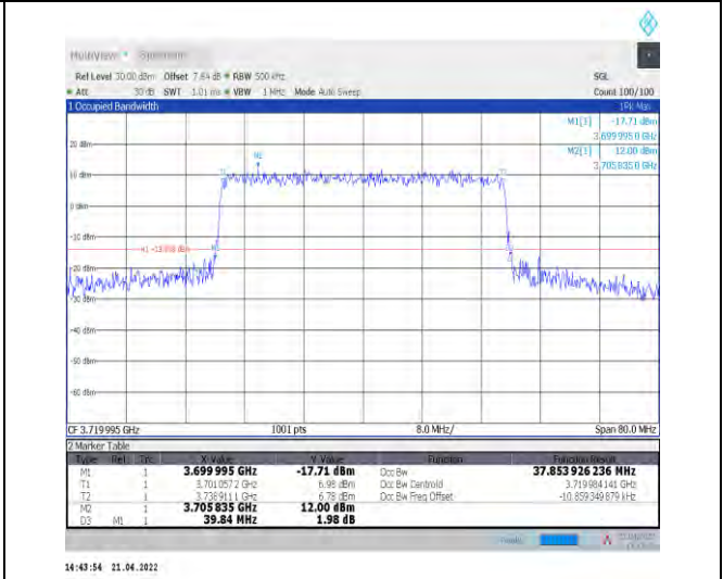
1-N77-3700-3980--30-40-L-8-CP-64QAM-Outer_Full-106@0-Ant1-37.849-39.840-<math>\leq 40</math>-PASS
