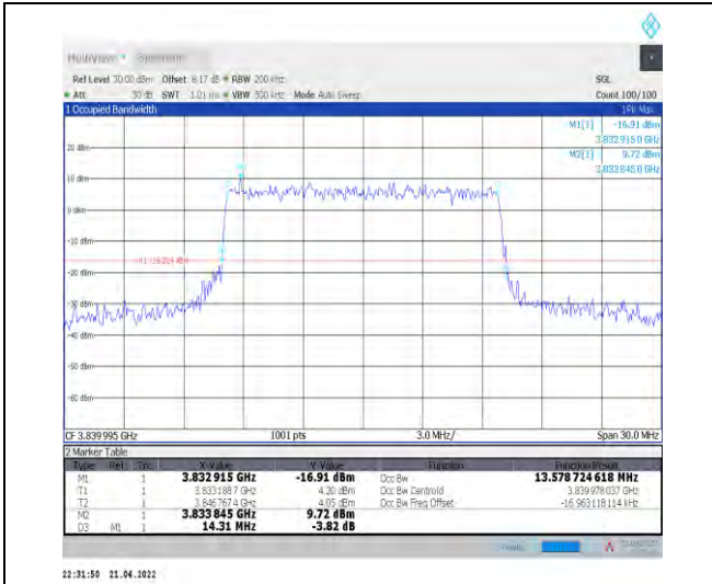
1-N77-3700-3980--30-15-M-9-CP-256QAM-Outer_Full-38@0-Ant1-13.579-14.310-≤15-PASS
