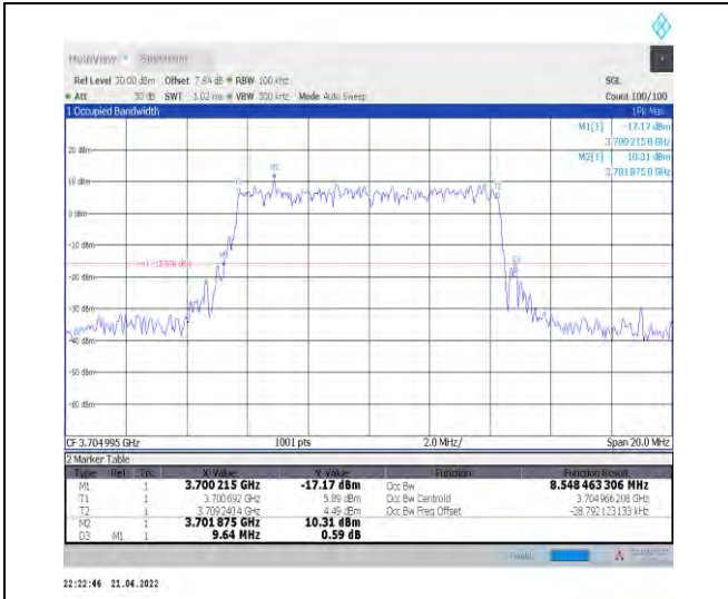
1-N77-3700-3980--30-10-L-5-DFT-256QAM-Outer_Full-24@0-Ant1-8.548-9.640-≤10-PASS
