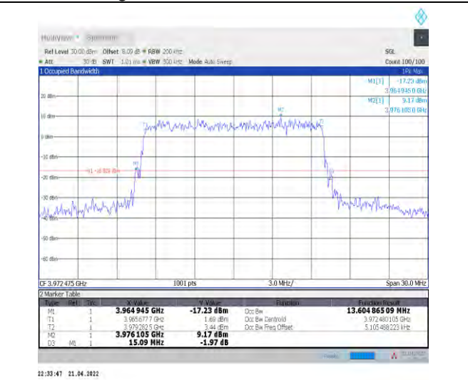
1-N77-3700-3980--30-15-H-9-CP-256QAM-Outer_Fu II-38@0-Ant1-13.605-15.090-≤15-PASS
