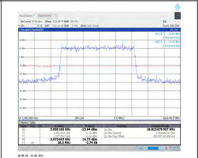
1-N77-3700-3980--30-30-H-1-DFT-QPSK-Outer_Full -75@0-Ant1-26.826-28.500-<30-PASS
