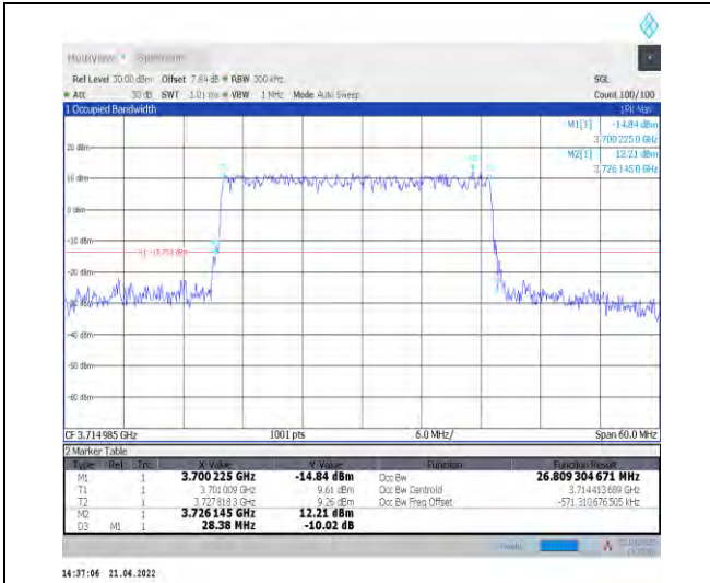
1-N77-3700-3980--30-30-L-4-DFT-64QAM-Outer_Fu ll-75@0-Ant1-26.809-28.380-≤30-PASS
