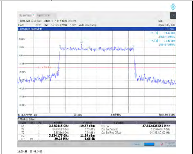
1-N77-3700-3980--30-30-M-8-CP-64QAM-Outer_Full -78@0-Ant1-27.843-29.280-<30-PASS
