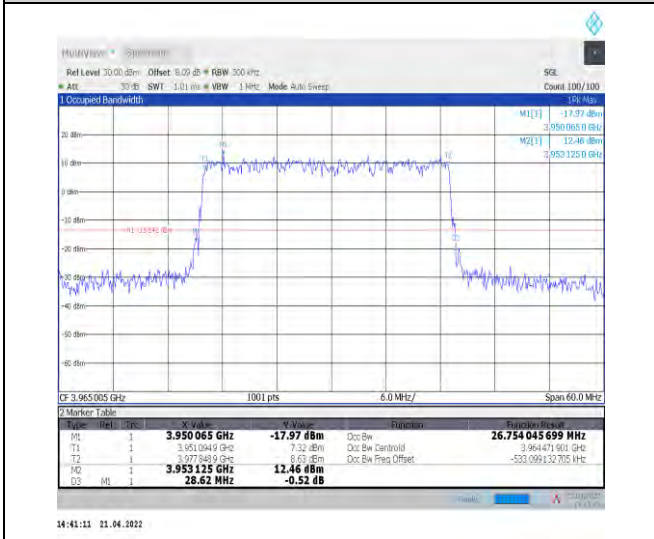
1-N77-3700-3980--30-30-H-4-DFT-64QAM-Outer_Full-75@0-Ant1-26.756-28.620-<=30-PASS
