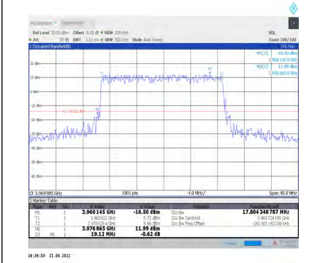
1-N77-3700-3980--30-20-H-3-DFT-16QAM-Outer_Full Full-50@0-Ant1-17.804-19.120-≤20-PASS
