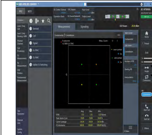
1-N77-3700-3980-PC2-30-100-M-1-DFT-PI2BPSK-Outer_Full-270@0-Ant1-see graph-PASS
