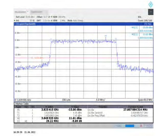
1-N77-3700-3980--30-30-M-6-CP-QPSK-Outer_Full-78@0-Ant1-27.809-29.220-≤30-PASS
