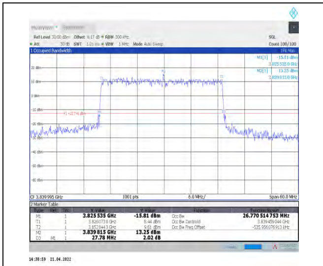
1-N77-3700-3980--30-30-M-3-DFT-16QAM-Outer_Full-75@0-Ant1-26.77-27.780-≤30-PASS
