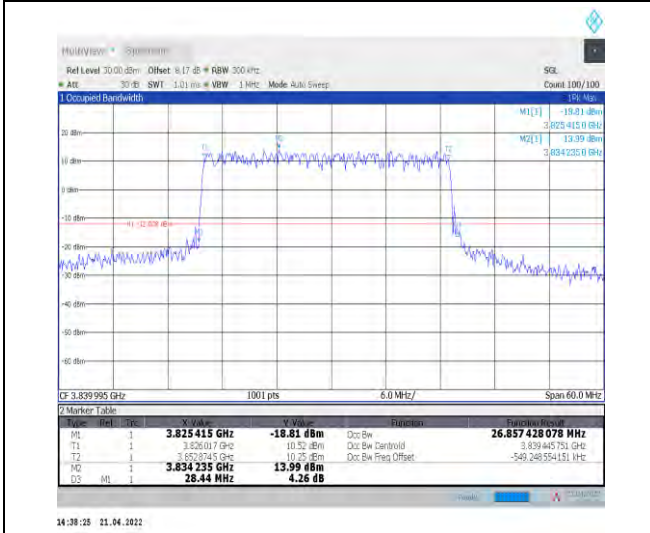
1-N77-3700-3980--30-30-M-1-DFT-QPSK-Outer_Full -75@0-Ant1-26.857-28.440-<30-PASS
