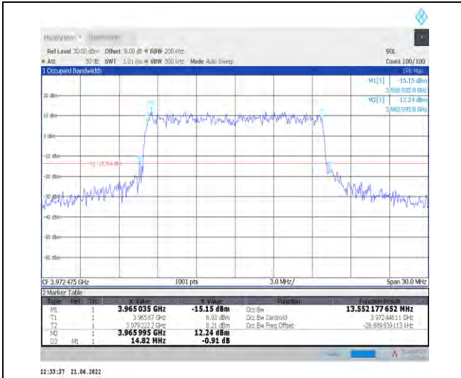
1-N77-3700-3980--30-15-H-8-CP-64QAM-Outer_Full -38@0-Ant1-13.552-14.820-≤15-PASS
