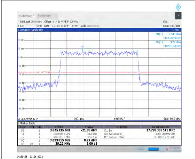
1-N77-3700-3980--30-30-M-9-CP-256QAM-Outer_Full -78@0-Ant1-27.798-29.220-<30-PASS
