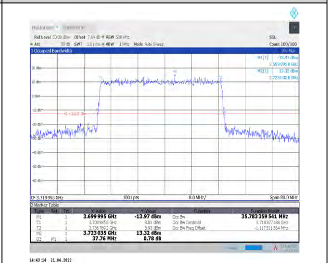
1-N77-3700-3980--30-40-L-4-DFT-64QAM-Outer_Full-100@0-Ant1-35.791-37.760-≤40-PASS
