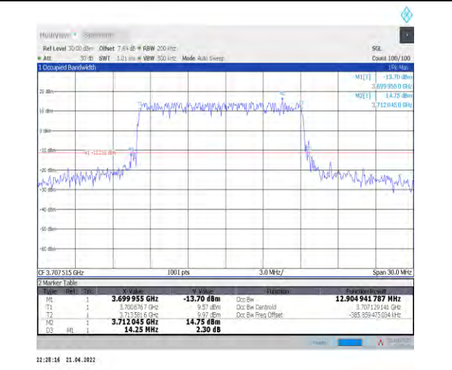
1-N77-3700-3980--30-15-L-1-DFT-QPSK-Outer_Full- 36@0-Ant1-12.905-14.250-≤15-PASS
