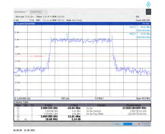
1-N77-3700-3980--30-20-H-4-DFT-64QAM-Outer_Full Full-50@0-Ant1-17.82-18.680-≤20-PASS
