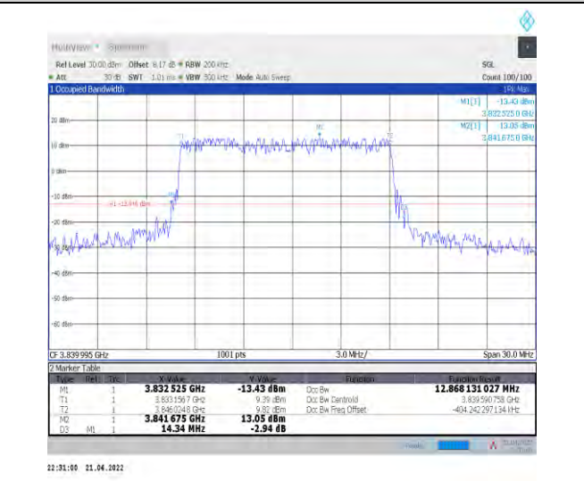
1-N77-3700-3980--30-15-M-4-DFT-64QAM-Outer_Full Full-36@0-Ant1-12.868-14.340-≤15-PASS
