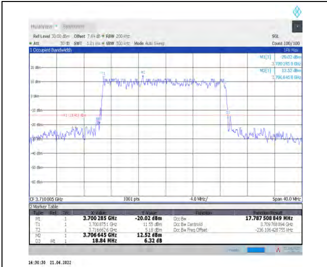
1-N77-3700-3980--30-20-L-3-DFT-16QAM-Outer_Fu ll-50@0-Ant1-17.788-18.840-≤20-PASS
