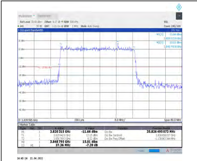
1-N77-3700-3980--30-40-M-4-DFT-64QAM-Outer_Full-100@0-Ant1-35.834-37.360-≤40-PASS
