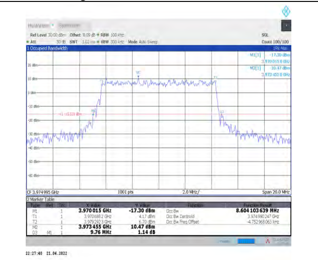
1-N77-3700-3980--30-10-H-8-CP-64QAM-Outer_Full -24@0-Ant1-8.604-9.760-≤10-PASS
