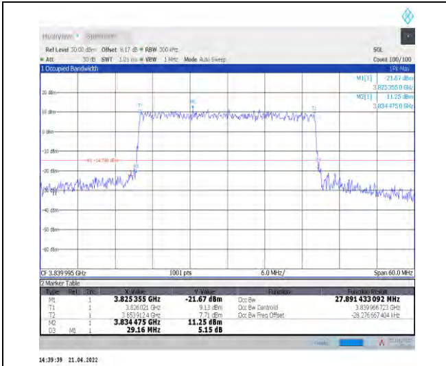
1-N77-3700-3980--30-30-M-7-CP-16QAM-Outer_Full I-78@0-Ant1-27.893-29.160-<30-PASS
