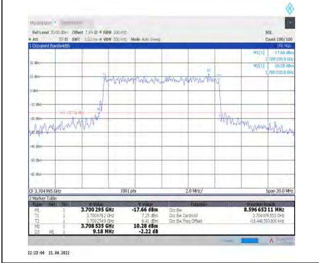
1-N77-3700-3980--30-10-L-7-CP-16QAM-Outer_Full-24@0-Ant1-8.597-9.180-≤10-PASS
