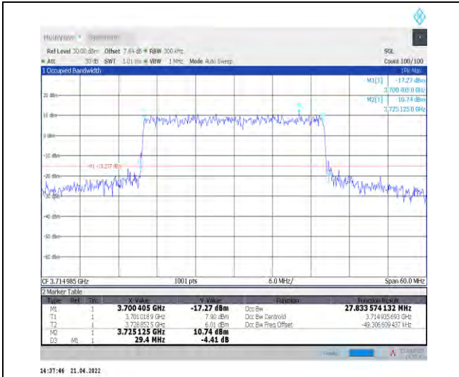
1-N77-3700-3980--30-30-L-8-CP-64QAM-Outer_Full -78@0-Ant1-27.833-29.400-<30-PASS
