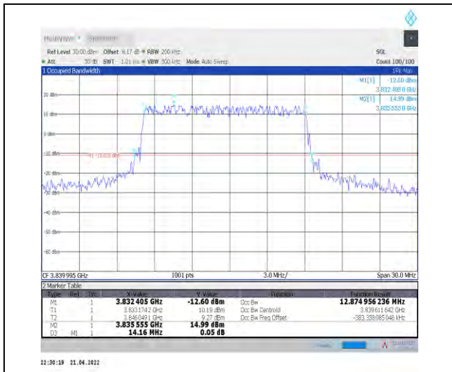
1-N77-3700-3980--30-15-M-1-DFT-QPSK-Outer_Full -36@0-Ant1-12.875-14.160-≤15-PASS
