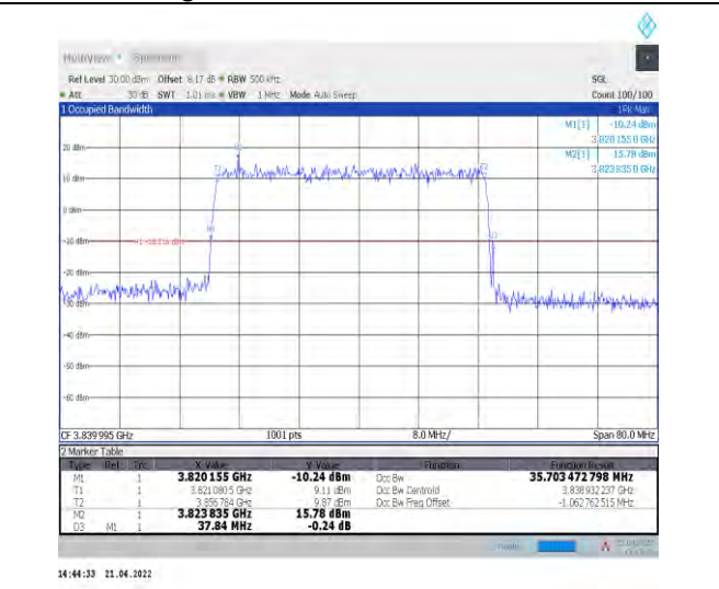
1-N77-3700-3980--30-40-M-1-DFT-QPSK-Outer_Full -100@0-Ant1-35.718-37.840-≤40-PASS
