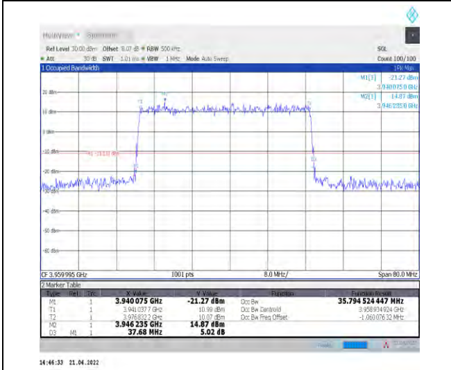
1-N77-3700-3980--30-40-H-1-DFT-QPSK-Outer_Full-I-100@0-Ant1-35.792-37.680-≤40-PASS
