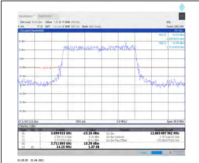
1-N77-3700-3980--30-15-L-2-DFT-PI2BPSK-Outer_Full-36@0-Ant1-12.865-14.250-≤15-PASS
