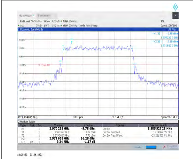
1-N77-3700-3980--30-10-H-1-DFT-QPSK-Outer_Full-24@0-Ant1-8.586-9.240-≤10-PASS
