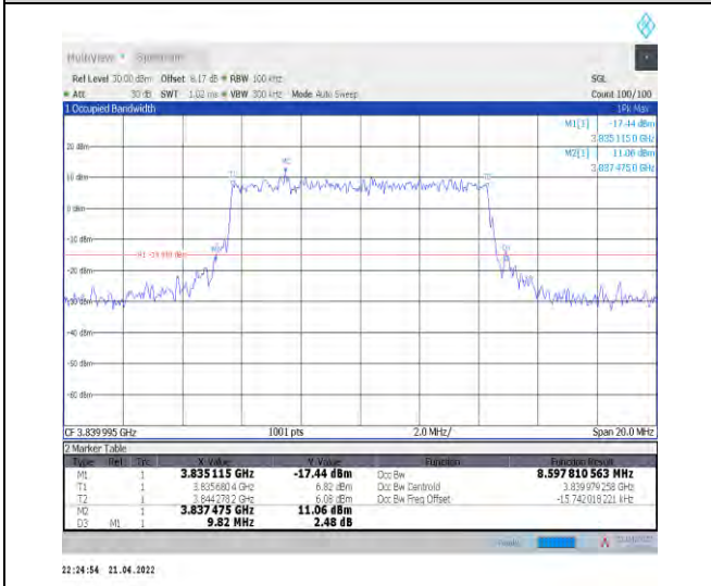
1-N77-3700-3980--30-10-M-6-CP-QPSK-Outer_Full-24@0-Ant1-8.598-9.820-≤10-PASS
