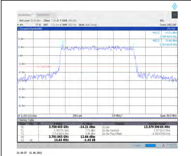
1-N77-3700-3980--30-15-L-8-CP-64QAM-Outer_Full-38@0-Ant1-13.579-14.640-≤15-PASS
