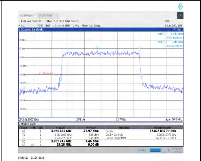
1-N77-3700-3980--30-30-H-9-CP-256QAM-Outer_Fu ll-78@0-Ant1-27.825-29.280-≤30-PASS
