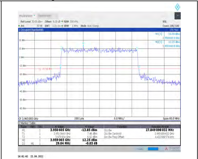
1-N77-3700-3980--30-30-H-7-CP-16QAM-Outer_Full-78@0-Ant1-27.85-29.040-≤30-PASS
