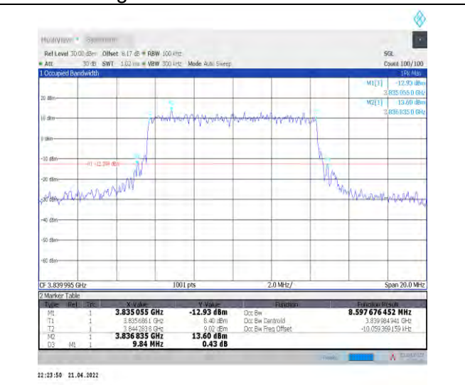
1-N77-3700-3980--30-10-M-1-DFT-QPSK-Outer_Full -24@0-Ant1-8.598-9.840-≤10-PASS
