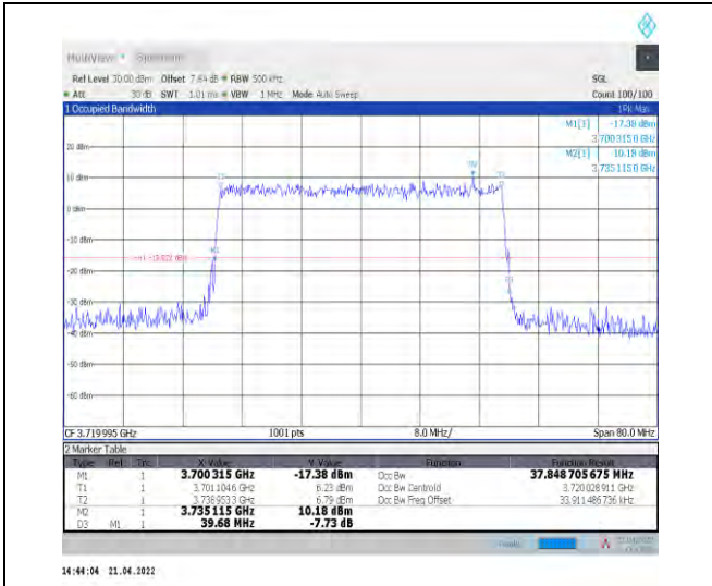
1-N77-3700-3980--30-40-L-9-CP-256QAM-Outer_Fu II-106@0-Ant1-37.853-39.680-≤40-PASS
