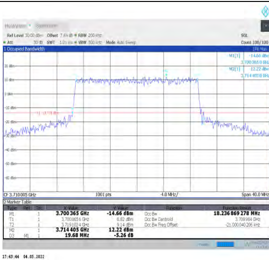
1-N78-3700-3800--30-20-L-7-CP-16QAM-Outer_Full -51@0-Ant1-18.237-19.680-≤20-PASS
