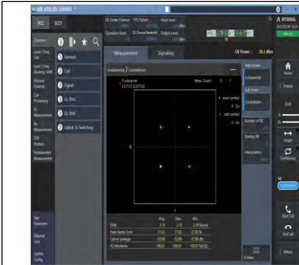
1-N78-3700-3800--30-100-M-1-DFT-PI2BPSK-Outer_F Full-270@0-Ant1-see graph-PASS
