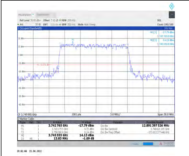
1-N78-3700-3800--30-15-M-3-DFT-16QAM-Outer_Full ull-36@0-Ant1-12.891-13.830-≤15-PASS
