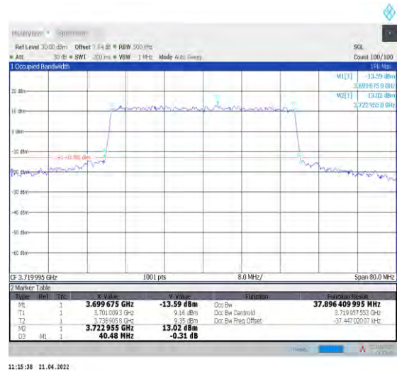
1-N78-3700-3800--30-40-L-8-CP-64QAM-Outer_Full-106@0-Ant1-37.896-40.480-≤40-PASS
