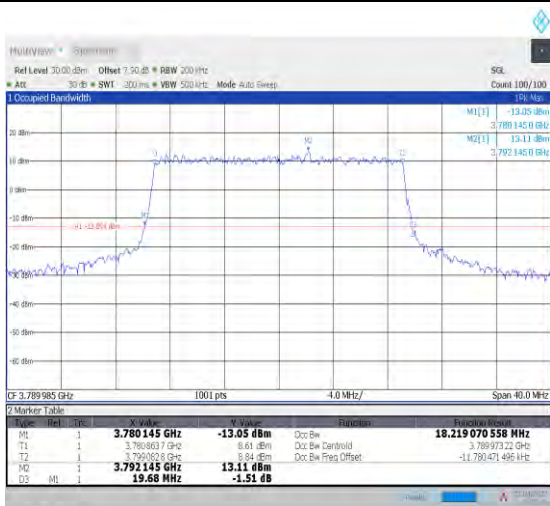
1-N78-3700-3800--30-20-H-5-DFT-256QAM-Outer_Full-50@0-Ant1-17.854-19.480-≤20-PASS
