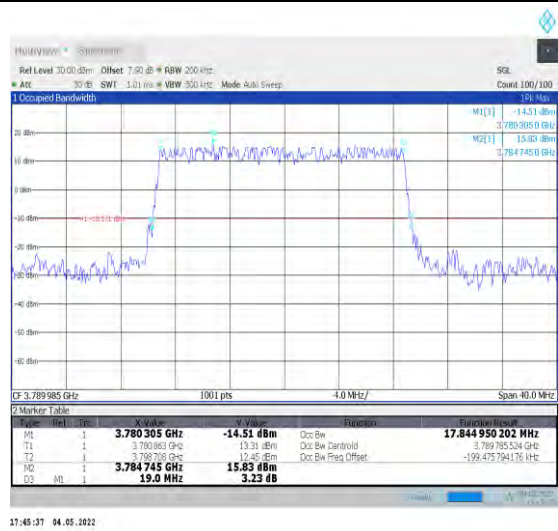
1-N78-3700-3800--30-20-H-2-DFT-PI2BPSK-Outer_Full Full-50@0-Ant1-17.845-19.000-≤20-PASS
