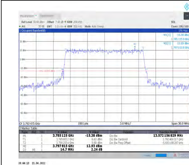
1-N78-3700-3800--30-15-H-6-CP-QPSK-Outer_Full-38@0-Ant1-13.572-14.700-≤15-PASS
