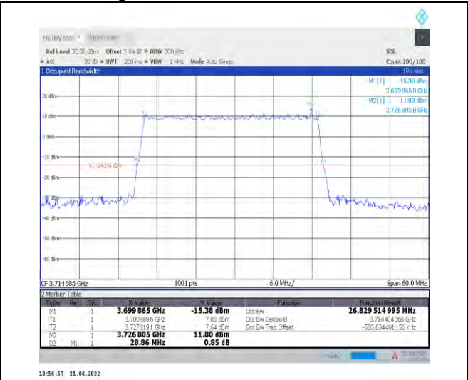
1-N78-3700-3800--30-30-L-5-DFT-256QAM-Outer_Full-75@0-Ant1-26.83-28.860-≤30-PASS
