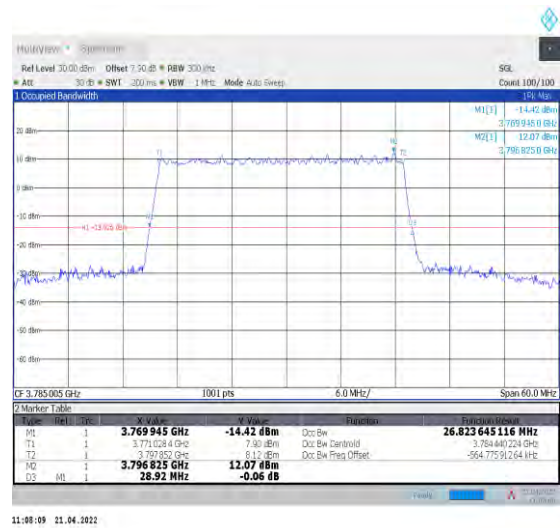
1-N78-3700-3800--30-30-H-5-DFT-256QAM-Outer_Full-75@0-Ant1-26.824-28.920-≤30-PASS
