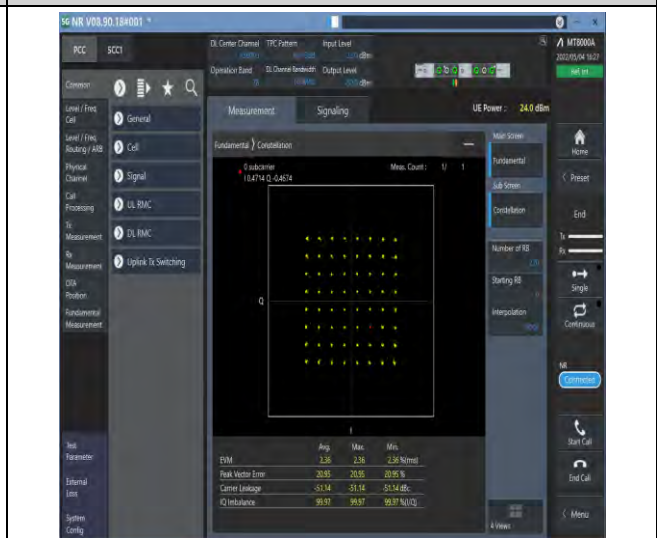
1-N78-3700-3800--30-100-M-4-DFT-64QAM-Outer_F Full-270@0-Ant1-see graph-PASS
