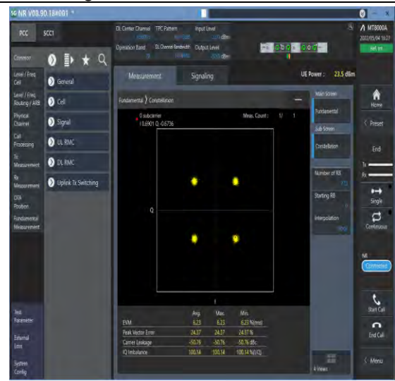
1-N78-3700-3800--30-100-M-6-CP-QPSK-Outer_Fu ll-273@0-Ant1-see graph-PASS
