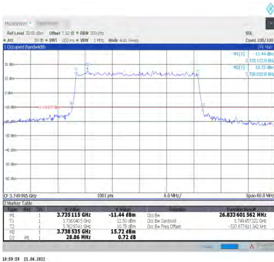
1-N78-3700-3800--30-30-M-1-DFT-QPSK-Outer_Full -75@0-Ant1-26.834-28.860-<30-PASS
