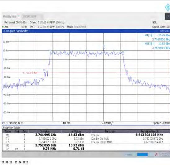
1-N78-3700-3800--30-10-M-8-CP-64QAM-Outer_Full -24@0-Ant1-8.613-9.760-≤10-PASS
