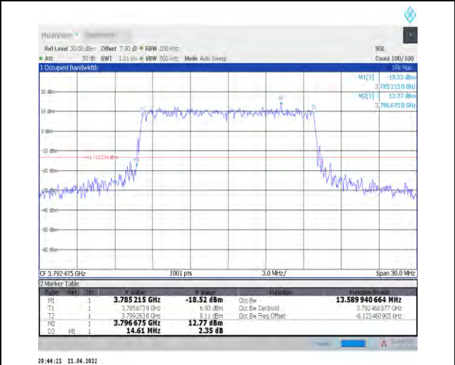
1-N78-3700-3800--30-15-H-7-CP-16QAM-Outer_Full-38@0-Ant1-13.59-14.610-≤15-PASS
