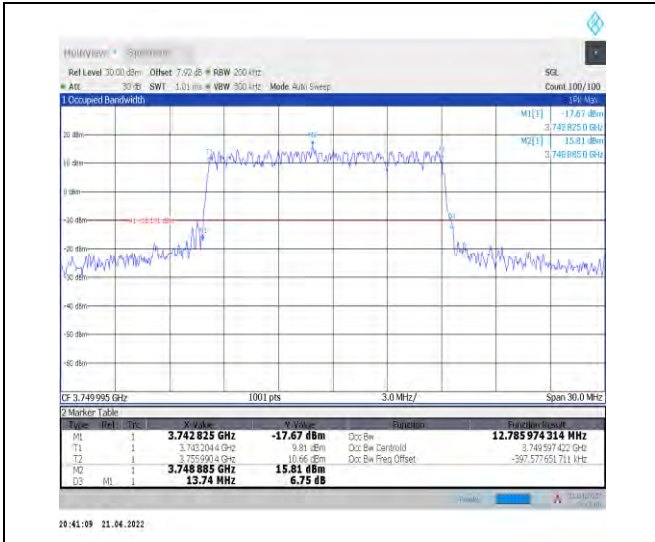
1-N78-3700-3800--30-15-M-1-DFT-QPSK-Outer_Full -36@0-Ant1-12.786-13.740-≤15-PASS
