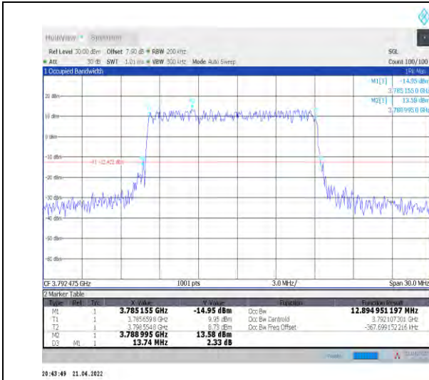
1-N78-3700-3800--30-15-H-4-DFT-64QAM-Outer_Fu II-36@0-Ant1-12.895-13.740-≤15-PASS
