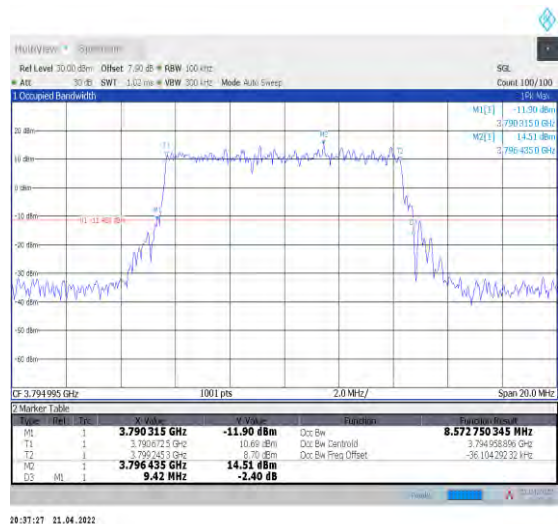
1-N78-3700-3800--30-10-H-2-DFT-PI2BPSK-Outer_ Full-24@0-Ant1-8.573-9.420-≤10-PASS
