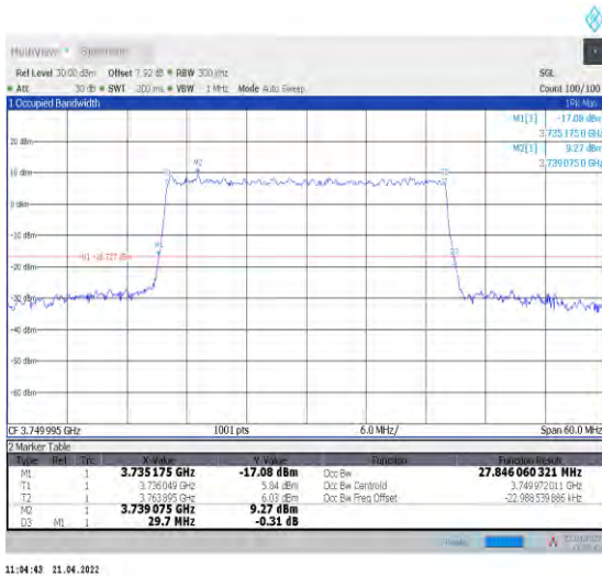
1-N78-3700-3800--30-30-M-9-CP-256QAM-Outer_F ull-78@0-Ant1-27.846-29.700-≤30-PASS
