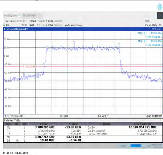
1-N78-3700-3800--30-20-L-8-CP-64QAM-Outer_Full -51@0-Ant1-18.185-19.480-≤20-PASS
