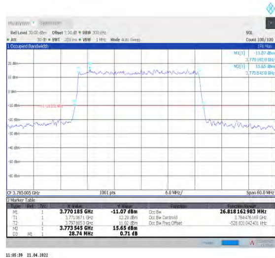
1-N78-3700-3800--30-30-H-1-DFT-QPSK-Outer_Full -75@0-Ant1-26.818-28.740-≤30-PASS
