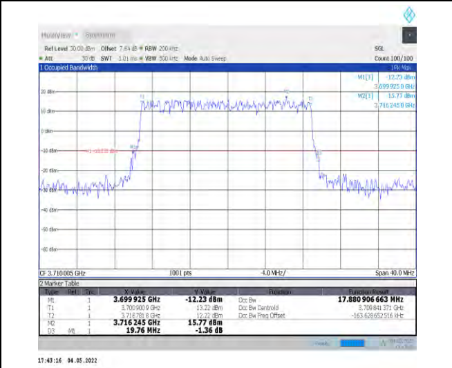
1-N78-3700-3800--30-20-L-2-DFT-PI2BPSK-Outer_Full Full-50@0-Ant1-17.881-19.760-≤20-PASS
