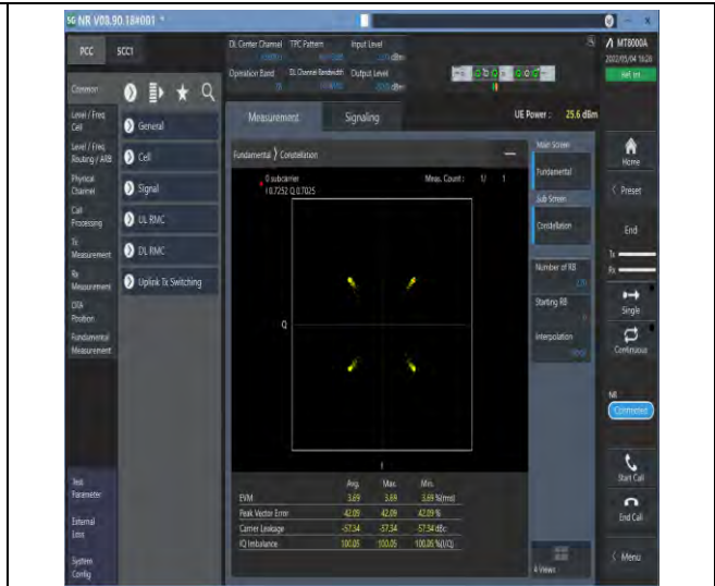
1-N78-3700-3800--30-100-M-2-DFT-QPSK-Outer_F Full-270@0-Ant1-see graph-PASS
