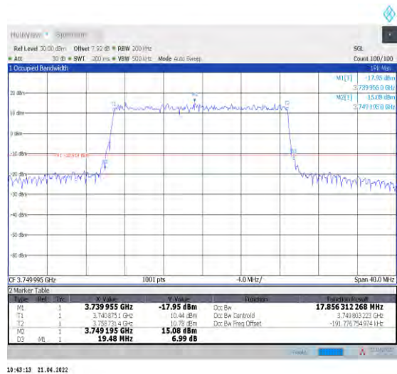
1-N78-3700-3800--30-20-M-1-DFT-QPSK-Outer_Full -50@0-Ant1-17.856-19.480-≤20-PASS
