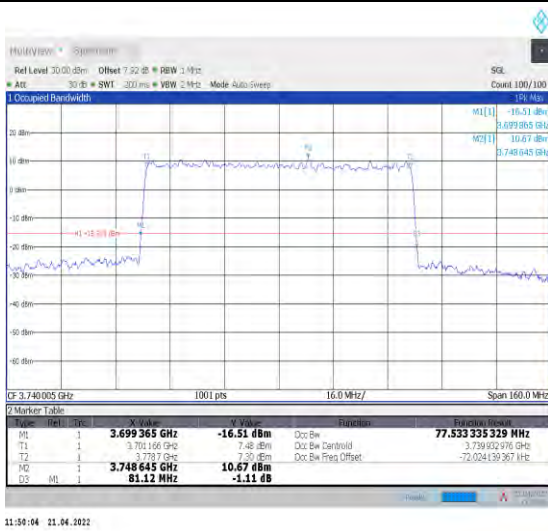
1-N78-3700-3800--30-80-L-9-CP-256QAM-Outer_Full-217@0-Ant1-77.533-81.120-≤80-PASS
