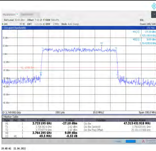
1-N78-3700-3800--30-50-M-9-CP-256QAM-Outer_Full-133@0-Ant1-47.315-49.500-≤50-PASS
