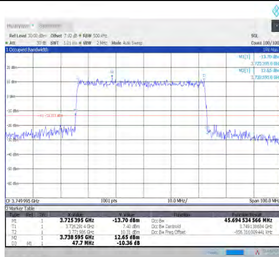
1-N78-3700-3800--30-50-M-2-DFT-PI2BPSK-Outer_Full Full-128@0-Ant1-45.704-47.400-≤50-PASS
