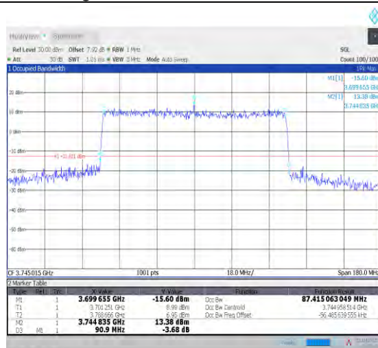
1-N78-3700-3800--30-90-L-7-CP-16QAM-Outer_Full -245@0-Ant1-87.415-90.900-<=90-PASS
