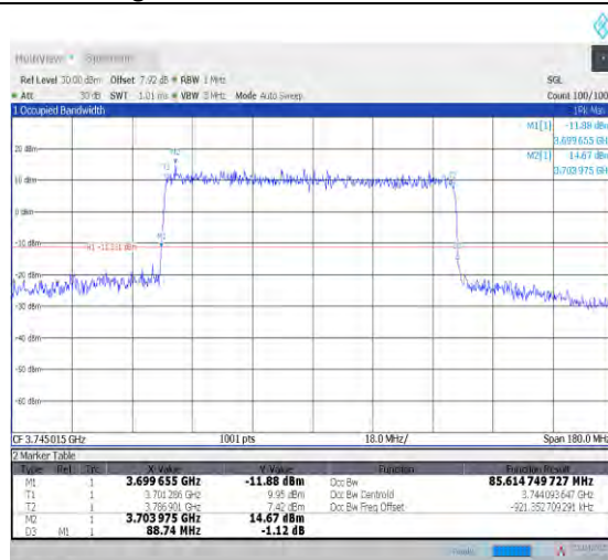
1-N78-3700-3800--30-90-L-3-DFT-16QAM-Outer_Full-240@0-Ant1-85.615-88.740-≤90-PASS
