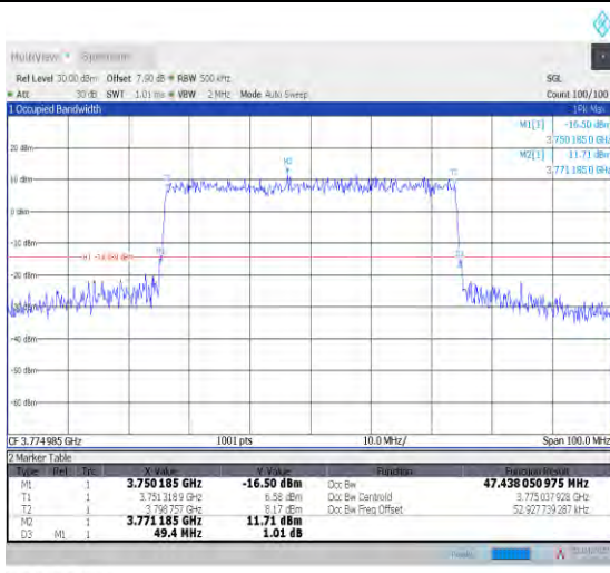
1-N78-3700-3800--30-50-H-8-CP-64QAM-Outer_Full-133@0-Ant1-47.438-49.400-≤50-PASS
