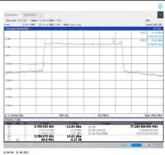
1-N78-3700-3800--30-80-M-1-DFT-QPSK-Outer_Full-216@0-Ant1-77.304-80.800-≤80-PASS
