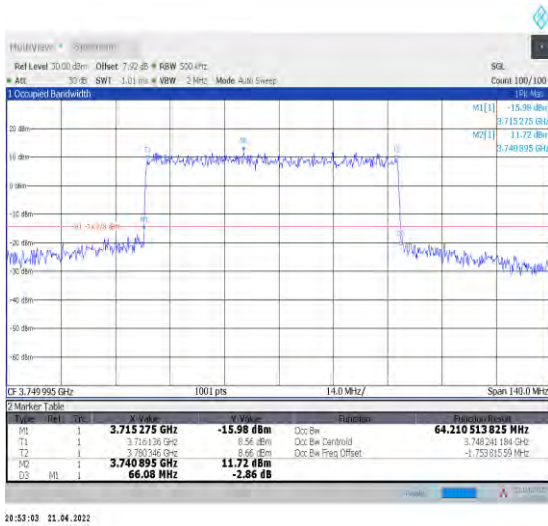
1-N78-3700-3800--30-70-M-1-DFT-QPSK-Outer_Full -180@0-Ant1-64.211-66.080-≤70-PASS
