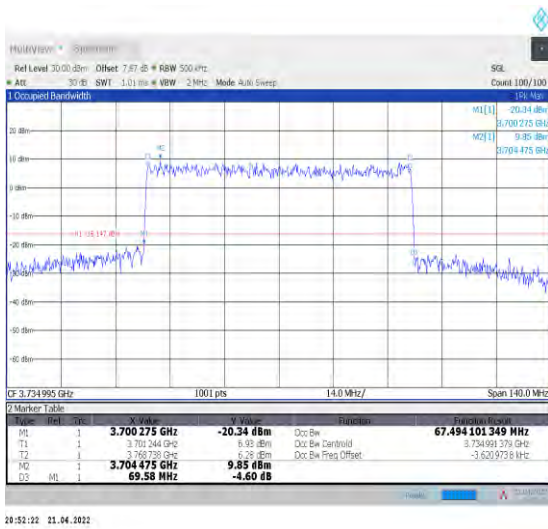
1-N78-3700-3800--30-70-L-8-CP-64QAM-Outer_Full -189@0-Ant1-67.494-69.580-≤70-PASS
