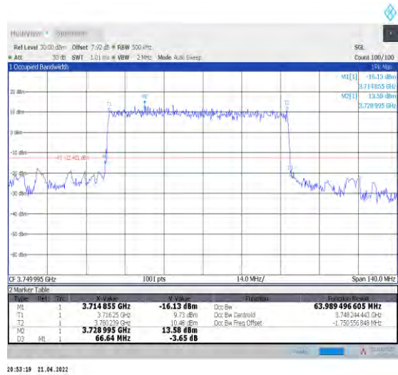
1-N78-3700-3800--30-70-M-2-DFT-PI2BPSK-Outer_Full Full-180@0-Ant1-63.989-66.640-≤70-PASS
