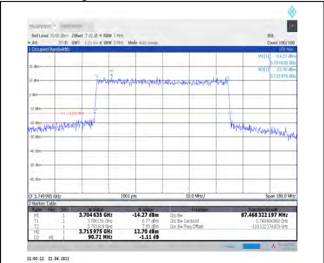
1-N78-3700-3800--30-90-M-6-CP-QPSK-Outer_Full-245@0-Ant1-87.468-90.720-≤90-PASS
