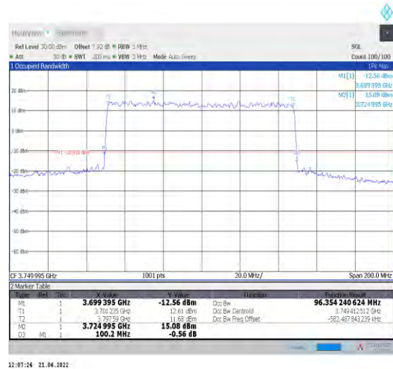
1-N78-3700-3800--30-100-M-1-DFT-QPSK-Outer_F ull-270@0-Ant1-96.354-100.200-≤100-PASS
