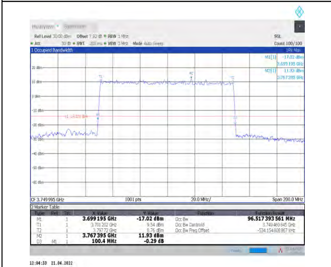
1-N78-3700-3800--30-100-L-5-DFT-256QAM-Outer_F ull-270@0-Ant1-96.517-100.400-≤100-PASS
