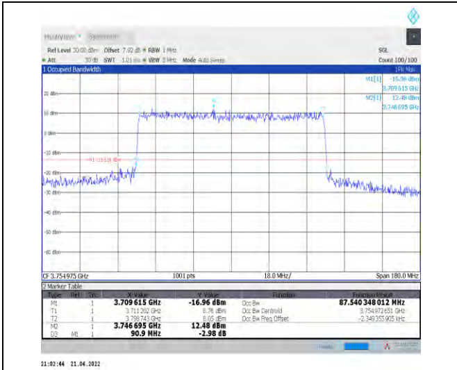
1-N78-3700-3800--30-90-H-8-CP-64QAM-Outer_Full -245@0-Ant1-87.54-90.900-≤90-PASS
