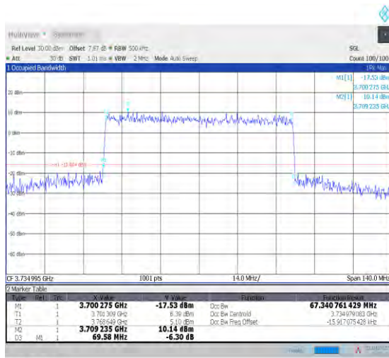
1-N78-3700-3800--30-70-L-5-DFT-256QAM-Outer_Full I-180@0-Ant1-64.107-66.640-≤70-PASS
