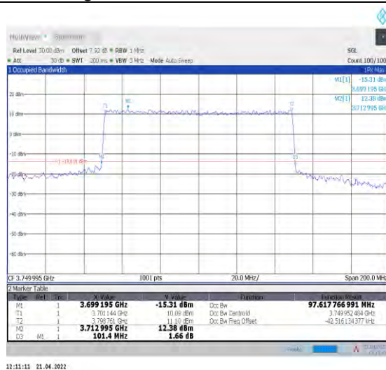
1-N78-3700-3800--30-100-M-7-CP-16QAM-Outer_Full-273@0-Ant1-97.618-101.400-≤100-PASS
