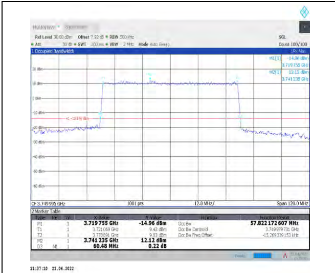
1-N78-3700-3800--30-60-M-6-CP-QPSK-Outer_Full-162@0-Ant1-57.822-60.480-<math>\leq 60</math>-PASS
