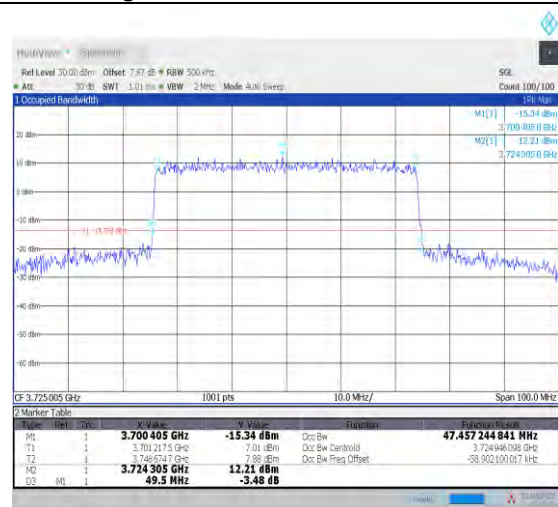
1-N78-3700-3800--30-50-L-7-CP-16QAM-Outer_Full -133@0-Ant1-47.457-49.500-≤50-PASS
