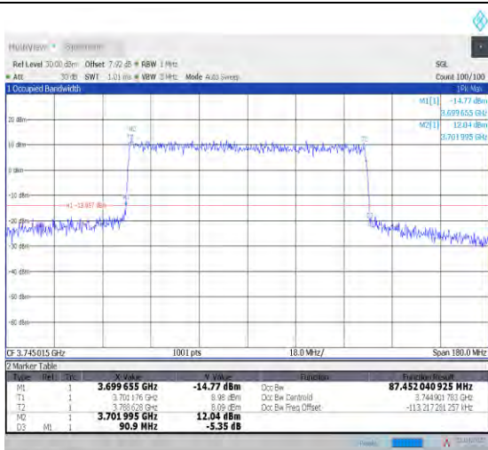
1-N78-3700-3800--30-90-L-6-CP-QPSK-Outer_Full-2 45@0-Ant1-87.452-90.900-<=90-PASS
