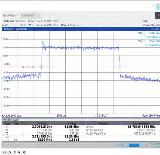
1-N78-3700-3800--30-90-H-4-DFT-64QAM-Outer_Fu II-240@0-Ant1-85.781-88.920-<=90-PASS
