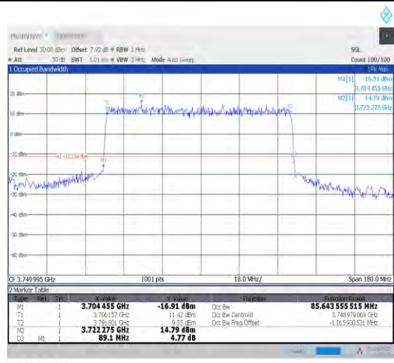
1-N78-3700-3800--30-90-M-2-DFT-PI2BPSK-Outer_Full Full-240@0-Ant1-85.644-89.100-≤90-PASS
