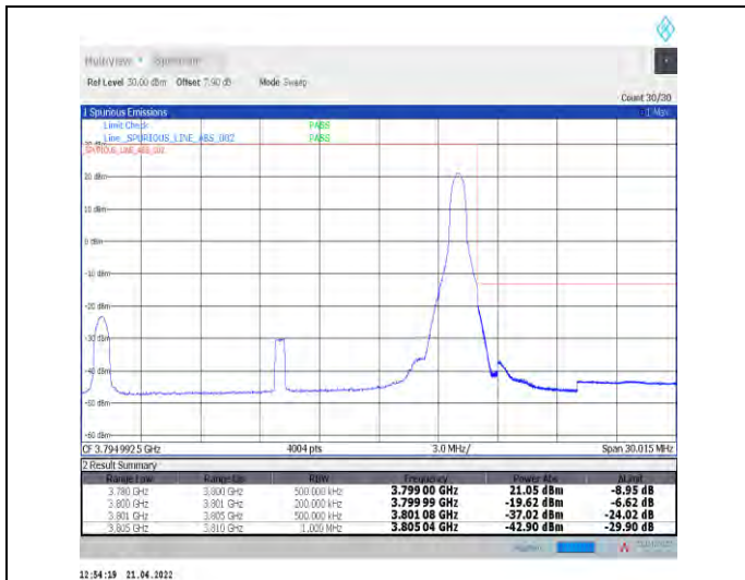
1-N78-3700-3800--30-20-H-2-DFT-PI2BPSK-Edge_1R_B_Right-1@50-Ant1-PASS-see graph
