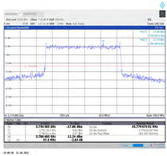
1-N78-3700-3800--30-50-H-3-DFT-16QAM-Outer_Full-128@0-Ant1-45.78-47.500-≤50-PASS
