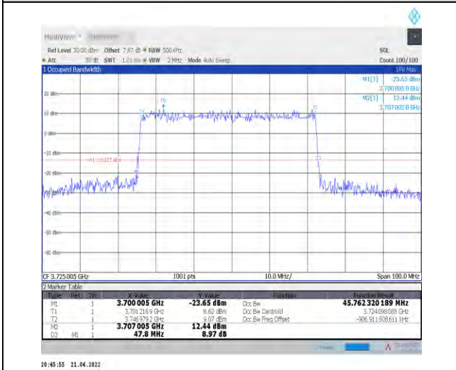
1-N78-3700-3800--30-50-L-4-DFT-64QAM-Outer_Full-128@0-Ant1-45.762-47.800-≤50-PASS
