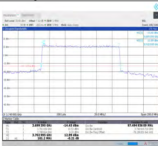
1-N78-3700-3800--30-100-H-6-CP-QPSK-Outer_Full-273@0-Ant1-97.495-101.200-≤100-PASS
