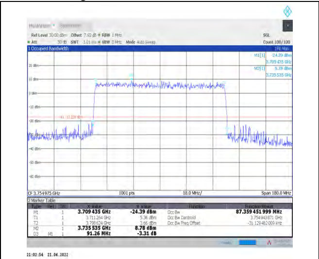
1-N78-3700-3800--30-90-H-9-CP-256QAM-Outer_Full -245@0-Ant1-87.359-91.260-≤90-PASS
