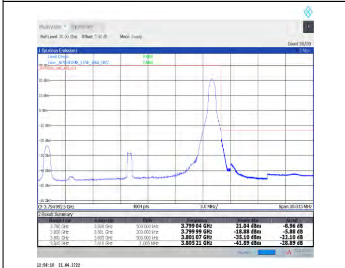
1-N78-3700-3800--30-20-H-5-CP-QPSK-Edge_1RB_R ight-1@50-Ant1-PASS-see graph
