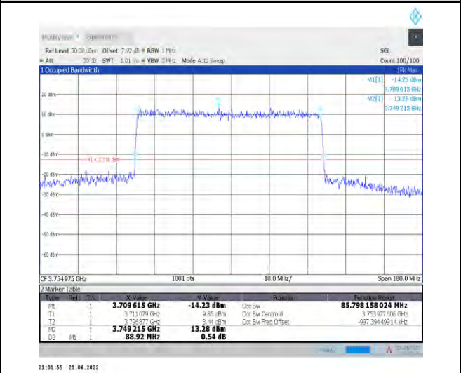
1-N78-3700-3800--30-90-H-3-DFT-16QAM-Outer_Full-240@0-Ant1-85.798-88.920-<=90-PASS
