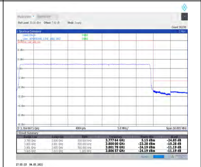
1-N78-3700-3800--30-40-H-6-CP-QPSK-Outer_Fu ll-106@0-Ant1-PASS-see graph
