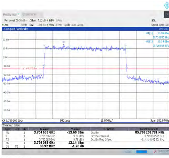
1-N78-3700-3800--30-90-M-3-DFT-16QAM-Outer_Full ull-240@0-Ant1-85.768-88.920-≤90-PASS
