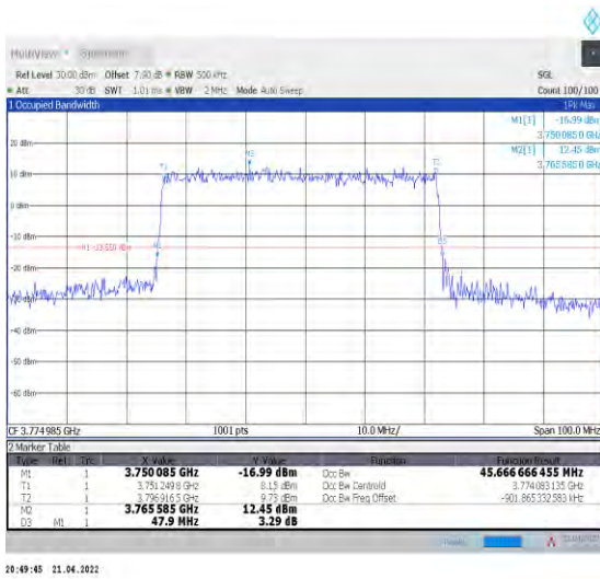
1-N78-3700-3800--30-50-H-4-DFT-64QAM-Outer_Fu ll-128@0-Ant1-45.667-47.900-≤50-PASS
