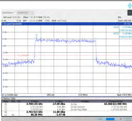
1-N78-3700-3800--30-70-L-4-DFT-64QAM-Outer_Full I-180@0-Ant1-64.366-66.360-≤70-PASS
