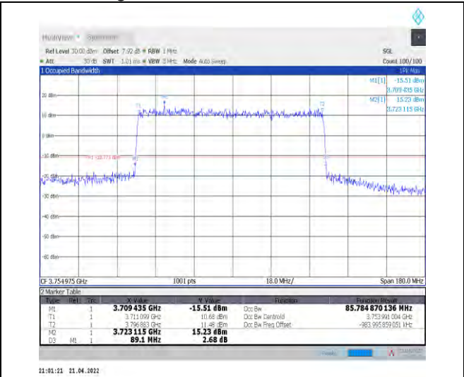
1-N78-3700-3800--30-90-H-1-DFT-QPSK-Outer_Full-240@0-Ant1-85.785-89.100-<=90-PASS
