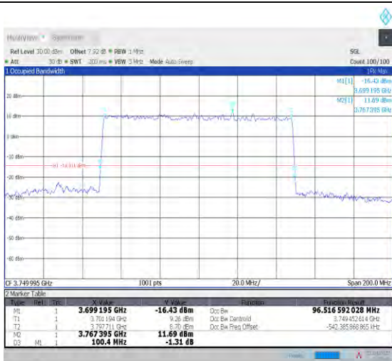
1-N78-3700-3800--30-100-H-5-DFT-256QAM-Outer_Full-270@0-Ant1-96.517-100.400-≤100-PASS
