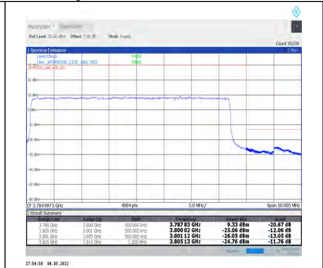
1-N78-3700-3800--30-40-H-3-DFT-PI2BPSK-Outer_Full-100@0-Ant1-PASS-see graph
