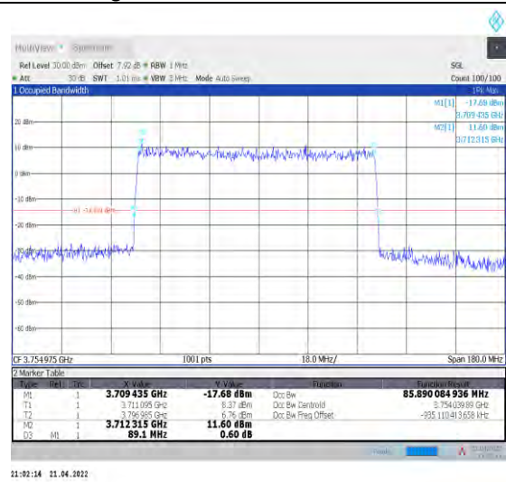
1-N78-3700-3800--30-90-H-5-DFT-256QAM-Outer_Full-240@0-Ant1-85.89-89.100-<=90-PASS
