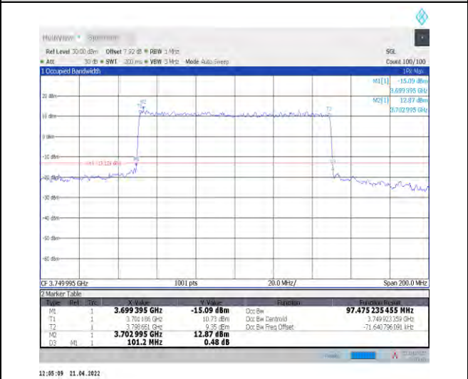
1-N78-3700-3800--30-100-L-6-CP-QPSK-Outer_F ull-273@0-Ant1-97.475-101.200-≤100-PASS
