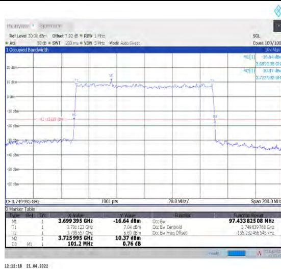
1-N78-3700-3800--30-100-M-9-CP-256QAM-Outer_Full-273@0-Ant1-97.434-101.200-≤100-PASS
