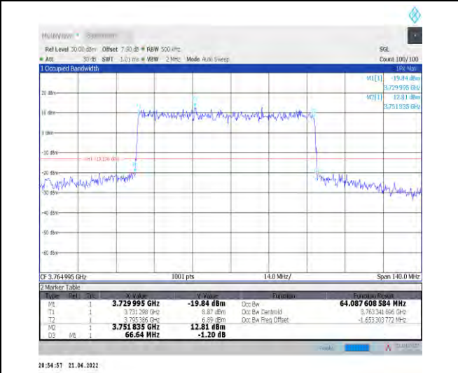
1-N78-3700-3800--30-70-H-1-DFT-QPSK-Outer_Full -180@0-Ant1-64.088-66.640-≤70-PASS
