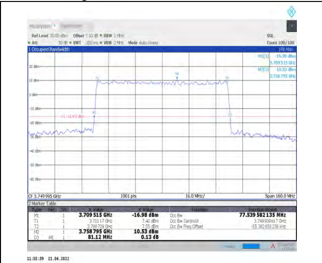
1-N78-3700-3800--30-80-M-9-CP-256QAM-Outer_Full -217@0-Ant1-77.54-81.120-<math>\leq 80</math>-PASS
