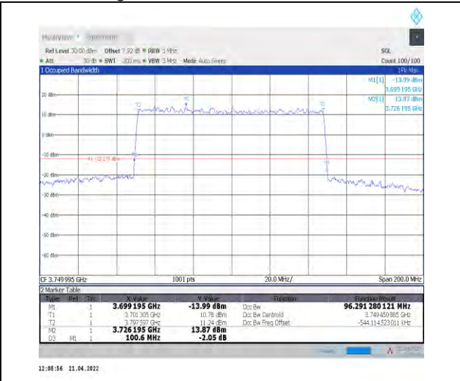
1-N78-3700-3800--30-100-M-3-DFT-16QAM-Outer_Full-270@0-Ant1-96.291-100.600-≤100-PASS
