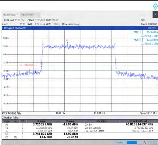
1-N78-3700-3800--30-50-M-1-DFT-QPSK-Outer_Full -128@0-Ant1-45.766-47.600-≤50-PASS
