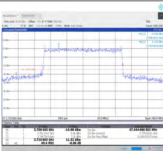
1-N78-3700-3800--30-50-L-6-CP-QPSK-Outer_Full-1 33@0-Ant1-47.445-49.400-≤50-PASS
