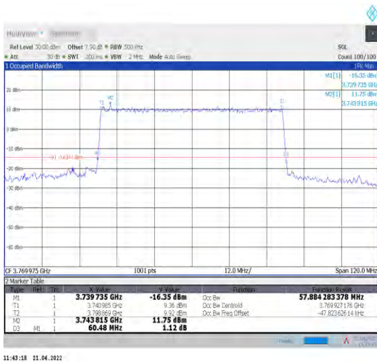
1-N78-3700-3800--30-60-H-7-CP-16QAM-Outer_Full-162@0-Ant1-57.884-60.480-≤60-PASS
