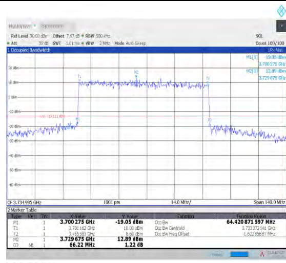
1-N78-3700-3800--30-70-L-1-DFT-QPSK-Outer_Full- 180@0-Ant1-64.421-66.220-≤70-PASS
