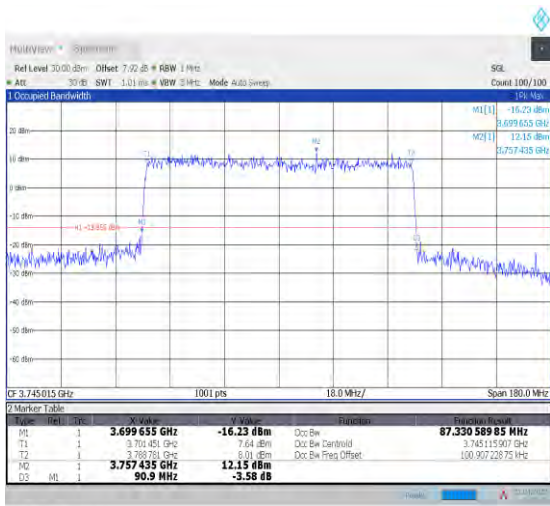
1-N78-3700-3800--30-90-L-8-CP-64QAM-Outer_Full -245@0-Ant1-87.331-90.900-<=90-PASS
