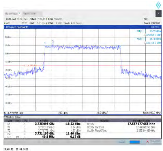
1-N78-3700-3800--30-50-M-8-CP-64QAM-Outer_Full-133@0-Ant1-47.558-49.500-<math>\leq 50</math>-PASS
