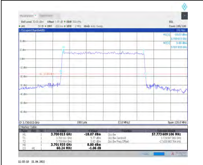
1-N78-3700-3800--30-60-L-9-CP-256QAM-Outer_Fu II-162@0-Ant1-57.774-60.240-≤60-PASS
