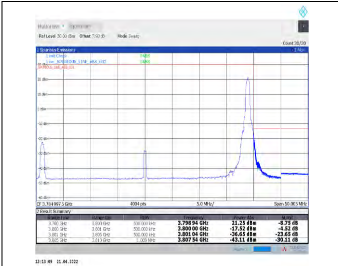
1-N78-3700-3800--30-40-H-2-DFT-PI2BPSK-Edge_1R_B_Right-1@105-Ant1-PASS-see graph
