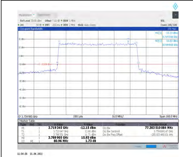
1-N78-3700-3800--30-80-H-1-DFT-QPSK-Outer_Full -216@0-Ant1-77.304-80.960-<math>\leq 80</math>-PASS
