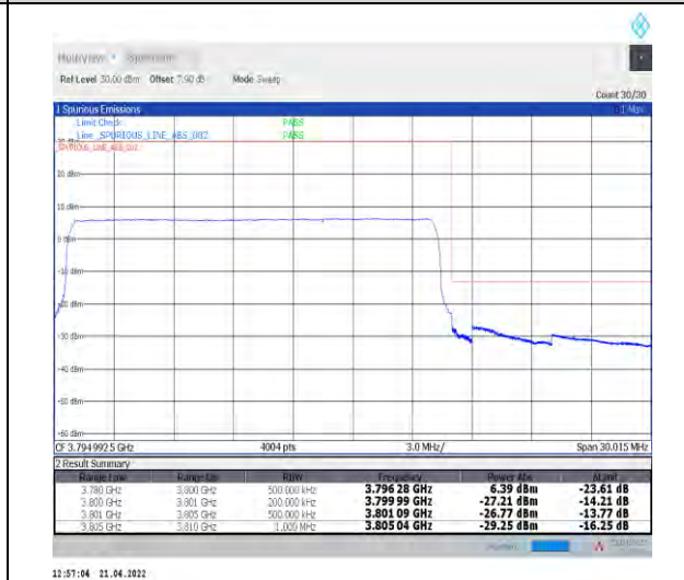
1-N78-3700-3800--30-20-H-6-CP-QPSK-Outer_Fu ll-51@0-Ant1-PASS-see graph
