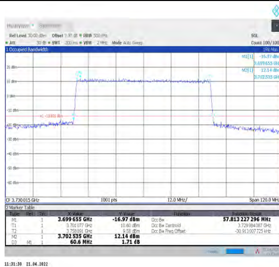
1-N78-3700-3800--30-60-L-6-CP-QPSK-Outer_Full- 162@0-Ant1-57.813-60.600-≤60-PASS
