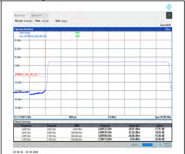
1-N78-3700-3800-PC2-30-40-L-6-CP-QPSK-Outer _Full-106@0-Ant1-PASS-see graph
