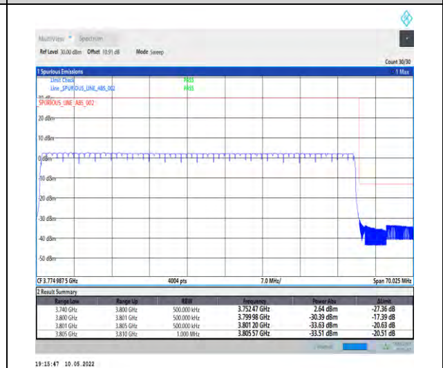
1-N78-3700-3800-PC2-30-60-H-6-CP-QPSK-Outer _Full-162@0-Ant1-PASS-see graph
