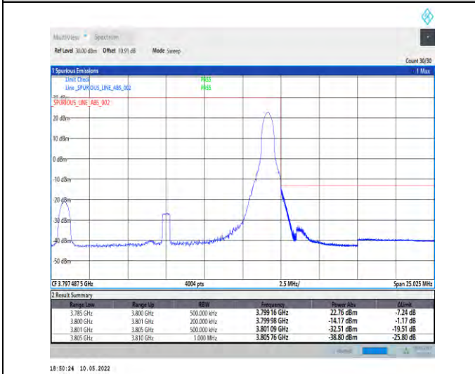
1-N78-3700-3800-PC2-30-15-H-5-CP-QPSK-Edge_1R B_Right-1@37-Ant1-PASS-see graph
