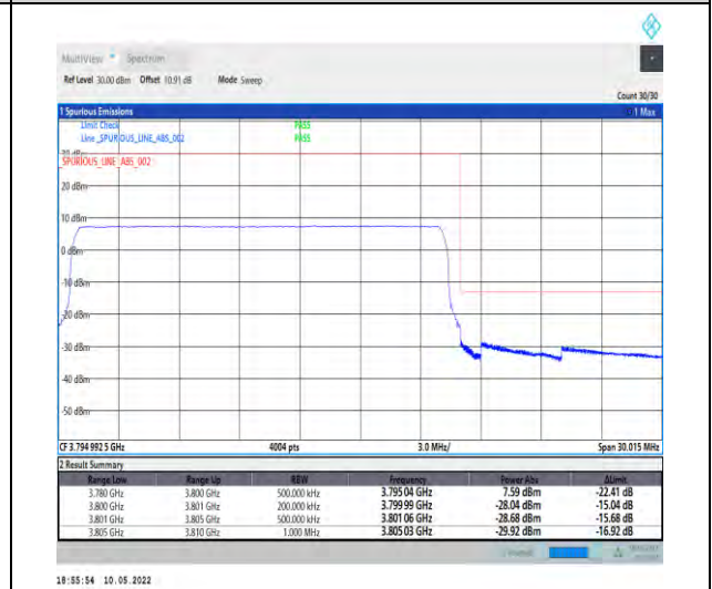
1-N78-3700-3800-PC2-30-20-H-6-CP-QPSK-Outer_Full-51@0-Ant1-PASS-see graph
