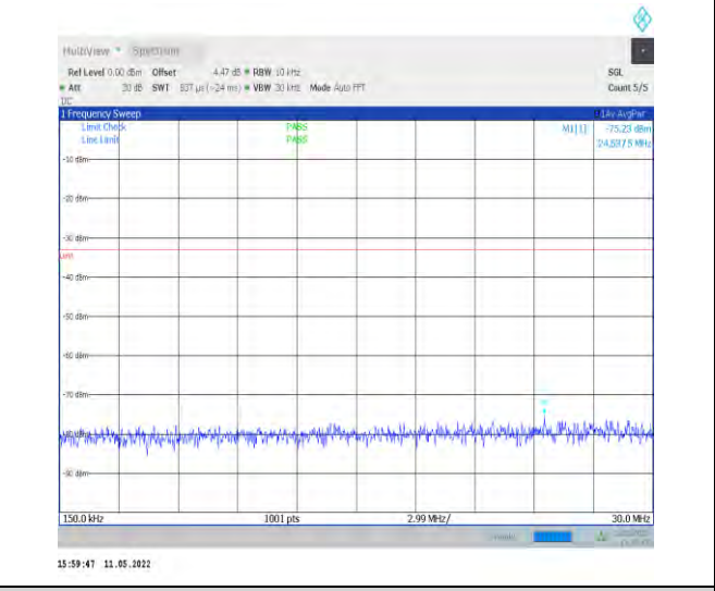
1-N78-3700-3800-PC2-30-100-M-1-DFT-QPSK-Edge _1RB_Left-1@0-0.15-30-Ant1--75.23--33-PASS
