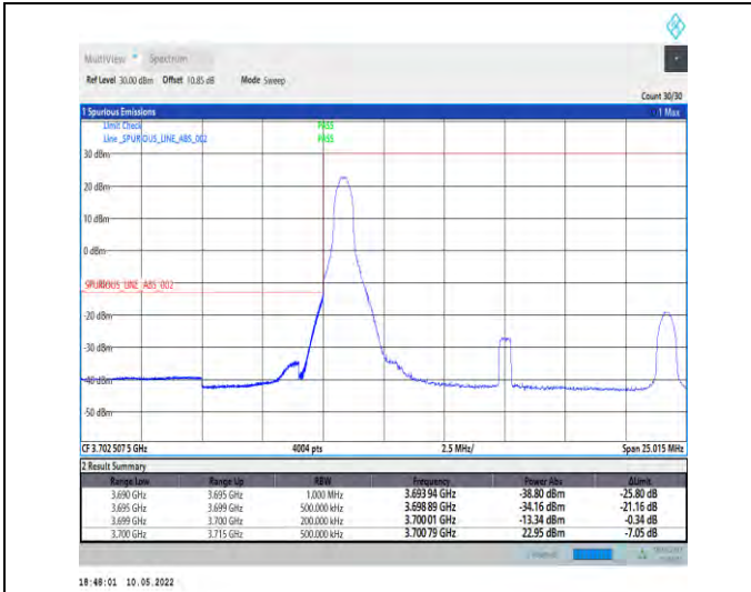
1-N78-3700-3800-PC2-30-15-L-4-CP-QPSK-Edge_1R B_Left-1@0-Ant1-PASS-see graph
