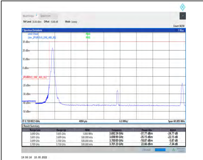
1-N78-3700-3800-PC2-30-50-L-4-CP-QPSK-Edge_1R B_Left-1@0-Ant1-PASS-see graph
