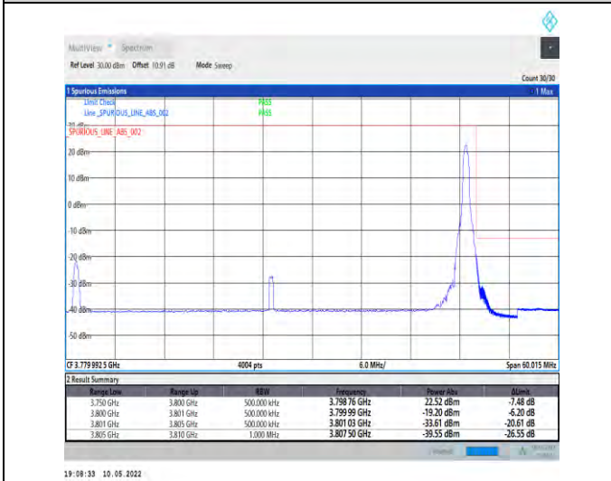
1-N78-3700-3800-PC2-30-50-H-5-CP-QPSK-Edge_1R B_Right-1@132-Ant1-PASS-see graph
