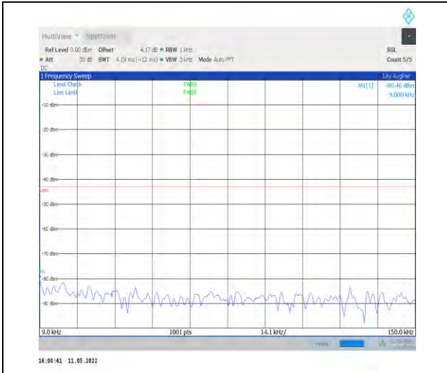
1-N78-3700-3800-PC2-30-100-H-1-DFT-QPSK-Edge e_1RB_Left-1@0-0.009-0.15-Ant1--80.46--43-PASS
