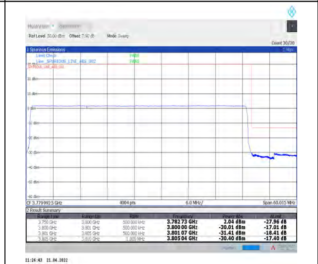
1-N78-3700-3800--30-50-H-6-CP-QPSK-Outer_Fu ll-133@0-Ant1-PASS-see graph
