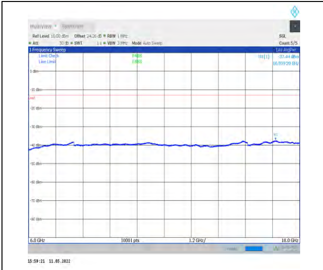
1-N78-3700-3800-PC2-30-100-L-1-DFT-QPSK-Edge _1RB_Left-1@0-6000-18000-Ant1--37.44--13-PASS
