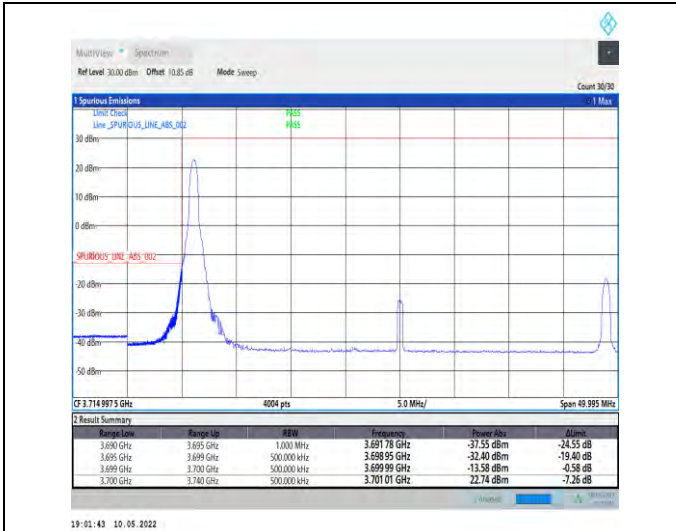
1-N78-3700-3800-PC2-30-40-L-4-CP-QPSK-Edge_1R B_Left-1@0-Ant1-PASS-see graph
