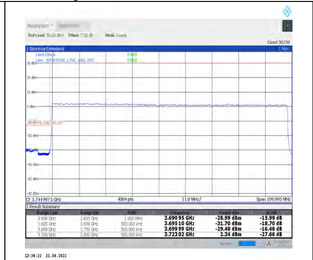
1-N78-3700-3800--30-100-L-3-DFT-PI2BPSK-Out er_Full-270@0-Ant1-PASS-see graph
