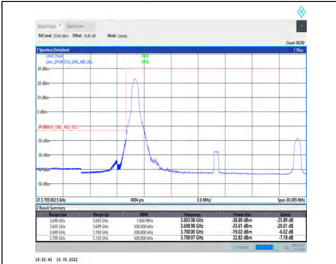
1-N78-3700-3800-PC2-30-20-L-4-CP-QPSK-Edge_1R_B_Left-1@0-Ant1-PASS-see graph
