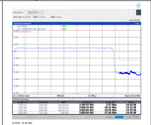
1-N78-3700-3800--30-50-H-3-DFT-PI2BPSK-Outer_Full-128@0-Ant1-PASS-see graph
