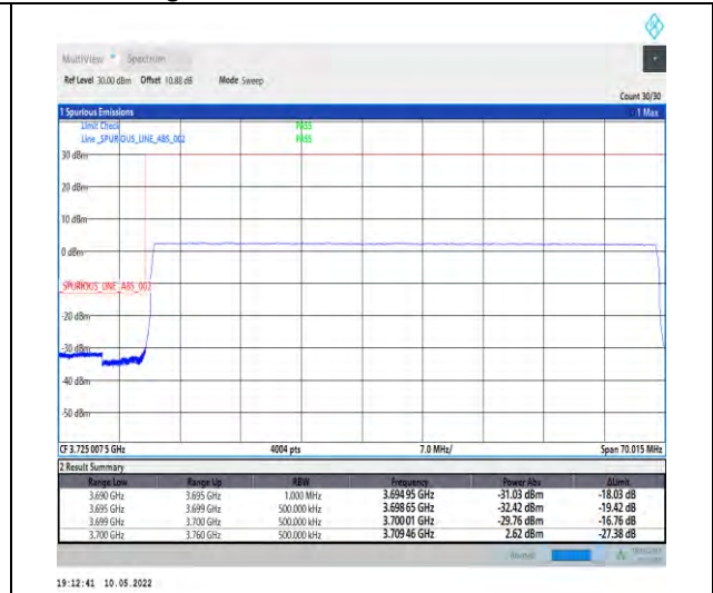
1-N78-3700-3800-PC2-30-60-L-6-CP-QPSK-Outer _Full-162@0-Ant1-PASS-see graph
