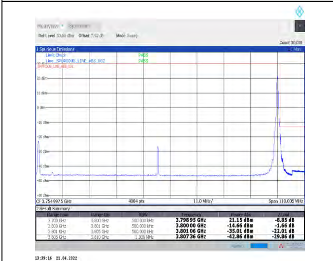
1-N78-3700-3800--30-100-H-5-CP-QPSK-Edge_1RB_Right-1@272-Ant1-PASS-see graph
