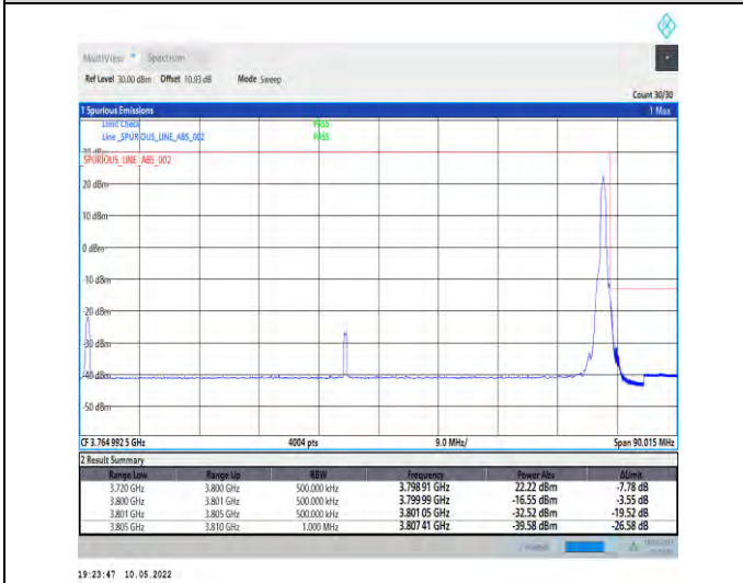
1-N78-3700-3800-PC2-30-80-H-5-CP-QPSK-Edge_1R B_Right-1@216-Ant1-PASS-see graph
