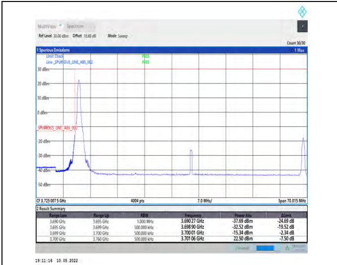
1-N78-3700-3800-PC2-30-60-L-4-CP-QPSK-Edge_1R B_Left-1@0-Ant1-PASS-see graph
