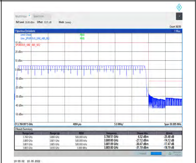
1-N78-3700-3800-PC2-30-40-H-6-CP-QPSK-Outer _Full-106@0-Ant1-PASS-see graph
