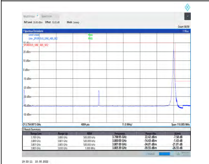
1-N78-3700-3800-PC2-30-100-H-5-CP-QPSK-Edge_1 RB_Right-1@272-Ant1-PASS-see graph
