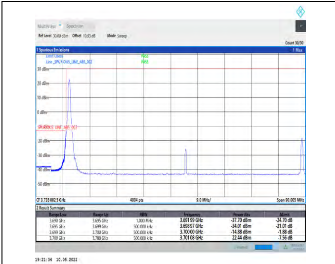
1-N78-3700-3800-PC2-30-80-L-4-CP-QPSK-Edge_1R B_Left-1@0-Ant1-PASS-see graph
