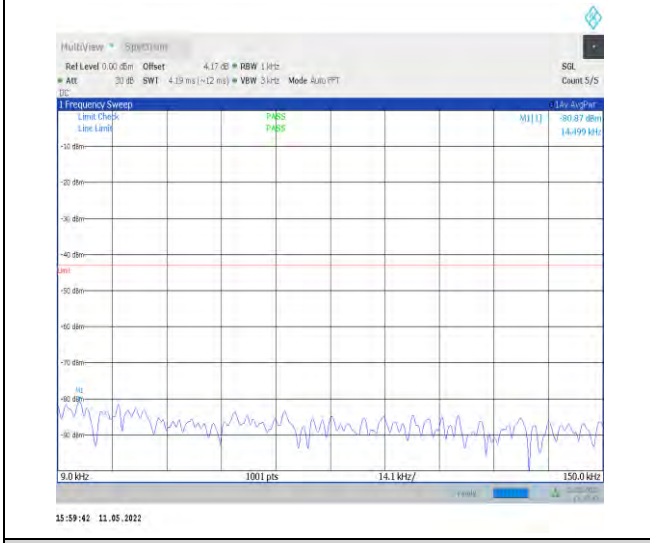
1-N78-3700-3800-PC2-30-100-M-1-DFT-QPSK-Edg e_1RB_Left-1@0-0.009-0.15-Ant1--80.87--43-PASS
