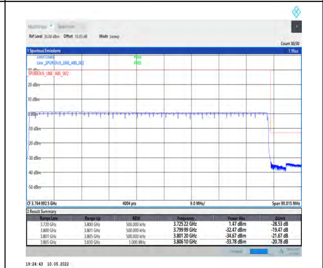
1-N78-3700-3800-PC2-30-80-H-6-CP-QPSK-Outer _Full-217@0-Ant1-PASS-see graph
