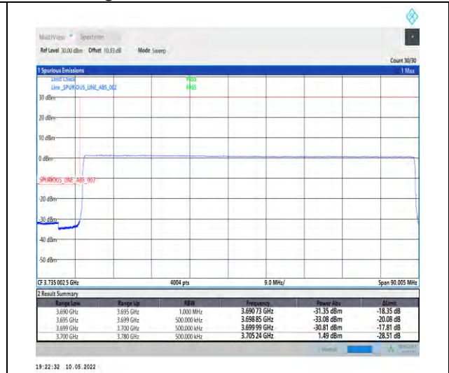
1-N78-3700-3800-PC2-30-80-L-6-CP-QPSK-Outer _Full-217@0-Ant1-PASS-see graph
