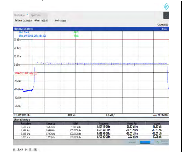
1-N78-3700-3800-PC2-30-70-L-6-CP-QPSK-Outer _Full-189@0-Ant1-PASS-see graph
