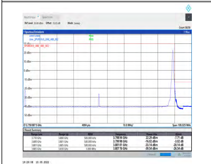
1-N78-3700-3800-PC2-30-90-H-5-CP-QPSK-Edge_1R B_Right-1@244-Ant1-PASS-see graph
