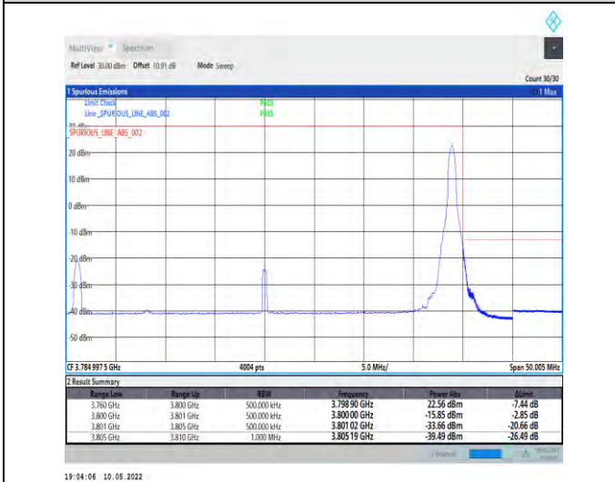
1-N78-3700-3800-PC2-30-40-H-5-CP-QPSK-Edge_1R B_Right-1@105-Ant1-PASS-see graph
