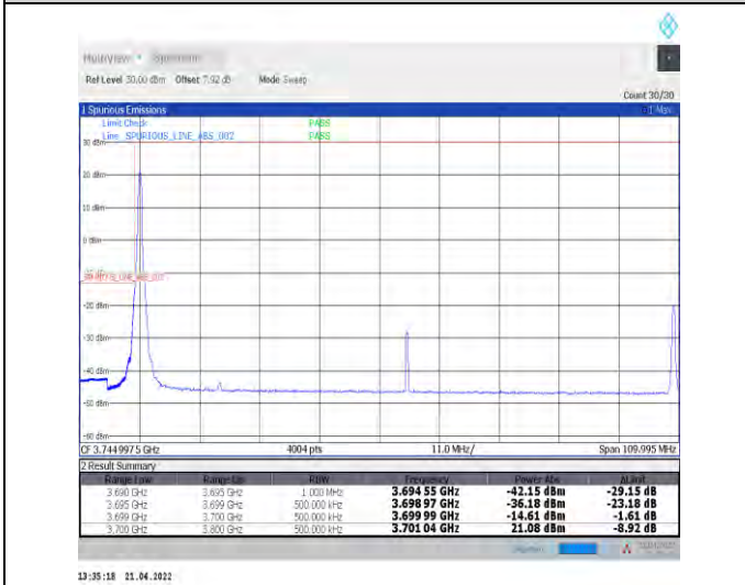
1-N78-3700-3800--30-100-L-4-CP-QPSK-Edge_1RB_Left-1@0-Ant1-PASS-see graph
