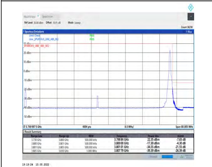
1-N78-3700-3800-PC2-30-70-H-5-CP-QPSK-Edge_1R B_Right-1@188-Ant1-PASS-see graph
