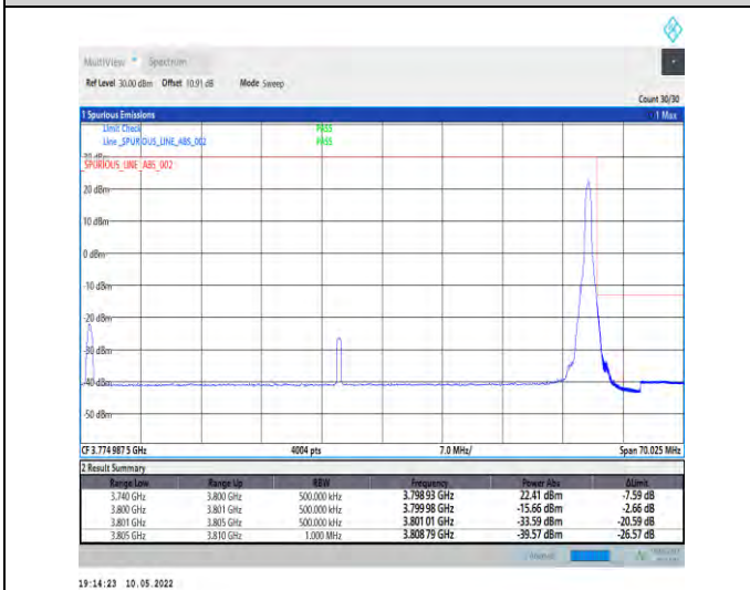
1-N78-3700-3800-PC2-30-60-H-5-CP-QPSK-Edge_1R B_Right-1@161-Ant1-PASS-see graph
