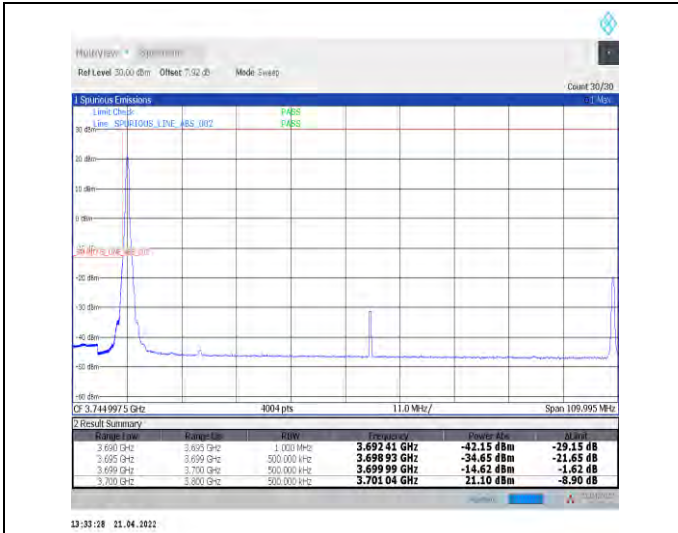
1-N78-3700-3800--30-100-L-1-DFT-PI2BPSK-Edge_1 RB_Left-1@0-Ant1-PASS-see graph
