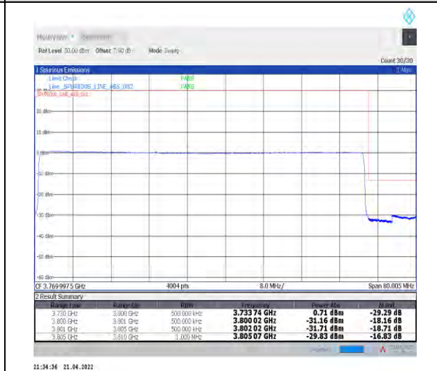
1-N78-3700-3800--30-70-H-6-CP-QPSK-Outer_Fu ll-189@0-Ant1-PASS-see graph
