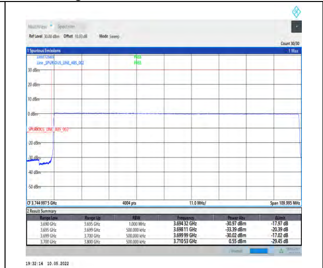
1-N78-3700-3800-PC2-30-100-L-6-CP-QPSK-Out er_Full-273@0-Ant1-PASS-see graph
