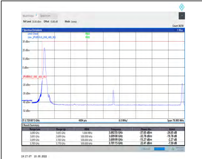
1-N78-3700-3800-PC2-30-70-L-4-CP-QPSK-Edge_1R B_Left-1@0-Ant1-PASS-see graph
