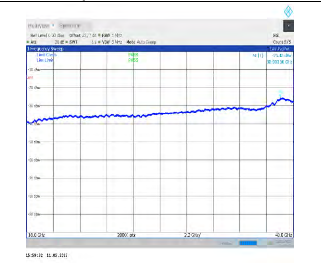
1-N78-3700-3800-PC2-30-100-L-1-DFT-QPSK-Edge _1RB_Left-1@0-18000-40000-Ant1--25.45--13-PASS
