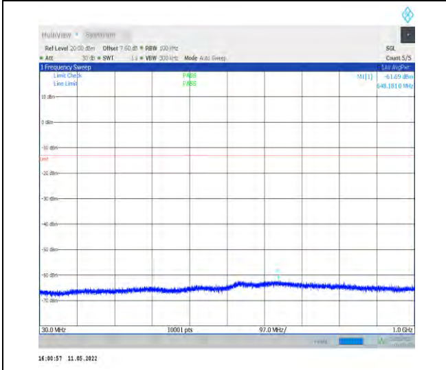
1-N78-3700-3800-PC2-30-100-H-1-DFT-QPSK-Edge e_1RB_Left-1@0-30-1000-Ant1--61.69--13-PASS
