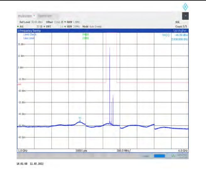
1-N78-3700-3800-PC2-30-100-H-1-DFT-QPSK-Edge _1RB_Left-1@0-1000-6000-Ant1--46.50--13-PASS
