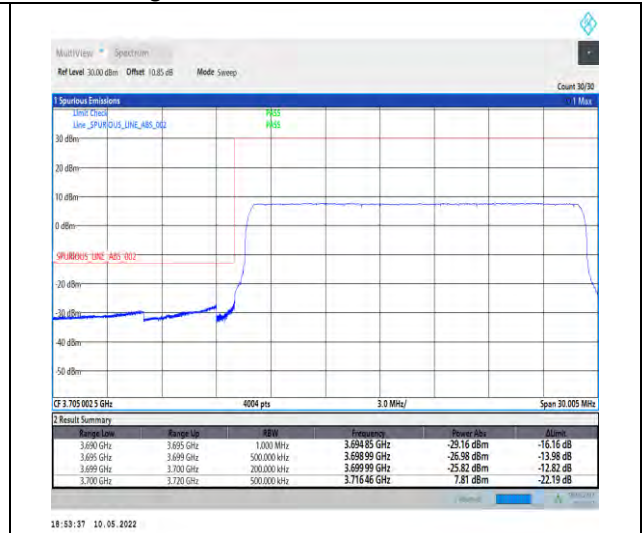
1-N78-3700-3800-PC2-30-20-L-6-CP-QPSK-Outer_Full-51@0-Ant1-PASS-see graph
