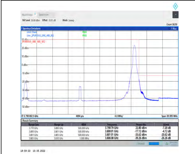
1-N78-3700-3800-PC2-30-30-H-5-CP-QPSK-Edge_1R B_Right-1@77-Ant1-PASS-see graph
