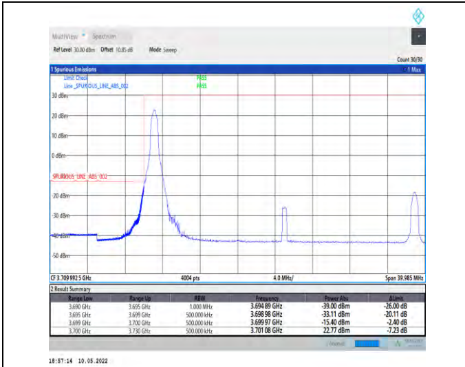
1-N78-3700-3800-PC2-30-30-L-4-CP-QPSK-Edge_1R B_Left-1@0-Ant1-PASS-see graph
