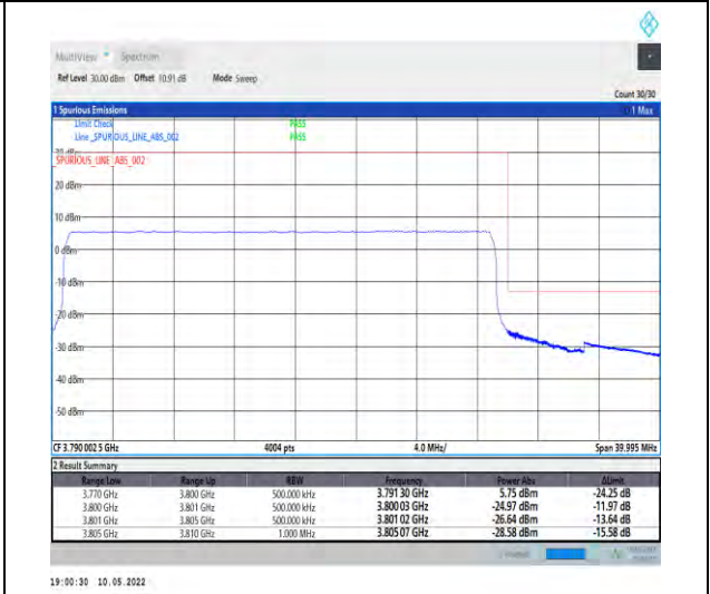
1-N78-3700-3800-PC2-30-30-H-6-CP-QPSK-Outer _Full-78@0-Ant1-PASS-see graph
