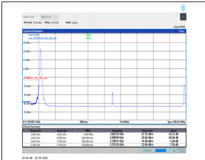
1-N78-3700-3800-PC2-30-90-L-4-CP-QPSK-Edge_1R B_Left-1@0-Ant1-PASS-see graph
