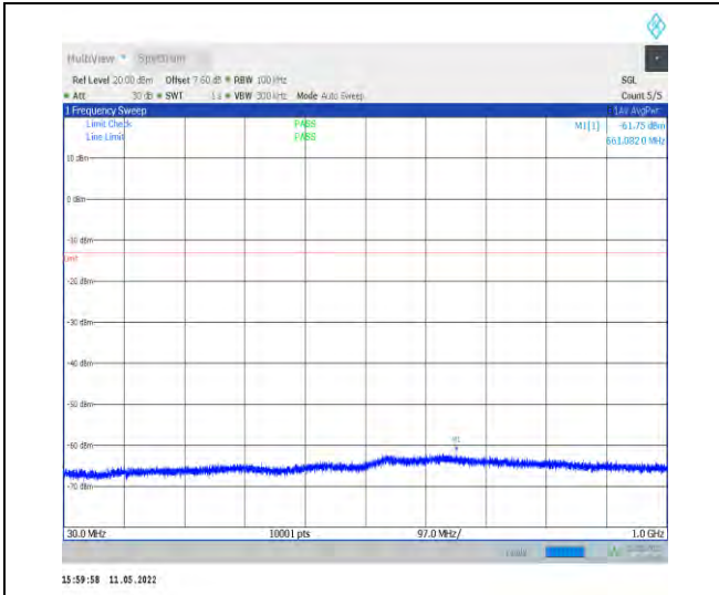
1-N78-3700-3800-PC2-30-100-M-1-DFT-QPSK-Edge e_1RB_Left-1@0-30-1000-Ant1--61.75--13-PASS
