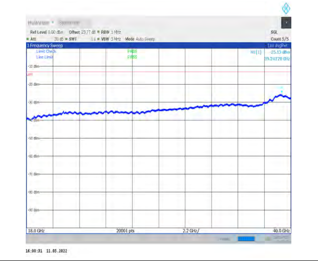
1-N78-3700-3800-PC2-30-100-M-1-DFT-QPSK-Edge _1RB_Left-1@0-18000-40000-Ant1--25.13--13-PASS
