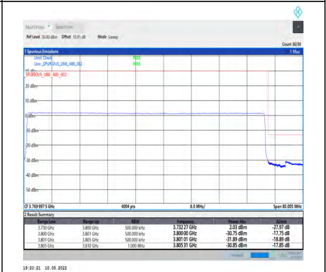
1-N78-3700-3800-PC2-30-70-H-6-CP-QPSK-Outer _Full-189@0-Ant1-PASS-see graph
