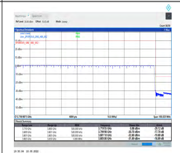
1-N78-3700-3800-PC2-30-90-H-6-CP-QPSK-Outer _Full-245@0-Ant1-PASS-see graph
