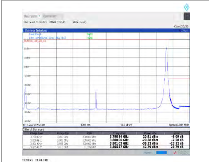
1-N78-3700-3800--30-70-H-5-CP-QPSK-Edge_1RB_R ight-1@188-Ant1-PASS-see graph
