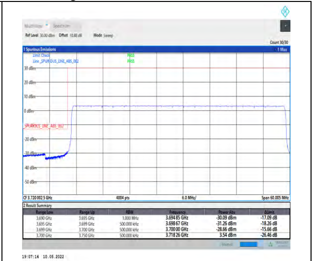
1-N78-3700-3800-PC2-30-50-L-6-CP-QPSK-Outer _Full-133@0-Ant1-PASS-see graph
