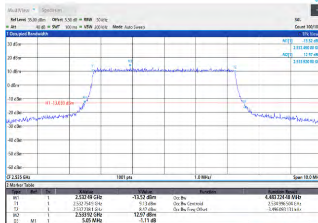
Band7-5MHz-QPSK-21100-25RB#0
