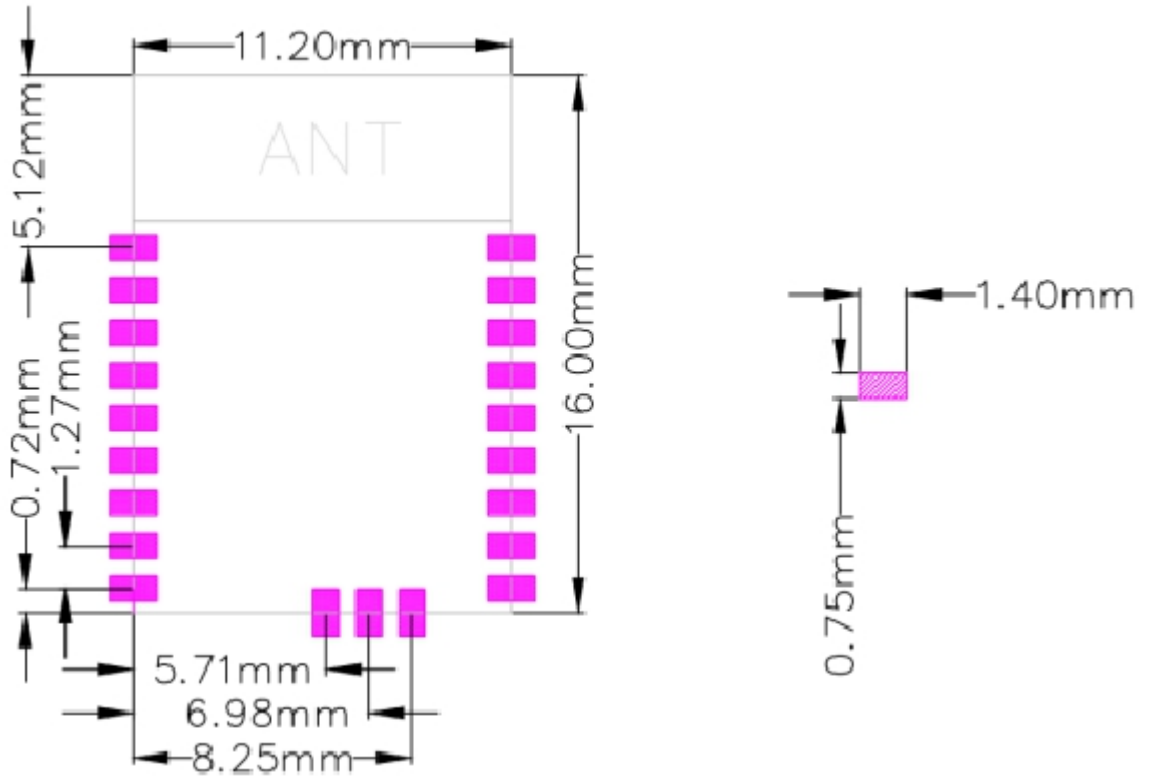
4-5 Reference packaging size
