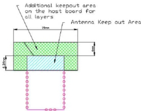
4- 4 Antenna Keep out
