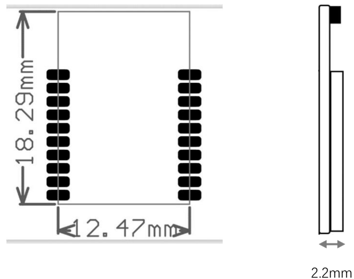
Figure 4: Module Dimensions
