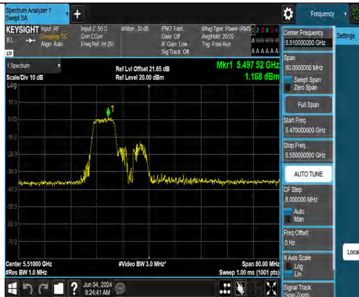
11BE40MIMO Ant4 5510 52+26 OFDMA 1
