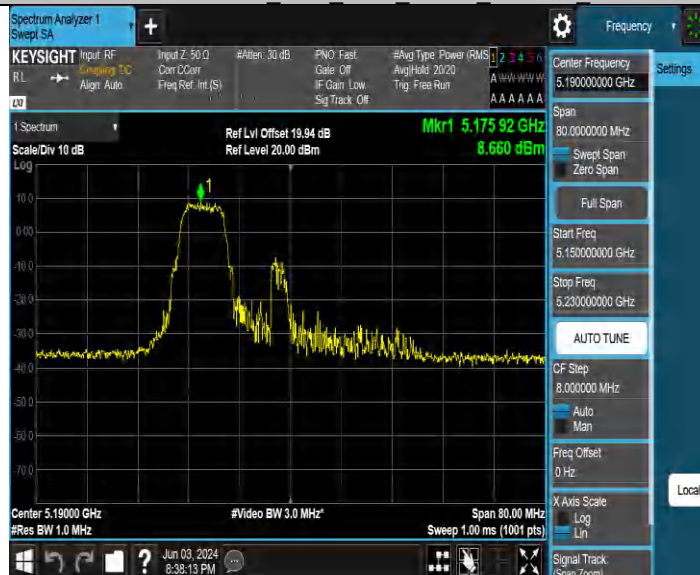
11BE40MIMO Ant4 5190 52+26 OFDMA 1
