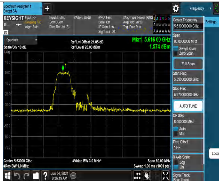
11BE40MIMO Ant3 5630 52+26 OFDMA 1
