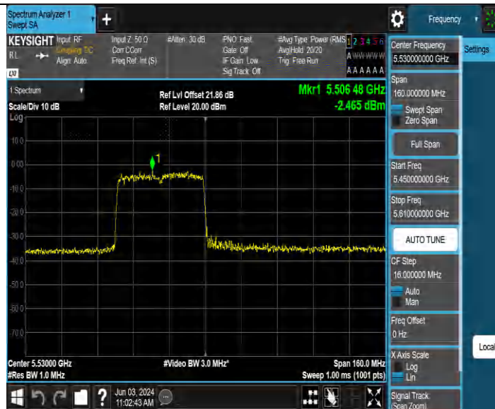
11BE80MIMO Ant2 5530 26Tone RU0
