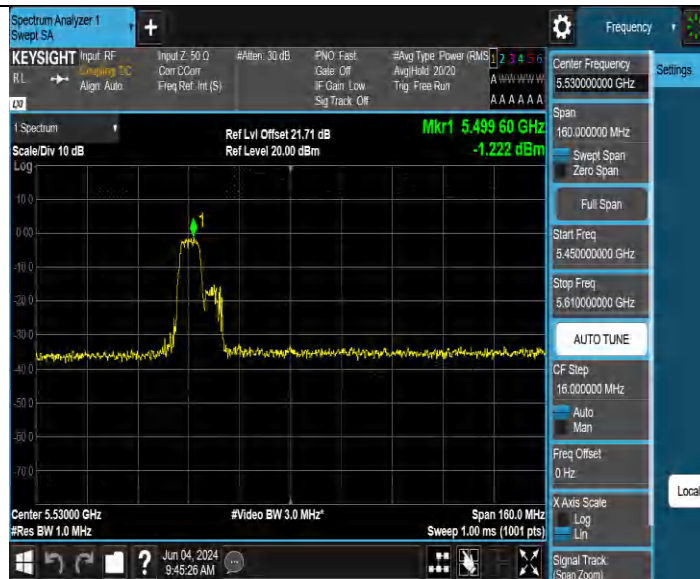
11BE80MIMO Ant4 5530 52+26 OFDMA 1
