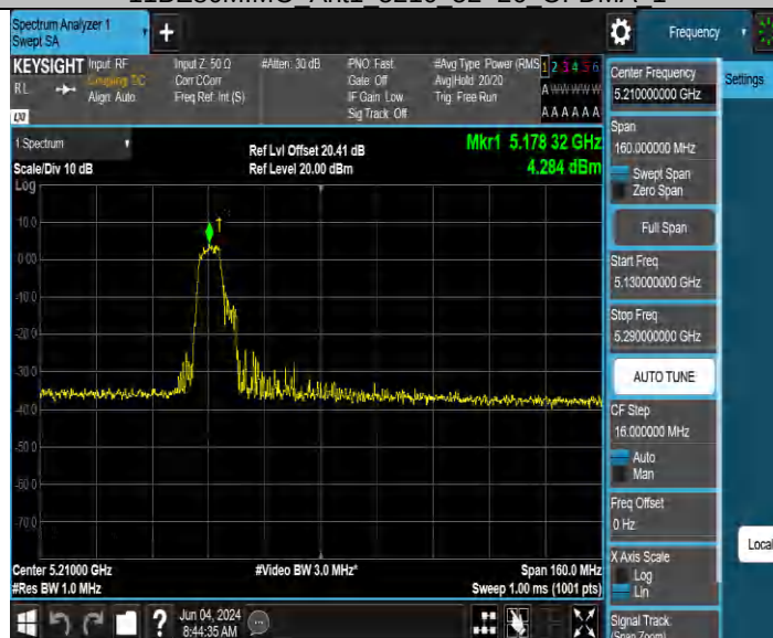
11BE80MIMO Ant2 5210 52+26 OFDMA 1
