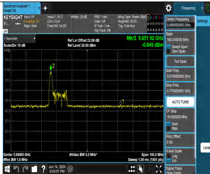
11BE80MIMO Ant1 5690 UNII-2C 484Tone RU65
