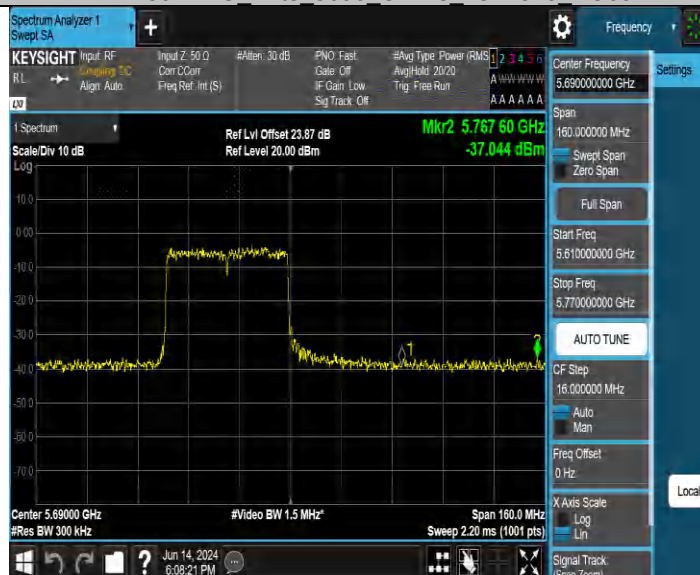
11BE80MIMO Ant4 5690 UNII-3 26Tone RU0
