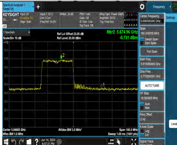
11BE80MIMO Ant2 5690 UNII-2C 26Tone RU0
