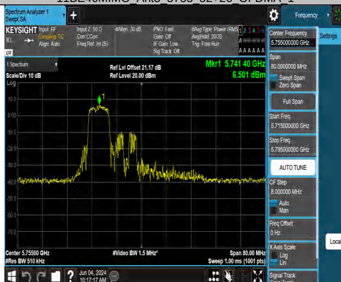
11BE40MIMO Ant4 5755 52+26 OFDMA 1
