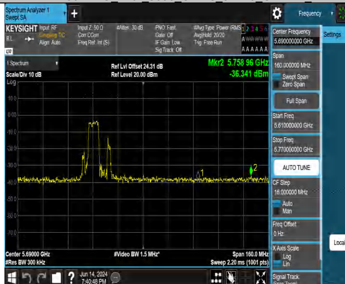
11BE80MIMO Ant2 5690 UNII-3 52+26 OFDMA 1
