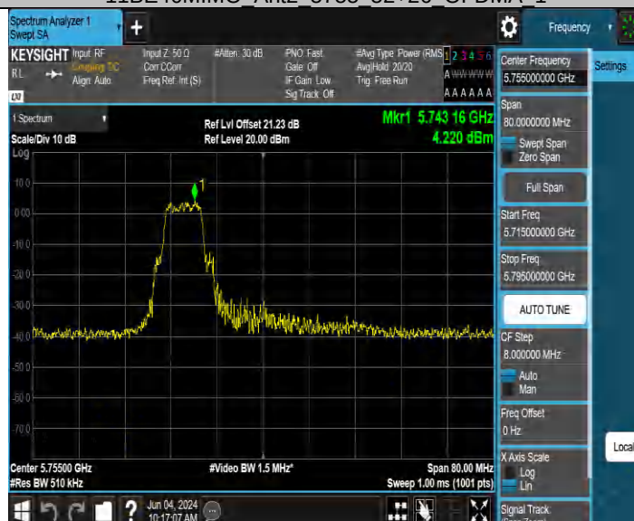
11BE40MIMO Ant3 5755 52+26 OFDMA 1
