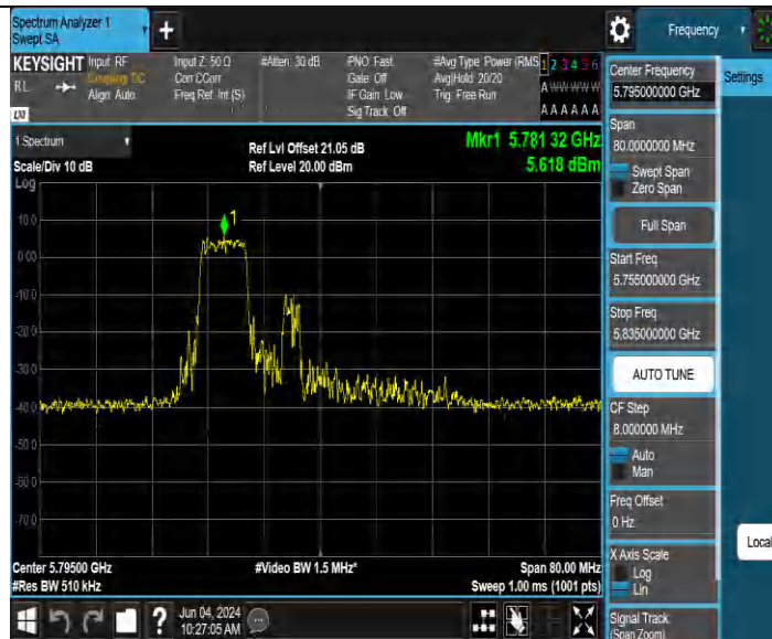
11BE40MIMO Ant4 5795 52+26 OFDMA 1
