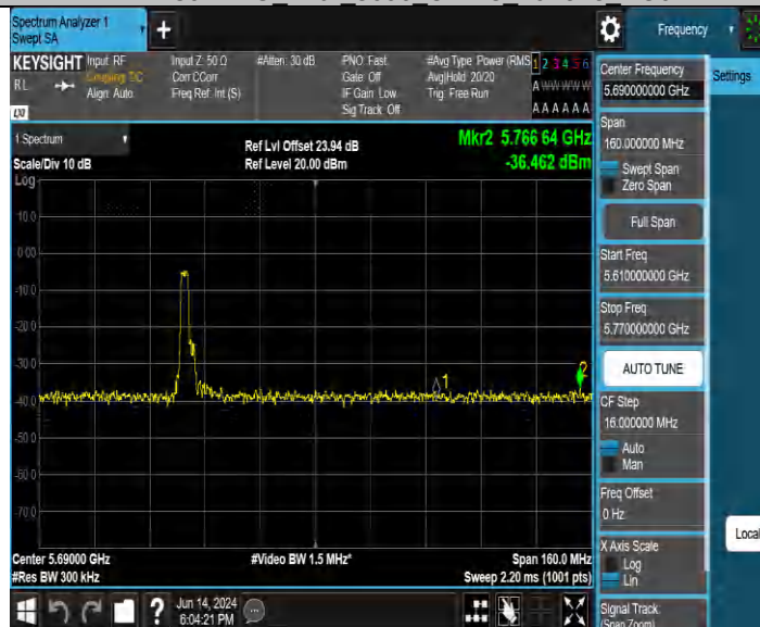
11BE80MIMO Ant2 5690 UNII-3 484Tone RU65
