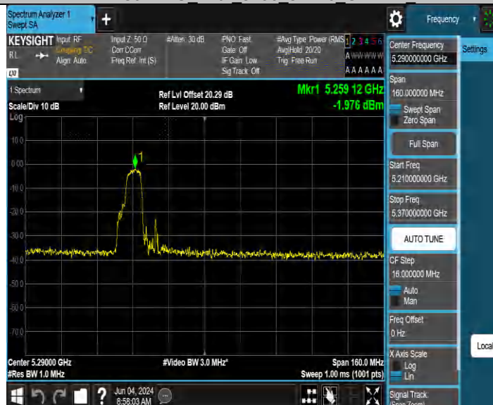
11BE80MIMO Ant3 5290 52+26 OFDMA 1
