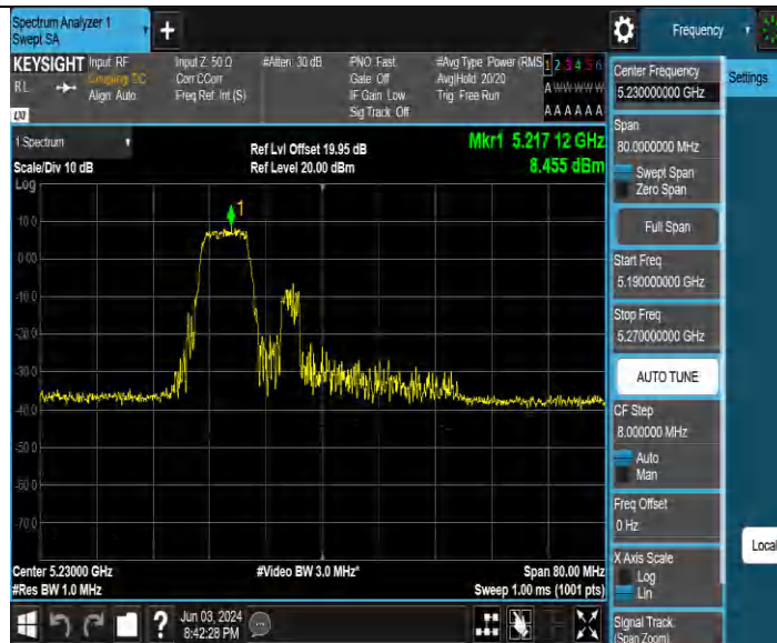
11BE40MIMO Ant4 5230 52+26 OFDMA 1
