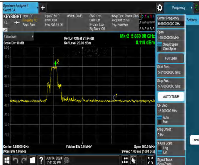
11BE80MIMO Ant1 5690 UNII-3 52+26 OFDMA 1
