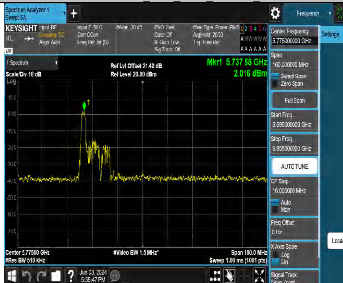
11BE80MIMO Ant4 5775 484Tone RU65
