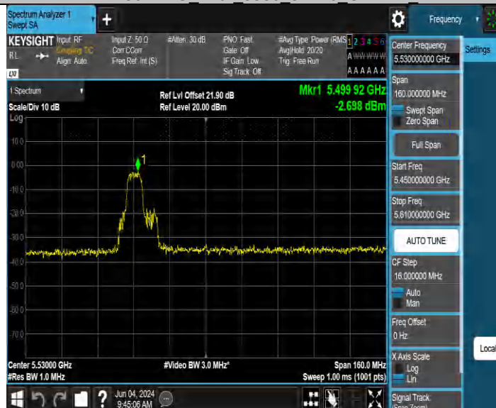
11BE80MIMO Ant2 5530 52+26 OFDMA 1
