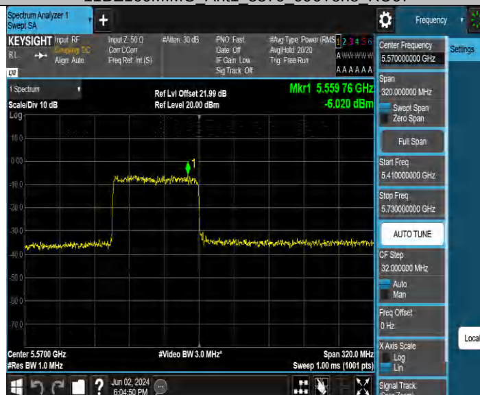
11BE160MIMO Ant2 5570 996Tone RU67
