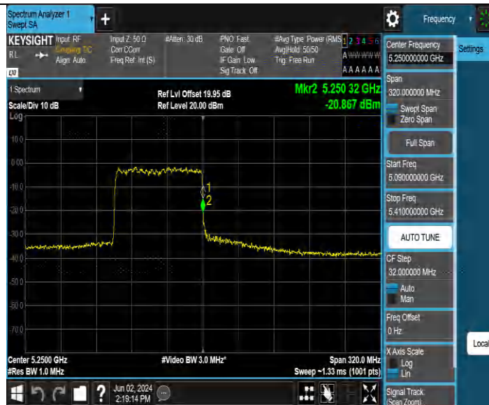
11BE160MIMO Ant4 5250 UNII-2A 996Tone RU67
