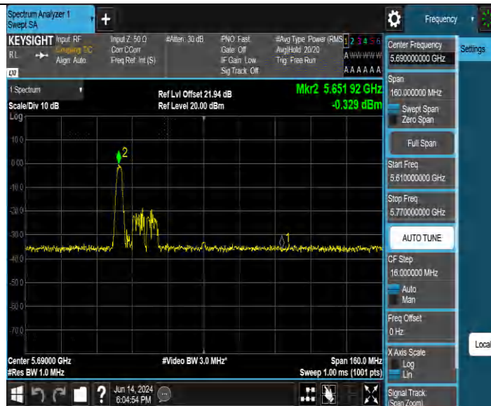
11BE80MIMO Ant4 5690 UNII-2C 484Tone RU65
