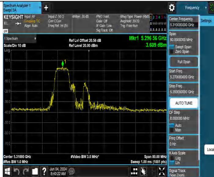
11BE40MIMO Ant2 5310 52+26 OFDMA 1
