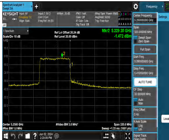
11BE160MIMO Ant1 5250 UNII-2A 996Tone RU67
