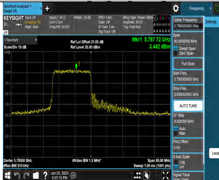
11BE40MIMO Ant4 5795 26Tone RU0
