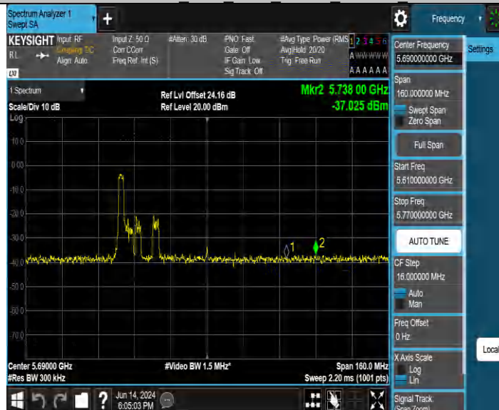
11BE80MIMO Ant4 5690 UNII-3 484Tone RU65
