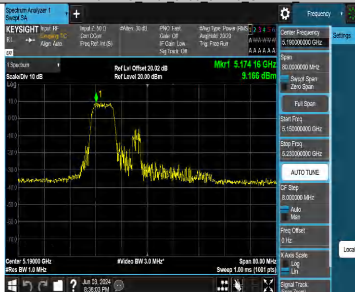
11BE40MIMO Ant3 5190 52+26 OFDMA 1
