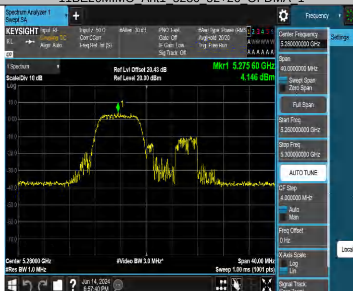
11BE20MIMO Ant2 5280 52+26 OFDMA 1
