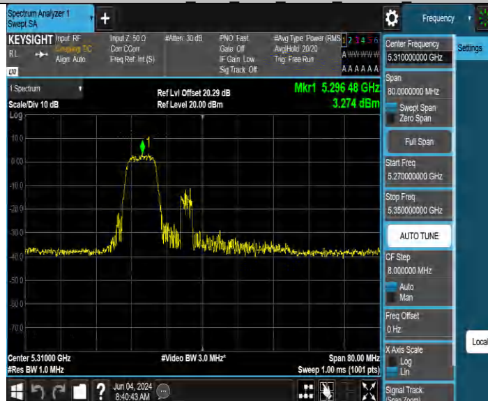
11BE40MIMO Ant4 5310 52+26 OFDMA 1
