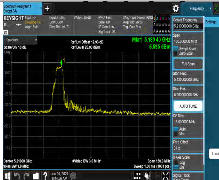
11BE80MIMO Ant4 5210 52+26 OFDMA 1
