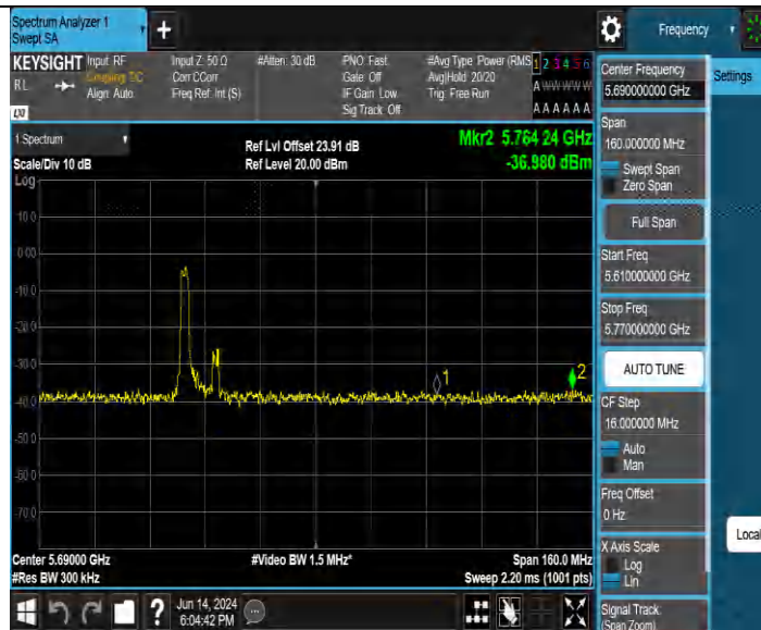
11BE80MIMO Ant3 5690 UNII-3 484Tone RU65
