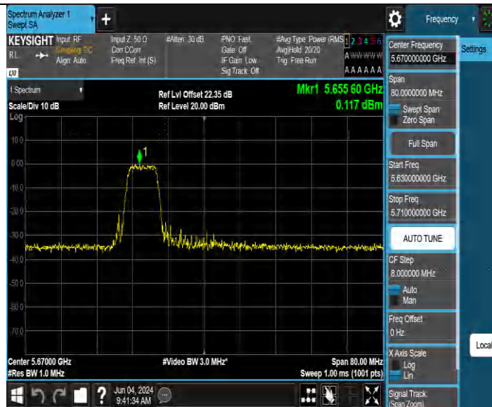
11BE40MIMO Ant2 5670 52+26 OFDMA 1
