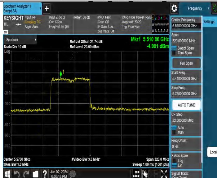
11BE160MIMO Ant4 5570 996Tone RU67
