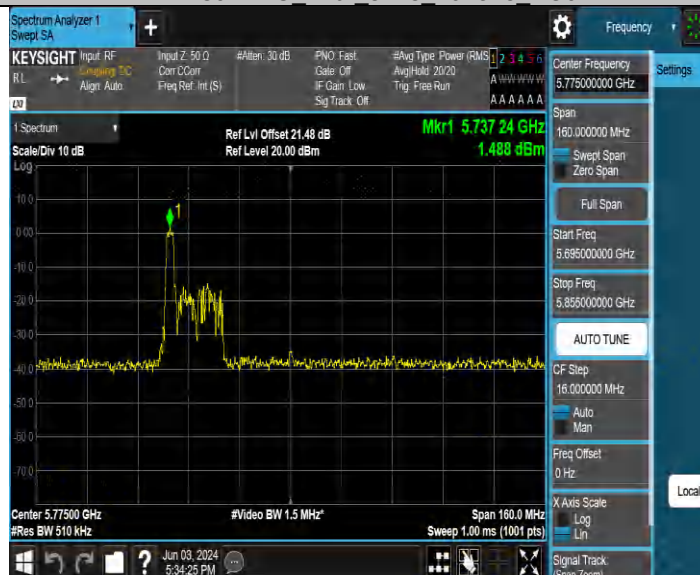
11BE80MIMO Ant1 5775 484Tone RU65
