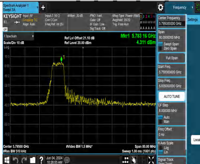
11BE40MIMO Ant3 5795 52+26 OFDMA 1
