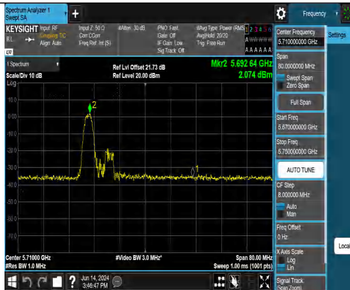
11AX40MIMO Ant2 5710 UNII-2C 242Tone RU61
