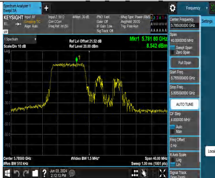
11AX20MIMO Ant2 5785 26Tone RU0
