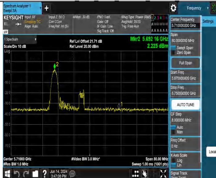
11AX40MIMO Ant3 5710 UNII-2C 242Tone RU61
