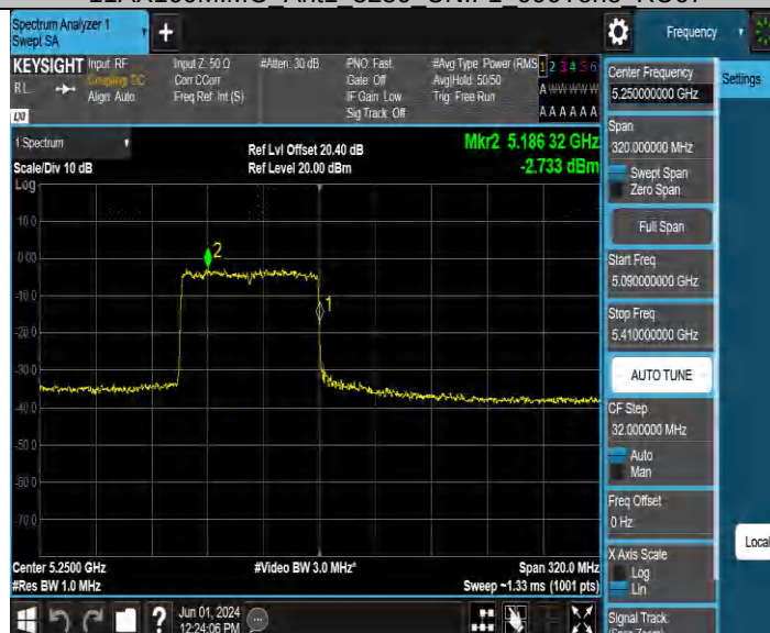
11AX160MIMO Ant2 5250 UNII-1 996Tone RU67
