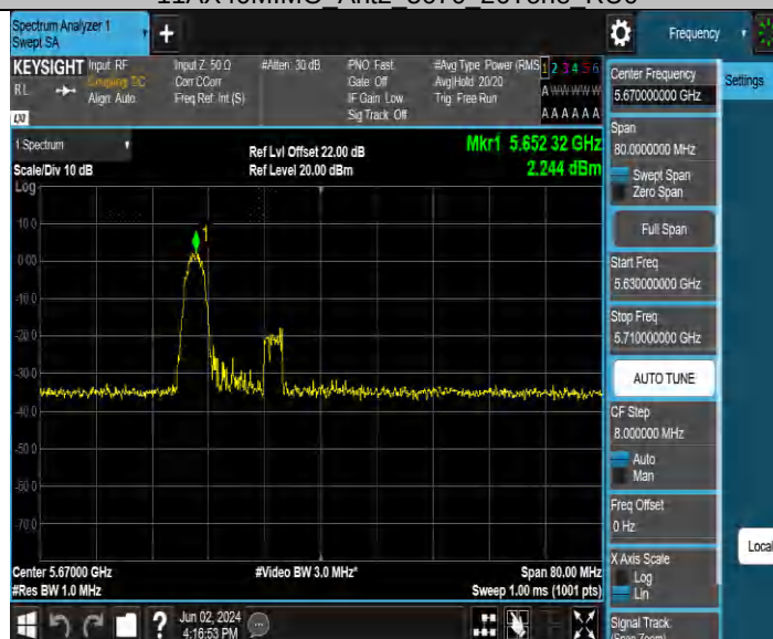
11AX40MIMO Ant2 5670 242Tone RU61
