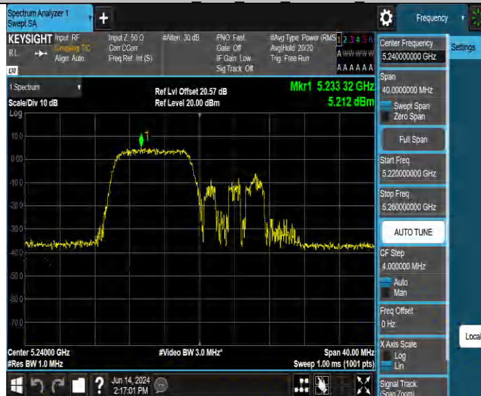
11AX20MIMO Ant3 5240 26Tone RU0
