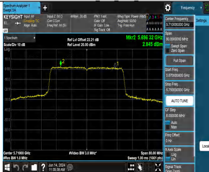
11BE40MIMO Ant1 5710 UNII-3
