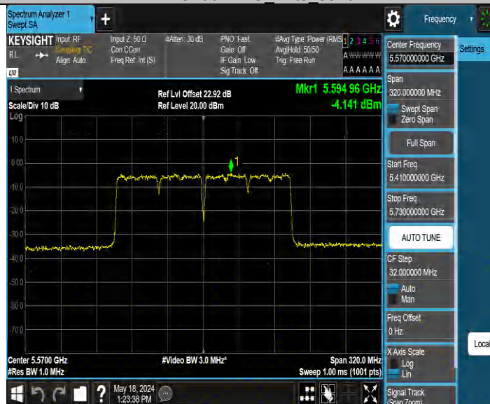
11AC160MIMO Ant4 5570
