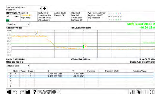
Band-edge Channel 11
