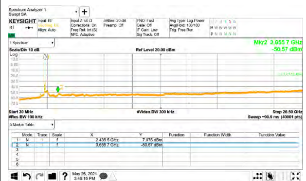
Out-Of-Band Channel 6
