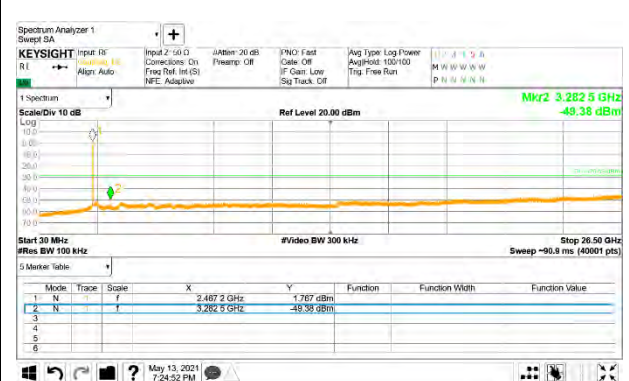
Out-Of-Band Channel 11
