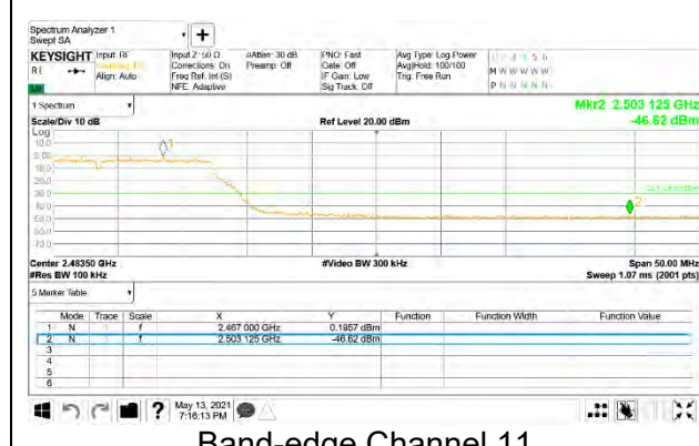
Band-edge Channel 11
