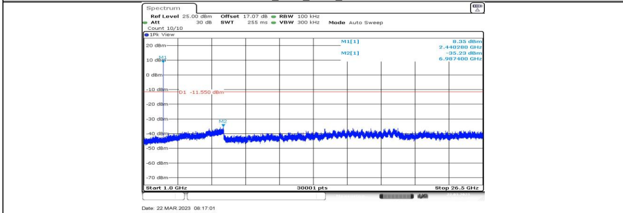
LE 1M_Ant1_2440_1000~26500
