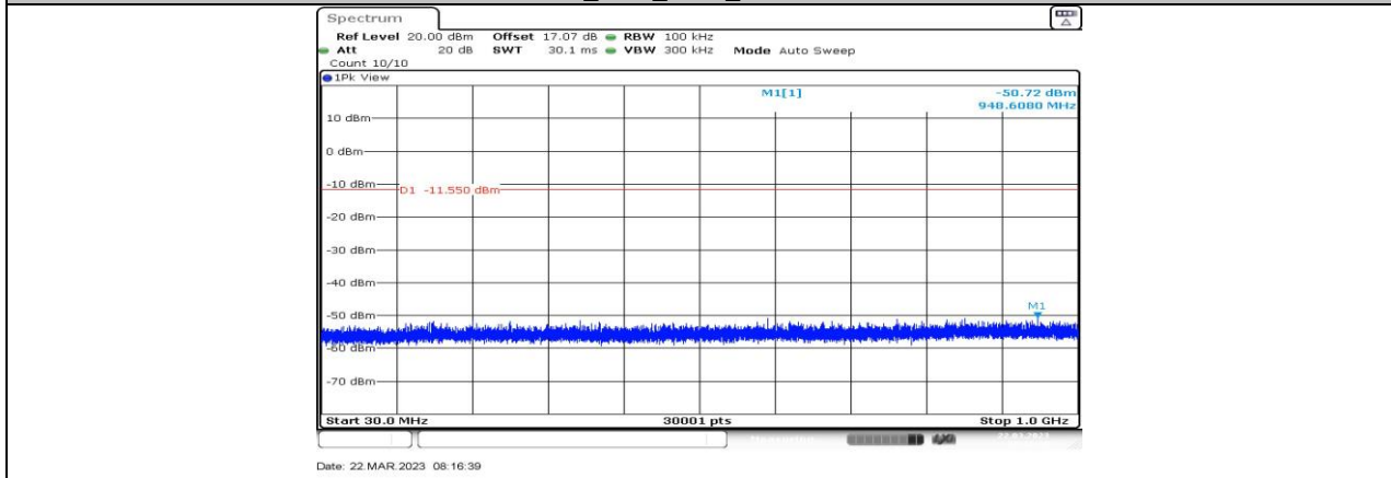
LE 1M_Ant1_2440_30~1000
