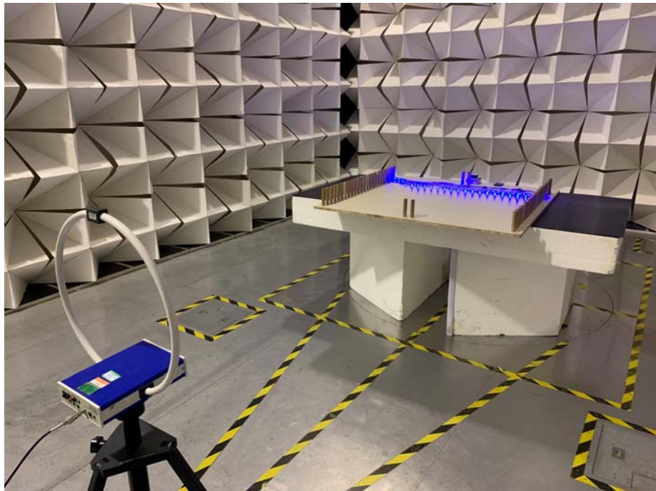
For 9KHz-30MHz Test Site 1#
