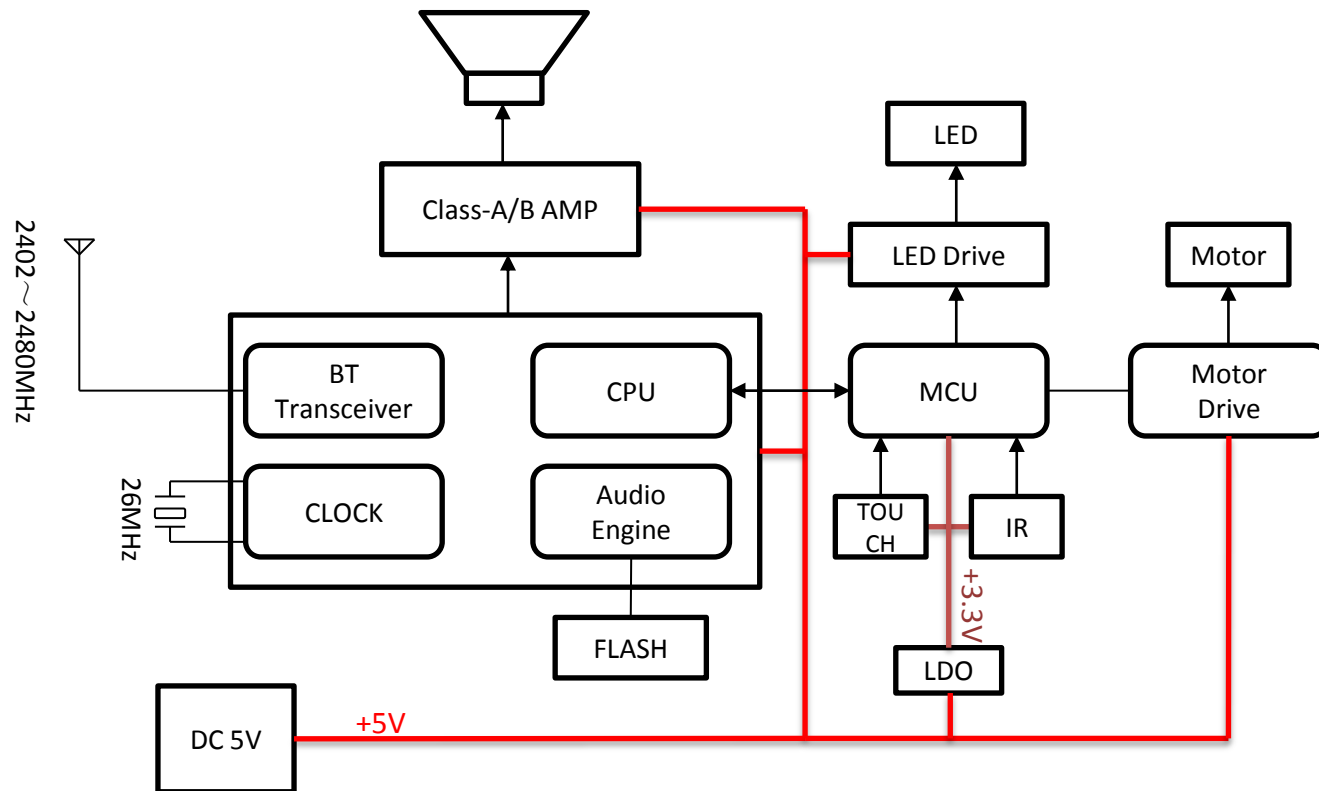
Block Diagram
