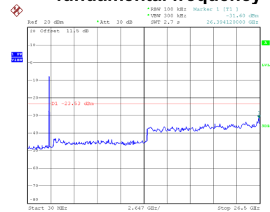
CH78 – 10th Harmonic of the fundamental frequency
