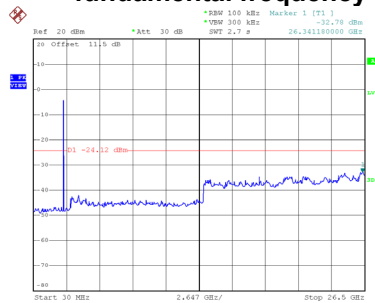
CH38 – 10th Harmonic of the fundamental frequency
