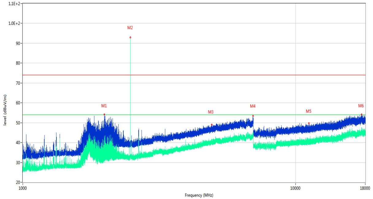
RE Test case_FCC Part 15C_FCC 15.247(24G)_1GHz-18GHz
