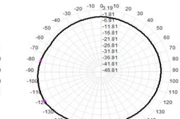
2400.0MHz Total(H), Max= -1.62dBi
