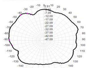
2470.0MHz Total(E2), Max= 2.29dBi
